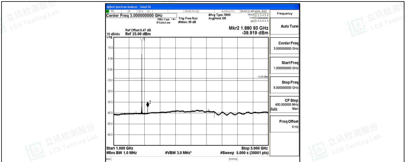
Band4-5MHz-16QAM-20175-1-0-Low-1000-5000--39.92-PASS
