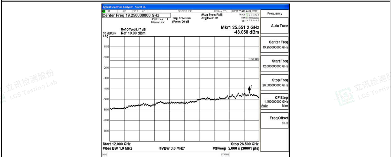
Band4-1.4MHz-QPSK-19957-1-0-Low-12000-26500--43.06-PASS
