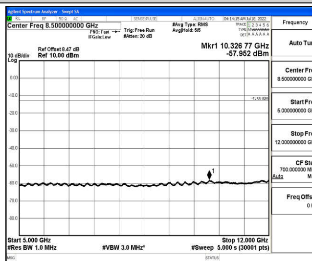
Band4-3MHz-16QAM-20385-1-0-High-5000-12000--57.95-PASS
