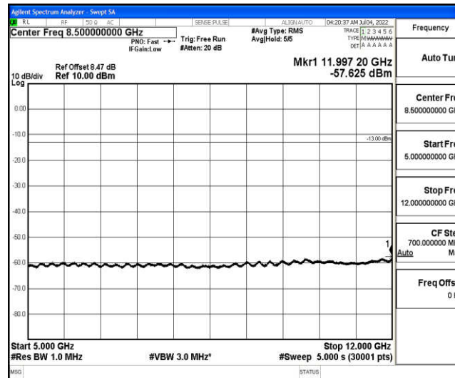
Band4-3MHz-QPSK-20175-1-0-Low-5000-12000--57.63-PASS
