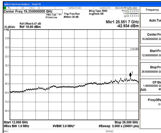
Band4-10MHz-16QAM-20000-1-0-Low-12000-26500--42.93-PASS
