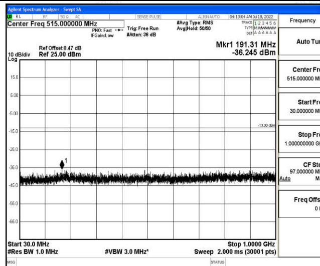
Band4-3MHz-16QAM-20385-1-0-High-30-1000--36.25-PASS
