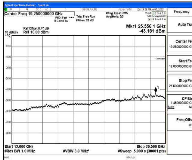
Band4-10MHz-QPSK-20000-1-0-Low-12000-26500--43.18-PASS
