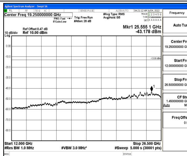
Band4-3MHz-QPSK-20175-1-0-Low-12000-26500--43.18-PASS
