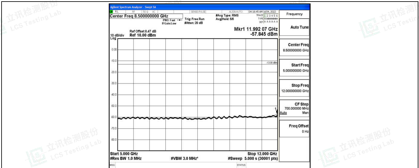
Band4-3MHz-QPSK-19965-1-0-Low-5000-12000--57.85-PASS
