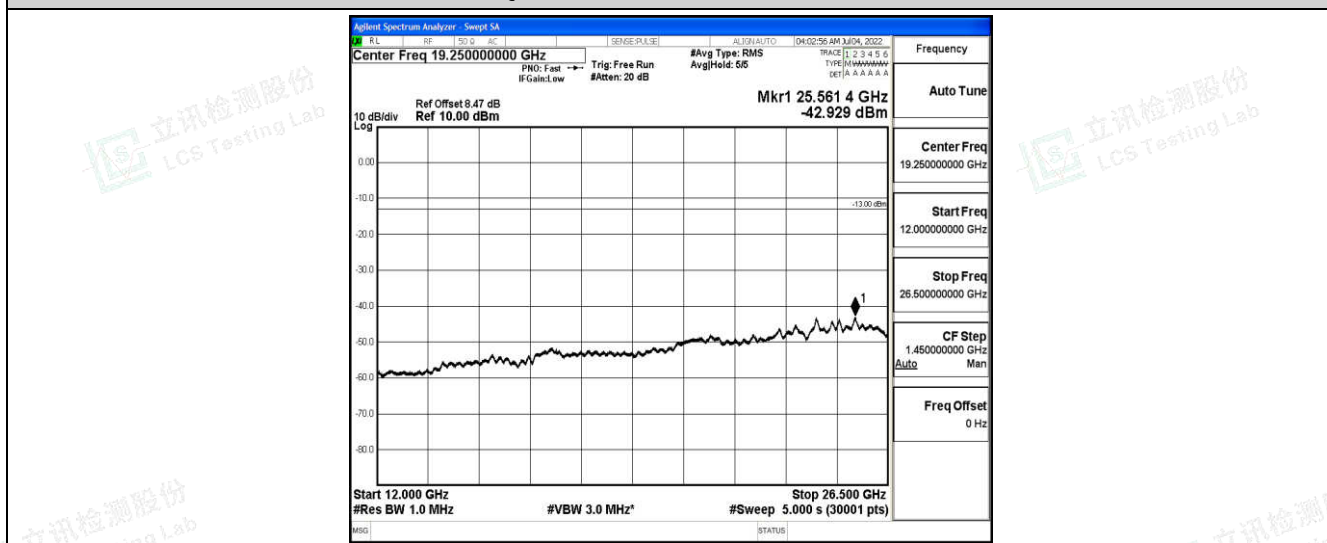
Band4-1.4MHz-16QAM-20175-1-0-Low-12000-26500--42.93-PASS
