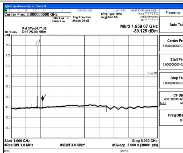
Band4-5MHz-QPSK-19975-1-0-Low-1000-5000--39.13-PASS
