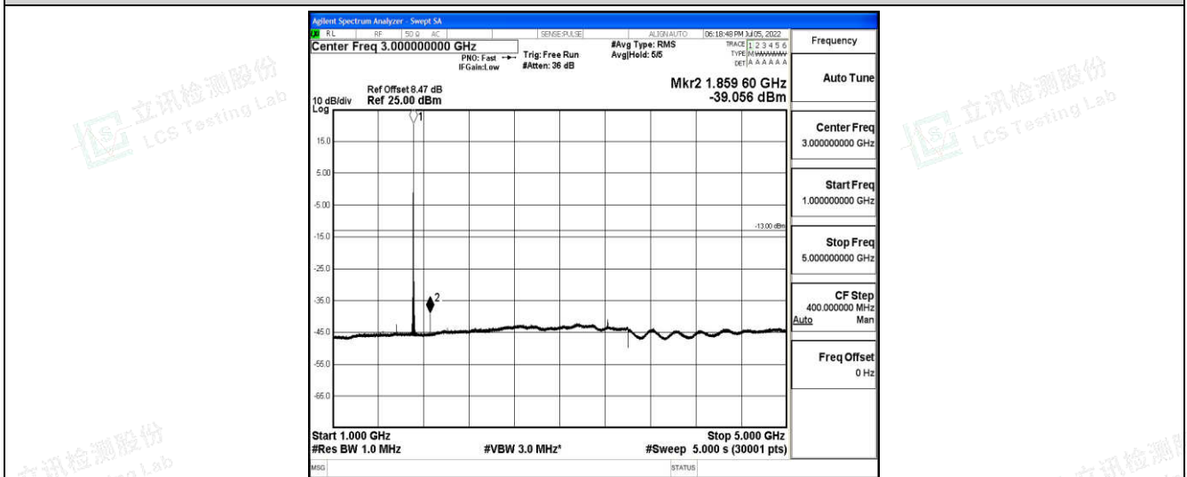
Band4-10MHz-QPSK-20000-1-0-Low-1000-5000--39.06-PASS
