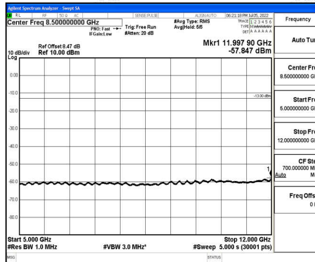
Band4-10MHz-16QAM-20000-1-0-Low-5000-12000--57.85-PASS
