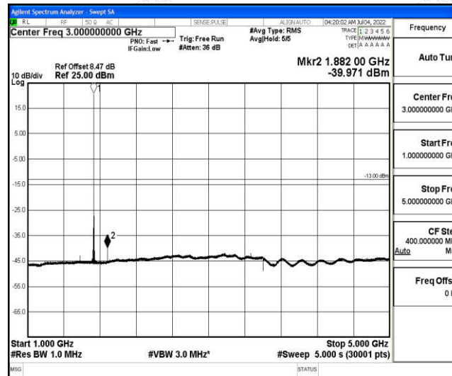
Band4-3MHz-QPSK-20175-1-0-Low-1000-5000--39.97-PASS
