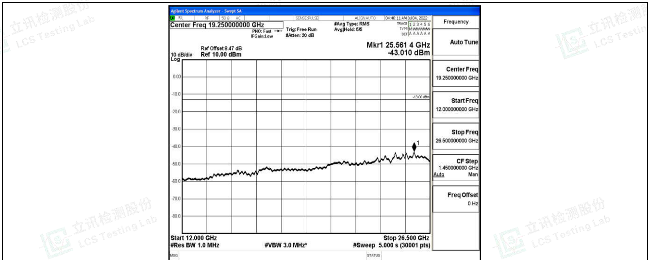
Band4-5MHz-16QAM-20375-1-0-High-12000-26500--43.01-PASS
