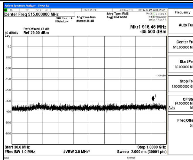
Band4-5MHz-QPSK-19975-1-0-Low-30-1000--35.5-PASS
