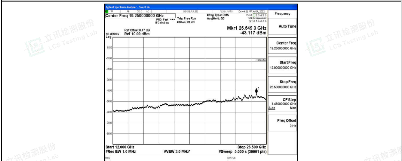
Band4-5MHz-16QAM-20175-1-0-Low-12000-26500--43.12-PASS
