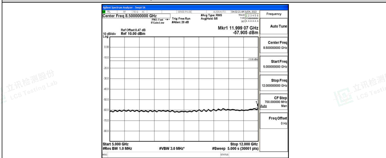
Band4-1.4MHz-16QAM-20175-1-0-Low-5000-12000--57.91-PASS
