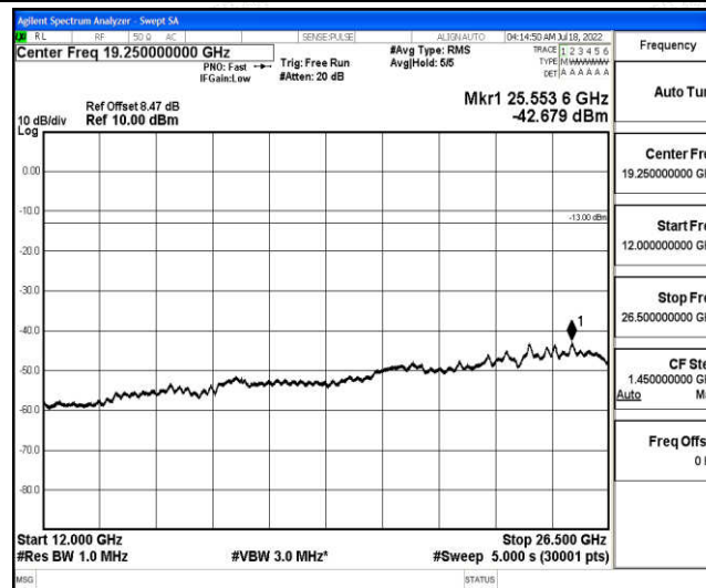
Band4-3MHz-16QAM-20385-1-0-High-12000-26500--42.68-PASS
