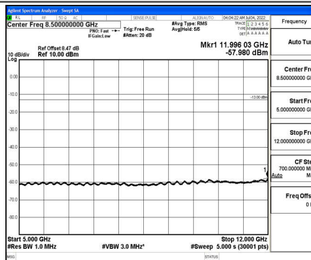
Band4-1.4MHz-QPSK-20393-1-0-High-5000-12000--57.98-PASS
