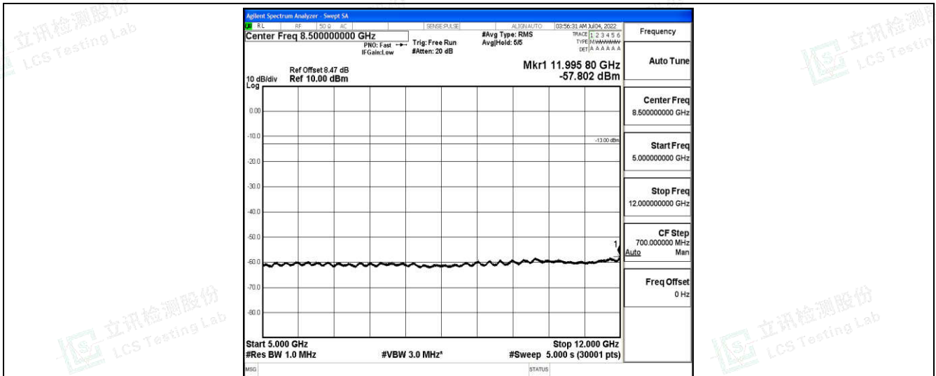
Band4-1.4MHz-QPSK-19957-1-0-Low-5000-12000--57.8-PASS
