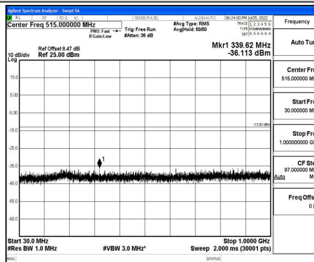
Band4-10MHz-16QAM-20175-1-0-Low-30-1000--36.11-PASS
