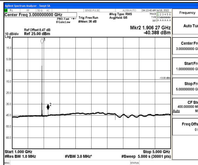
Band4-3MHz-16QAM-20385-1-0-High-1000-5000--40.39-PASS
