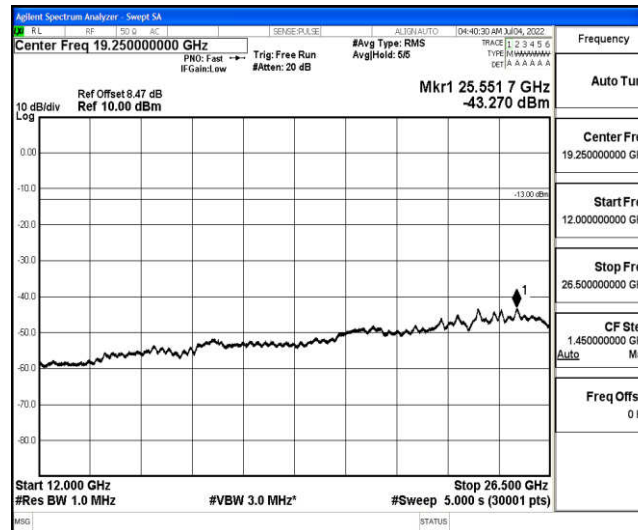
Band4-5MHz-16QAM-19975-1-0-Low-12000-26500--43.27-PASS
