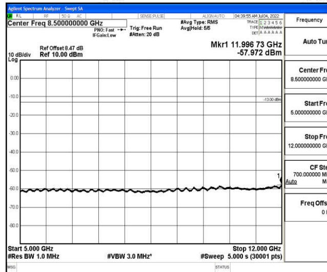
Band4-5MHz-16QAM-19975-1-0-Low-5000-12000--57.97-PASS
