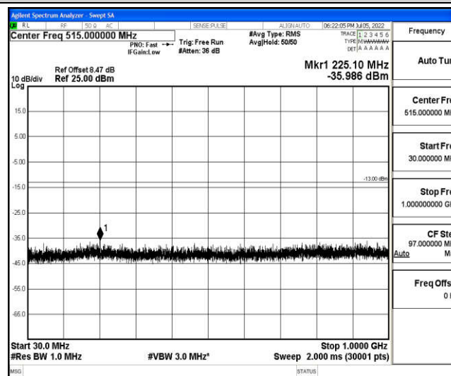
Band4-10MHz-QPSK-20175-1-0-Low-30-1000--35.99-PASS
