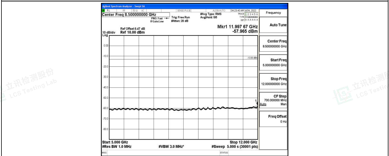
Band4-3MHz-16QAM-20175-1-0-Low-5000-12000--57.97-PASS
