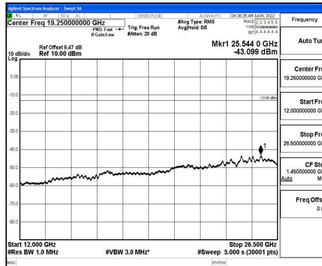
Band4-5MHz-QPSK-19975-1-0-Low-12000-26500--43.1-PASS
