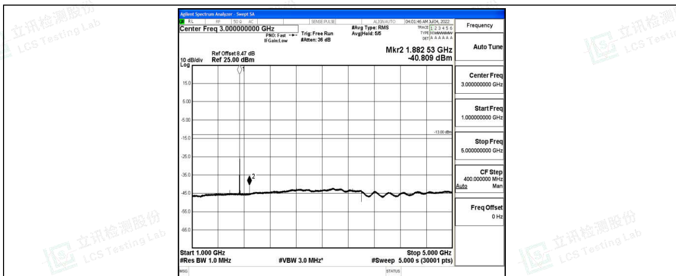
Band4-1.4MHz-16QAM-20175-1-0-Low-1000-5000--40.81-PASS
