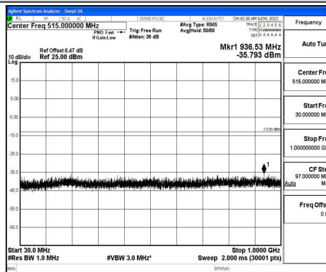
Band4-5MHz-16QAM-20175-1-0-Low-30-1000--35.79-PASS
