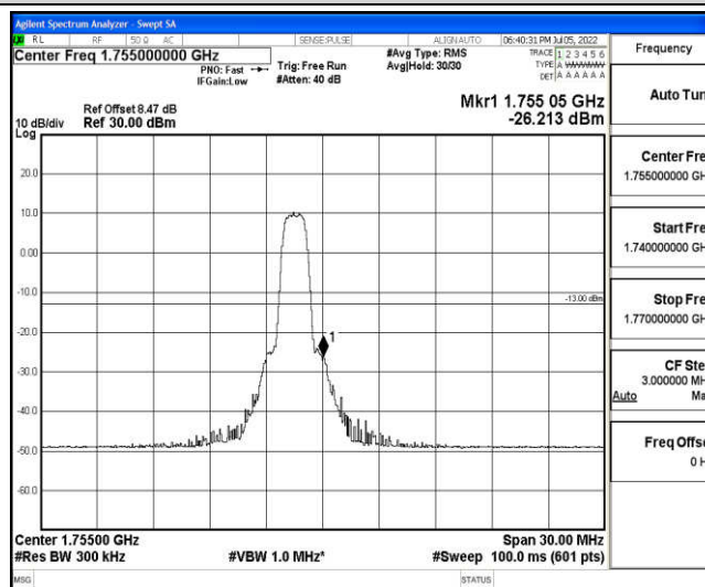
Band4-15MHz-16QAM-20325-6-0-High--26.21-PASS
