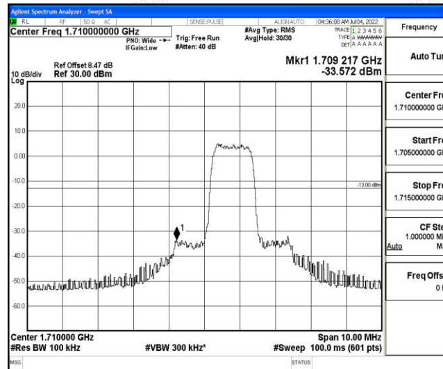
Band4-5MHz-QPSK-19975-6-0-Low--33.57-PASS
