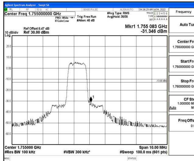
Band4-5MHz-QPSK-20375-6-0-High--31.35-PASS
