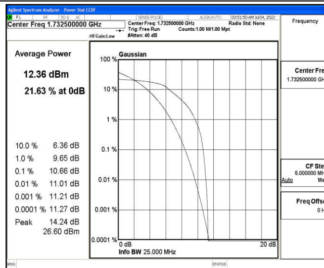
Band4-1.4MHz-QPSK-20175-6-0-Low-10.66-&lt;=13-PASS
