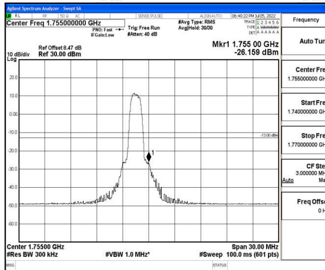
Band4-15MHz-QPSK-20325-6-0-High--26.16-PASS
