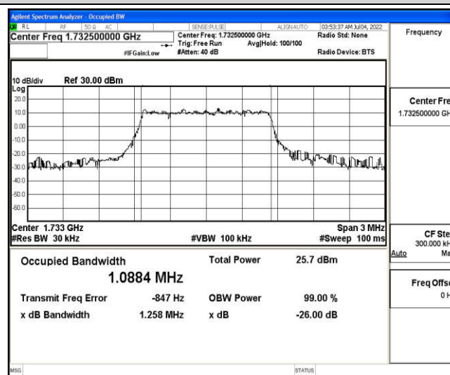
Band4-1.4MHz-16QAM-20175-6-0-Low-1.0884-1.258-PASS
