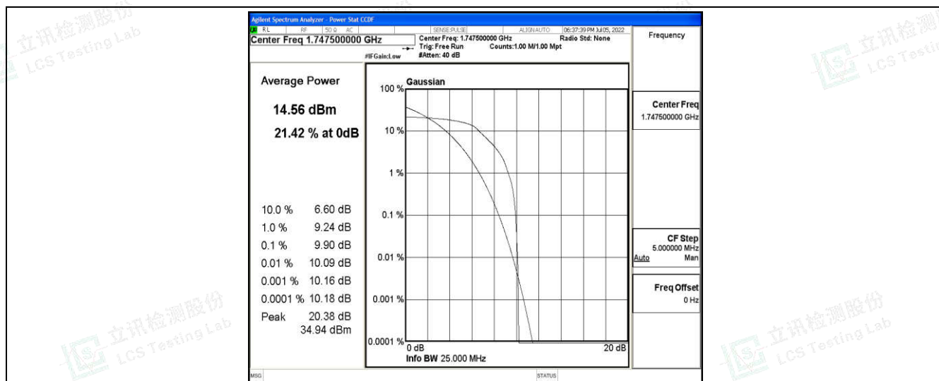
Band4-15MHz-QPSK-20325-6-0-High-9.90-&lt;=13-PASS
