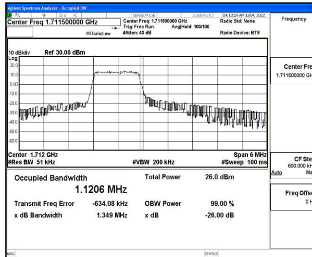
Band4-3MHz-16QAM-19965-6-0-Low-1.1206-1.349-PASS
