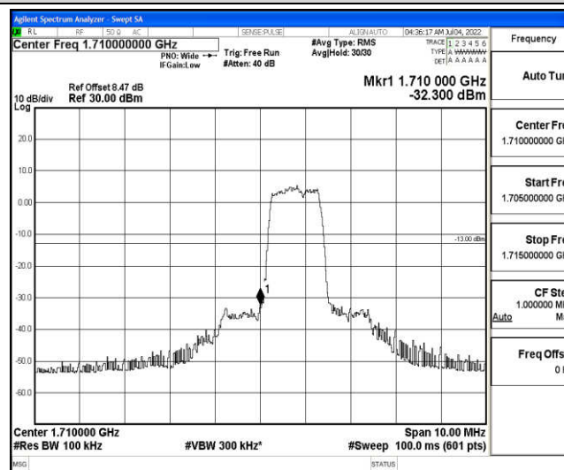
Band4-5MHz-16QAM-19975-6-0-Low--32.30-PASS
