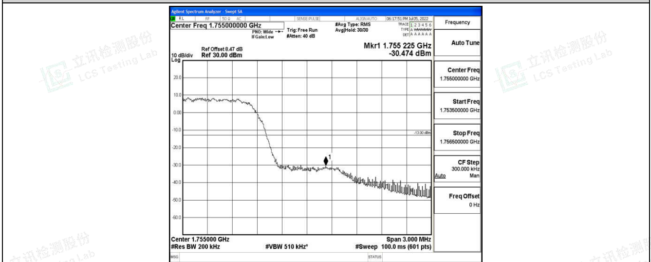
Band4-10MHz-QPSK-20350-6-0-High--30.47-PASS
