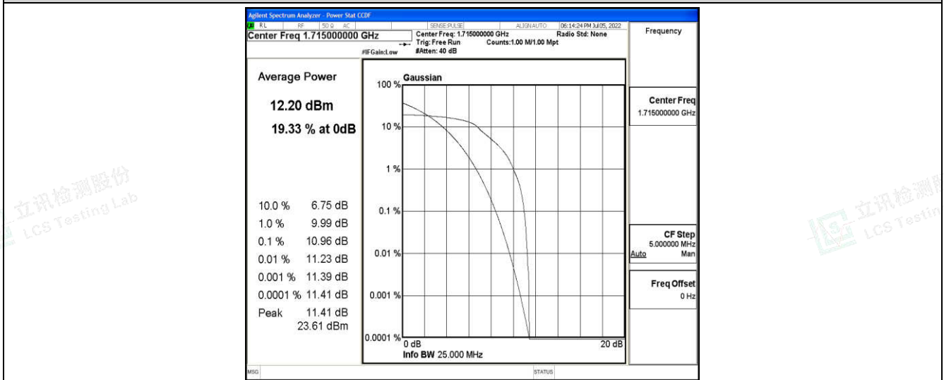
Band4-10MHz-QPSK-20000-6-0-Low-10.96-&lt;=13-PASS
