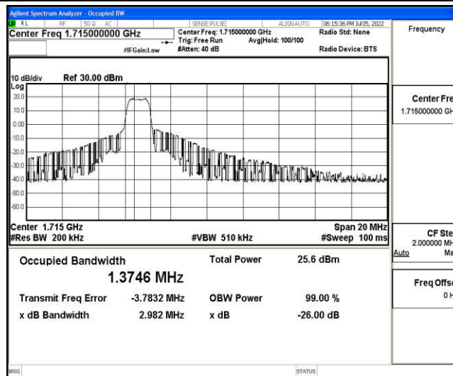
Band4-10MHz-QPSK-20000-6-0-Low-1.3746-2.982-PASS
