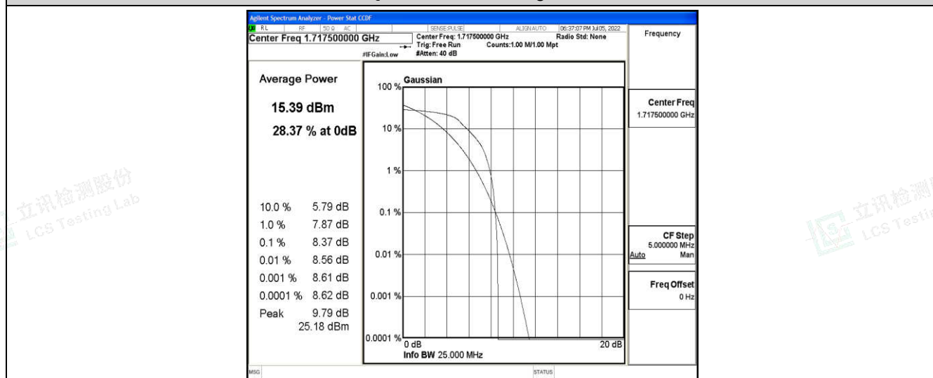
Band4-15MHz-16QAM-20025-6-0-Low-8.37-&lt;=13-PASS
