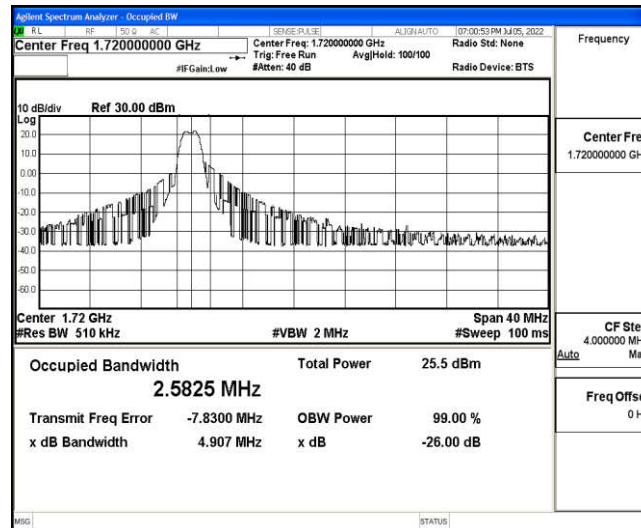
Band4-20MHz-16QAM-20050-6-0-Low-2.5825-4.907-PASS
