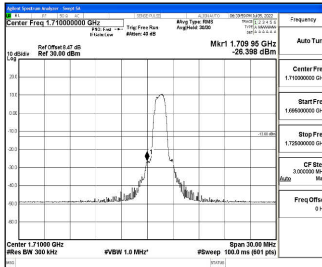
Band4-15MHz-16QAM-20025-6-0-Low--26.40-PASS
