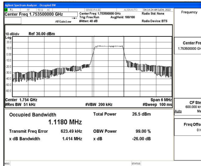
Band4-3MHz-QPSK-20385-6-0-High-1.1180-1.414-PASS
