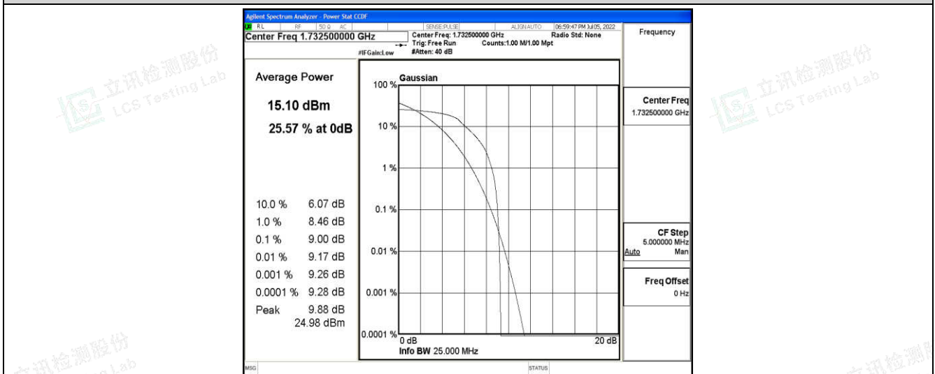
Band4-20MHz-QPSK-20175-6-0-Low-9.00-&lt;=13-PASS
