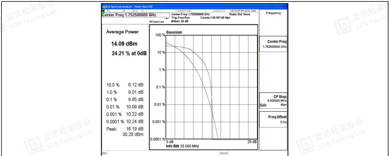
Band4-5MHz-16QAM-20375-6-0-High-9.85-&lt;=13-PASS
