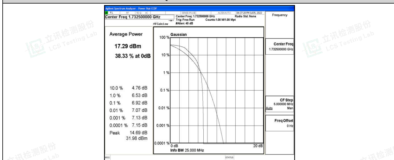
Band4-15MHz-16QAM-20175-6-0-Low-6.92-&lt;=13-PASS
