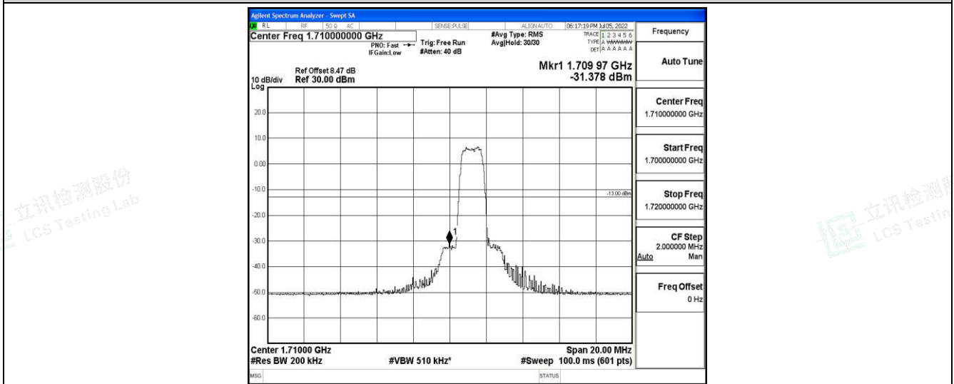
Band4-10MHz-QPSK-20000-6-0-Low--31.38-PASS
