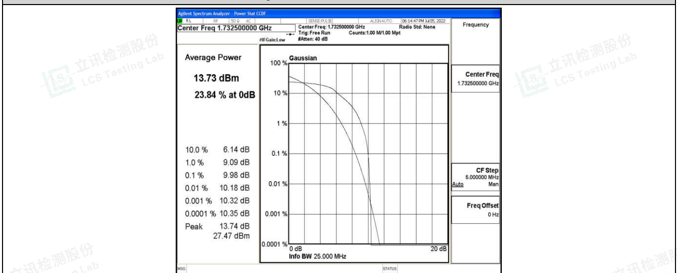
Band4-10MHz-QPSK-20175-6-0-Low-9.98-&lt;=13-PASS
