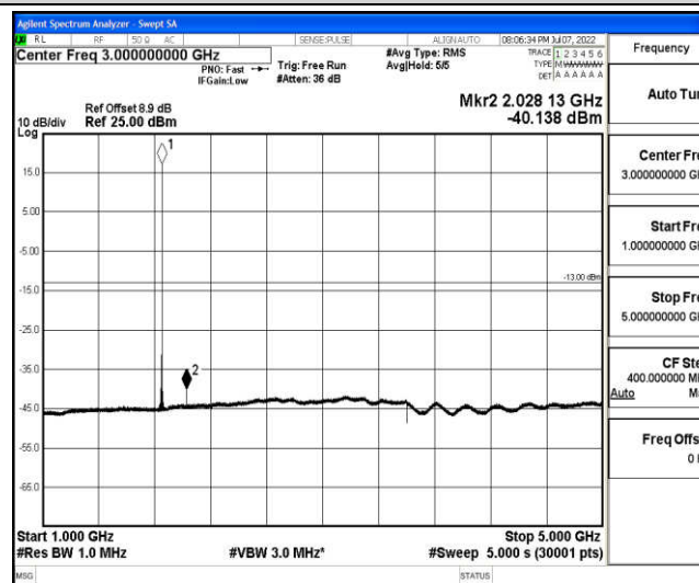
Band2-20MHz-QPSK-18700-1-0-Low-1000-5000--40.14-PASS
