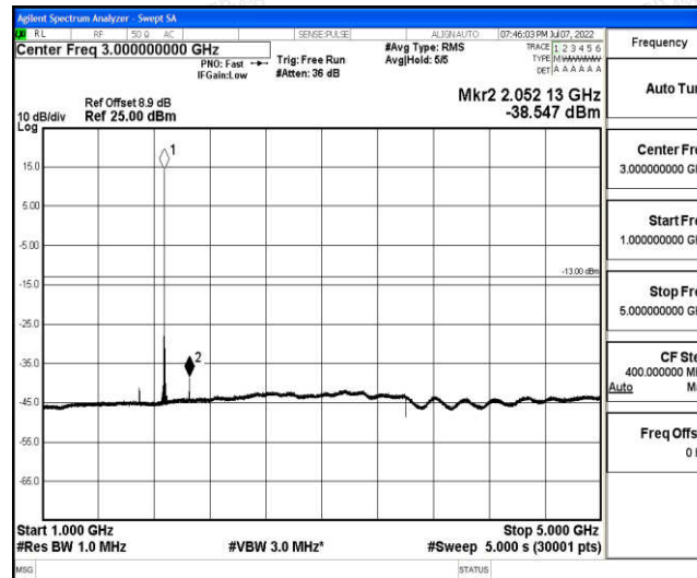
Band2-15MHz-16QAM-18900-1-0-Low-1000-5000--38.55-PASS
