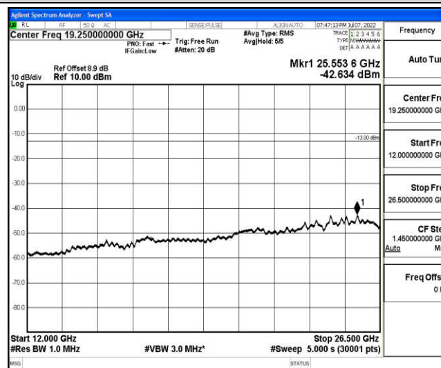
Band2-15MHz-16QAM-18900-1-0-Low-12000-26500--42.63-PASS
