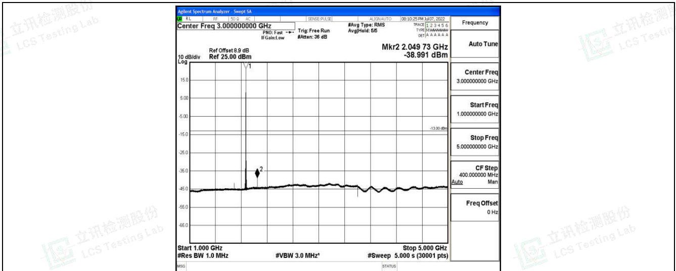
Band2-20MHz-QPSK-18900-1-0-Low-1000-5000--38.99-PASS
