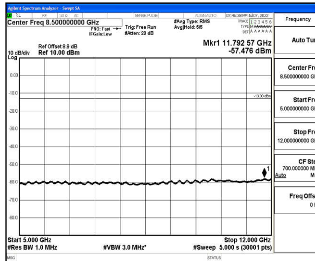
Band2-15MHz-16QAM-18900-1-0-Low-5000-12000--57.48-PASS
