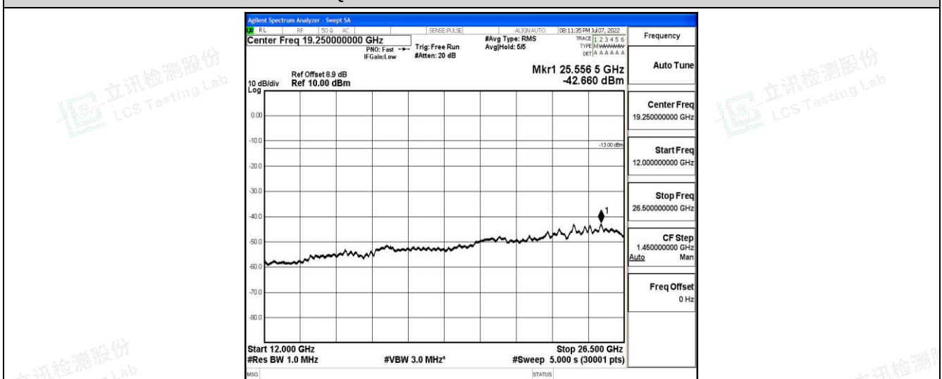
Band2-20MHz-QPSK-18900-1-0-Low-12000-26500--42.66-PASS
