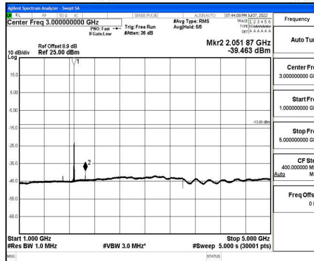
Band2-15MHz-QPSK-18900-1-0-Low-1000-5000--39.46-PASS
