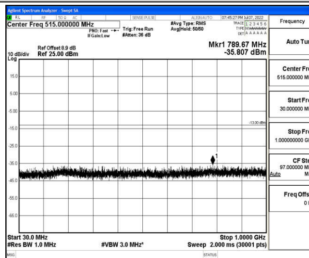
Band2-15MHz-16QAM-18900-1-0-Low-30-1000--35.81-PASS
