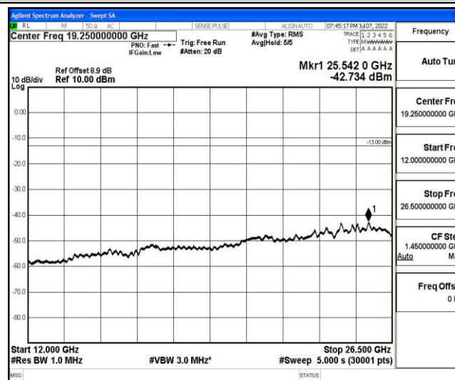
Band2-15MHz-QPSK-18900-1-0-Low-12000-26500--42.73-PASS
