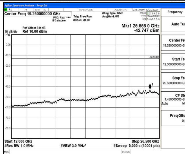
Band2-15MHz-16QAM-19125-1-0-High-12000-26500--42.75-PASS
