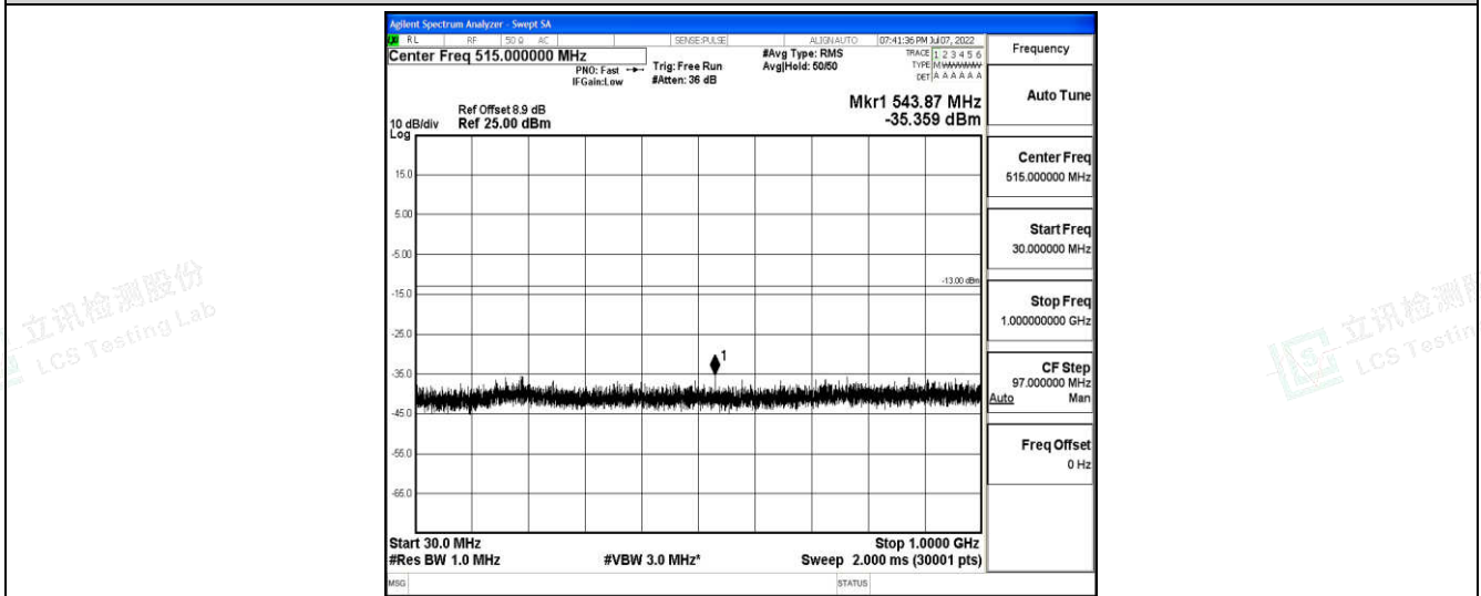
Band2-15MHz-16QAM-18675-1-0-Low-30-1000--35.36-PASS
