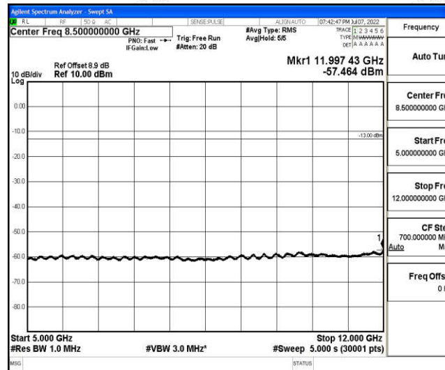
Band2-15MHz-16QAM-18675-1-0-Low-5000-12000--57.46-PASS
