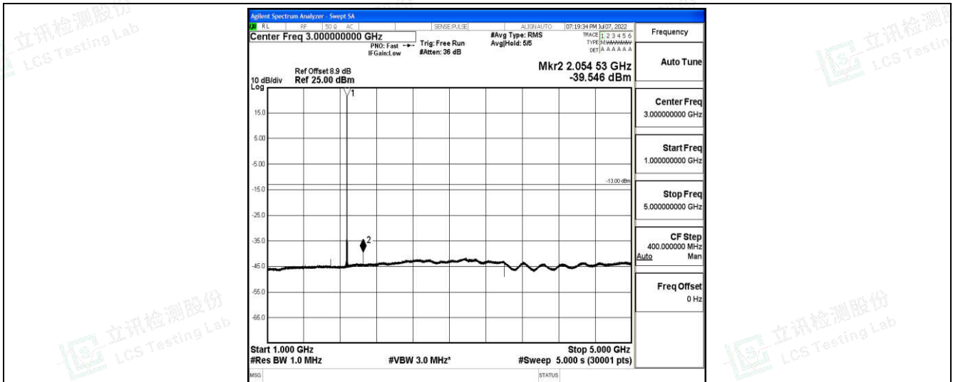
Band2-10MHz-QPSK-18900-1-0-Low-1000-5000--39.55-PASS
