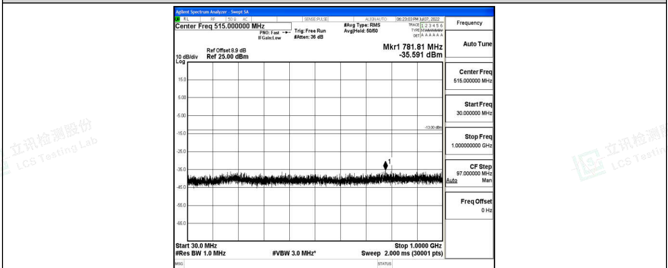
Band2-3MHz-16QAM-18615-1-0-Low-30-1000--35.59-PASS
