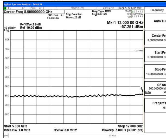
Band2-5MHz-16QAM-18625-1-0-Low-5000-12000--57.25-PASS
