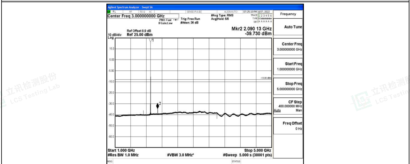
Band2-10MHz-16QAM-19150-1-0-High-1000-5000--39.73-PASS
