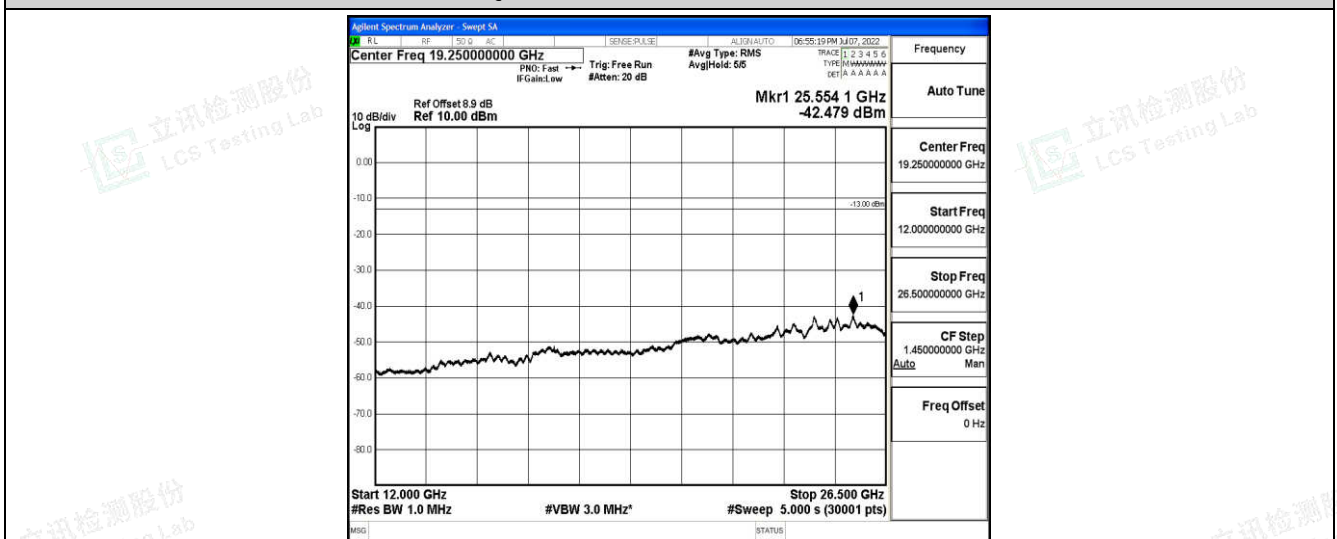
Band2-5MHz-16QAM-18900-1-0-Low-12000-26500--42.48-PASS
