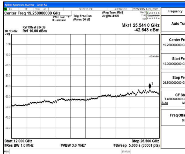
Band2-1.4MHz-QPSK-18607-1-0-Low-12000-26500--42.64-PASS
