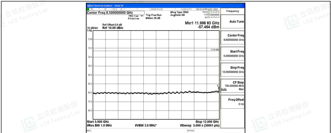
Band2-3MHz-QPSK-18615-1-0-Low-5000-12000--57.46-PASS
