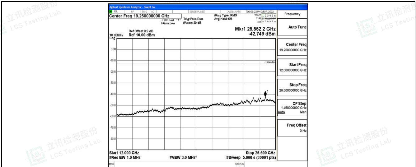
Band2-1.4MHz-16QAM-19193-1-0-High-12000-26500--42.75-PASS
