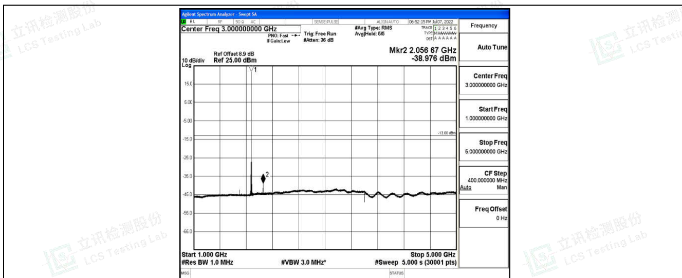
Band2-5MHz-QPSK-18900-1-0-Low-1000-5000--38.98-PASS
