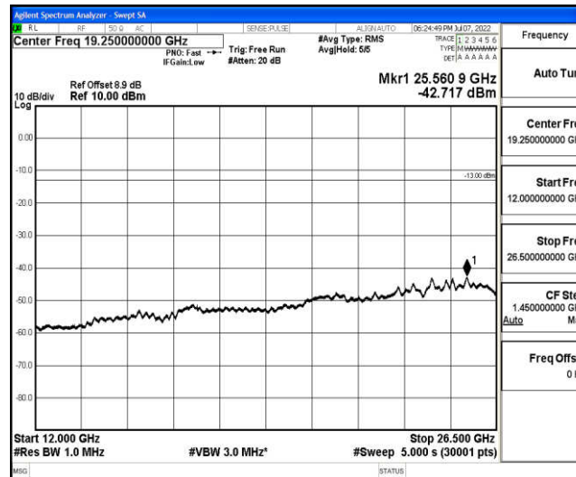
Band2-3MHz-16QAM-18615-1-0-Low-12000-26500--42.72-PASS
