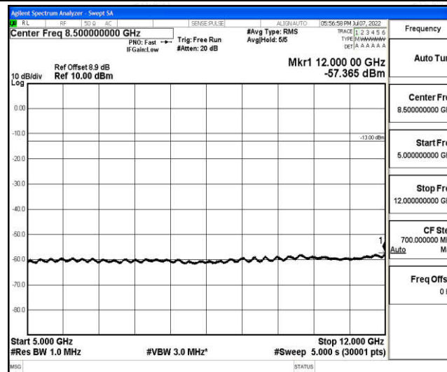
Band2-1.4MHz-16QAM-18607-1-0-Low-5000-12000--57.37-PASS
