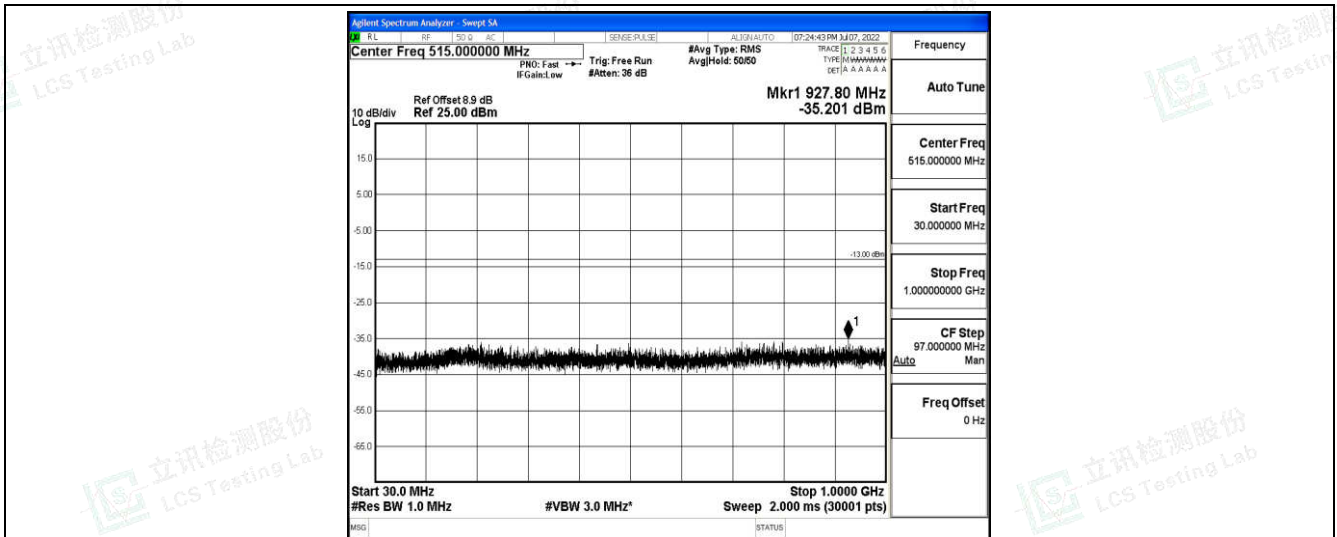
Band2-10MHz-16QAM-19150-1-0-High-30-1000--35.2-PASS
