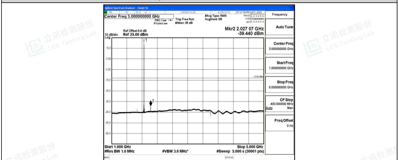
Band2-10MHz-16QAM-18650-1-0-Low-1000-5000--39.44-PASS
