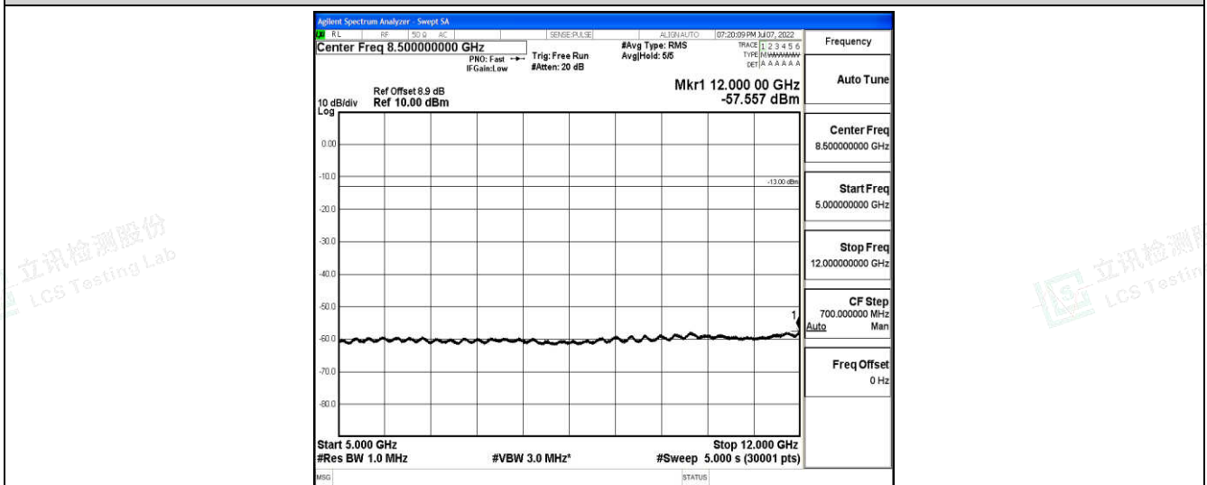
Band2-10MHz-QPSK-18900-1-0-Low-5000-12000--57.56-PASS
