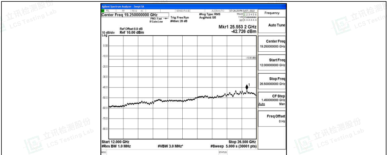
Band2-10MHz-16QAM-19150-1-0-High-12000-26500--42.73-PASS
