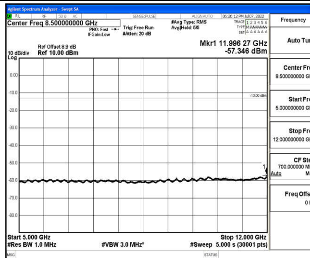
Band2-3MHz-QPSK-18900-1-0-Low-5000-12000--57.35-PASS
