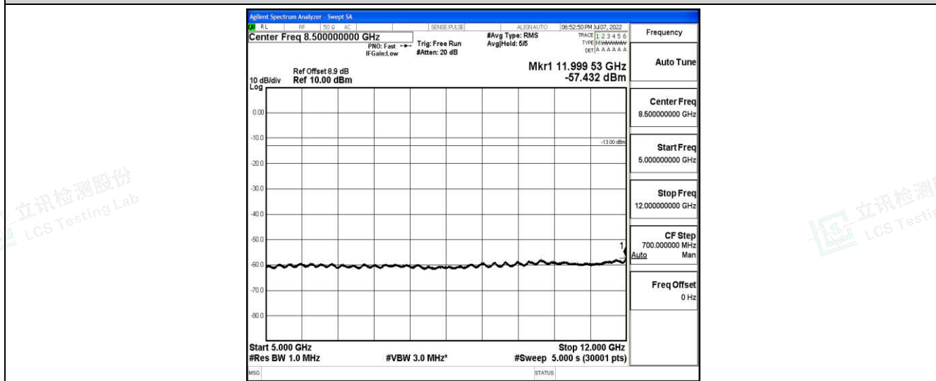
Band2-5MHz-QPSK-18900-1-0-Low-5000-12000--57.43-PASS
