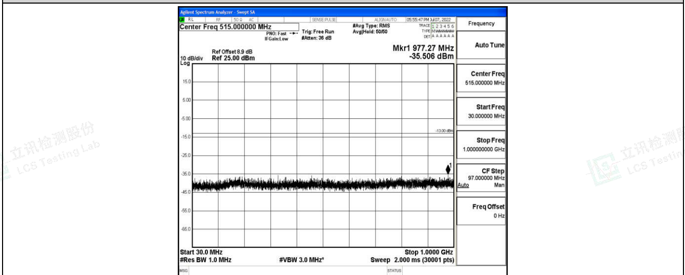
Band2-1.4MHz-16QAM-18607-1-0-Low-30-1000--35.51-PASS
