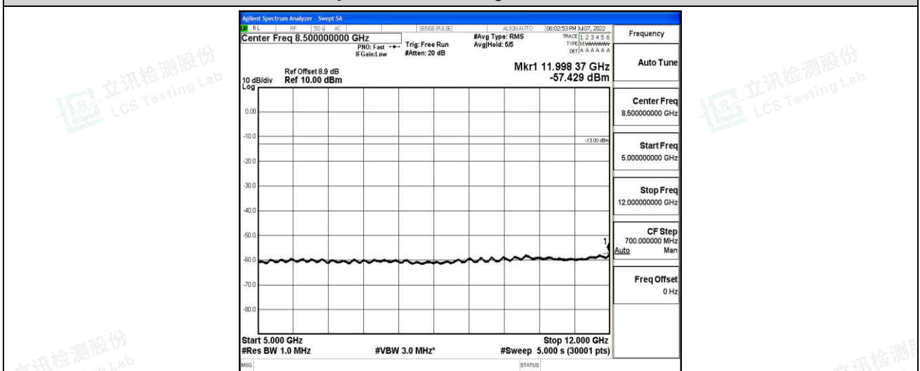
Band2-1.4MHz-QPSK-19193-1-0-High-5000-12000--57.43-PASS
