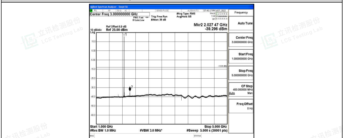
Band2-15MHz-QPSK-18675-1-0-Low-1000-5000--39.3-PASS
