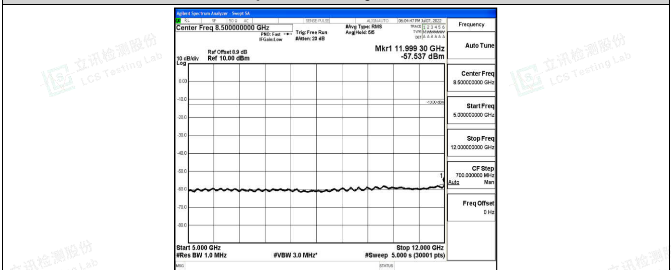
Band2-1.4MHz-16QAM-19193-1-0-High-5000-12000--57.54-PASS
