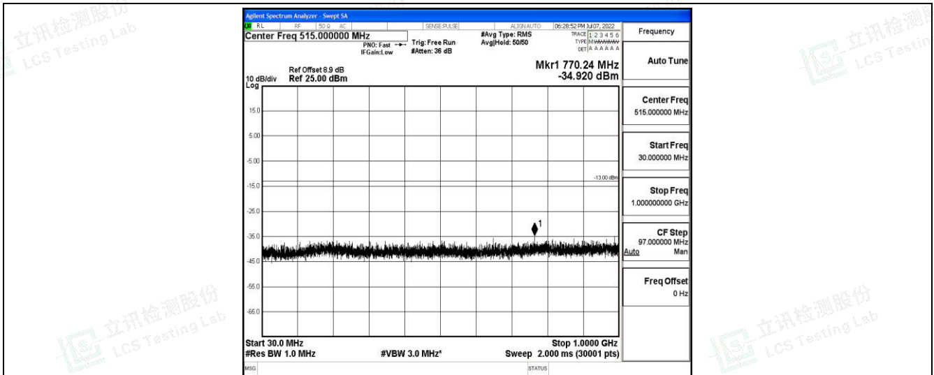
Band2-3MHz-QPSK-19185-1-0-High-30-1000--34.92-PASS
