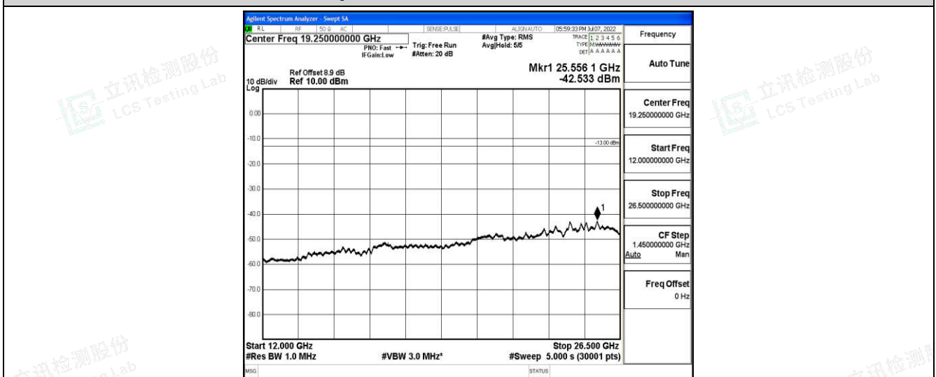
Band2-1.4MHz-QPSK-18900-1-0-Low-12000-26500--42.53-PASS
