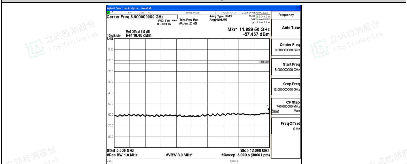
Band2-10MHz-16QAM-19150-1-0-High-5000-12000--57.47-PASS
