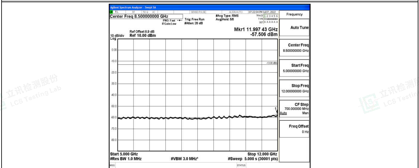
Band2-10MHz-16QAM-18900-1-0-Low-5000-12000--57.51-PASS
