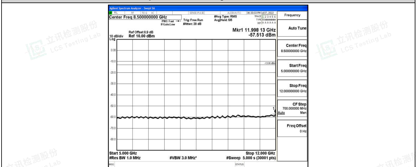
Band2-3MHz-QPSK-19185-1-0-High-5000-12000--57.51-PASS
