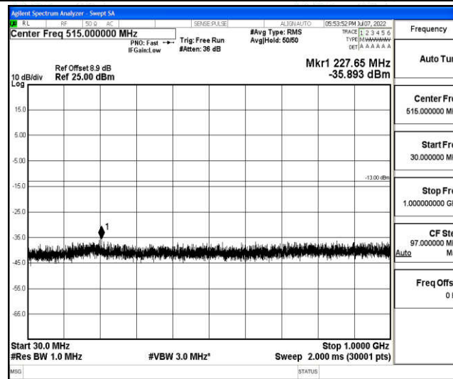
Band2-1.4MHz-QPSK-18607-1-0-Low-30-1000--35.89-PASS
