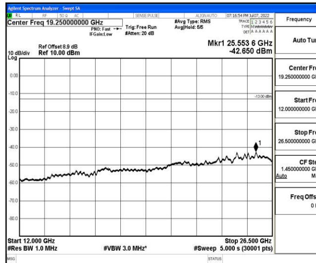
Band2-10MHz-QPSK-18650-1-0-Low-12000-26500--42.65-PASS
