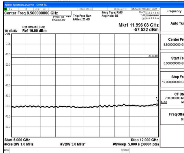
Band2-1.4MHz-QPSK-18607-1-0-Low-5000-12000--57.53-PASS
