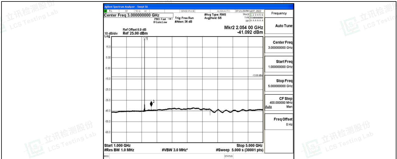
Band2-10MHz-16QAM-18900-1-0-Low-1000-5000--41.09-PASS
