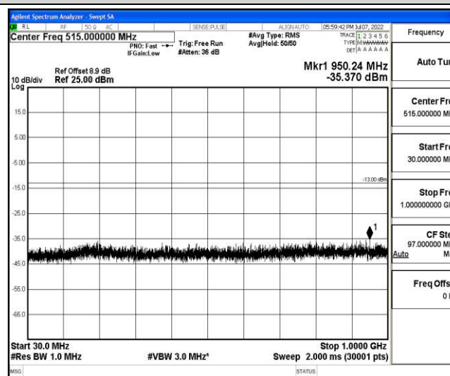
Band2-1.4MHz-16QAM-18900-1-0-Low-30-1000--35.37-PASS
