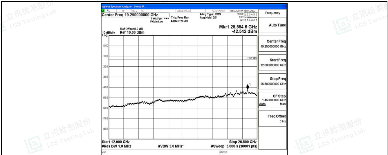
Band2-3MHz-QPSK-19185-1-0-High-12000-26500--42.54-PASS
