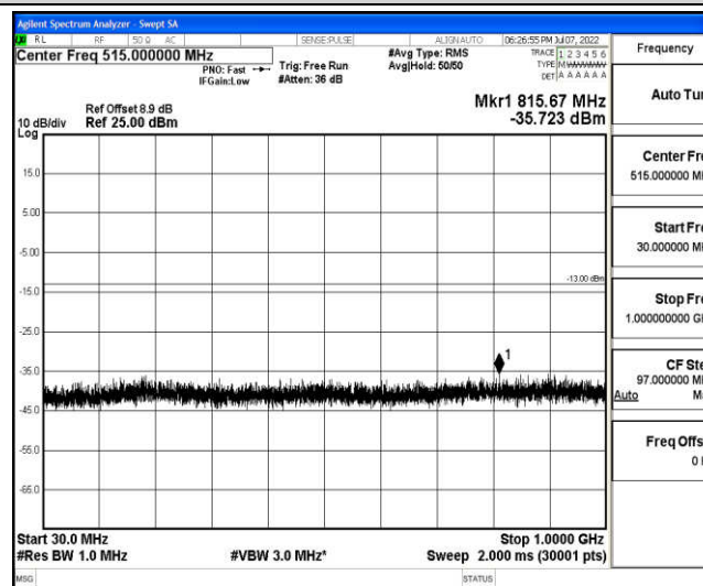
Band2-3MHz-16QAM-18900-1-0-Low-30-1000--35.72-PASS
