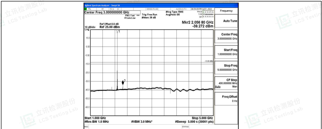
Band2-5MHz-16QAM-18900-1-0-Low-1000-5000--39.27-PASS
