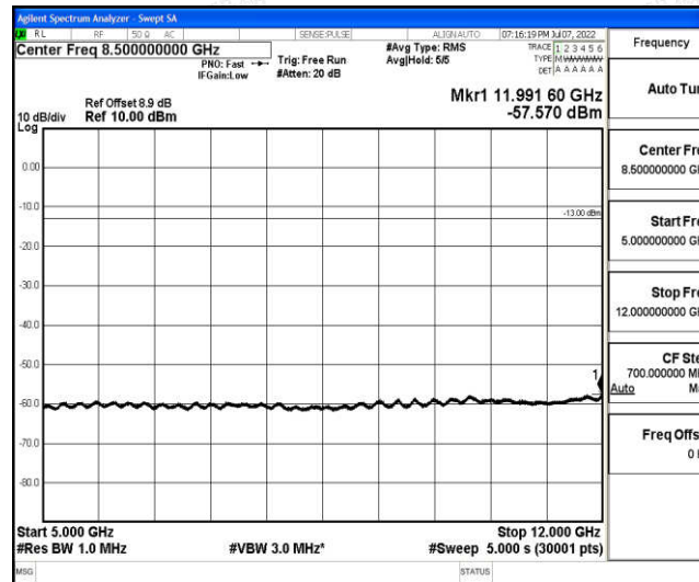
Band2-10MHz-QPSK-18650-1-0-Low-5000-12000--57.57-PASS
