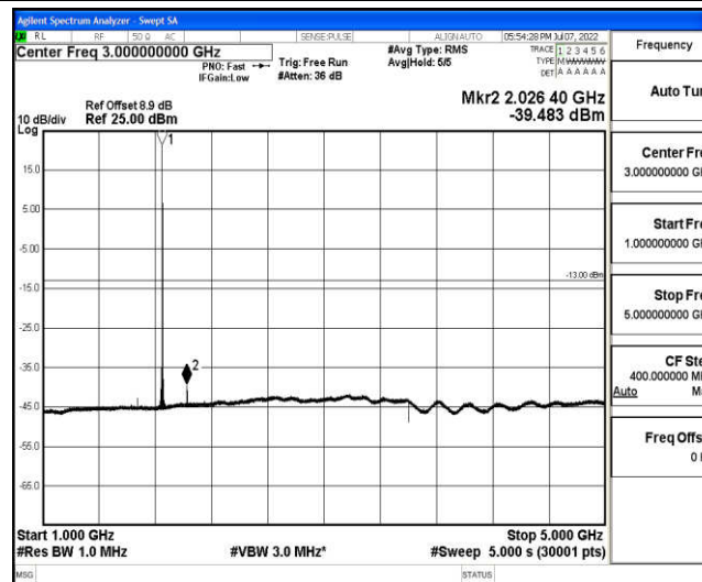
Band2-1.4MHz-QPSK-18607-1-0-Low-1000-5000--39.48-PASS
