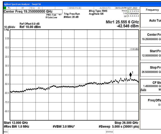
Band2-5MHz-16QAM-18625-1-0-Low-12000-26500--42.55-PASS
