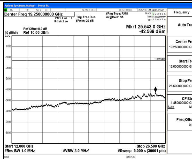
Band2-1.4MHz-16QAM-18607-1-0-Low-12000-26500--42.57-PASS
