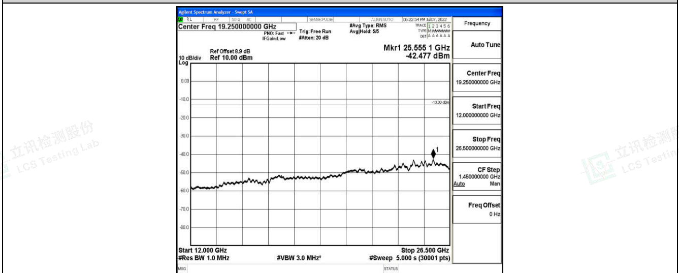
Band2-3MHz-QPSK-18615-1-0-Low-12000-26500--42.48-PASS
