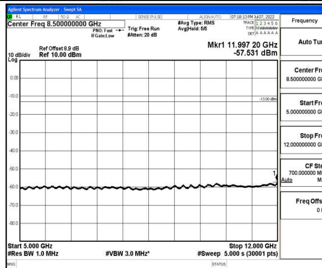
Band2-10MHz-16QAM-18650-1-0-Low-5000-12000--57.53-PASS
