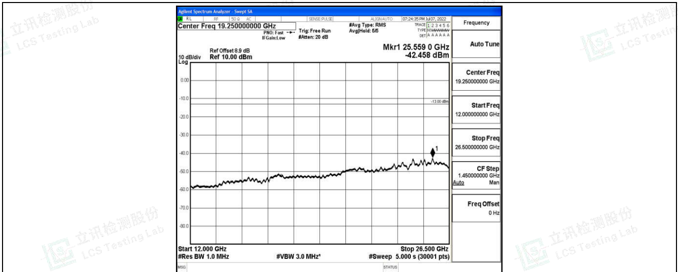
Band2-10MHz-QPSK-19150-1-0-High-12000-26500--42.46-PASS
