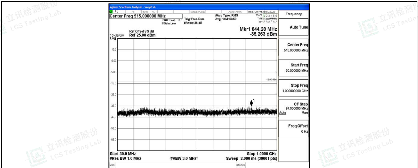
Band2-5MHz-16QAM-19175-1-0-High-30-1000--35.26-PASS
