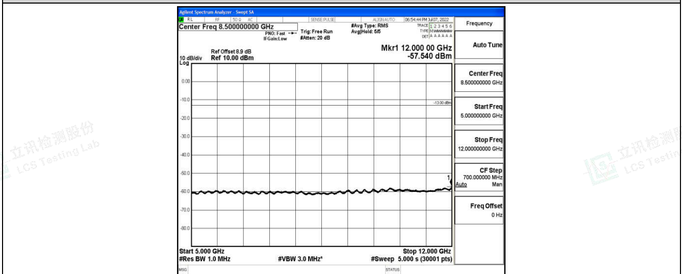
Band2-5MHz-16QAM-18900-1-0-Low-5000-12000--57.54-PASS
