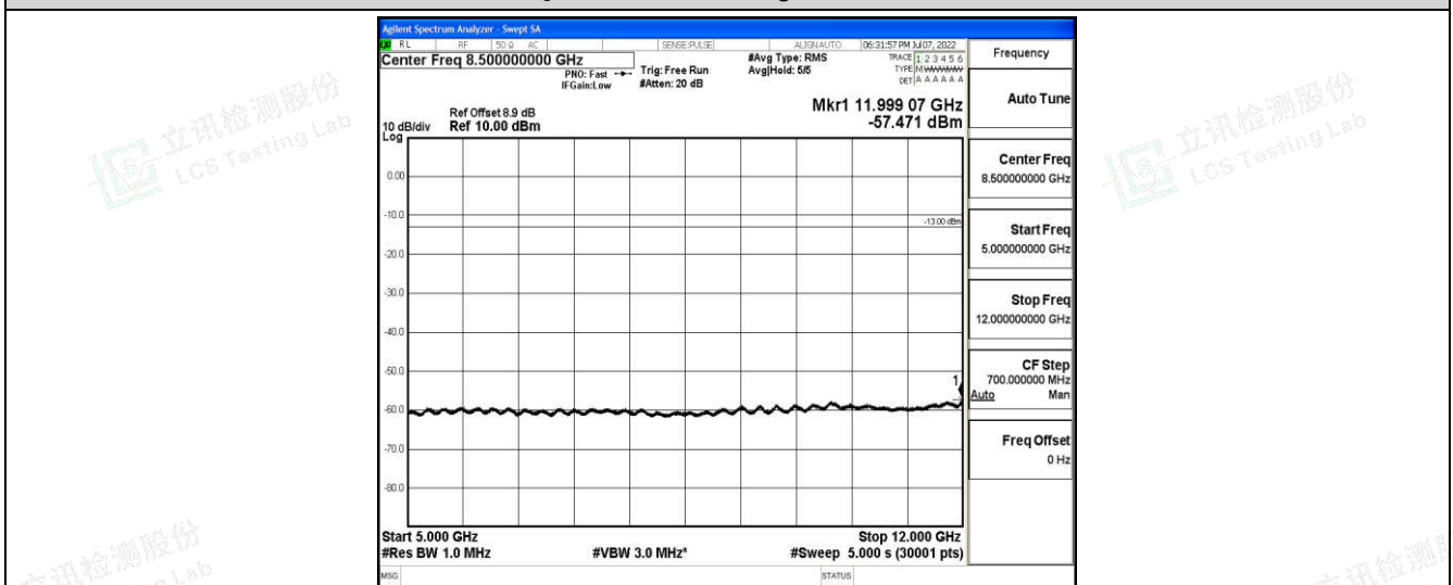
Band2-3MHz-16QAM-19185-1-0-High-5000-12000--57.47-PASS
