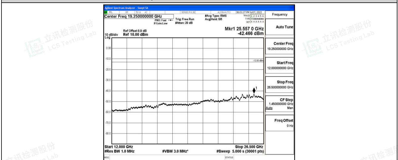
Band2-1.4MHz-16QAM-18900-1-0-Low-12000-26500--42.47-PASS
