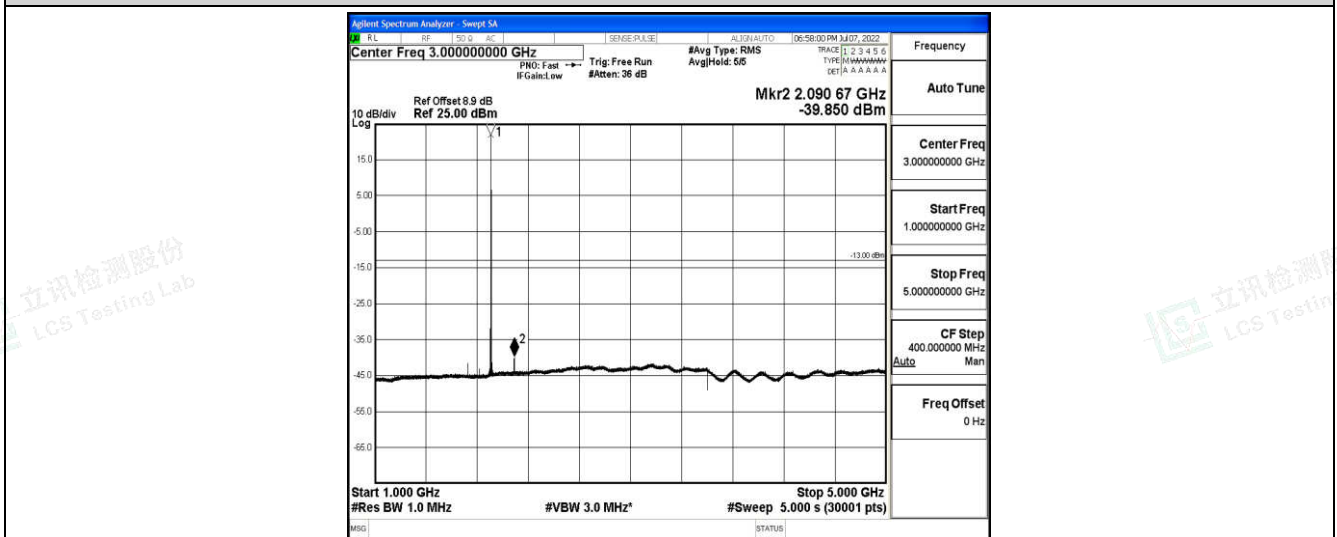
Band2-5MHz-16QAM-19175-1-0-High-1000-5000--39.85-PASS
