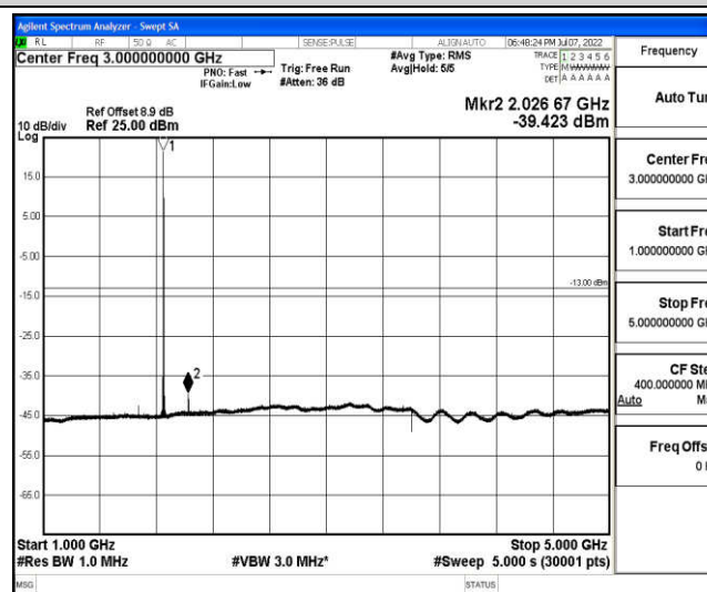
Band2-5MHz-QPSK-18625-1-0-Low-1000-5000--39.42-PASS
