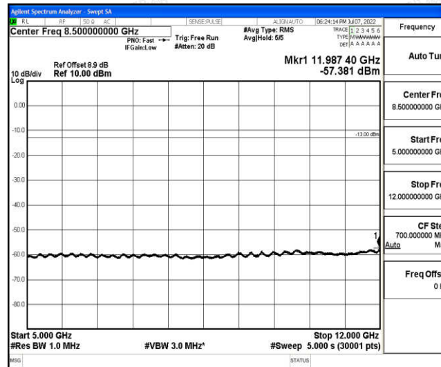
Band2-3MHz-16QAM-18615-1-0-Low-5000-12000--57.38-PASS
