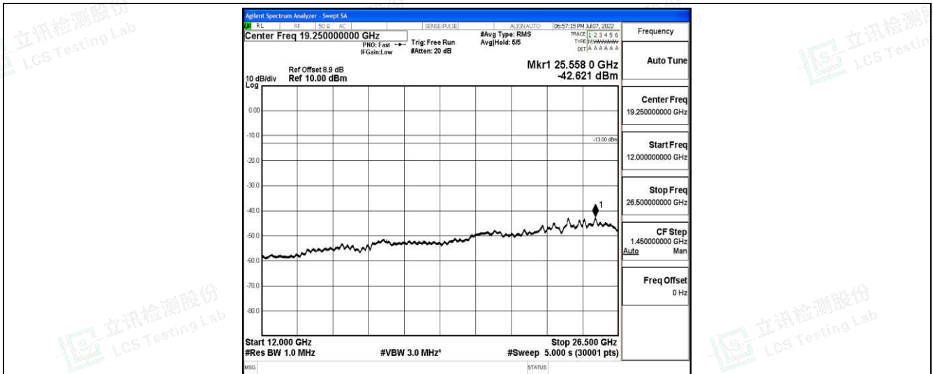
Band2-5MHz-QPSK-19175-1-0-High-12000-26500--42.62-PASS
