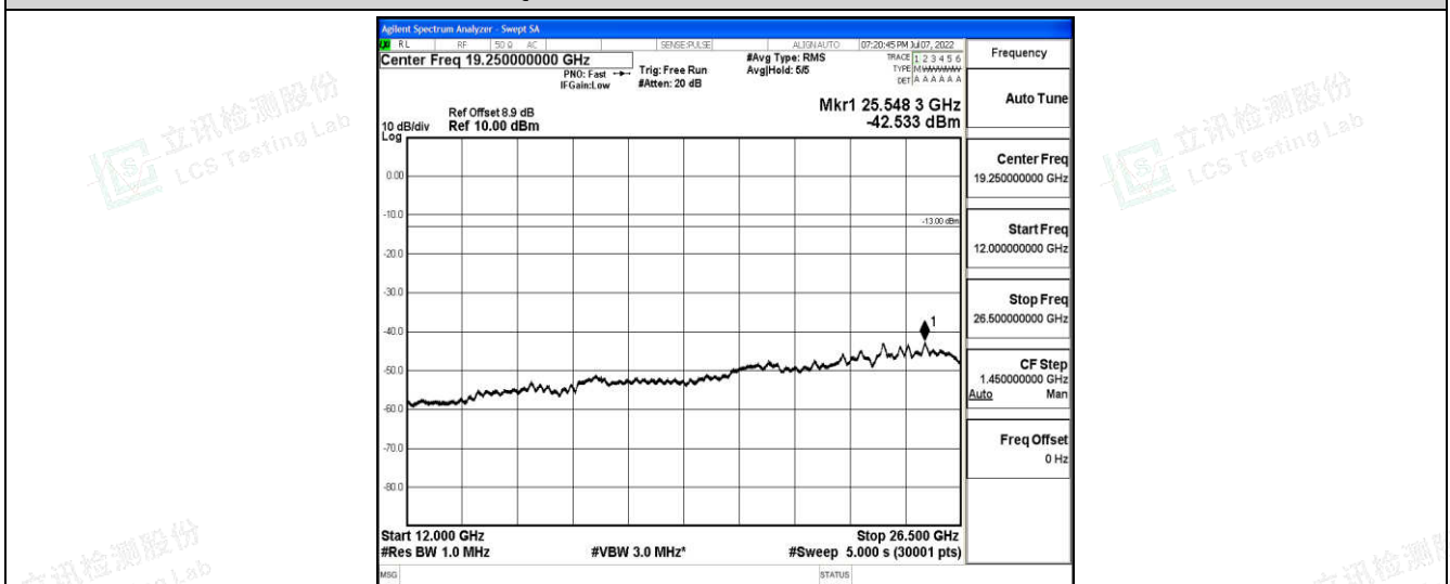
Band2-10MHz-QPSK-18900-1-0-Low-12000-26500--42.53-PASS
