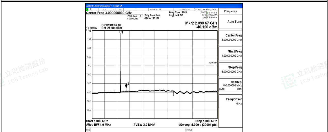
Band2-3MHz-16QAM-19185-1-0-High-1000-5000--40.12-PASS
