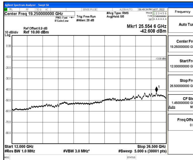
Band2-5MHz-QPSK-18625-1-0-Low-12000-26500--42.61-PASS
