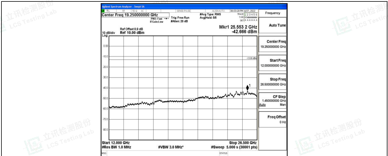
Band2-1.4MHz-QPSK-19193-1-0-High-12000-26500--42.67-PASS
