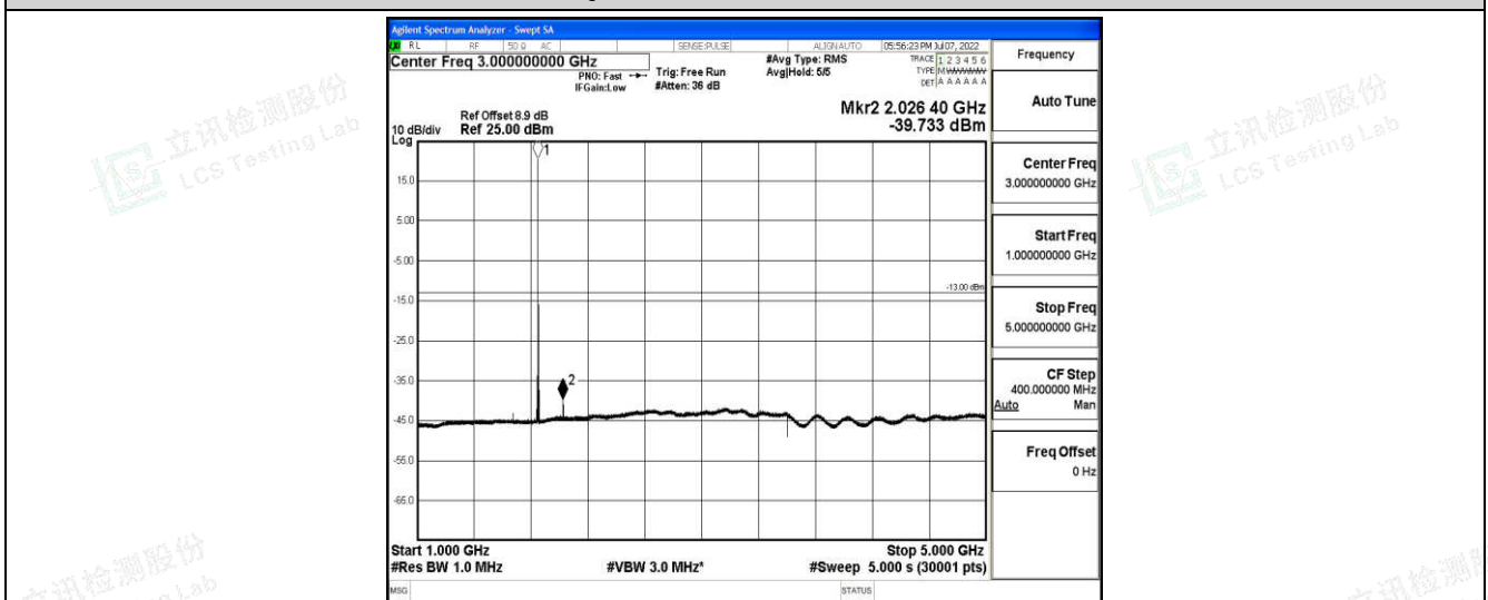
Band2-1.4MHz-16QAM-18607-1-0-Low-1000-5000--39.73-PASS
