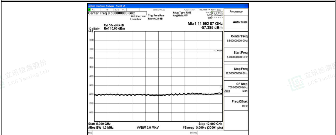
Band2-3MHz-16QAM-18900-1-0-Low-5000-12000--57.39-PASS
