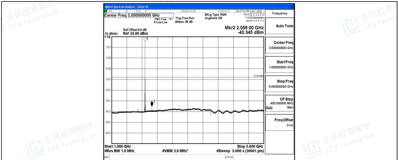
Band2-3MHz-16QAM-18900-1-0-Low-1000-5000--40.35-PASS
