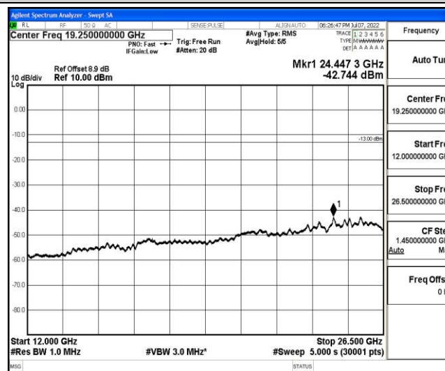
Band2-3MHz-QPSK-18900-1-0-Low-12000-26500--42.74-PASS
