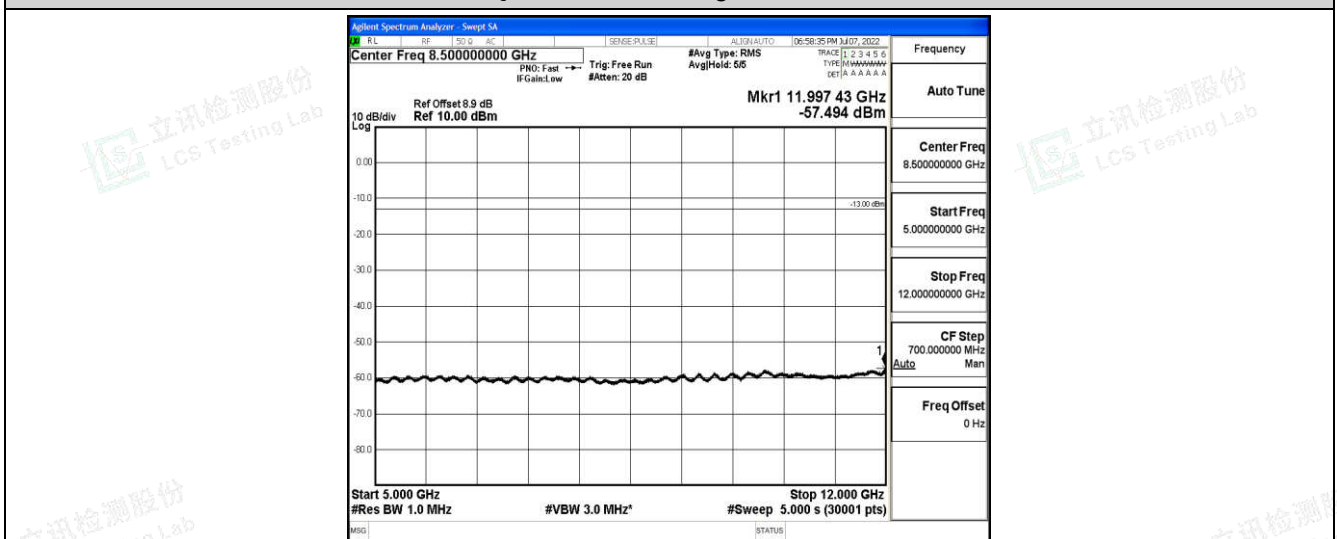
Band2-5MHz-16QAM-19175-1-0-High-5000-12000--57.49-PASS
