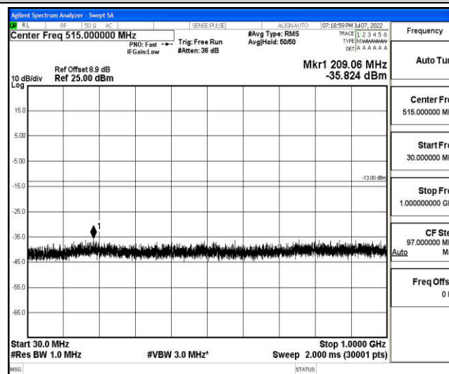
Band2-10MHz-QPSK-18900-1-0-Low-30-1000--35.82-PASS
