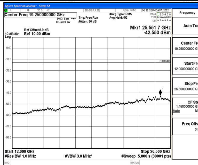
Band2-3MHz-16QAM-19185-1-0-High-12000-26500--42.55-PASS
