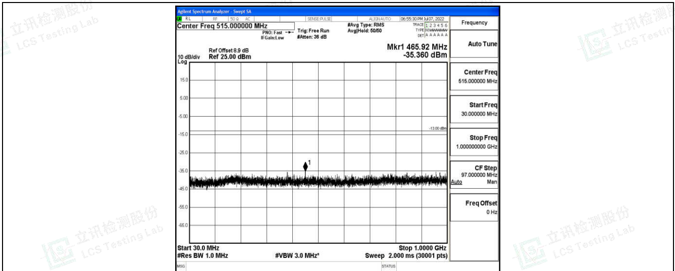
Band2-5MHz-QPSK-19175-1-0-High-30-1000--35.36-PASS
