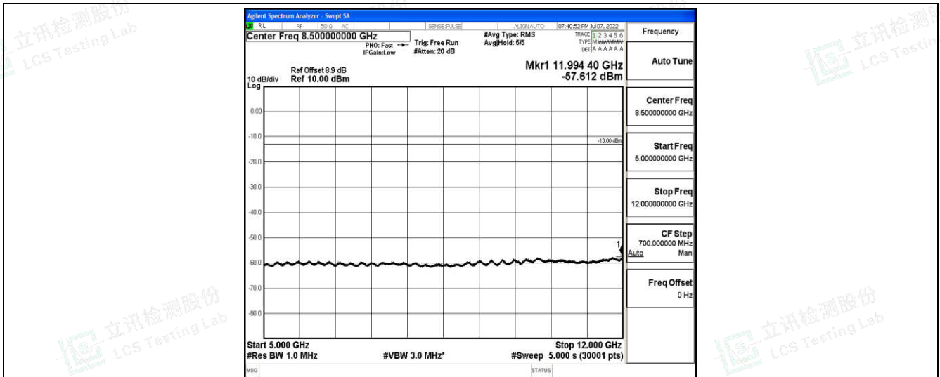
Band2-15MHz-QPSK-18675-1-0-Low-5000-12000--57.61-PASS
