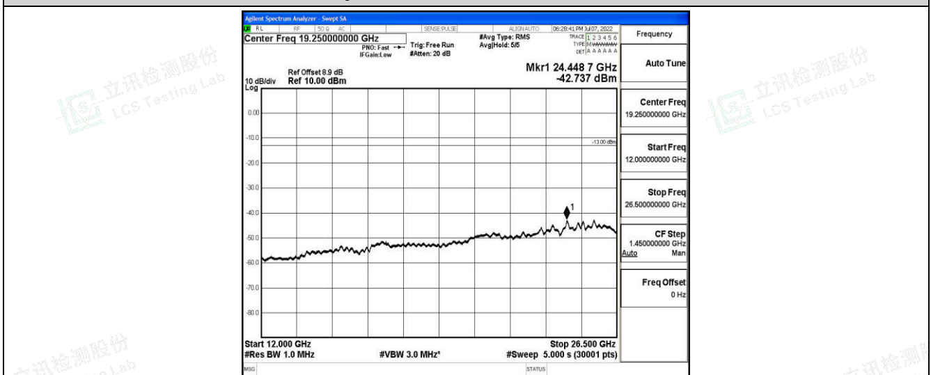
Band2-3MHz-16QAM-18900-1-0-Low-12000-26500--42.74-PASS
