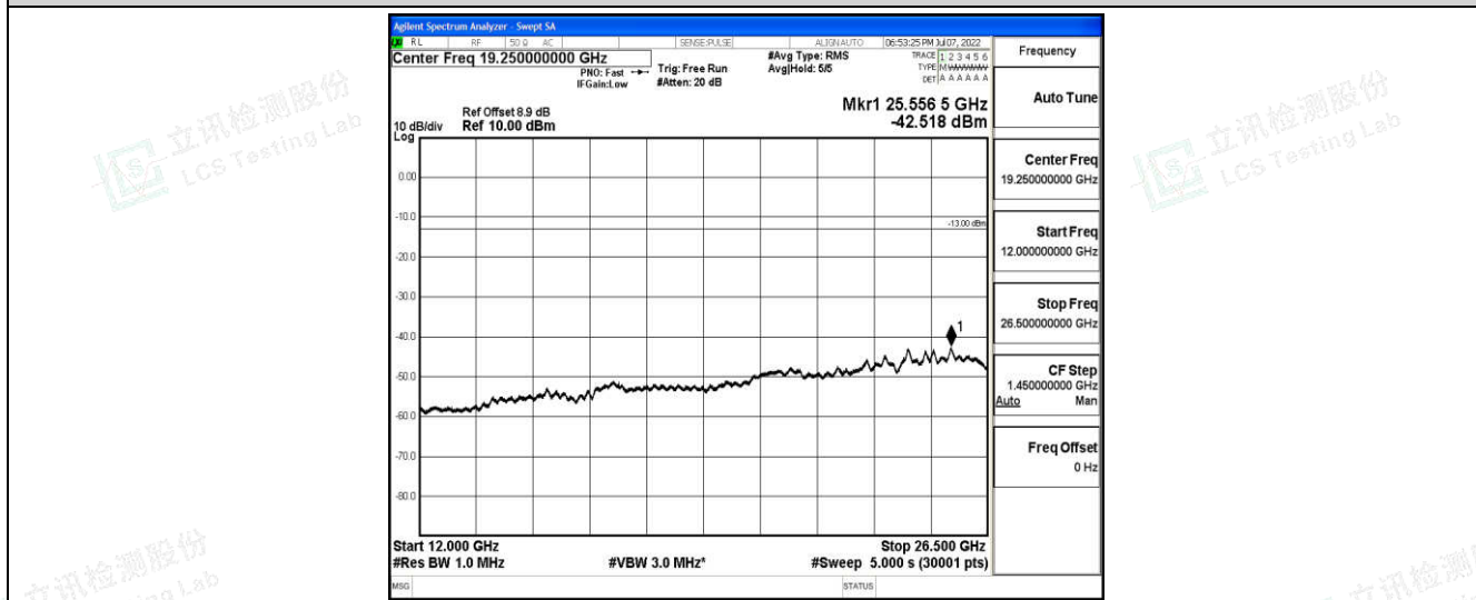
Band2-5MHz-QPSK-18900-1-0-Low-12000-26500--42.52-PASS
