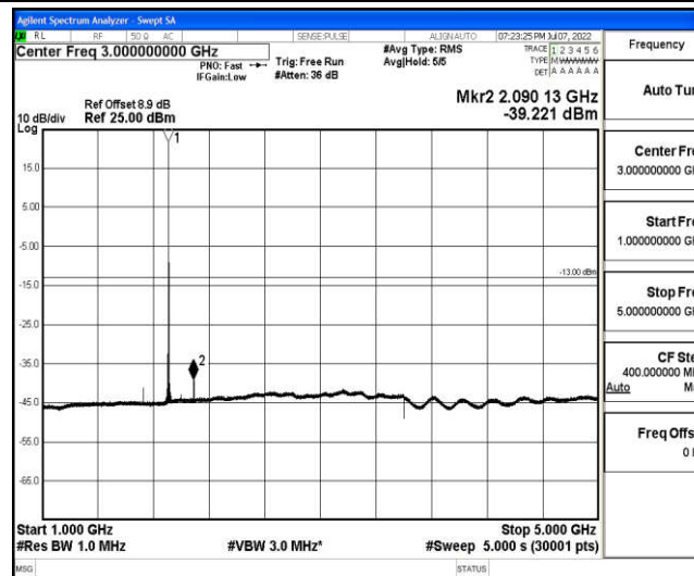
Band2-10MHz-QPSK-19150-1-0-High-1000-5000--39.22-PASS
