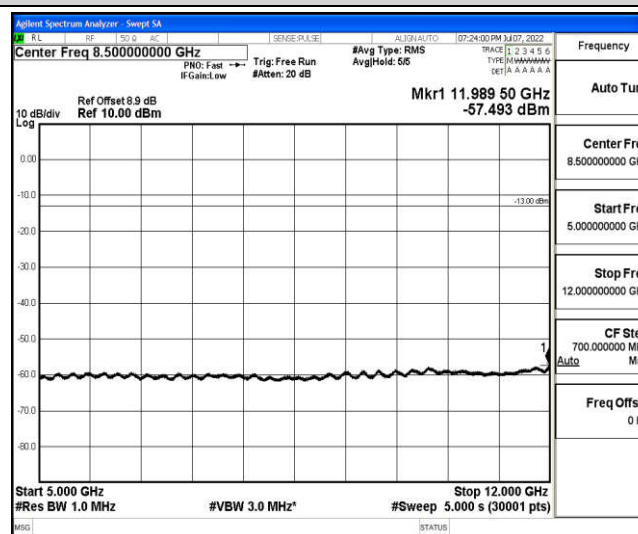
Band2-10MHz-QPSK-19150-1-0-High-5000-12000--57.49-PASS
