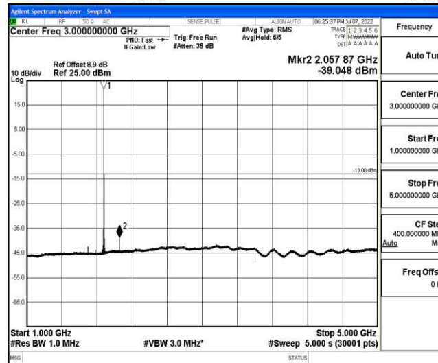
Band2-3MHz-QPSK-18900-1-0-Low-1000-5000--39.05-PASS
