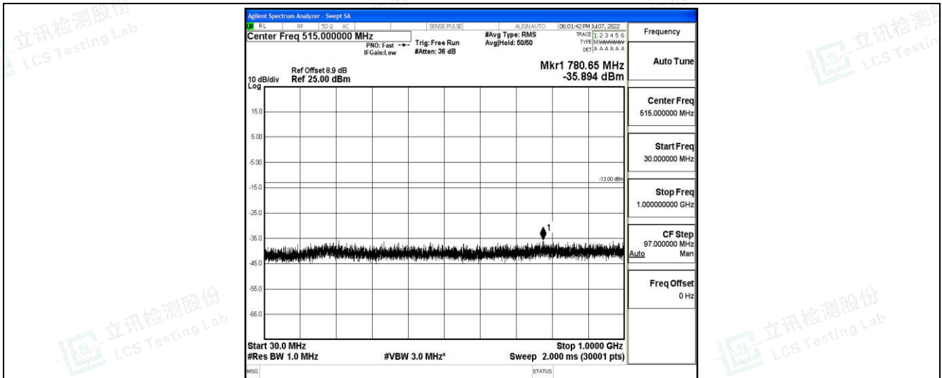
Band2-1.4MHz-QPSK-19193-1-0-High-30-1000--35.89-PASS
