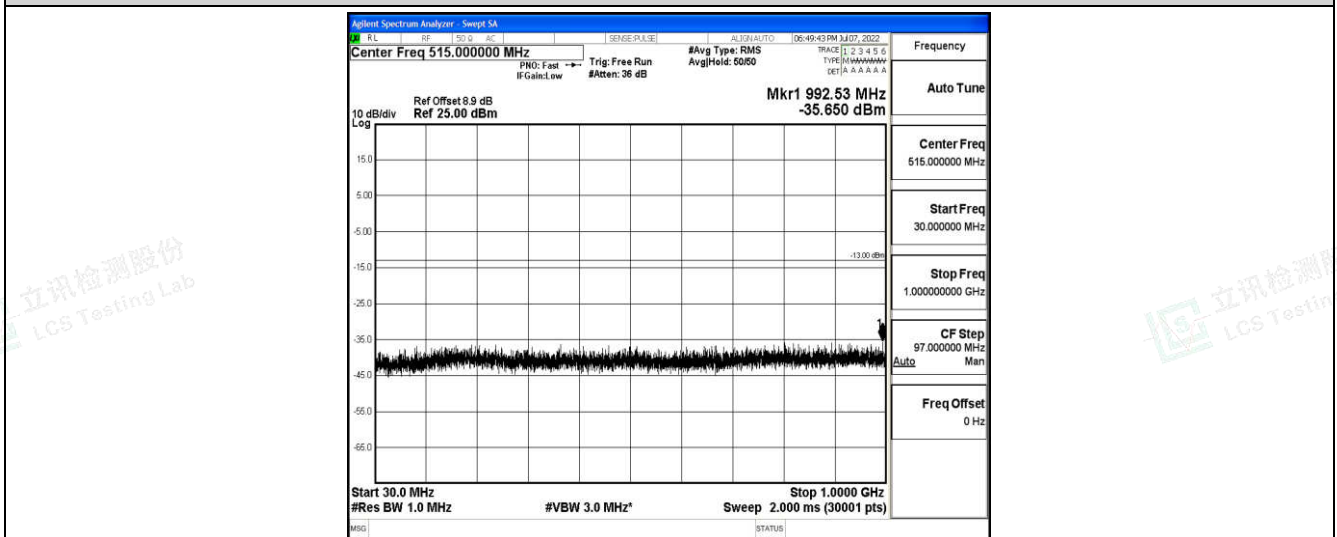
Band2-5MHz-16QAM-18625-1-0-Low-30-1000--35.65-PASS
