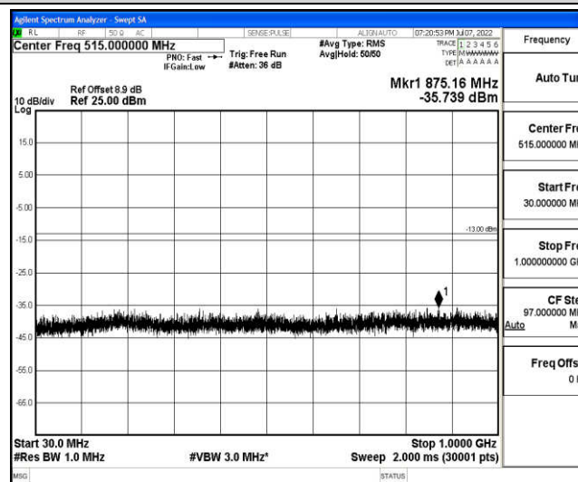
Band2-10MHz-16QAM-18900-1-0-Low-30-1000--35.74-PASS
