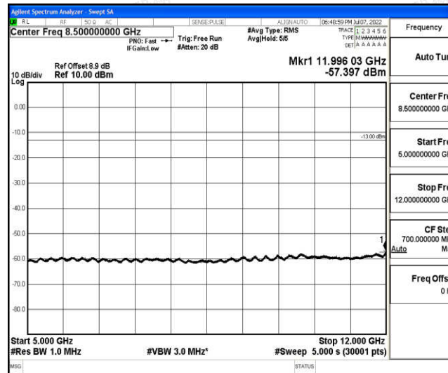
Band2-5MHz-QPSK-18625-1-0-Low-5000-12000--57.4-PASS
