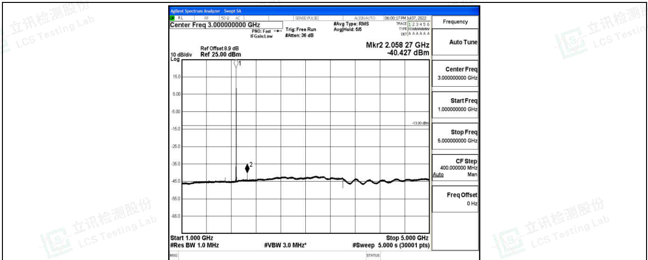
Band2-1.4MHz-16QAM-18900-1-0-Low-1000-5000--40.43-PASS
