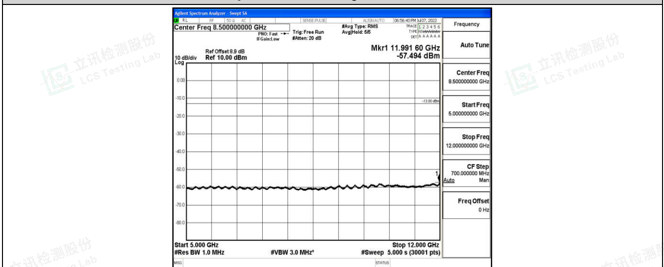
Band2-5MHz-QPSK-19175-1-0-High-5000-12000--57.49-PASS
