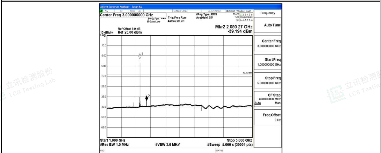
Band2-5MHz-QPSK-19175-1-0-High-1000-5000--39.19-PASS
