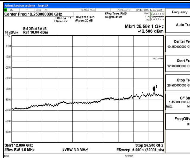
Band2-10MHz-16QAM-18650-1-0-Low-12000-26500--42.59-PASS
