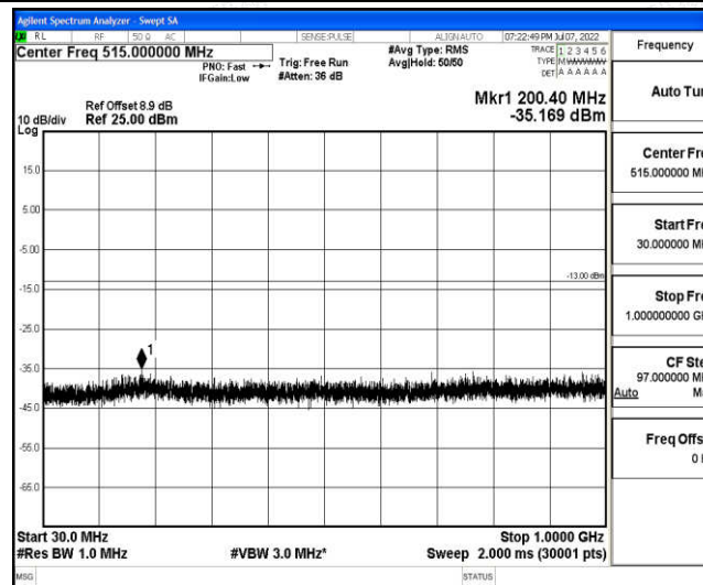
Band2-10MHz-QPSK-19150-1-0-High-30-1000--35.17-PASS
