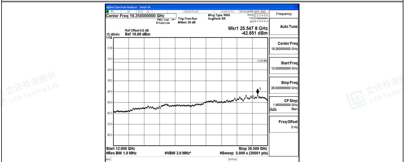
Band2-15MHz-QPSK-18675-1-0-Low-12000-26500--42.65-PASS
