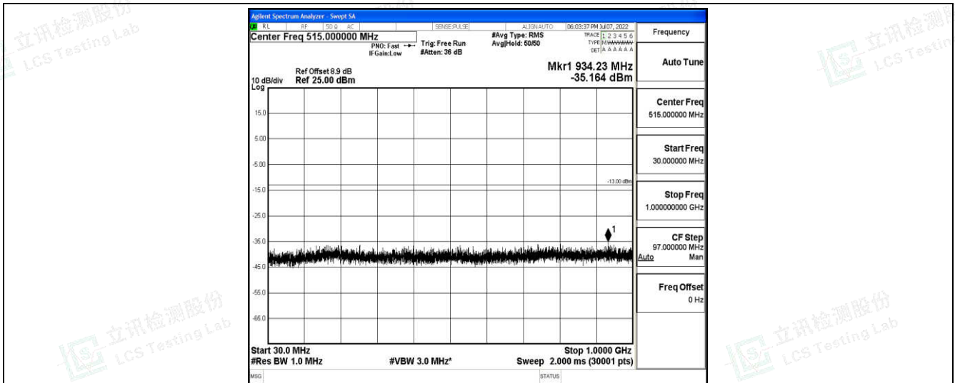
Band2-1.4MHz-16QAM-19193-1-0-High-30-1000--35.16-PASS
