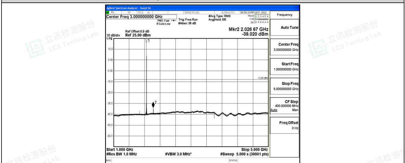
Band2-5MHz-16QAM-18625-1-0-Low-1000-5000--39.02-PASS
