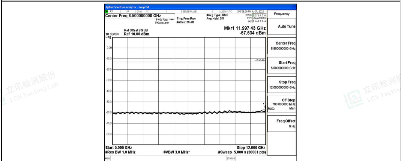
Band2-1.4MHz-QPSK-18900-1-0-Low-5000-12000--57.53-PASS
