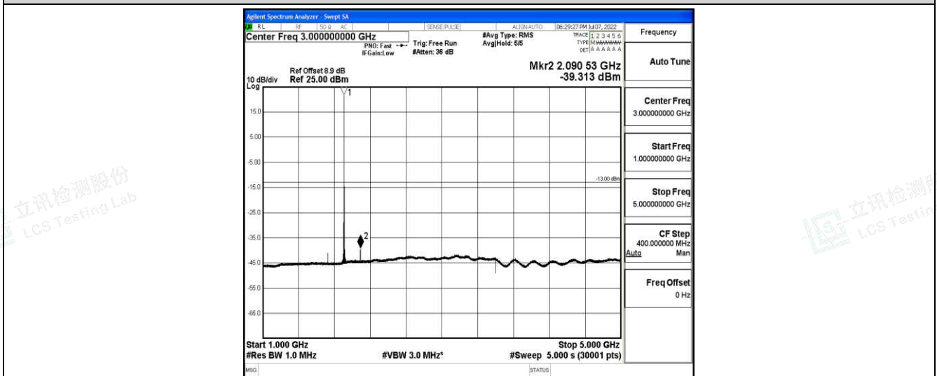
Band2-3MHz-QPSK-19185-1-0-High-1000-5000--39.31-PASS
