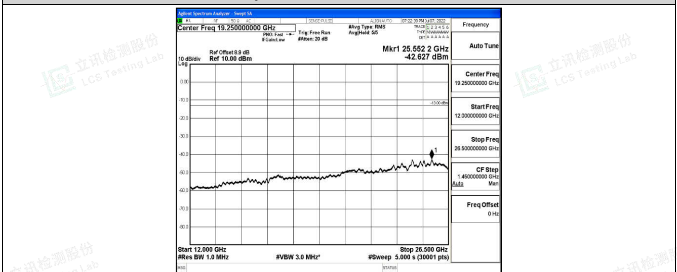
Band2-10MHz-16QAM-18900-1-0-Low-12000-26500--42.63-PASS
