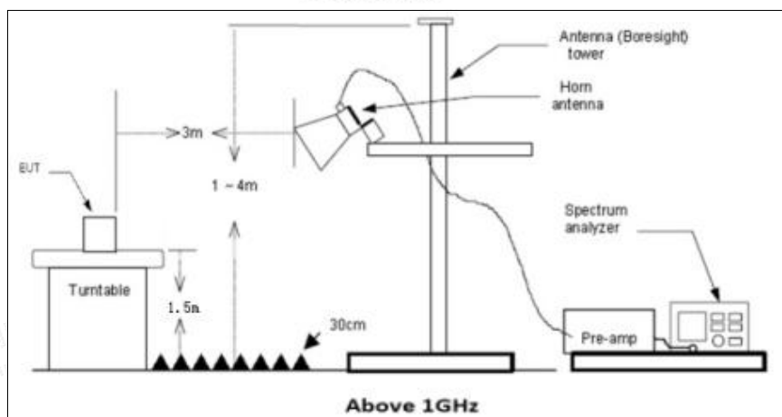
Above 1GHz
