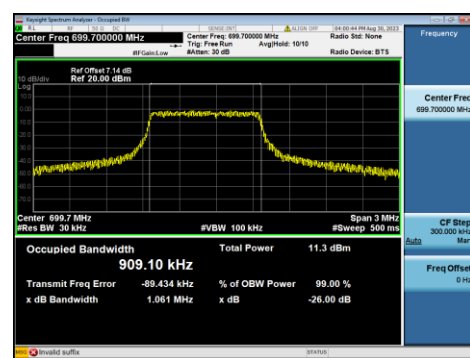
B12-1.4M-Mid CH-OBW-Q16
