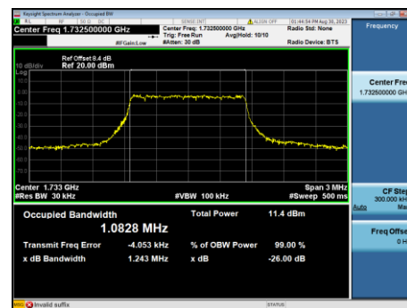
B4-1.4M-Mid CH-OBW-QPSK
