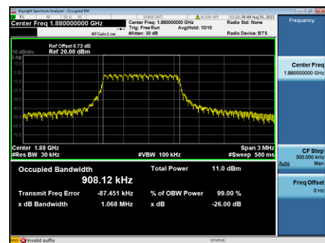
B2-1.4M-Mid CH-OBW-Q16
