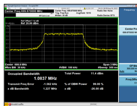
B12-3M-Mid CH-OBW-QPSK
