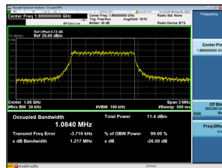
B2-1.4M-Mid CH-OBW-QPSK
