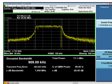
B4-3M-Mid CH-OBW-Q16
