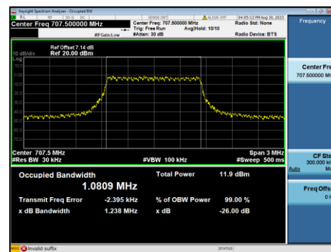
B12-1.4M-Mid CH-OBW-QPSK
