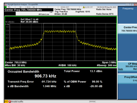
B12-5M-Mid CH-OBW-Q16
