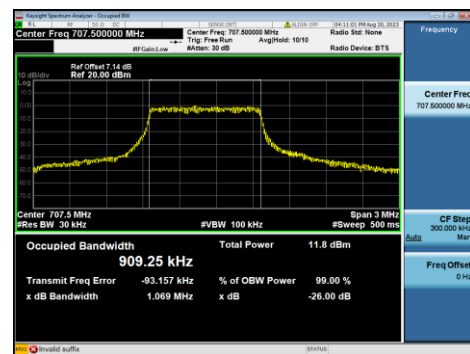
B12-1.4M-Mid CH-OBW-Q16
