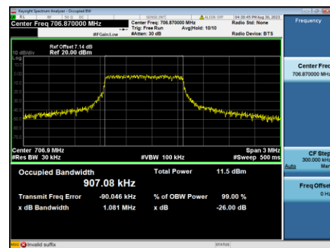
B12-3M-Mid CH-OBW-Q16
