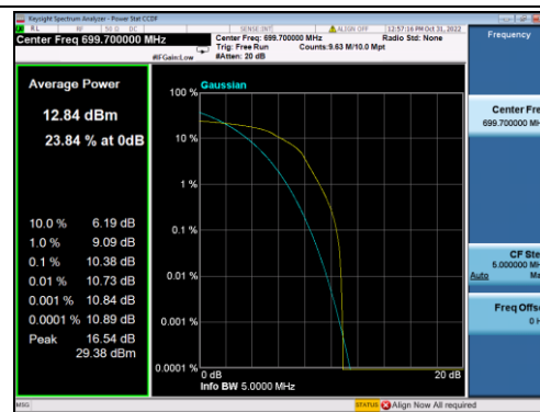
B12-1.4M-Low CH-PAPR-QPSK
