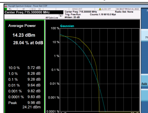
B12-1.4M-Mid CH-PAPR-QPSK
