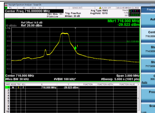
B12-1.4M-High CH-BE-QPSK-1 RB MAX
