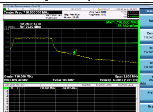
B12-3M-High CH-BE-QPSK-Full RB 0
