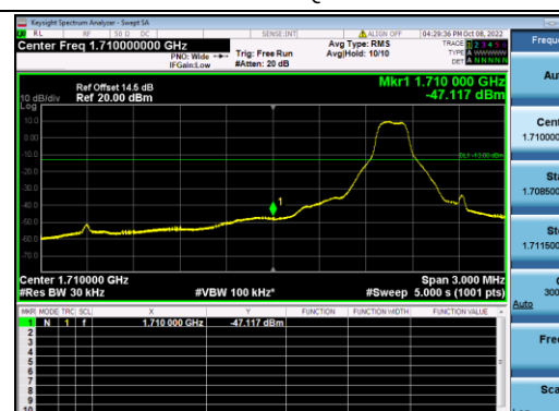
B4-10M-Low CH-BE-QPSK-1 RB 0
