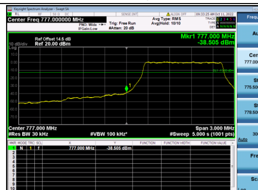
B13-5M-Low CH-BE-QPSK-Full RB 0
