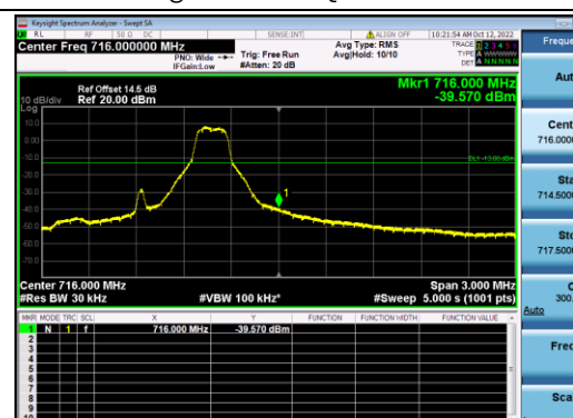
B12-3M-High CH-BE-QPSK-1 RB MAX
