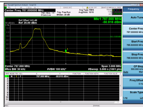
B13-10M-Low CH-BE-Q16-1 RB 0
