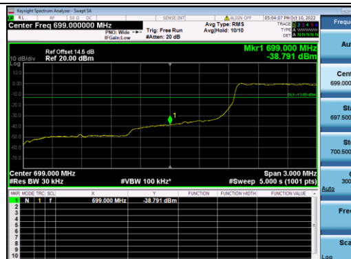
B12-5M-Low CH-BE-QPSK-Full RB 0
