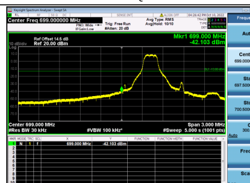
B12-3M-Low CH-BE-QPSK-1 RB 0
