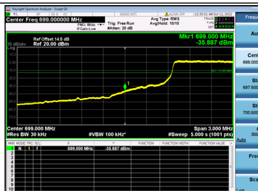
B12-5M-Low CH-BE-QPSK-1 RB 0
