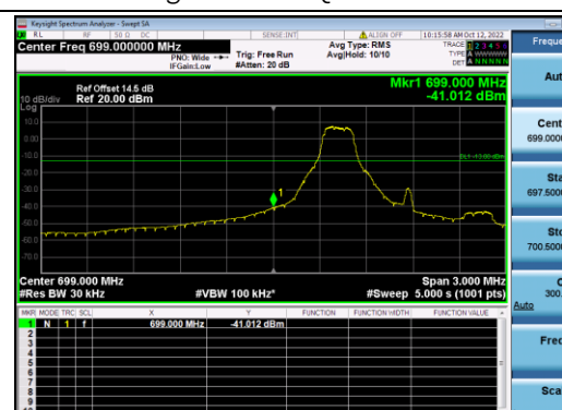
B12-3M-Low CH-BE-Q16-1 RB 0
