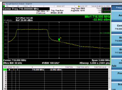
B12-1.4M-High CH-BE-QPSK-Full RB 0
