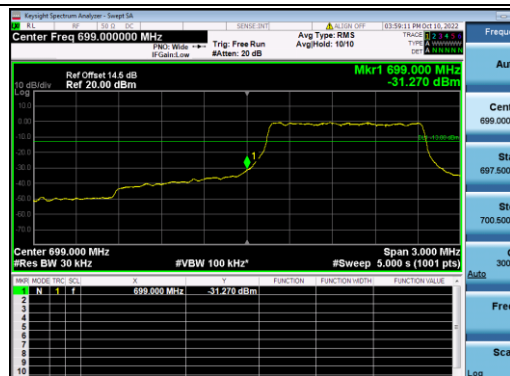
B12-1.4M-Low CH-BE-QPSK-Full RB 0
