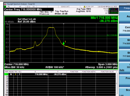
B12-10M-High CH-BE-Q16-Full RB 0
