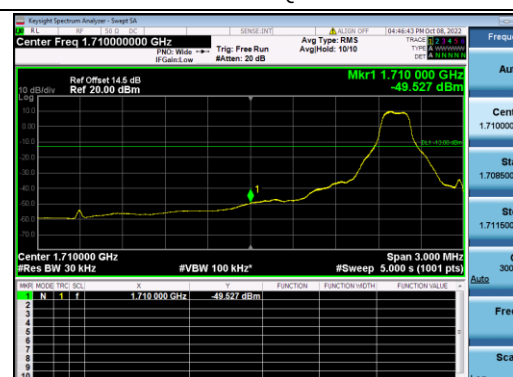
B4-15M-Low CH-BE-QPSK-1 RB 0
