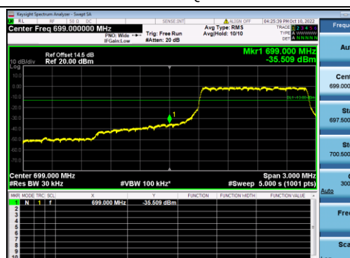
B12-3M-Low CH-BE-QPSK-Full RB 0
