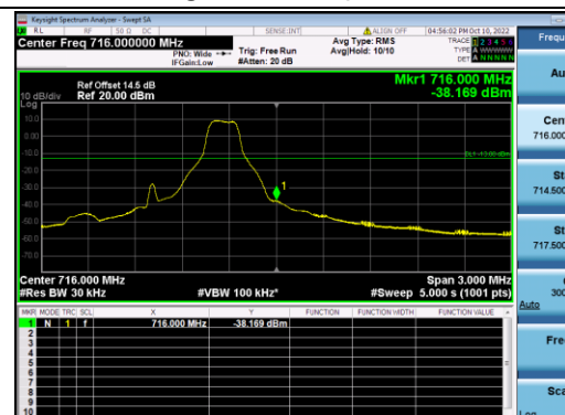
B12-10M-High CH-BE-QPSK-Full RB 0
