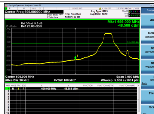
B12-10M-Low CH-BE-QPSK-1 RB 0
