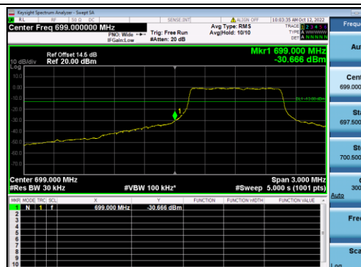
B12-1.4M-Low CH-BE-Q16-Full RB 0
