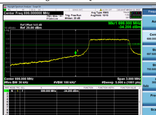
B12-3M-Low CH-BE-Q16-Full RB 0
