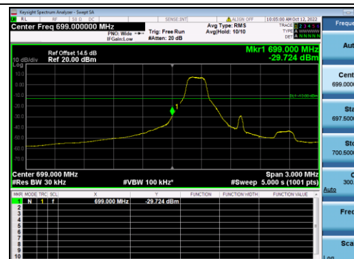
B12-1.4M-Low CH-BE-Q16-1 RB 0
