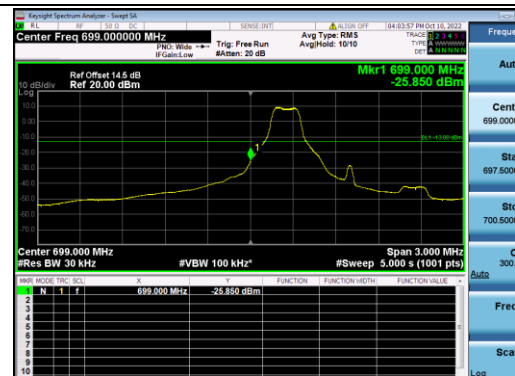
B12-1.4M-Low CH-BE-QPSK-1 RB 0
