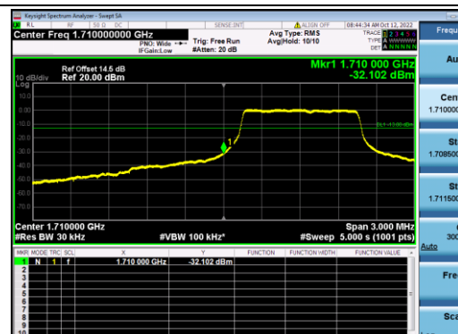
B4-1.4M-Low CH-BE-Q16-Full RB 0
