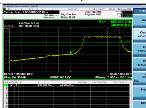
B2-15M-Low CH-BE-QPSK-Full RB 0
