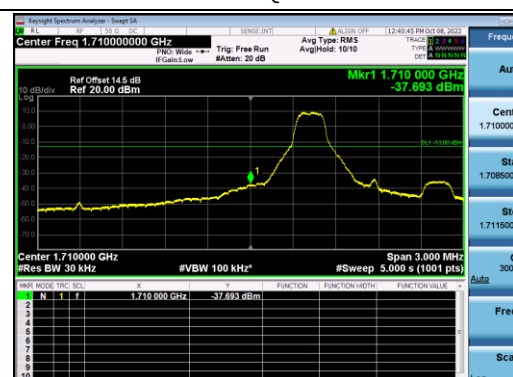
B4-3M-Low CH-BE-QPSK-1 RB 0
