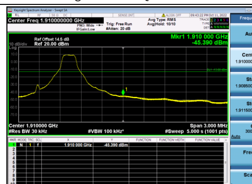
B2-10M-High CH-BE-QPSK-1 RB MAX
