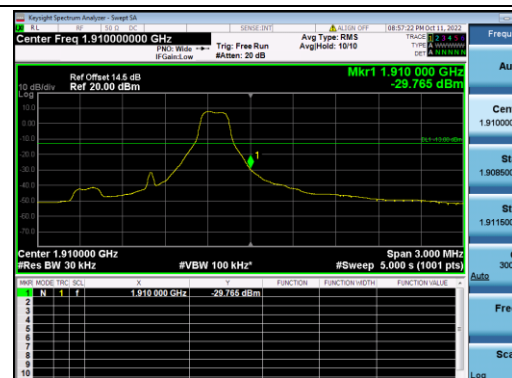
B2-1.4M-High CH-BE-QPSK-1 RB MAX
