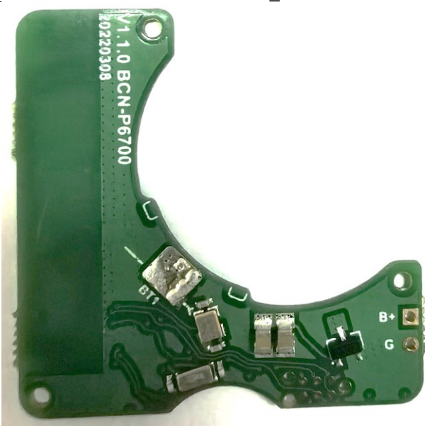
EUT bottom side view_smB1-111
