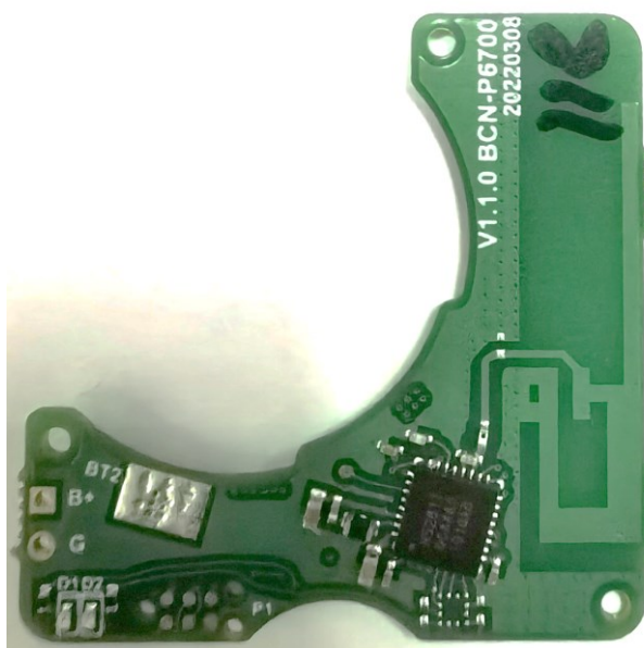
EUT top side view_smb1-111
