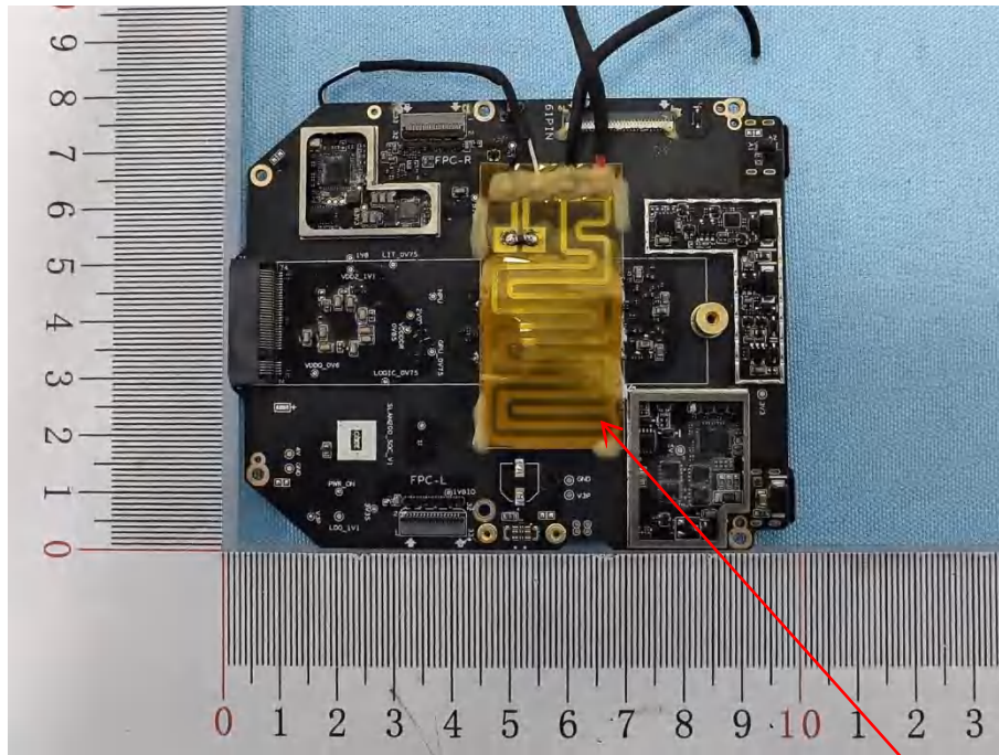
Heating film
