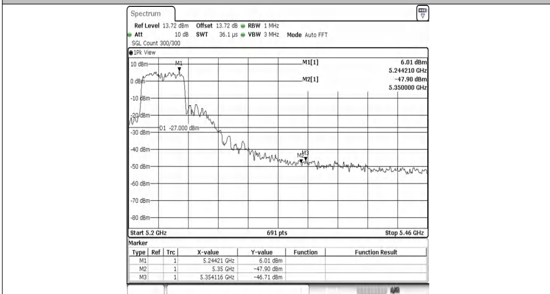
11N40MIMO-Ant2-5230-PASS
