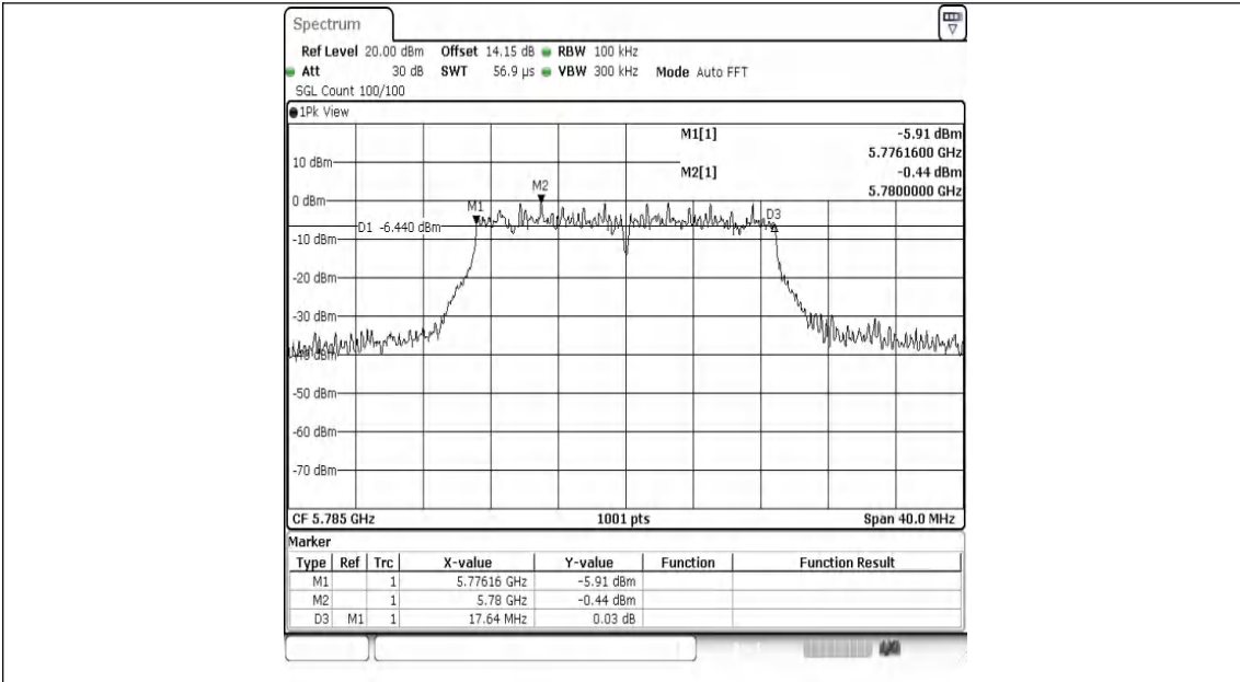
11AC20MIMO-Ant1-5785-PASS
