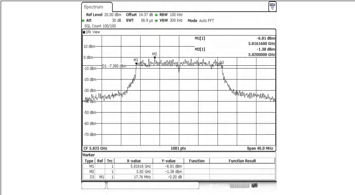
11N20MIMO-Ant1-5825-PASS
