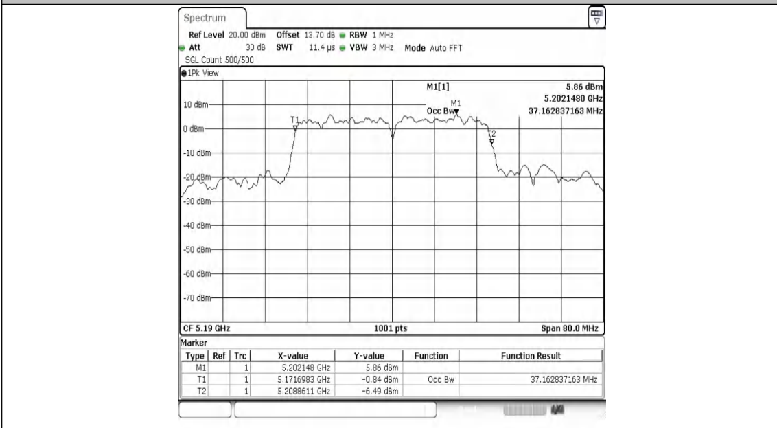
11N40MIMO-Ant2-5190
