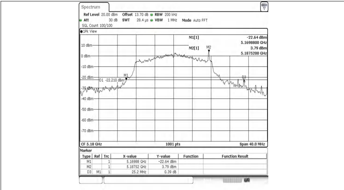
11A-Ant1-5180
