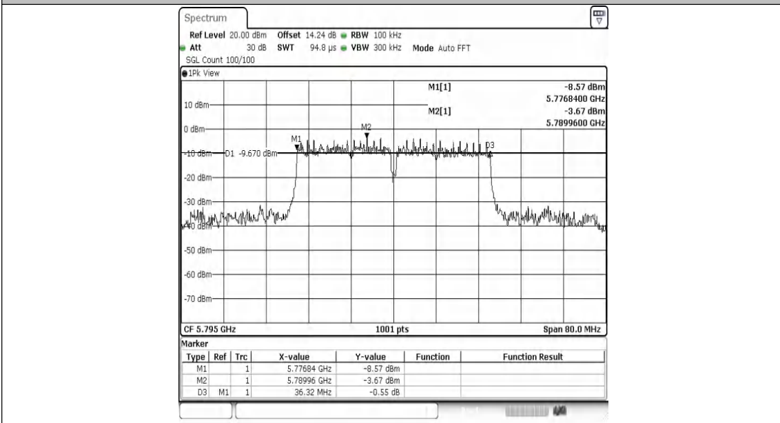
11N40MIMO-Ant2-5795-PASS
