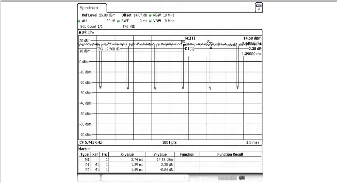
NTNV-11A-Ant2-5745
