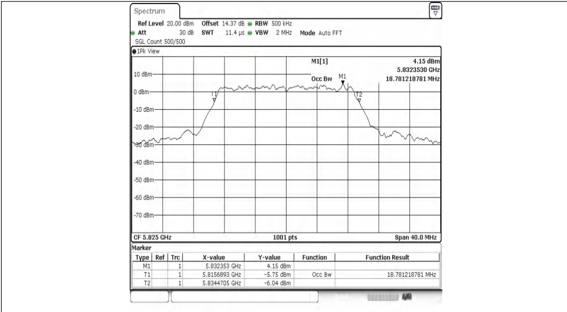
11AC20MIMO-Ant1-5825
