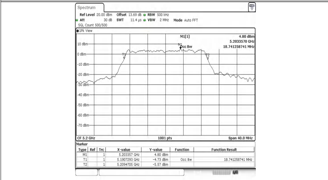
11AC20MIMO-Ant2-5200
