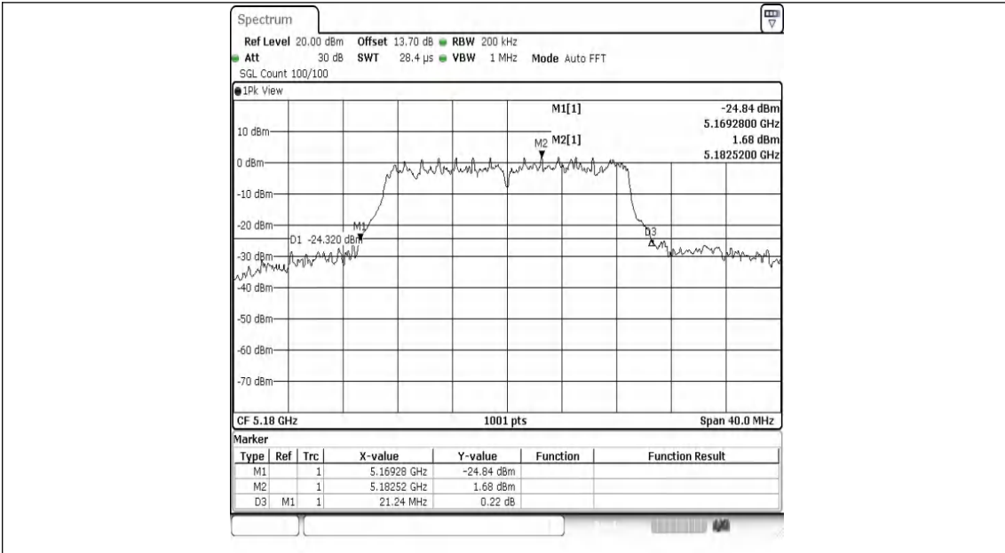
11AC20MIMO-Ant1-5180
