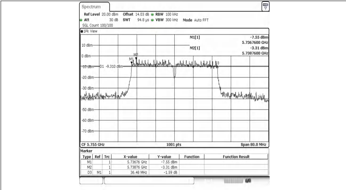
11AC40MIMO-Ant1-5755-PASS
