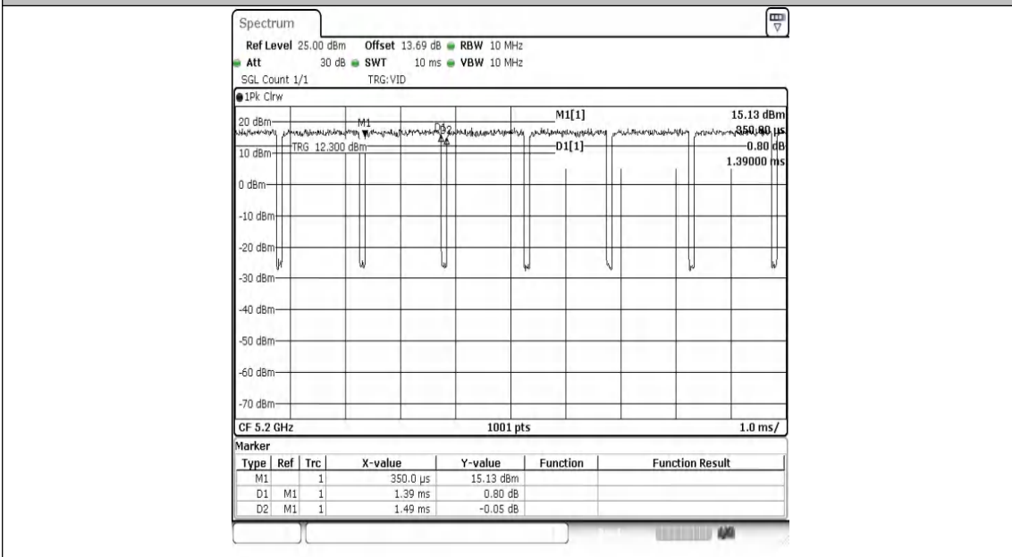
NTNV-11A-Ant2-5200
