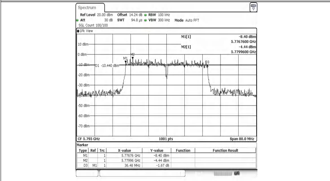
11AC40MIMO-Ant2-5795-PASS
