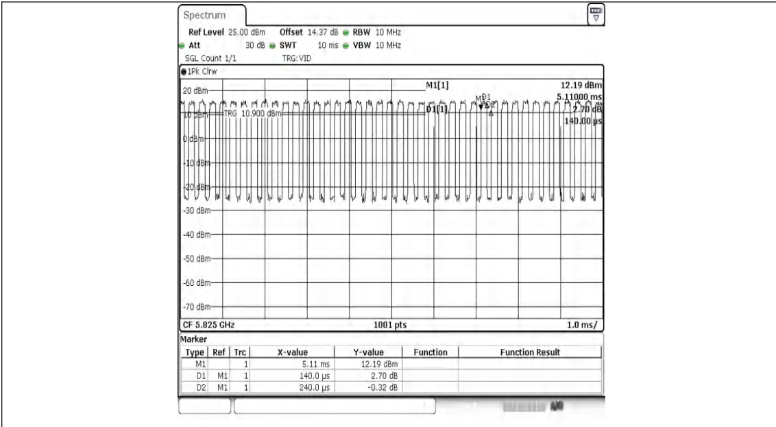
NTNV-11AC20MIMO-Ant1-5825
