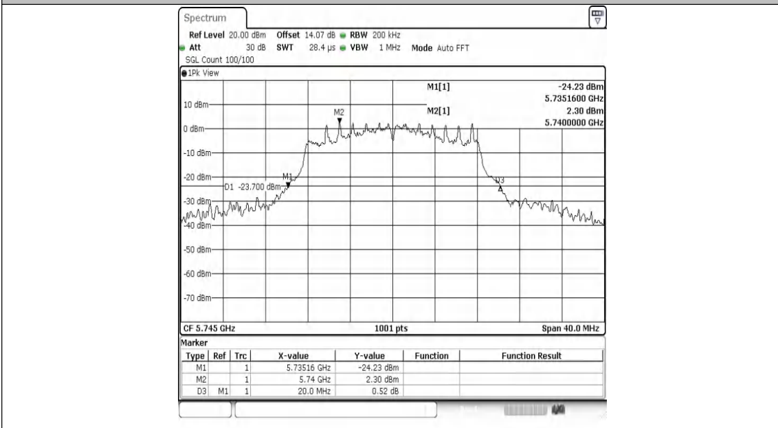
11A-Ant2-5745
