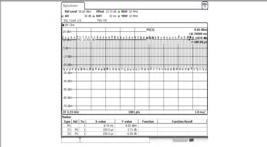
NTVN-11N40MIMO-Ant2-5230
