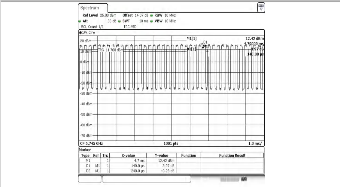
NTNV-11AC20MIMO-Ant2-5745
