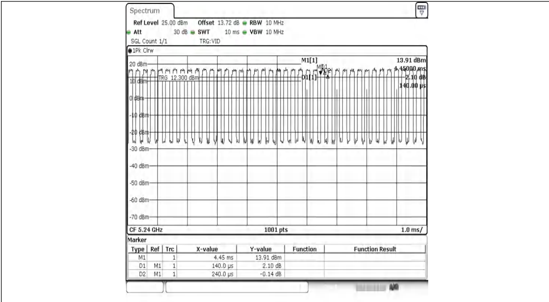
NTNV-11AC20MIMO-Ant1-5240
