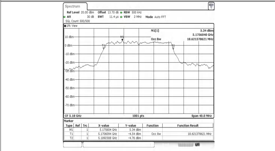
11AC20MIMO-Ant2-5180
