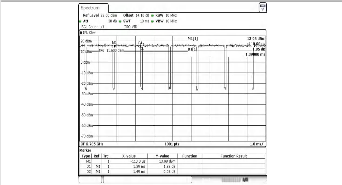
NTNV-11A-Ant2-5785
