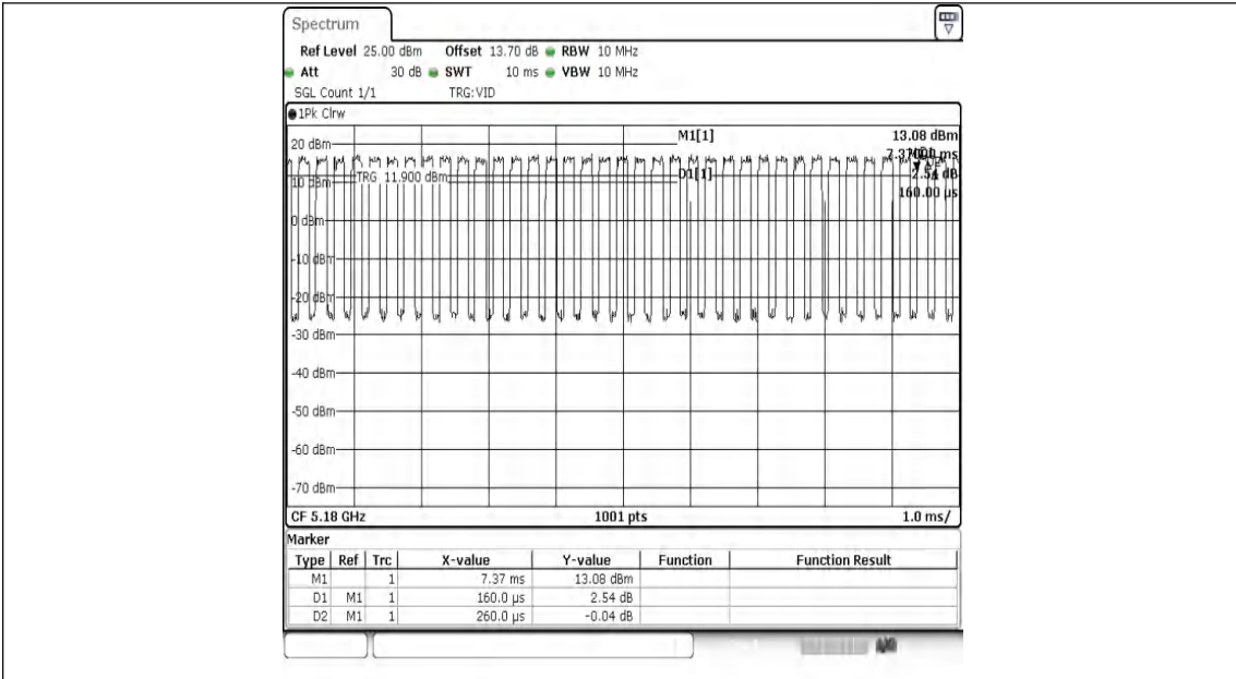
NTVN-11N20MIMO-Ant1-5180
