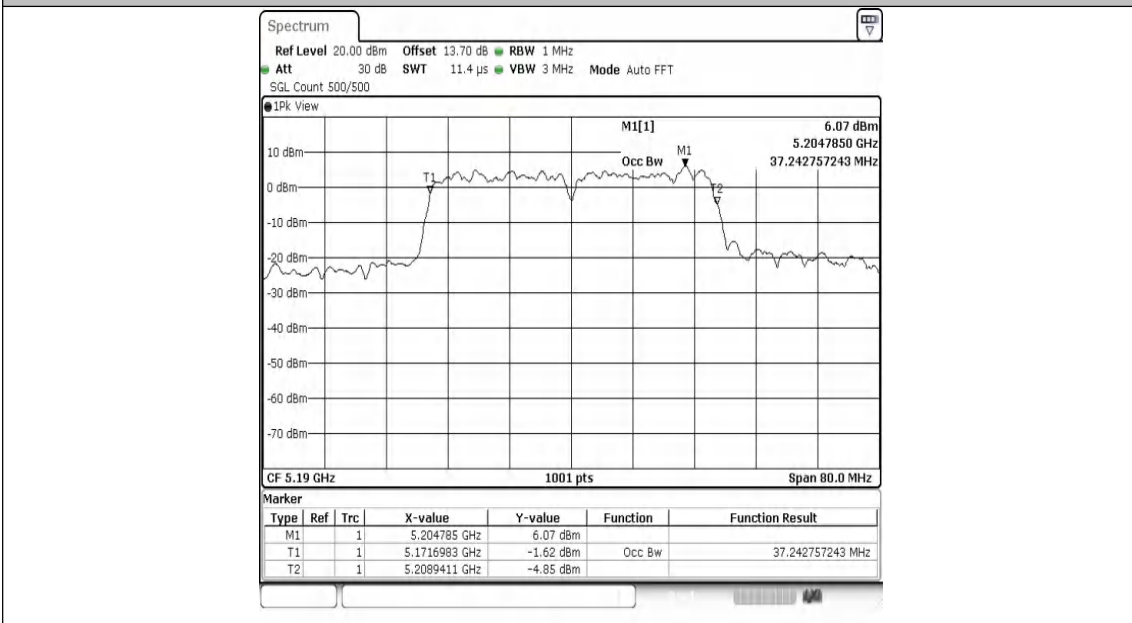
11AC40MIMO-Ant2-5190
