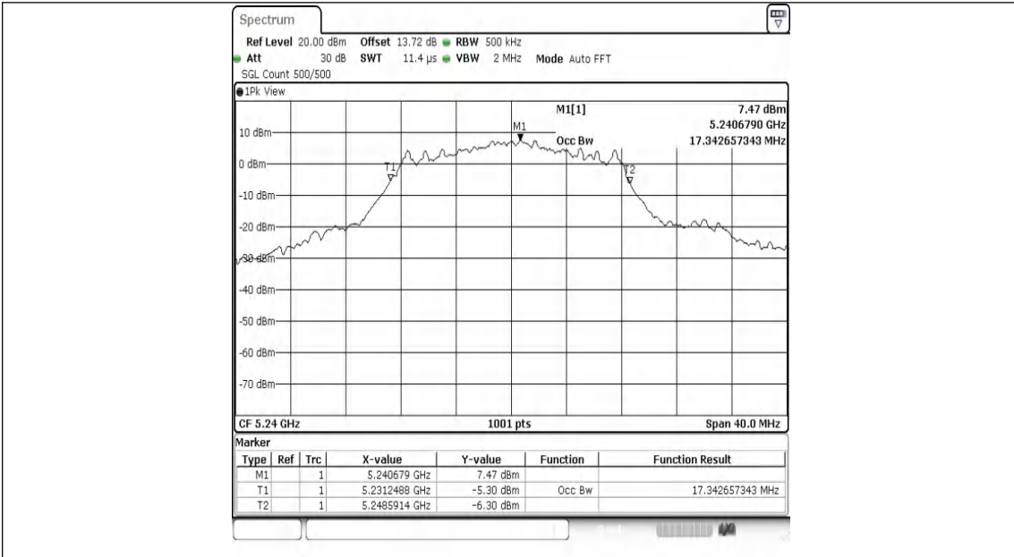
11A-Ant1-5240
