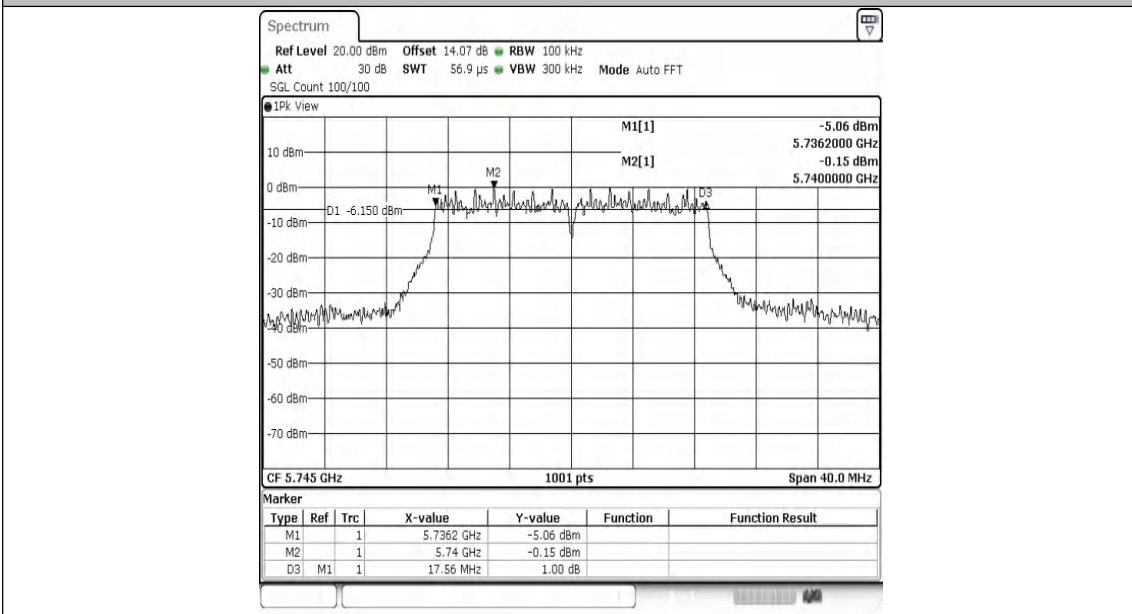
11AC20MIMO-Ant2-5745-PASS
