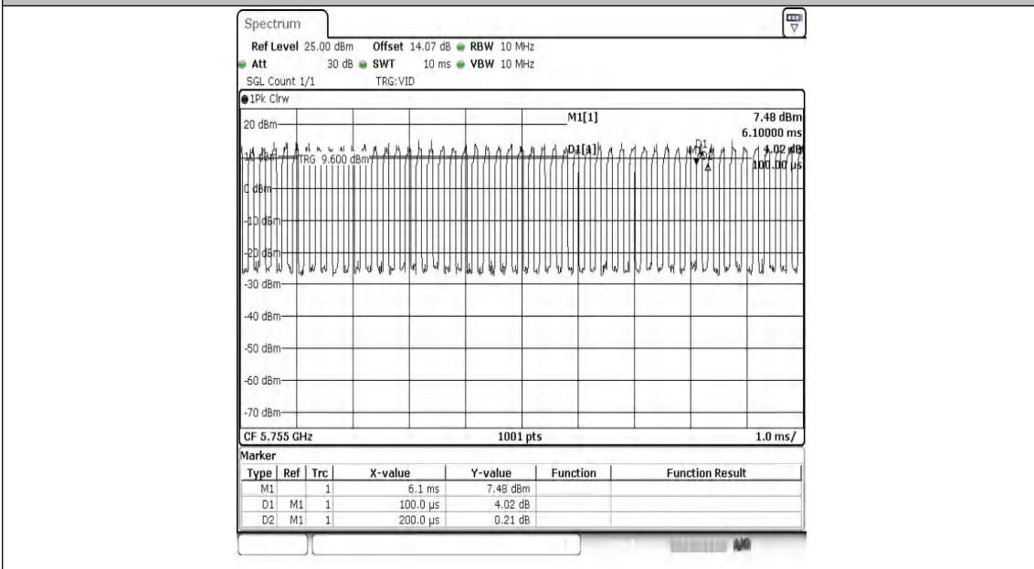
NTVN-11N40MIMO-Ant2-5755
