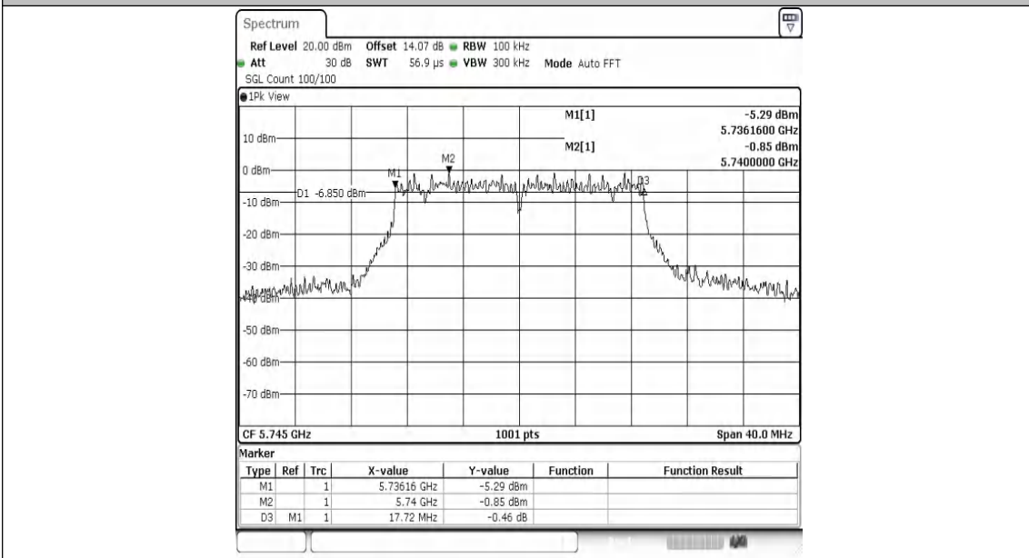
11N20MIMO-Ant2-5745-PASS
