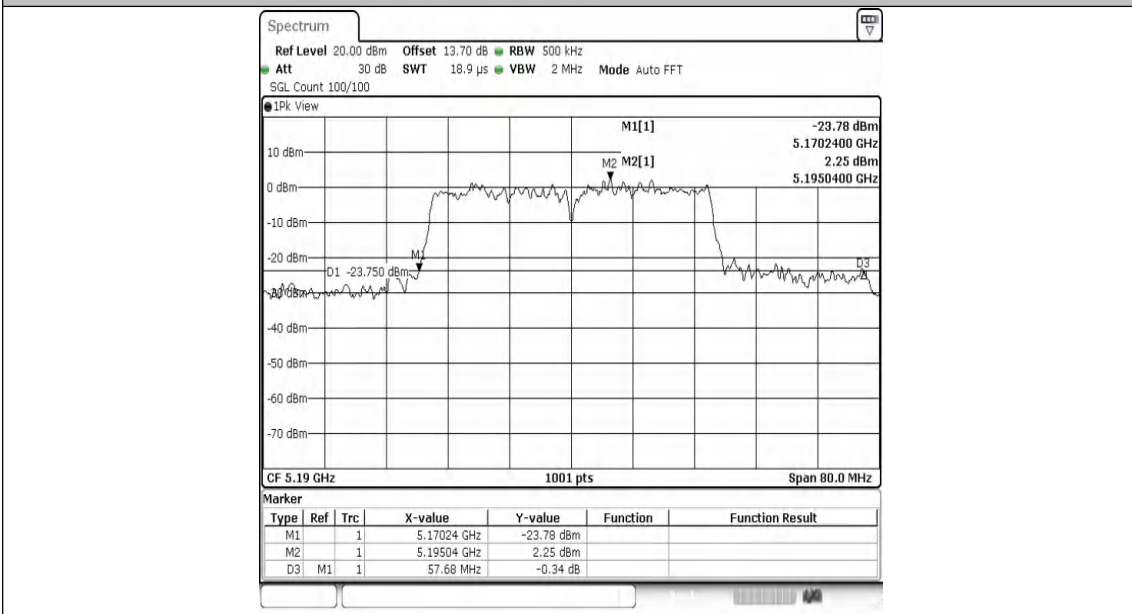
11AC40MIMO-Ant2-5190
