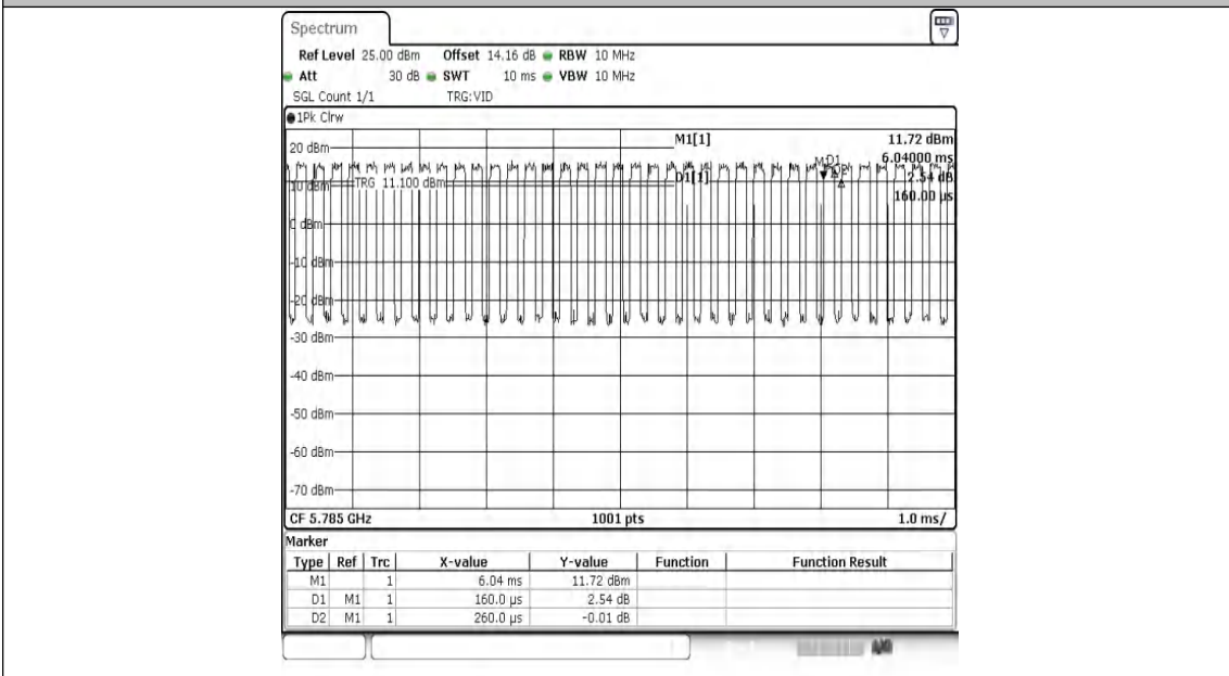
NTNV-11N20MIMO-Ant2-5785
