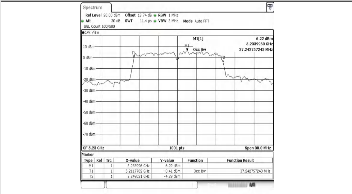
11AC40MIMO-Ant2-5230
