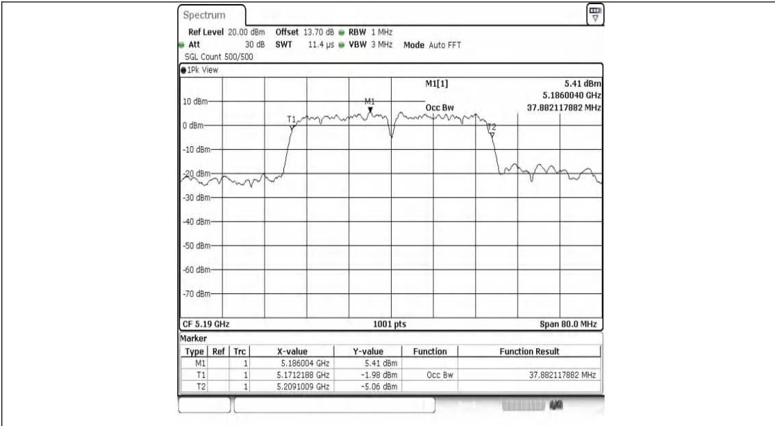
11AC40MIMO-Ant1-5190
