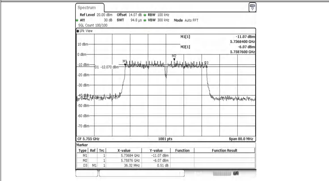
11AC40MIMO-Ant2-5755-PASS
