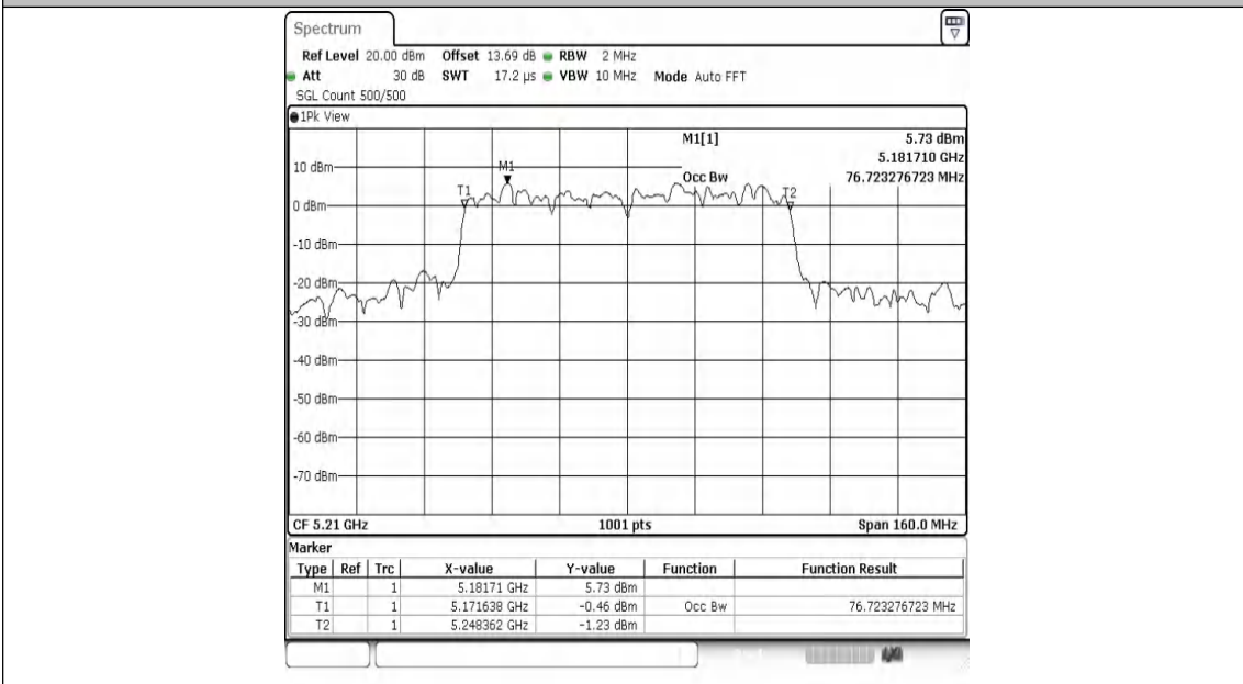
11AC80MIMO-Ant2-5210
