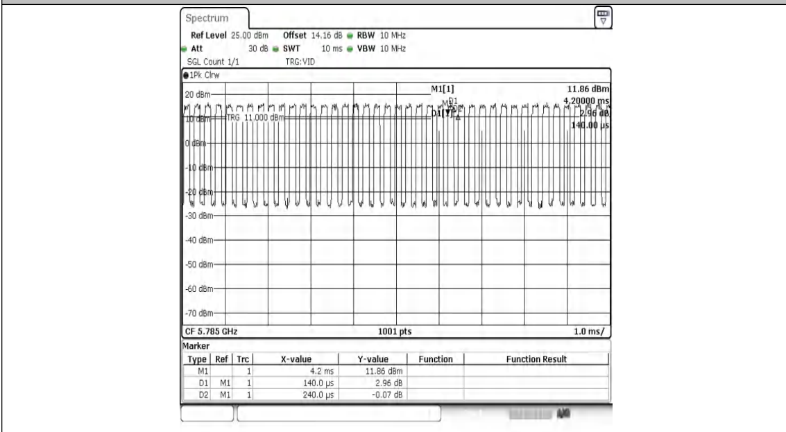
NTNV-11AC20MIMO-Ant2-5785
