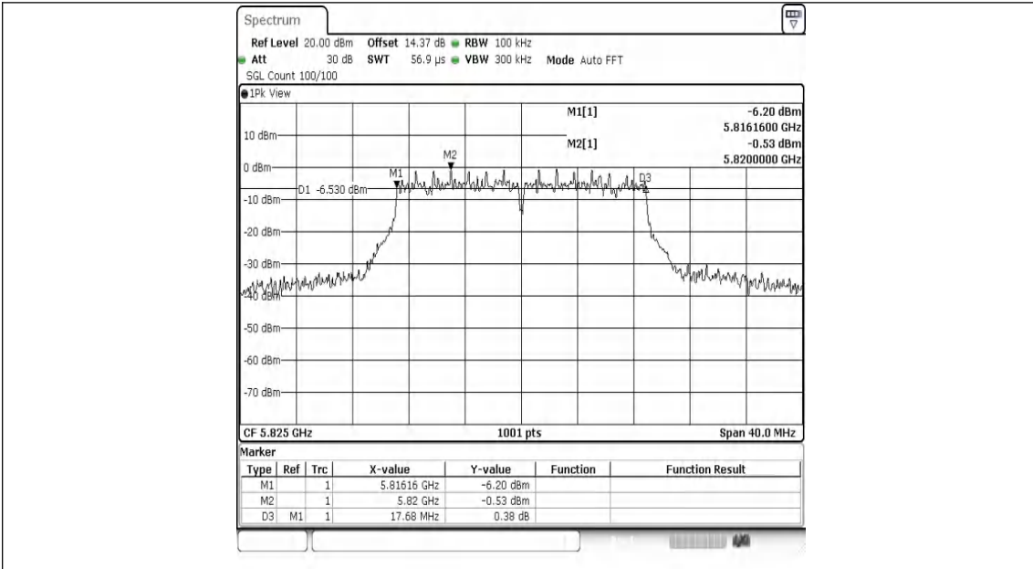
11AC20MIMO-Ant1-5825-PASS
