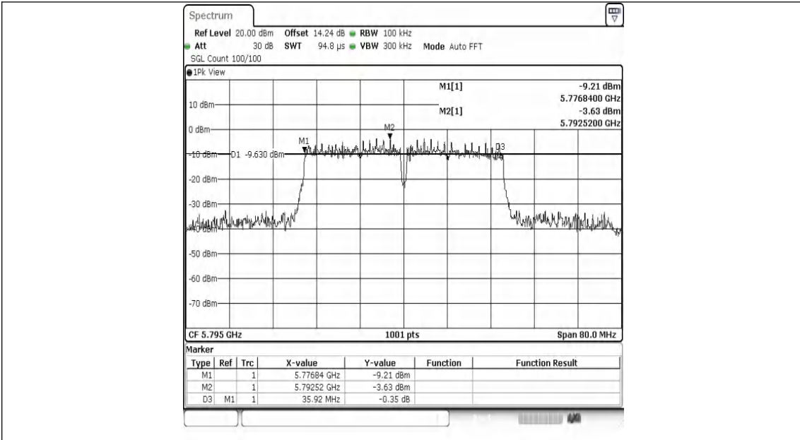
11AC40MIMO-Ant1-5795-PASS
