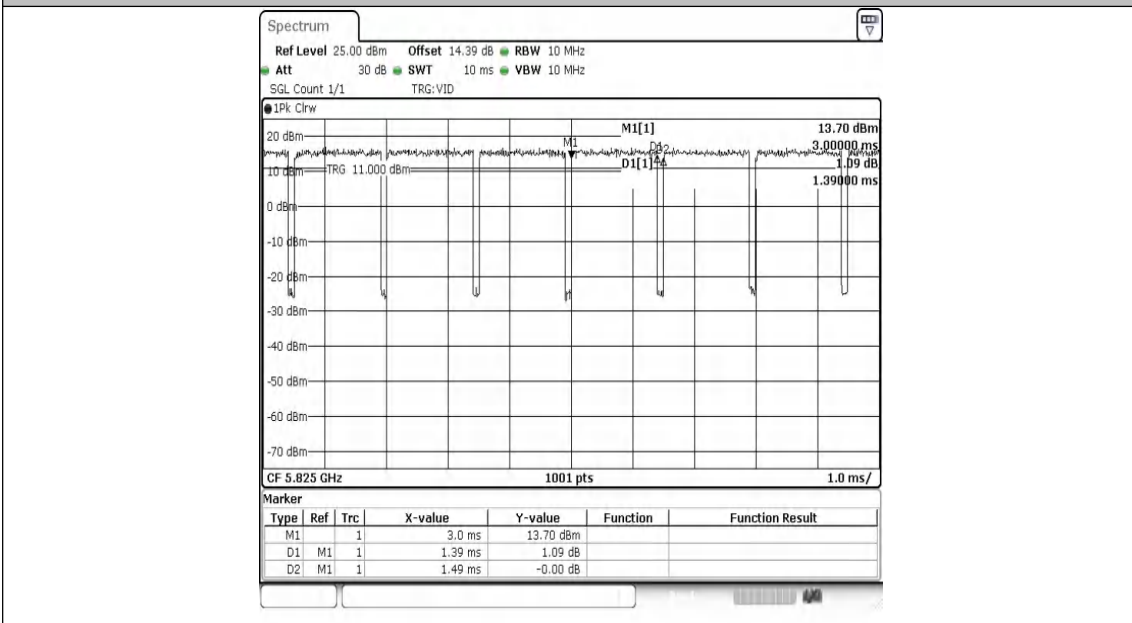
NTNV-11A-Ant2-5825
