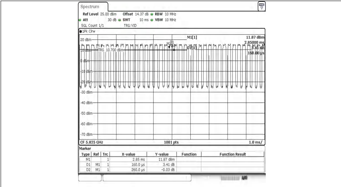
NTVN-11N20MIMO-Ant1-5825
