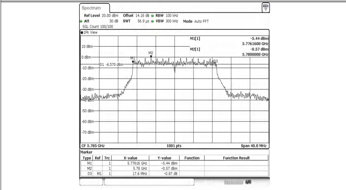
11AC20MIMO-Ant2-5785-PASS
