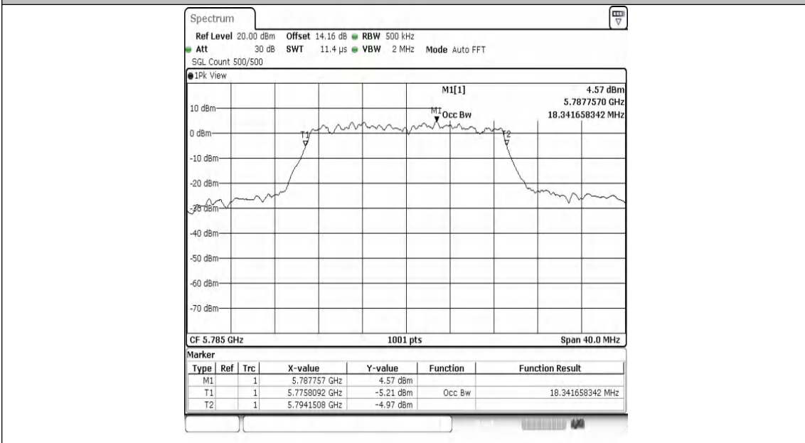
11N20MIMO-Ant2-5785
