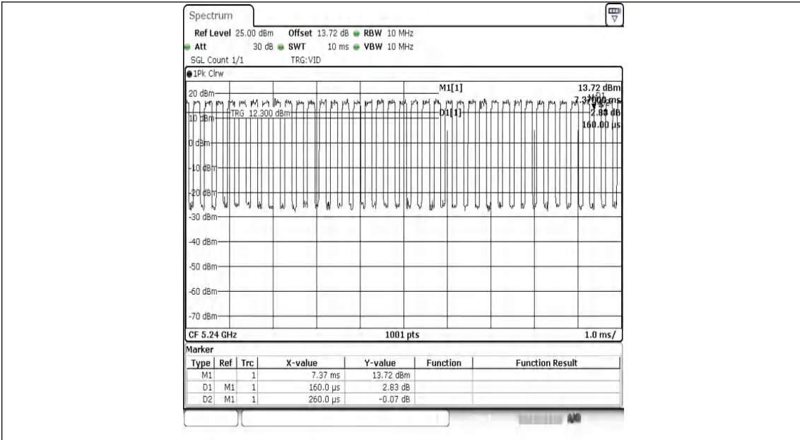
NTVN-11N20MIMO-Ant1-5240
