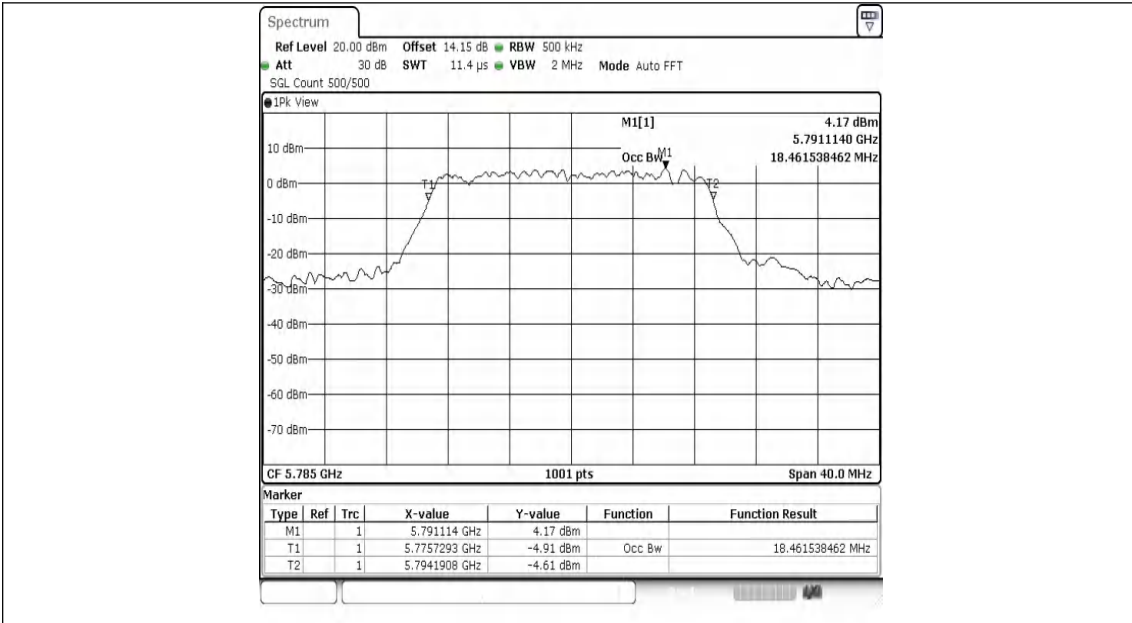
11N20MIMO-Ant1-5785
