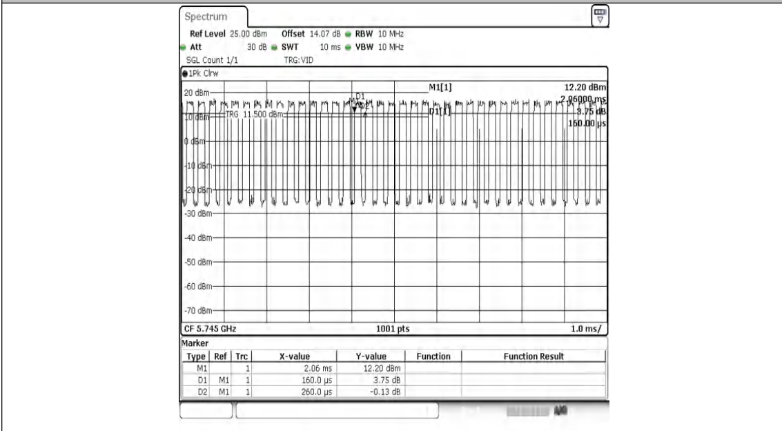
NTNV-11N20MIMO-Ant2-5745
