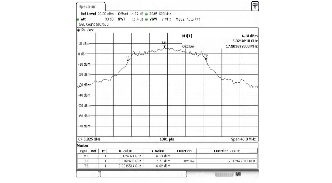
11A-Ant1-5825
