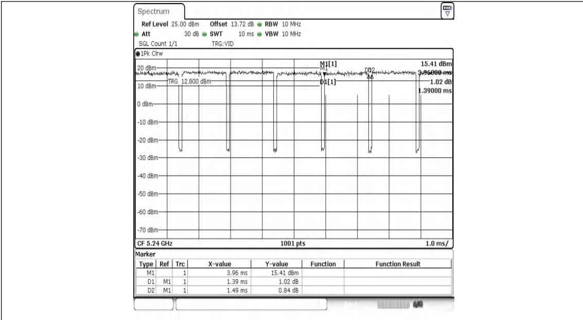
NTNV-11A-Ant1-5240
