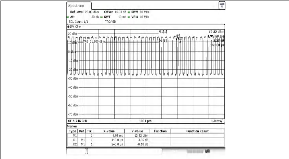
NTNV-11AC20MIMO-Ant1-5745
