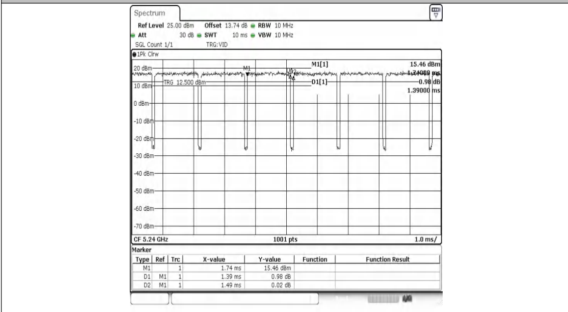
NTNV-11A-Ant2-5240
