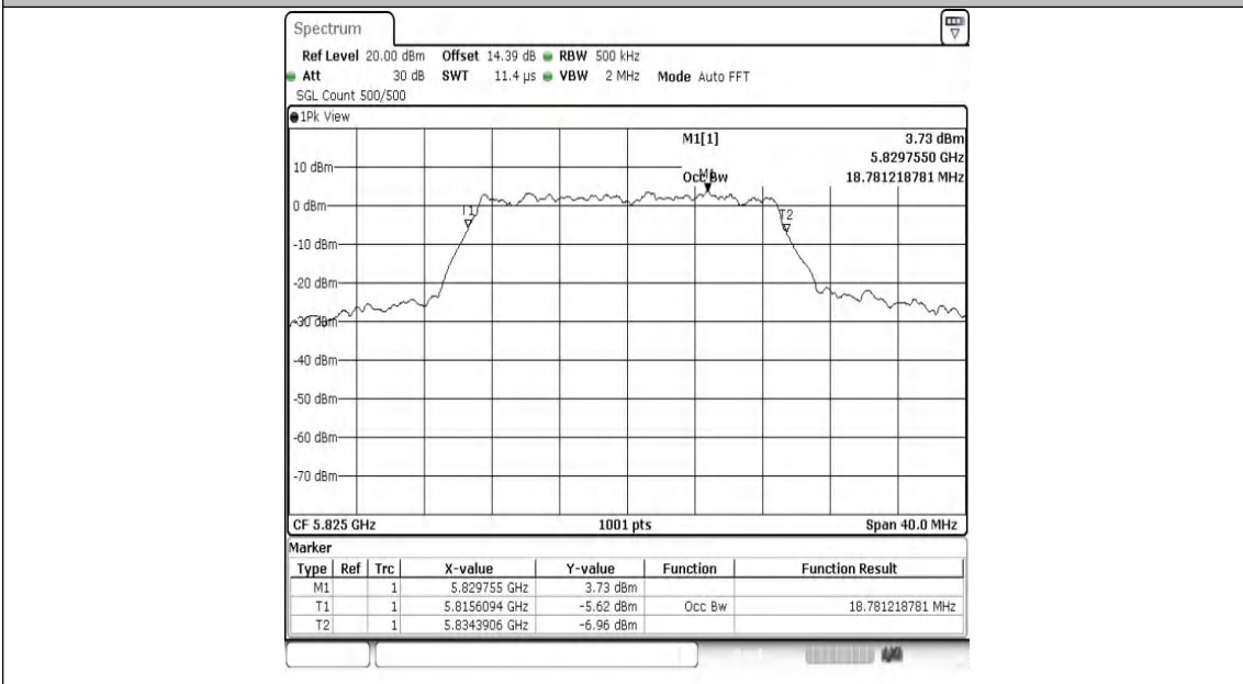
11AC20MIMO-Ant2-5825
