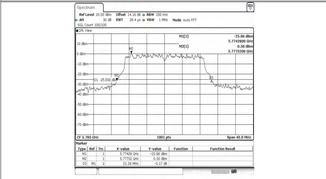
11AC20MIMO-Ant2-5785
