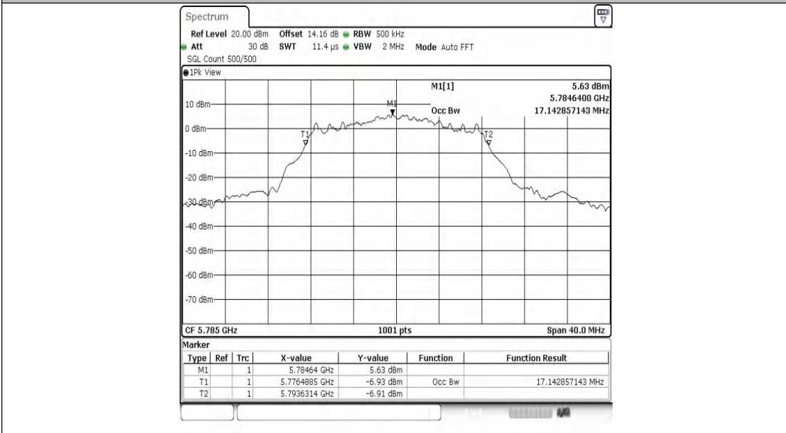
11A-Ant2-5785
