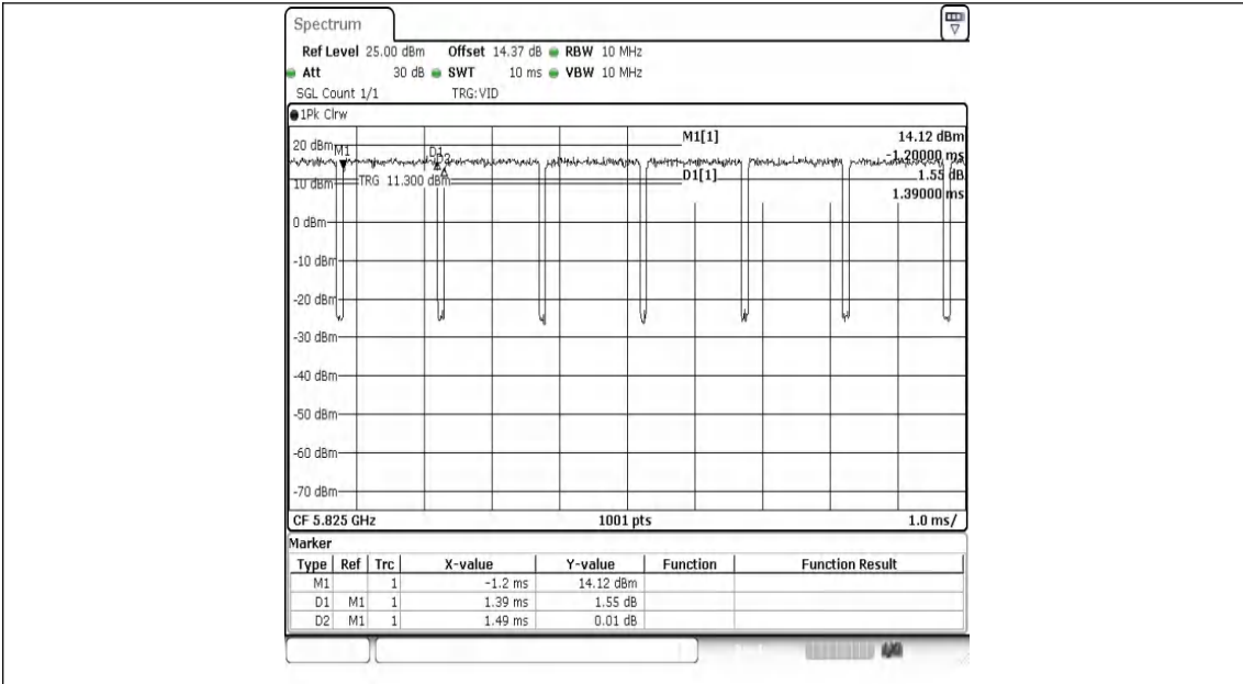
NTNV-11A-Ant1-5825
