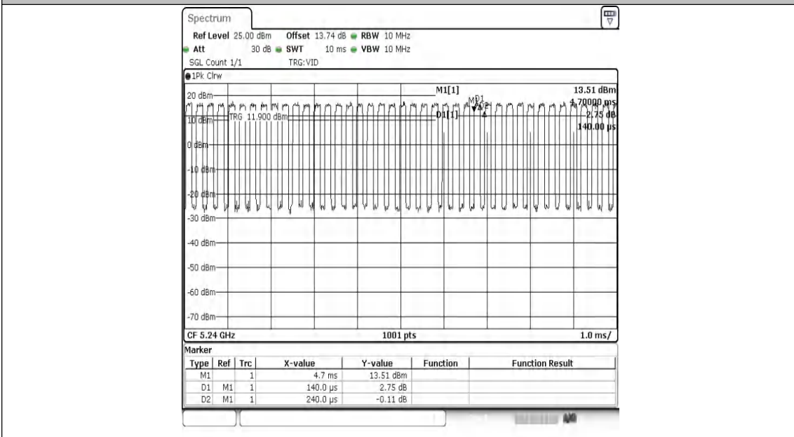
NTNV-11AC20MIMO-Ant2-5240
