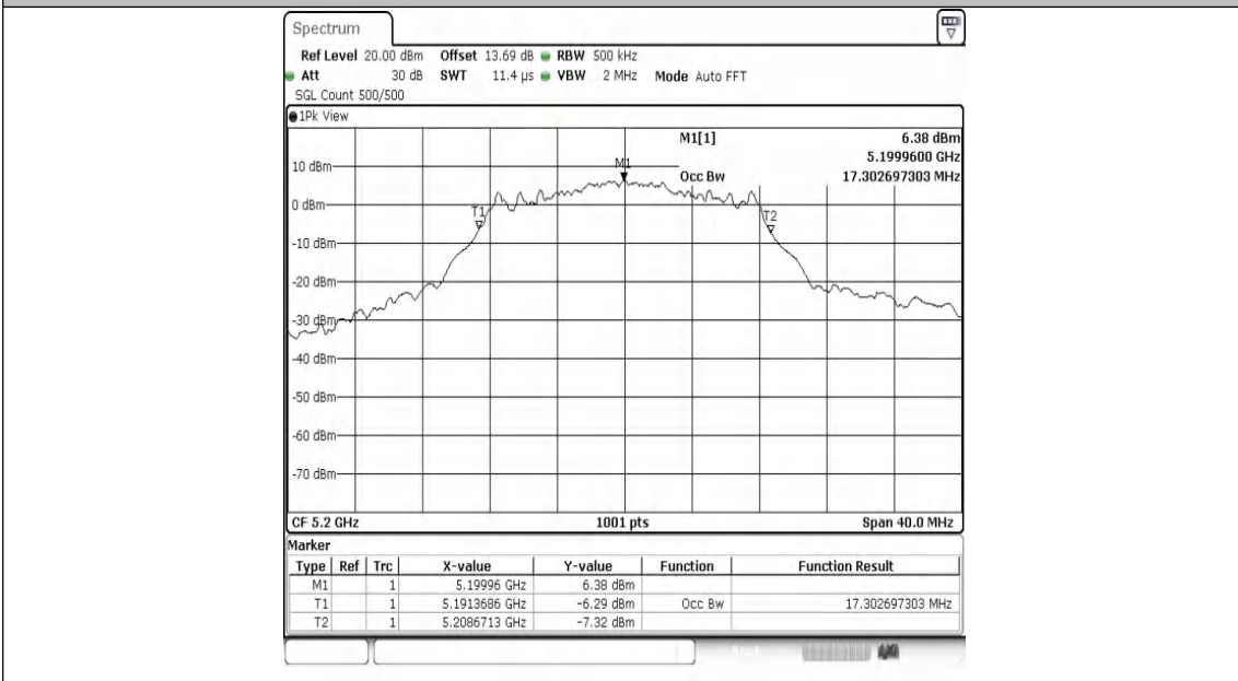
11A-Ant2-5200
