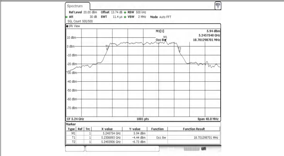
11AC20MIMO-Ant2-5240
