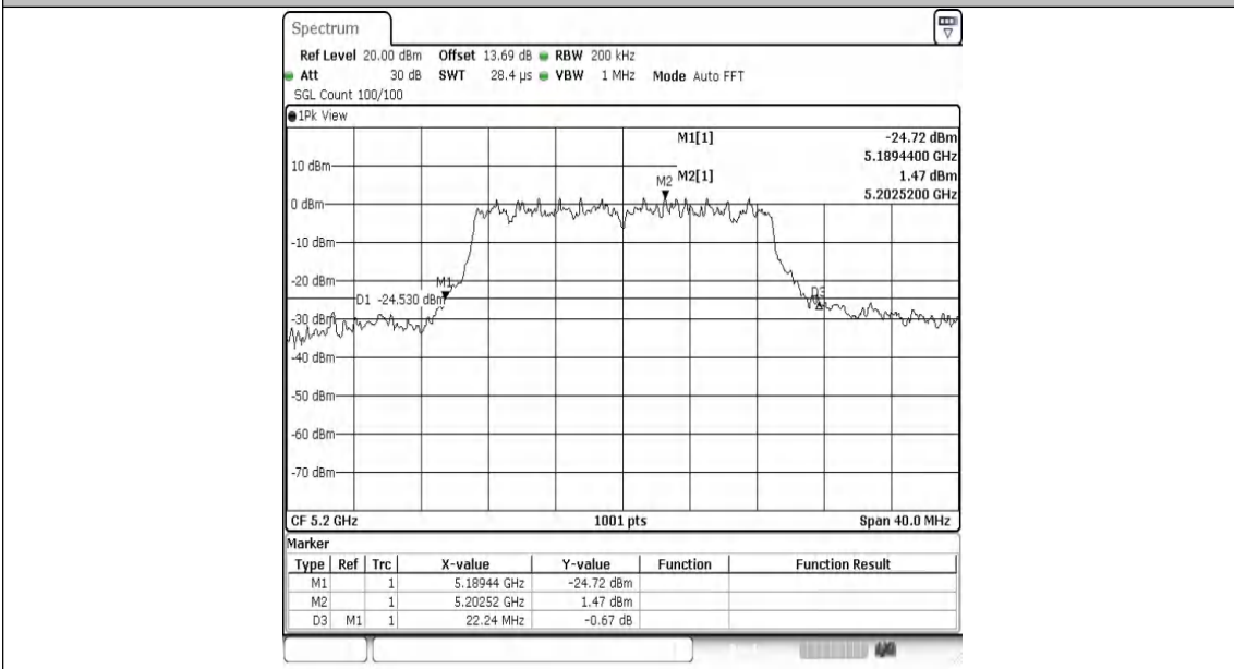
11AC20MIMO-Ant2-5200
