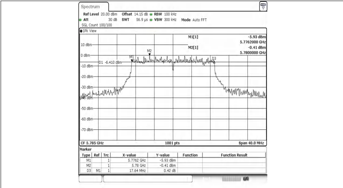
11N20MIMO-Ant1-5785-PASS
