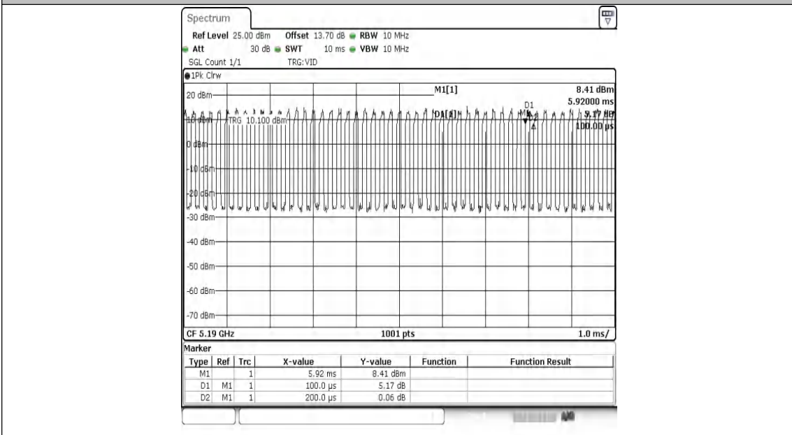
NTNV-11N40MIMO-Ant2-5190
