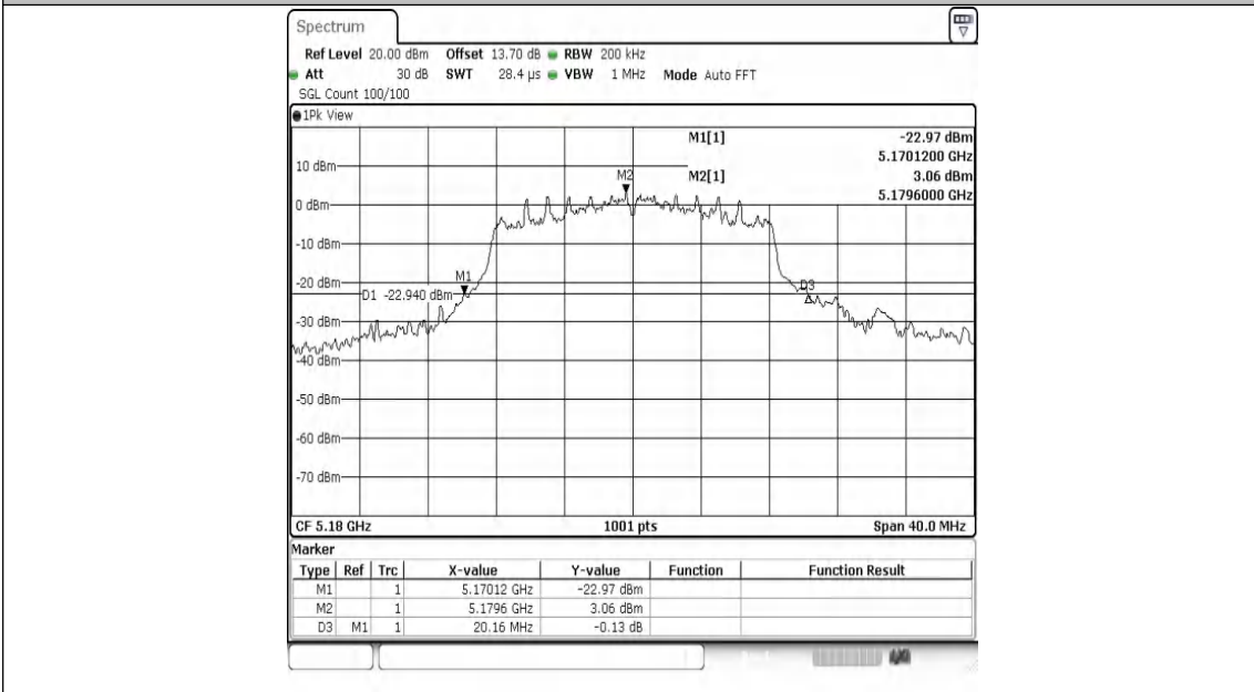
11A-Ant2-5180
