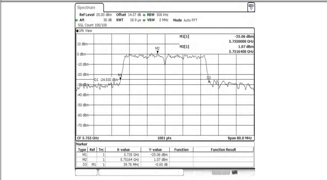
11N40MIMO-Ant2-5755
