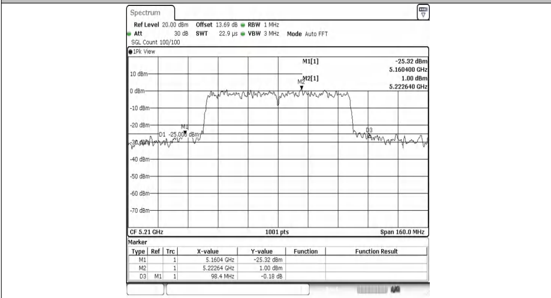
11AC80MIMO-Ant2-5210
