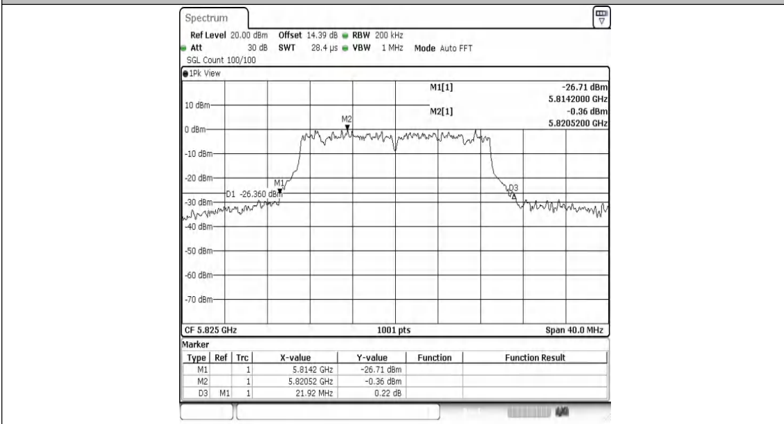
11AC20MIMO-Ant2-5825
