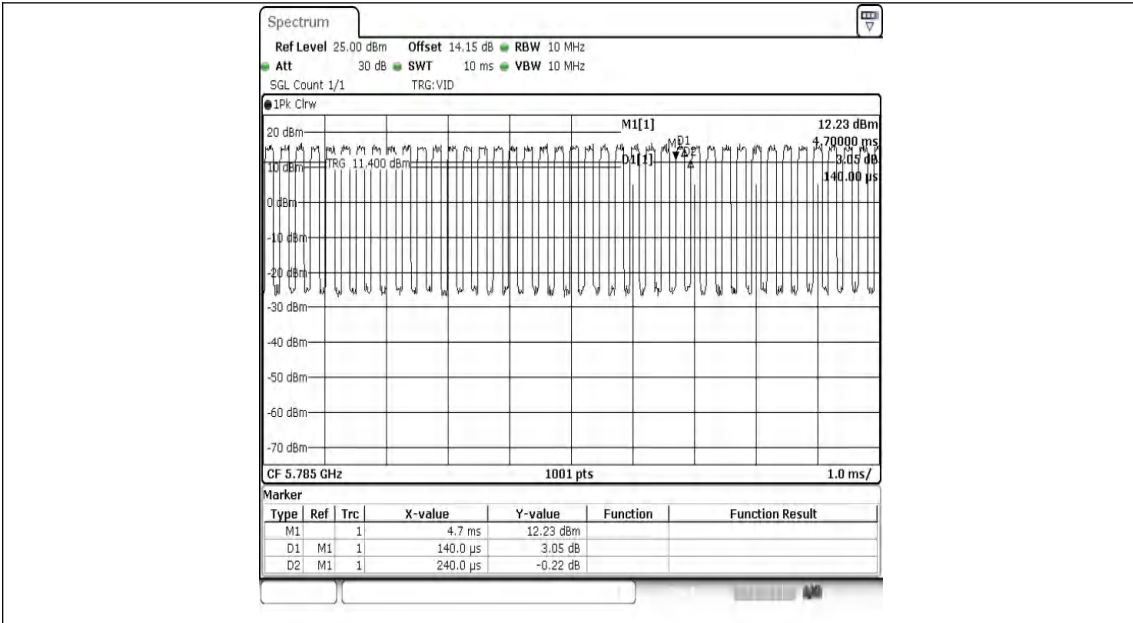
NTNV-11AC20MIMO-Ant1-5785
