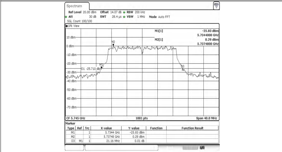
11AC20MIMO-Ant2-5745
