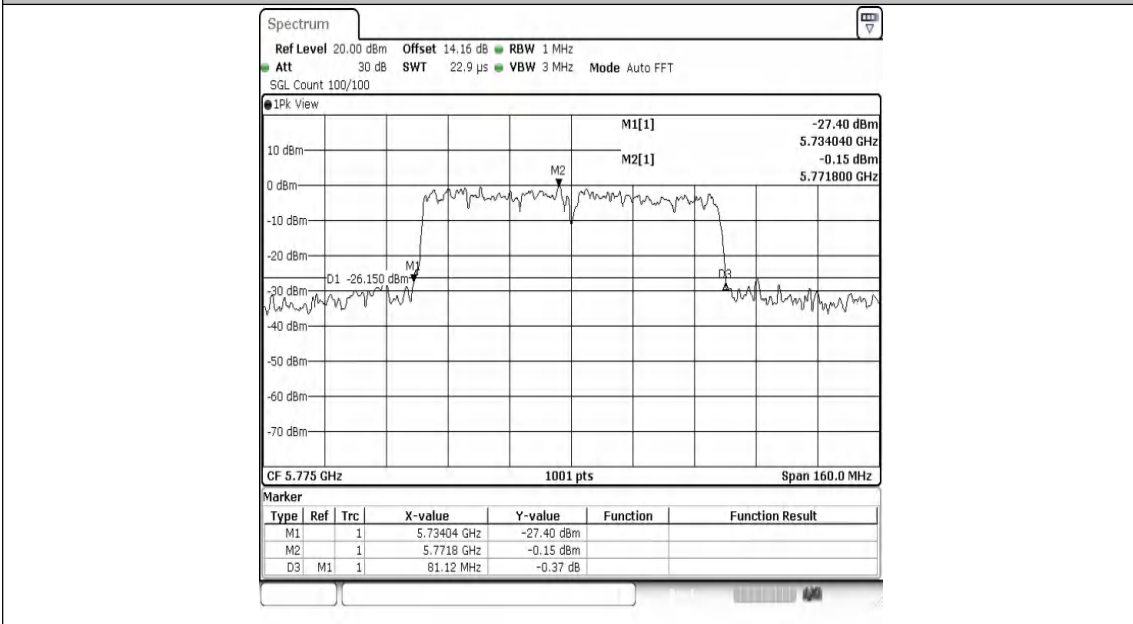
11AC80MIMO-Ant2-5775
