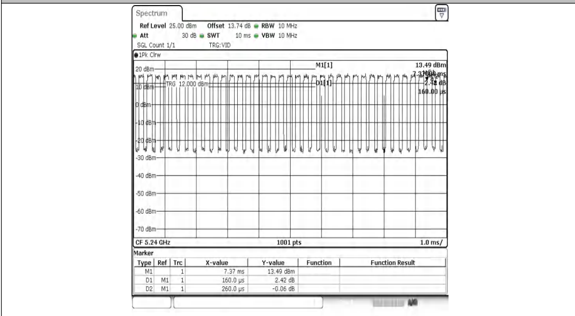
NTVN-11N20MIMO-Ant2-5240
