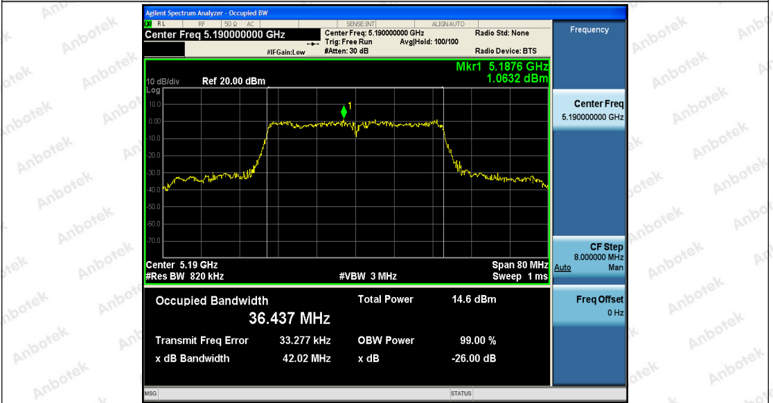
11AC40SISO_Ant2_5190
