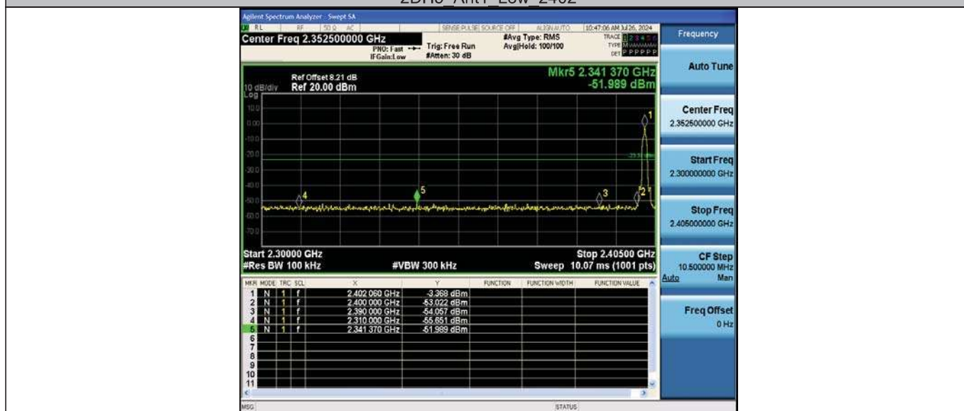
2DH5_Ant2_Low_2402
