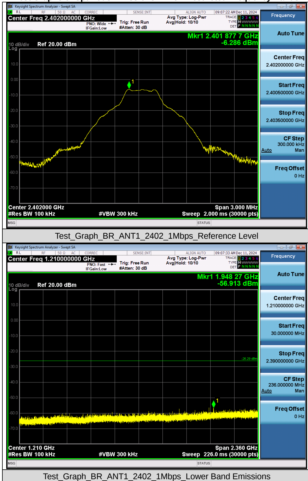
Test Graphs of Spurious Emissions in Non-Restricted Frequency Bands
