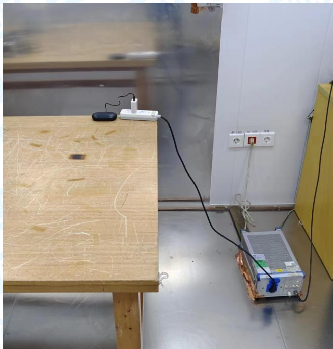
Photo of Setup for Conducted Emission
