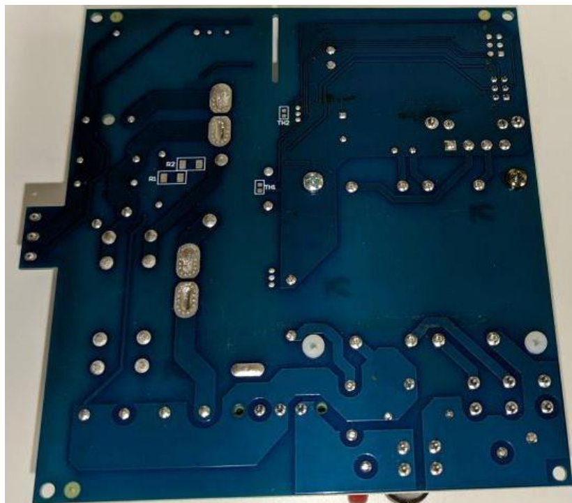
PCB125R7 bottom view
