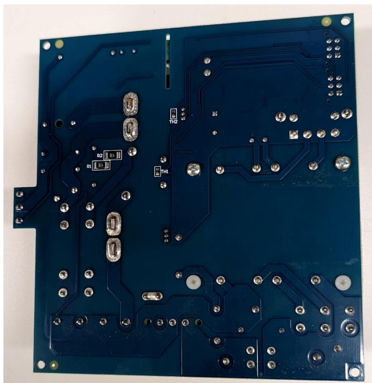
PCB125R7 bottom view
