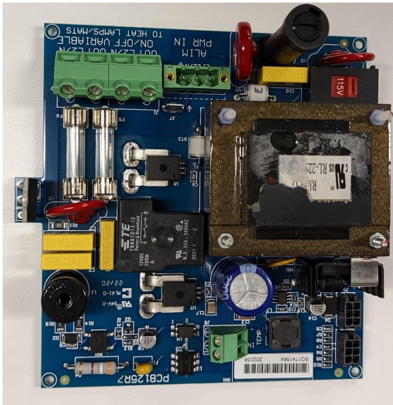
PCB125R7 top view
