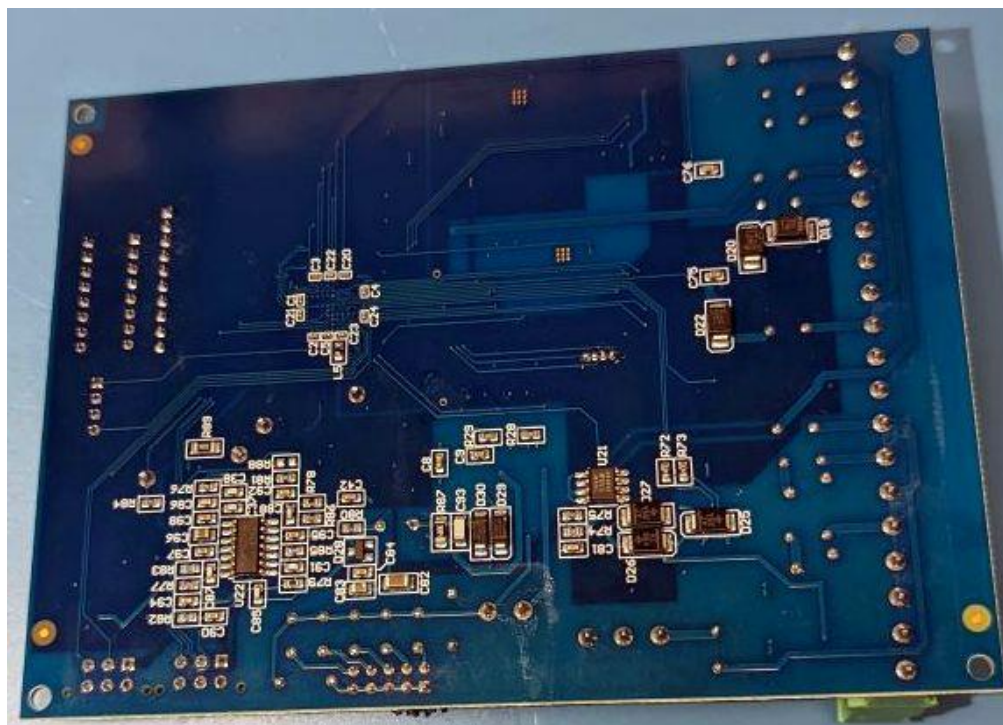
PCB124R5 bottom view
