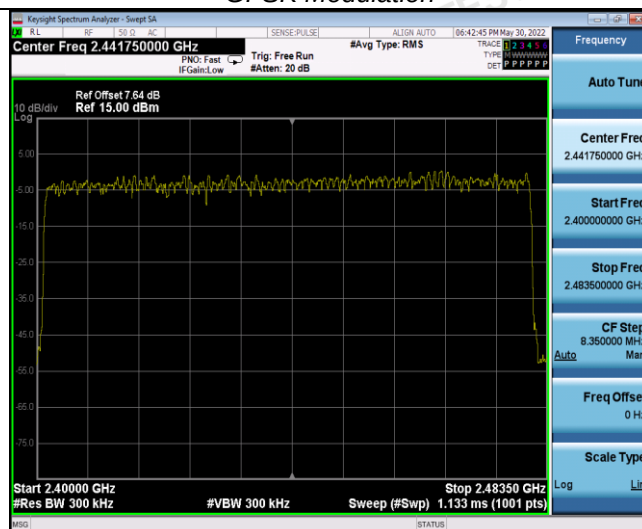
m/4DQPSK Modulation
