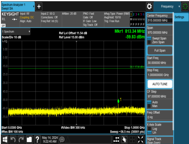
2DH5-Ant1-2441-30~1000-PASS
