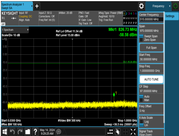
3DH5-Ant1-2480-30~1000-PASS
