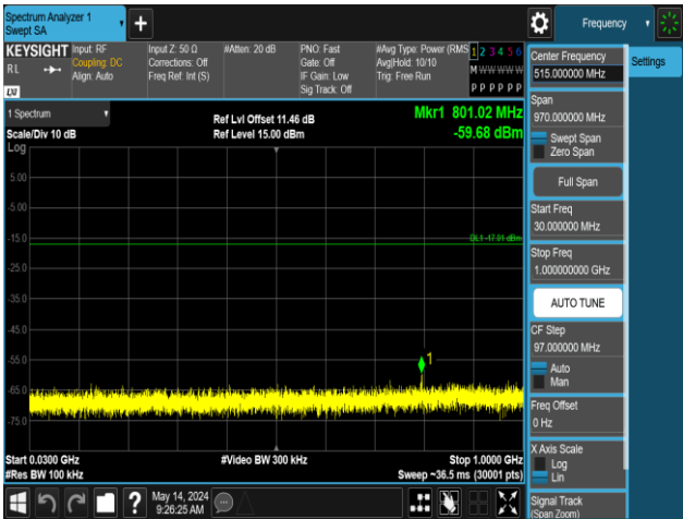
3DH5-Ant1-2402-30~1000-PASS
