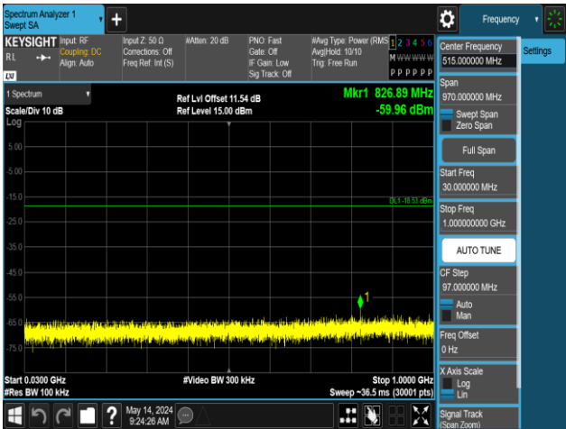
2DH5-Ant1-2480-30~1000-PASS
