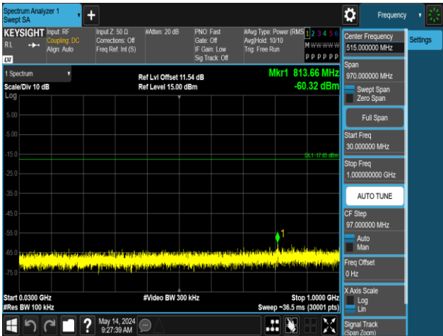
3DH5-Ant1-2441-30~1000-PASS
