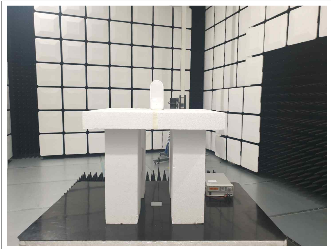
Radiated Emission Test Setup Above 1GHz_H
