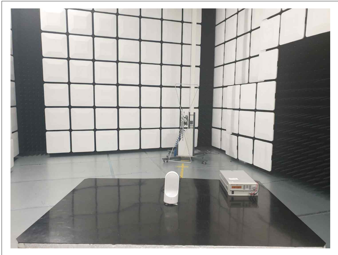
Radiated Emission Test Setup Below 1GHz_V
