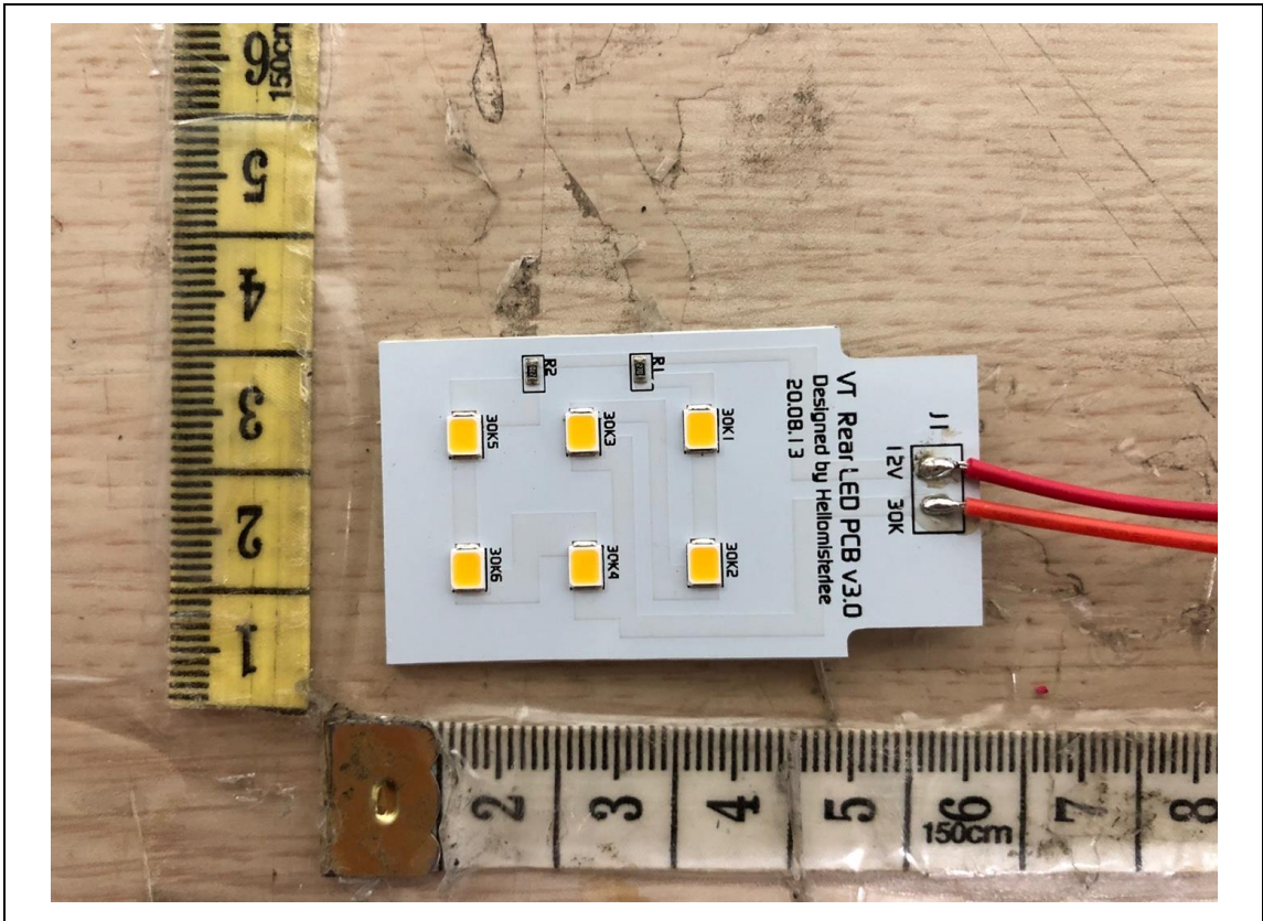
Sub Board 1(Front)
