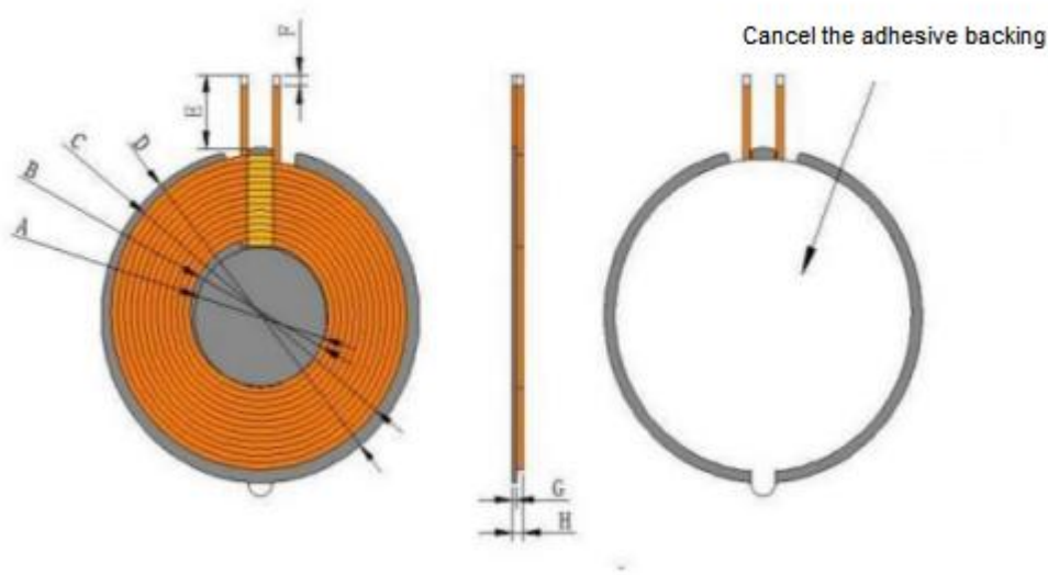
外形图/OUTSIDE DIAGRA
