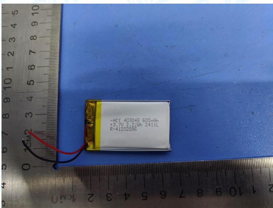
Photo 16 Battery Appearance
