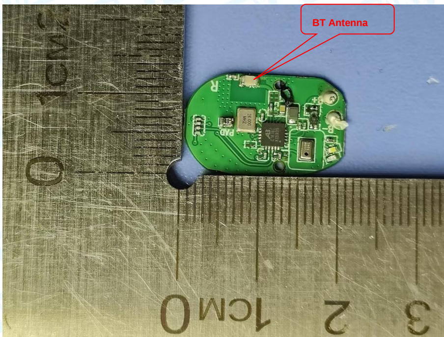
Photo 12 Appearance of PCB (Right)
