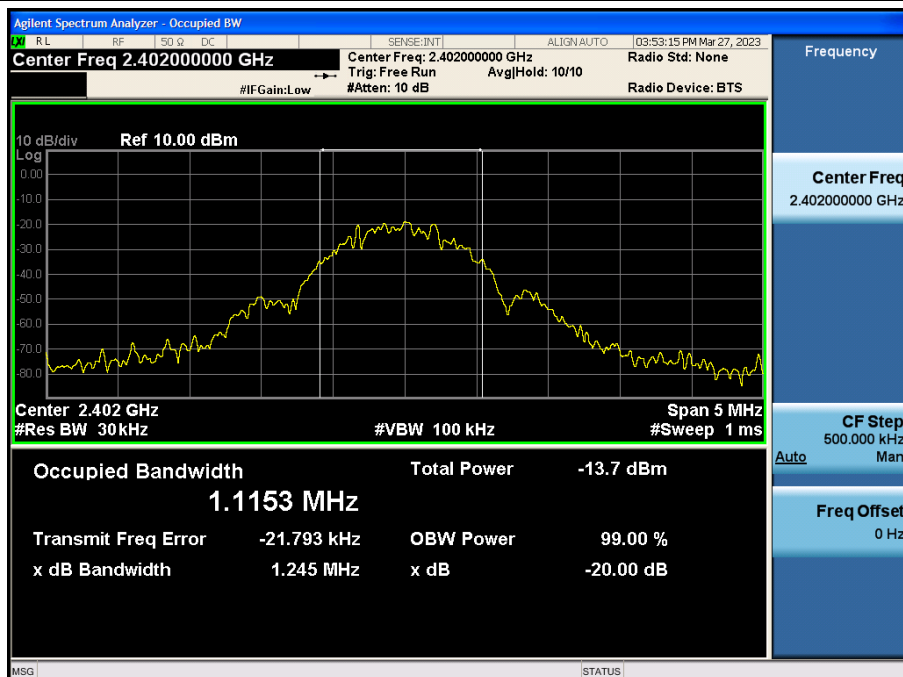
2402MHz-99% bandwidth
