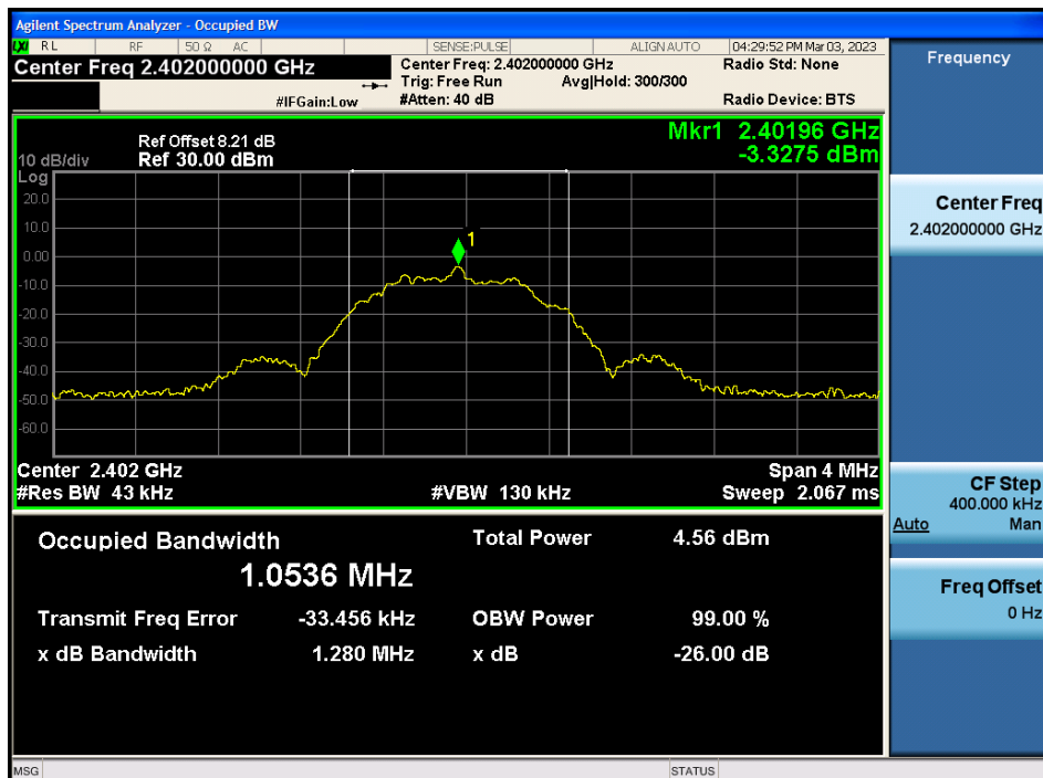
2402MHz-99% bandwidth
