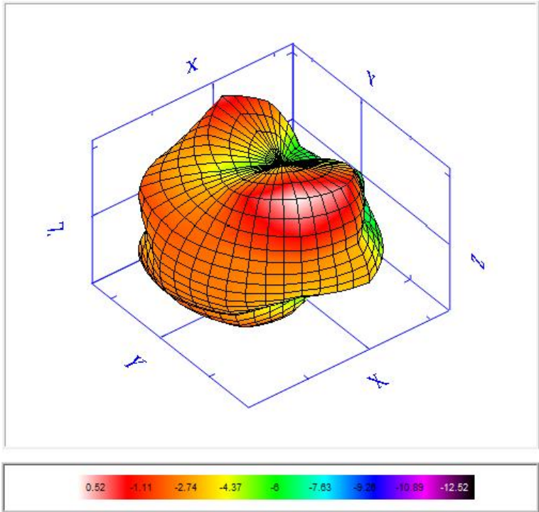
ZY plane 2450MHz
