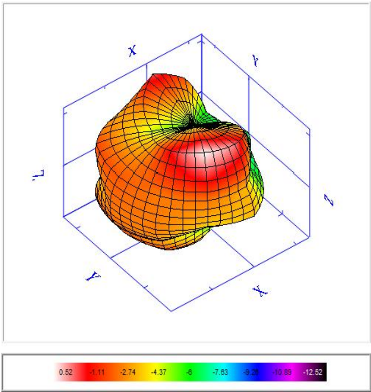
ZX plane 2450MHz
