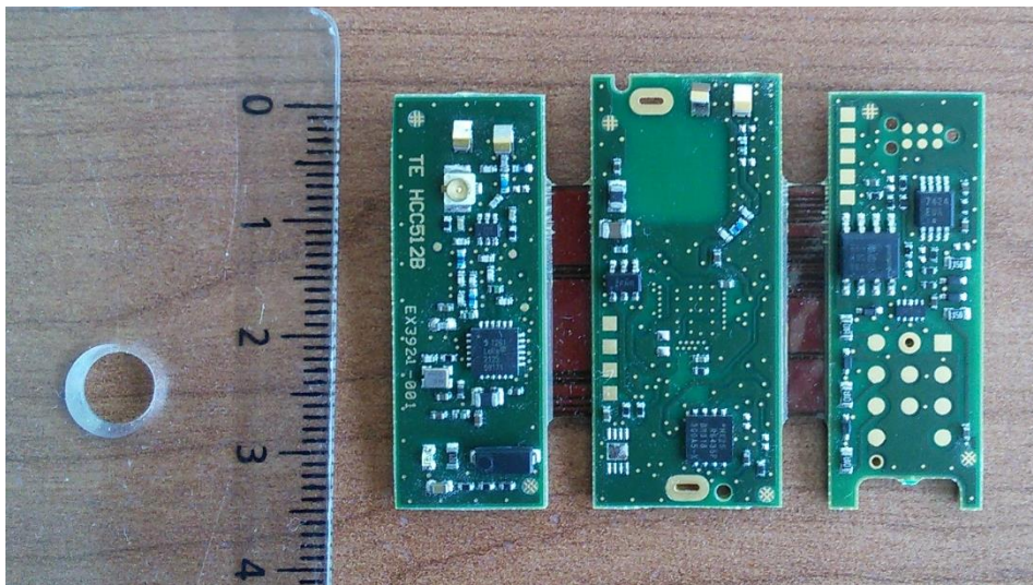
PCB Top view
