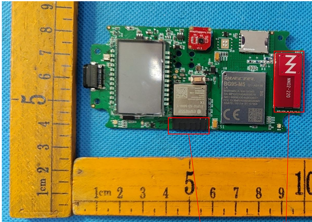
Wifi Antenna
