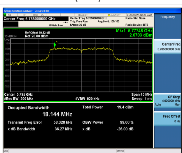
11ac (HT20) CH157
