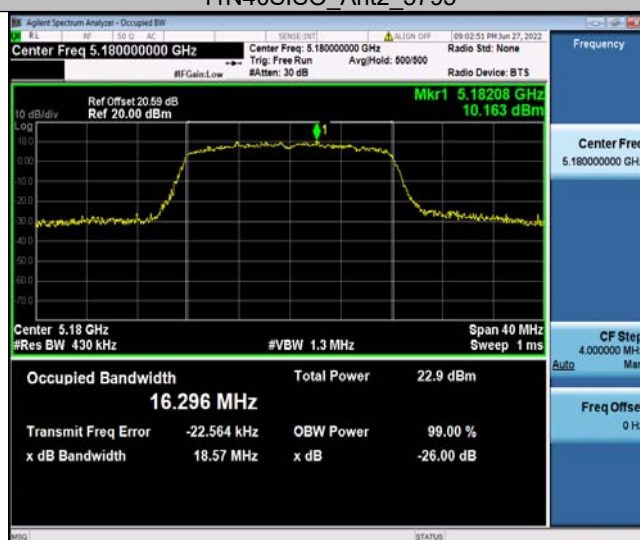
11AC20SISO_Ant1_5180
