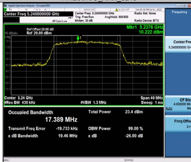
11N20SISO_Ant2_5240
