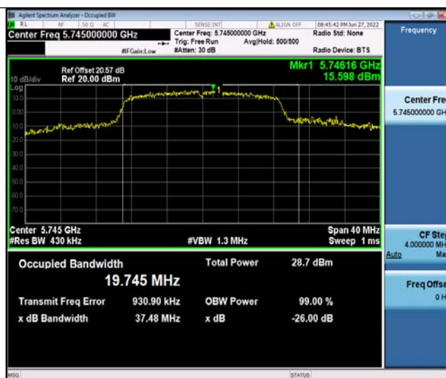
11N20SISO_Ant1_5745
