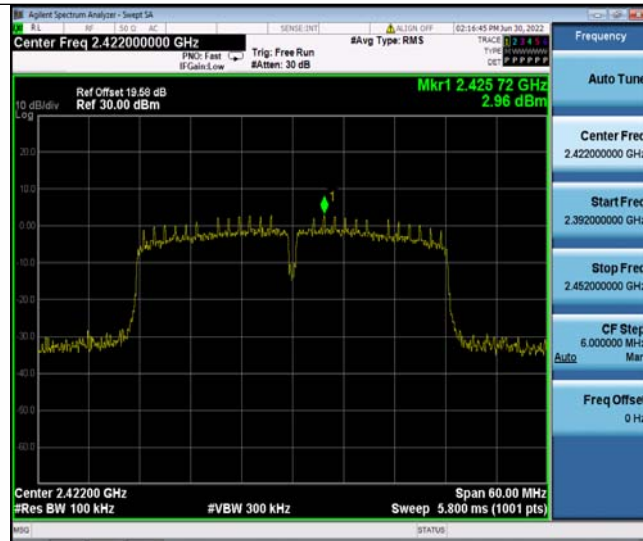
11N40SISO_Ant1_2422_0~Reference
