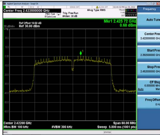
11N40SISO_Ant2_2422_0~Reference
