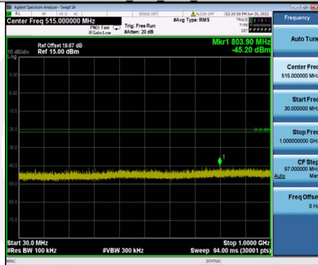
11N40SISO_Ant1_2452_30~1000
