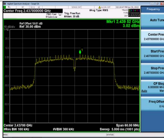
11N40SISO_Ant1_2437_0~Reference
