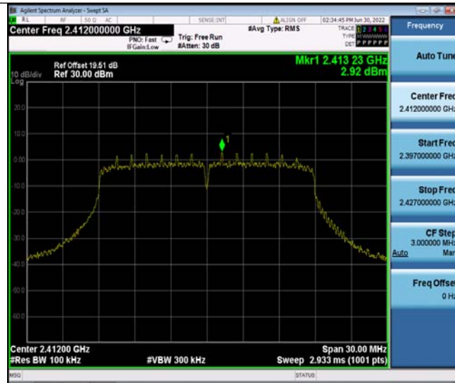
11N20SISO_Ant2_2412_0~Reference
