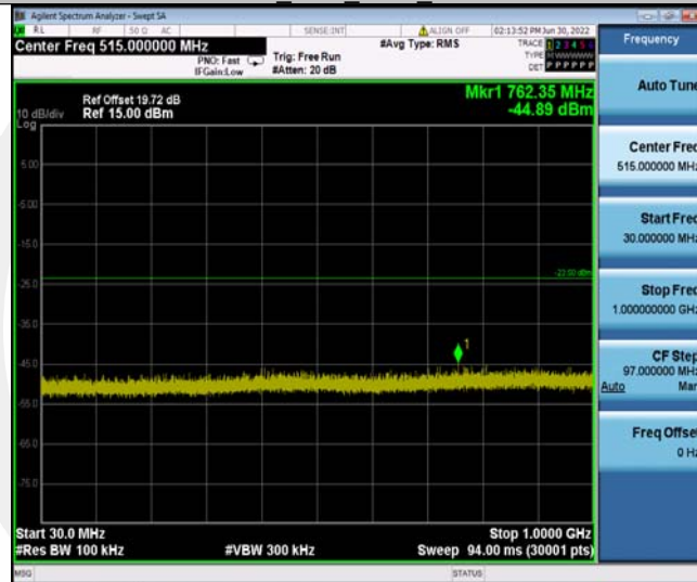
11N20SISO_Ant1_2462_30~1000
