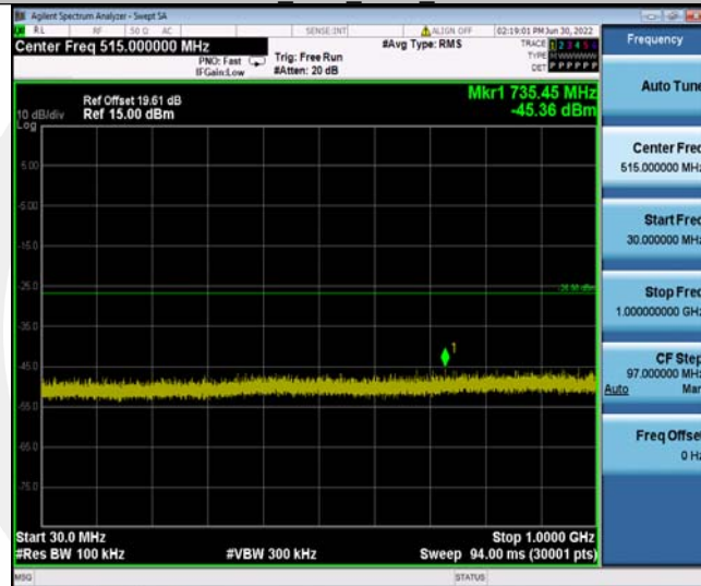
11N40SISO_Ant1_2437_30~1000
