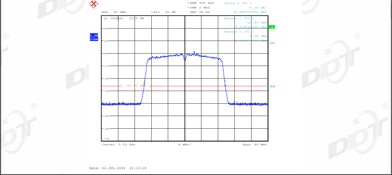
11AC40MIMO Ant1 5270
