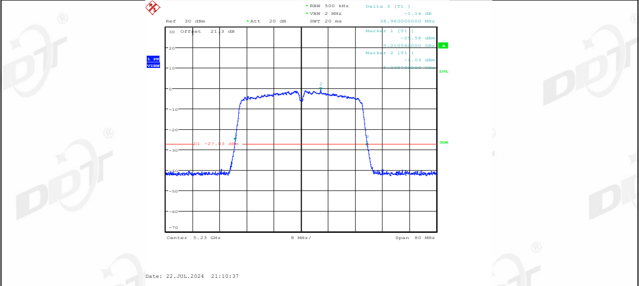
11AC40MIMO Ant2 5230
