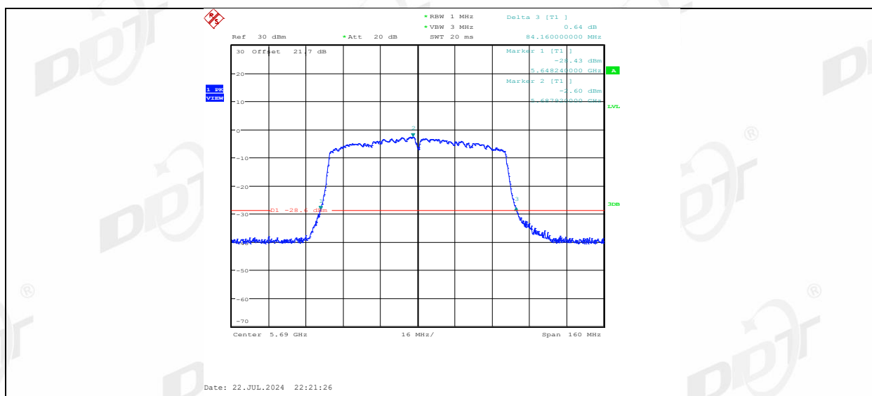
11AC80MIMO Ant2 5690
