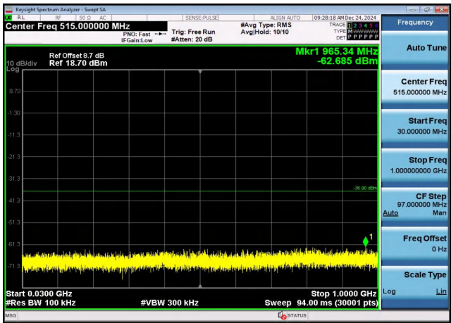
30MHz-1GHz
