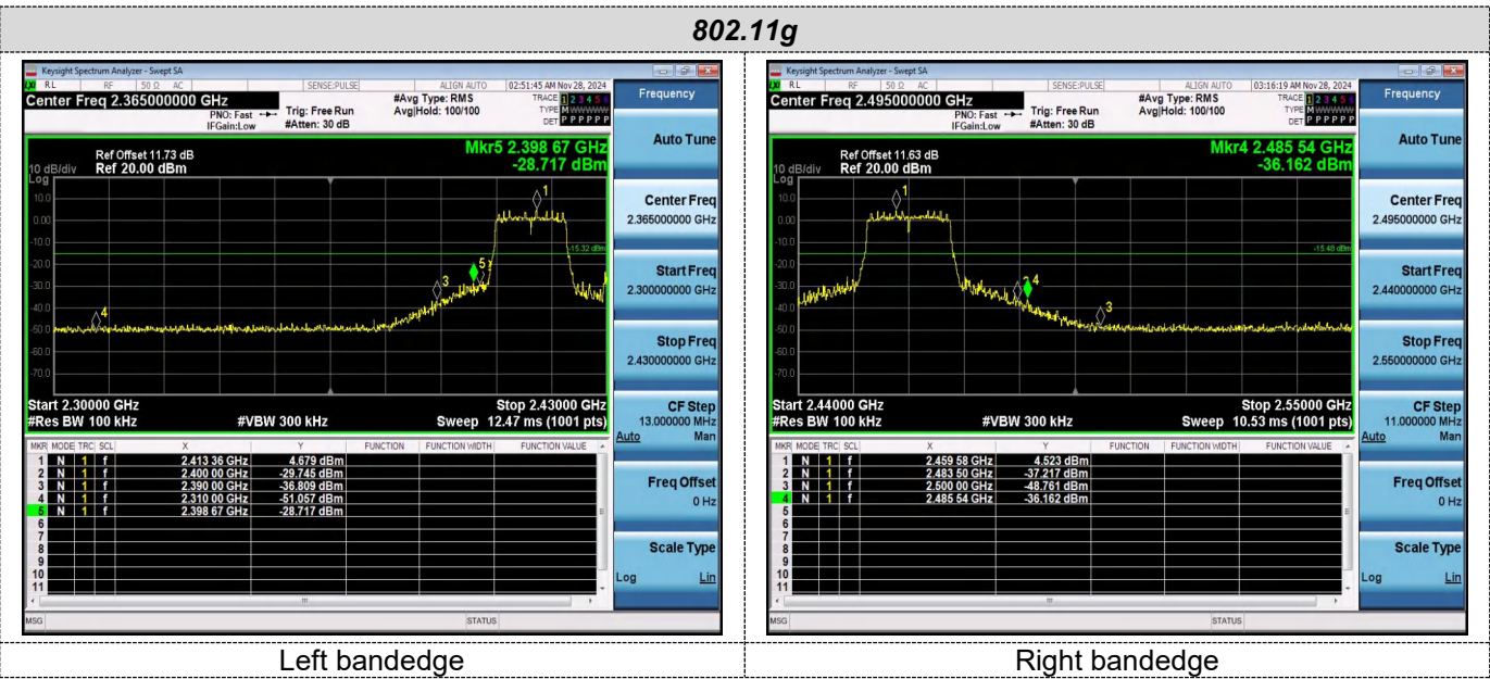
Left bandedge
