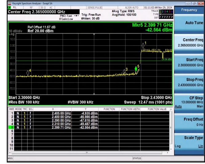
Left bandedge
