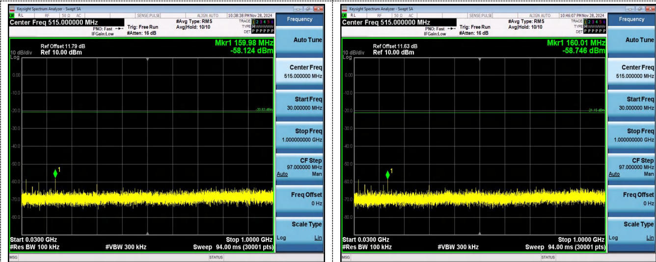
30MHz-1GHz
