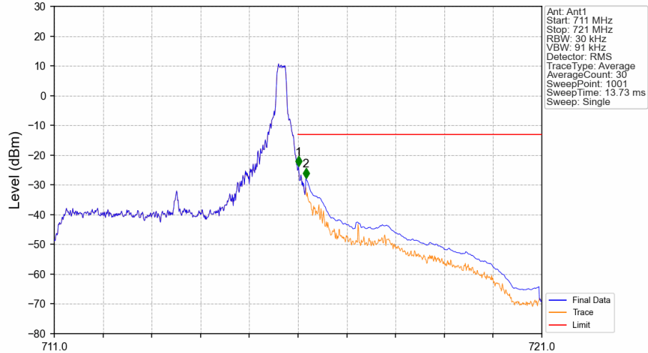
Band17_5MHz_QPSK_HCH_713.5MHz_RB_1_24_NTNV
