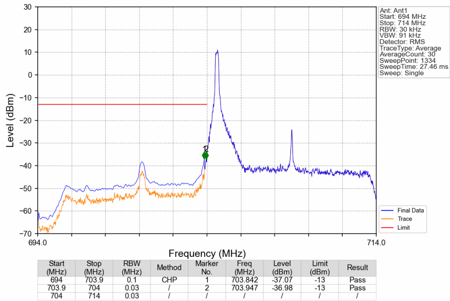
Band17 10MHz QPSK LCH 709MHz RB 1 0 NTN
