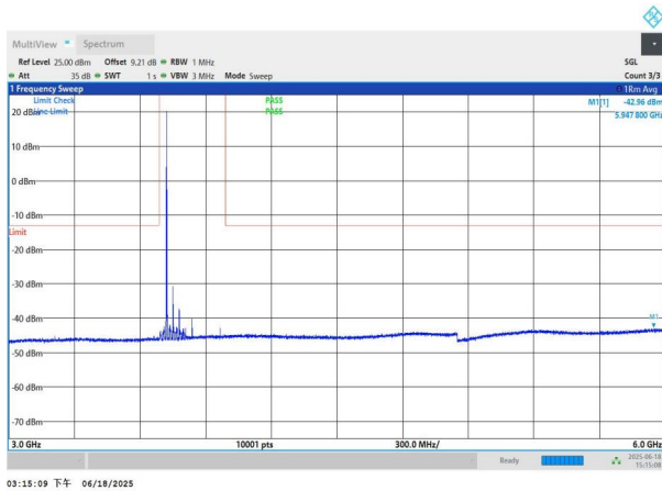
NTNV-n78(3700-3800)-PC3-30-60-M-DFT-BPSK-Edge_1RB_Left -3000-6000-PASS
