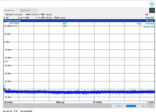
NTNV-n78(3700-3800)-PC3-30-70-M-DFT-QPSK-Edge_1RB_Left -30-1000-PASS
