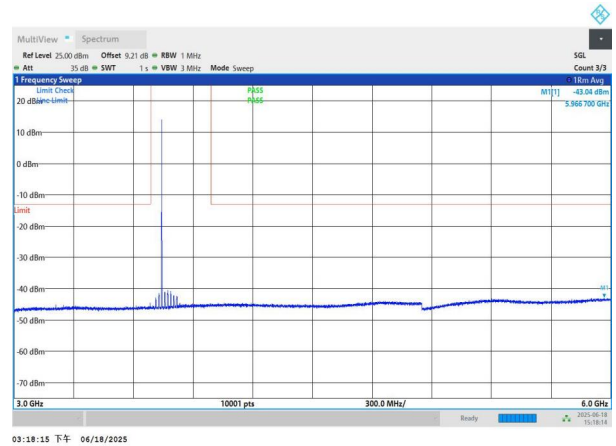
NTNV-n78(3700-3800)-PC3-30-60-H-DFT-QPSK-Edge_1RB_Left -3000-6000-PASS
