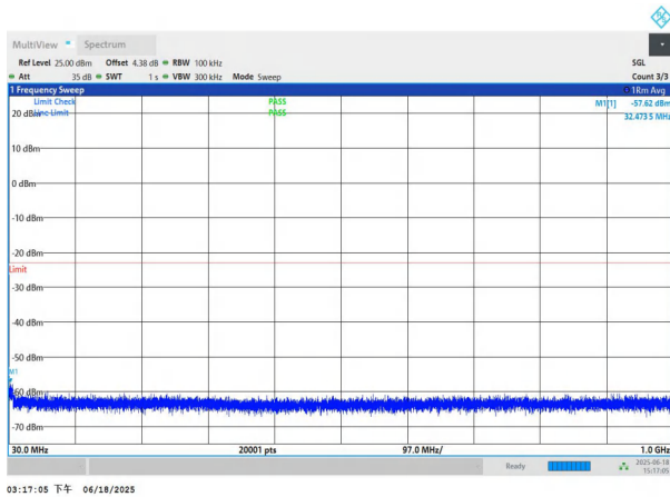
NTNV-n78(3700-3800)-PC3-30-60-H-DFT-BPSK-Edge_1RB_Left -30-1000-PASS
