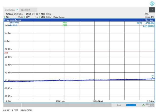
NTNV-n78(3700-3800)-PC3-30-70-L-DFT-BPSK-Edge_1RB_Left- 1000-3000-PASS
