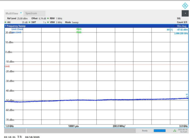
NTNV-n78(3700-3800)-PC3-30-60-M-DFT-BPSK-Edge_1RB_Left -1000-3000-PASS
