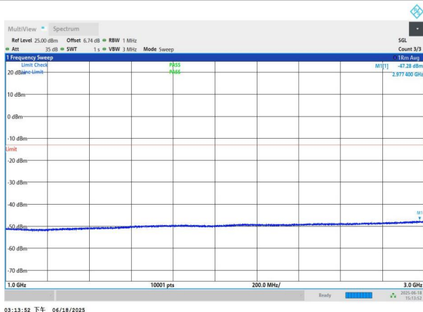
NTNV-n78(3700-3800)-PC3-30-60-L-DFT-QPSK-Edge_1RB_Left- 1000-3000-PASS
