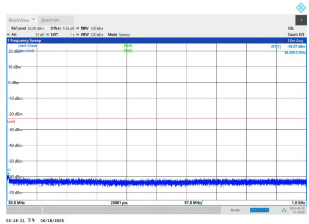
NTNV-n78(3700-3800)-PC3-30-60-H-DFT-QPSK-Edge_1RB_Left -30-1000-PASS
