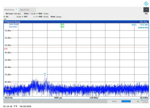
NTNV-n78(3700-3800)-PC3-30-70-L-DFT-BPSK-Edge_1RB_Left- 0.15-30-PASS
