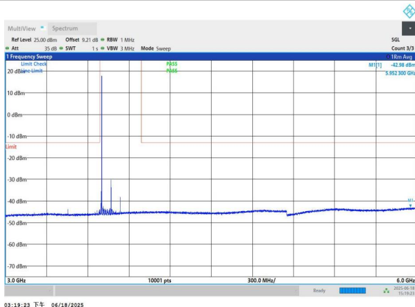
NTNV-n78(3700-3800)-PC3-30-70-L-DFT-BPSK-Edge_1RB_Left- 3000-6000-PASS
