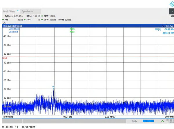
NTNV-n78(3700-3800)-PC3-30-70-L-DFT-QPSK-Edge_1RB_Left- 0.15-30-PASS
