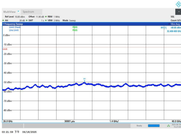
NTNV-n78(3700-3800)-PC3-30-70-M-DFT-BPSK-Edge_1RB_Left -26000-40000-PASS
