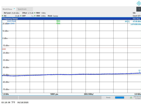
NTNV-n78(3700-3800)-PC3-30-60-H-DFT-QPSK-Edge_1RB_Left -1000-3000-PASS
