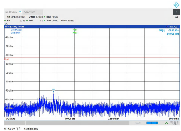
NTNV-n78(3700-3800)-PC3-30-60-M-DFT-BPSK-Edge_1RB_Left -0.15-30-PASS
