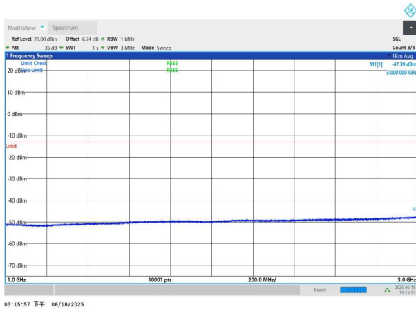
NTNV-n78(3700-3800)-PC3-30-60-M-DFT-QPSK-Edge_1RB_Left -1000-3000-PASS
