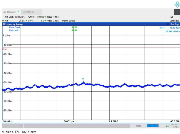
NTNV-n78(3700-3800)-PC3-30-60-L-DFT-BPSK-Edge_1RB_Left- 26000-40000-PASS
