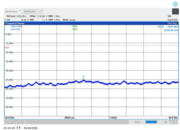
NTNV-n78(3700-3800)-PC3-30-60-M-DFT-QPSK-Edge_1RB_Left -26000-40000-PASS
