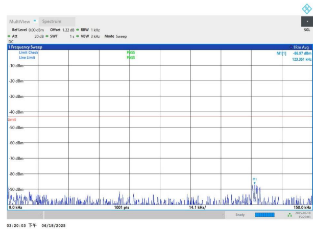
NTNV-n78(3700-3800)-PC3-30-70-L-DFT-QPSK-Edge_1RB_Left- 0.009-0.15-PASS
