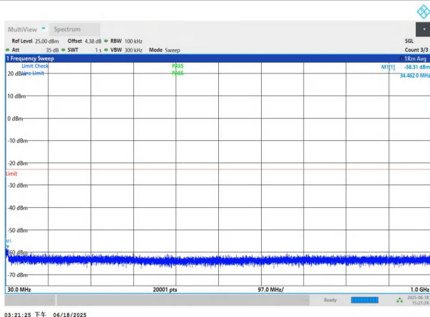
NTNV-n78(3700-3800)-PC3-30-70-M-DFT-BPSK-Edge_1RB_Left -30-1000-PASS
