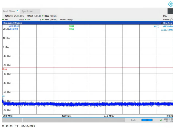
NTNV-n78(3700-3800)-PC3-30-70-L-DFT-BPSK-Edge_1RB_Left- 30-1000-PASS
