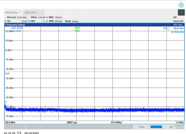
NTNV-n78(3700-3800)-PC3-30-60-M-DFT-QPSK-Edge_1RB_Left -30-1000-PASS
