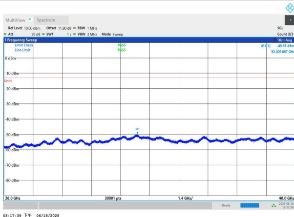
NTNV-n78(3700-3800)-PC3-30-60-H-DFT-BPSK-Edge_1RB_Left -26000-40000-PASS
