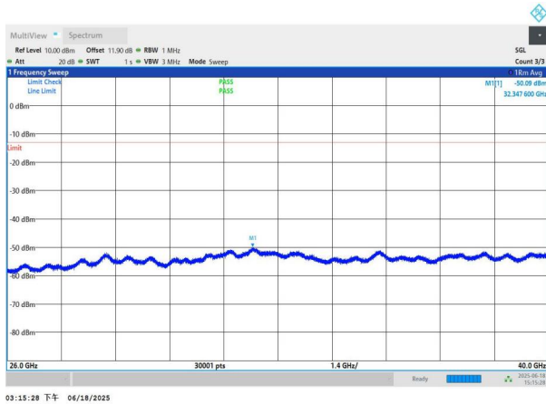
NTNV-n78(3700-3800)-PC3-30-60-M-DFT-BPSK-Edge_1RB_Left -26000-40000-PASS
