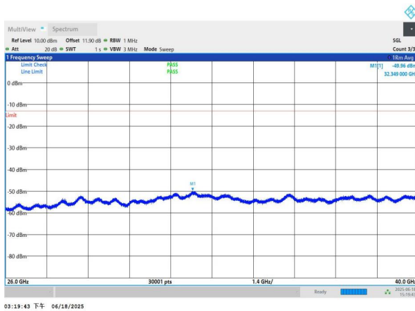
NTNV-n78(3700-3800)-PC3-30-70-L-DFT-BPSK-Edge_1RB_Left- 26000-40000-PASS
