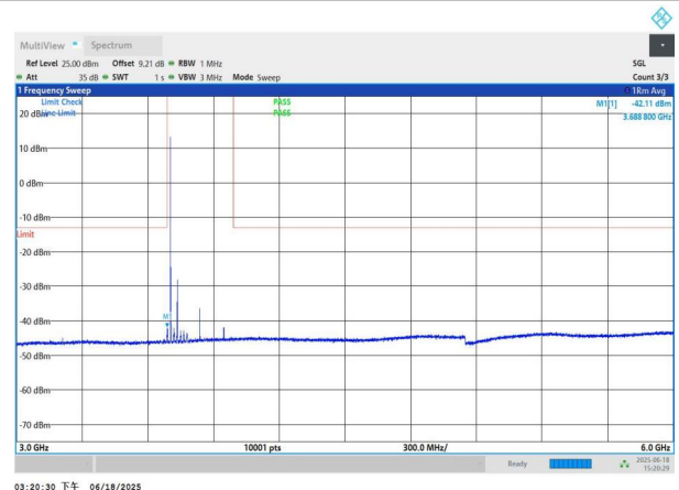
NTNV-n78(3700-3800)-PC3-30-70-L-DFT-QPSK-Edge_1RB_Left- 3000-6000-PASS
