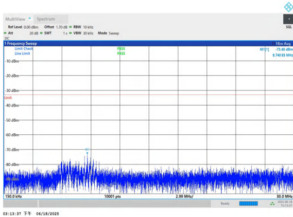
NTNV-n78(3700-3800)-PC3-30-60-L-DFT-QPSK-Edge_1RB_Left- 0.15-30-PASS
