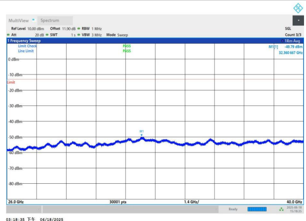
NTNV-n78(3700-3800)-PC3-30-60-H-DFT-QPSK-Edge_1RB_Left -26000-40000-PASS
