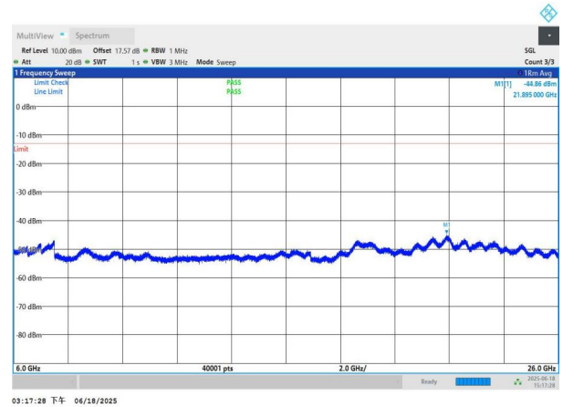
NTNV-n78(3700-3800)-PC3-30-60-H-DFT-BPSK-Edge_1RB_Left 6000-26000-PASS
