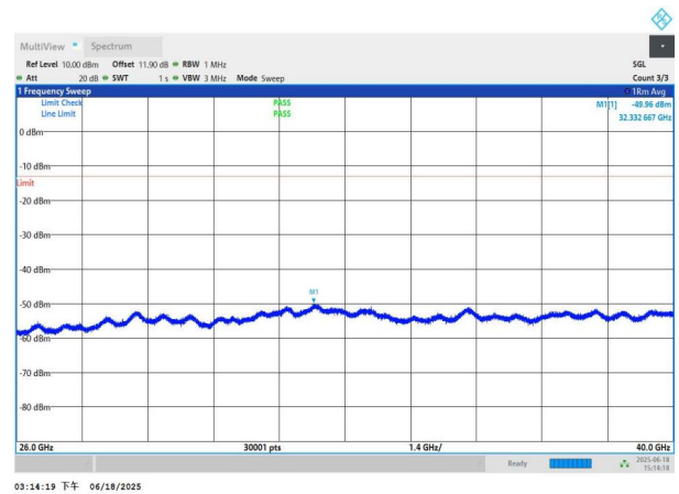
NTNV-n78(3700-3800)-PC3-30-60-L-DFT-QPSK-Edge_1RB_Left- 26000-40000-PASS
