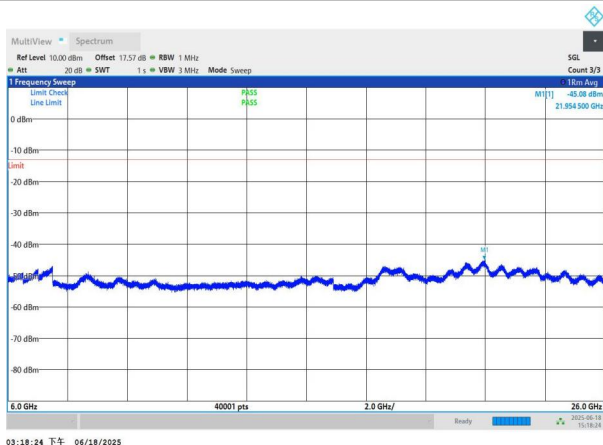
NTNV-n78(3700-3800)-PC3-30-60-H-DFT-QPSK-Edge_1RB_Left -6000-26000-PASS
