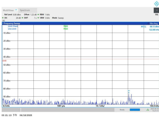
NTNV-n78(3700-3800)-PC3-30-70-M-DFT-BPSK-Edge_1RB_Left -0.009-0.15-PASS
