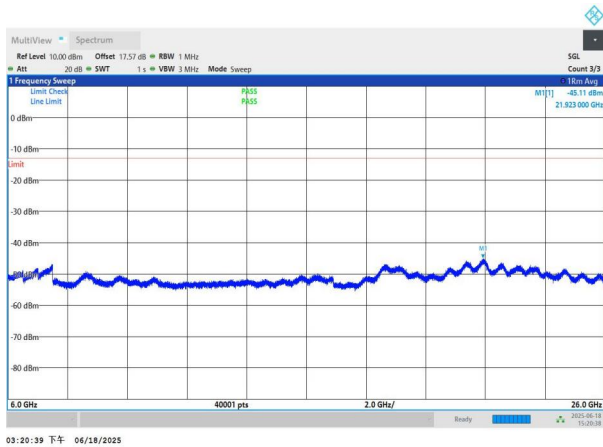
NTNV-n78(3700-3800)-PC3-30-70-L-DFT-QPSK-Edge_1RB_Left- 6000-26000-PASS
