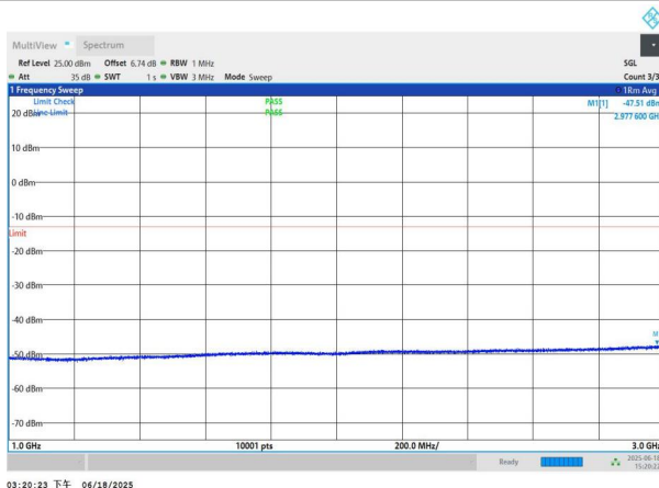
NTNV-n78(3700-3800)-PC3-30-70-L-DFT-QPSK-Edge_1RB_Left- 1000-3000-PASS
