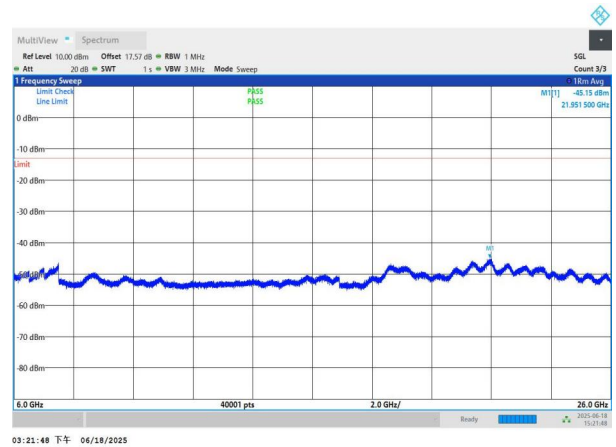
NTNV-n78(3700-3800)-PC3-30-70-M-DFT-BPSK-Edge_1RB_Left -6000-26000-PASS
