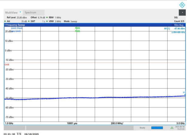
NTNV-n78(3700-3800)-PC3-30-70-M-DFT-BPSK-Edge_1RB_Left -1000-3000-PASS
