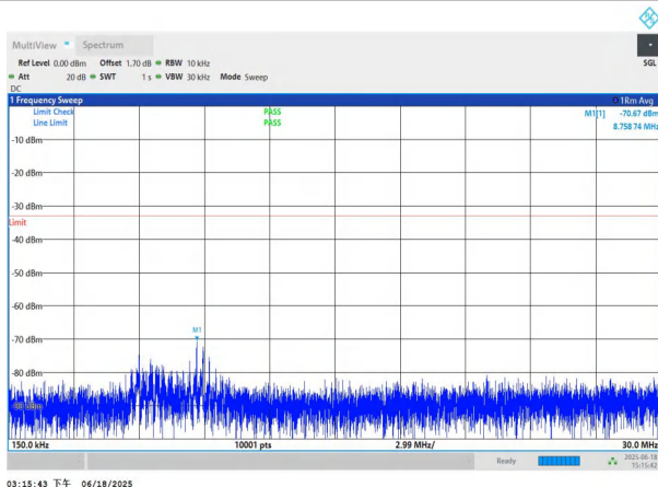
NTNV-n78(3700-3800)-PC3-30-60-M-DFT-QPSK-Edge_1RB_Left -0.15-30-PASS
