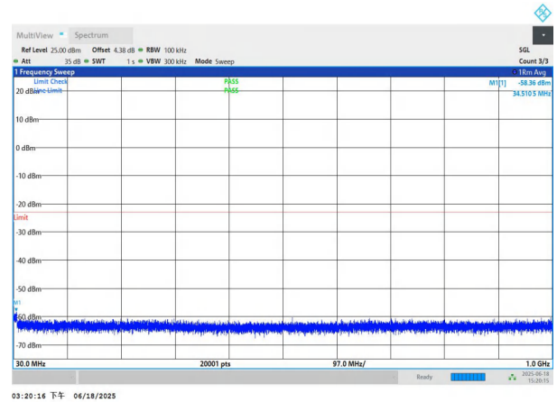
NTNV-n78(3700-3800)-PC3-30-70-L-DFT-QPSK-Edge_1RB_Left- 30-1000-PASS
