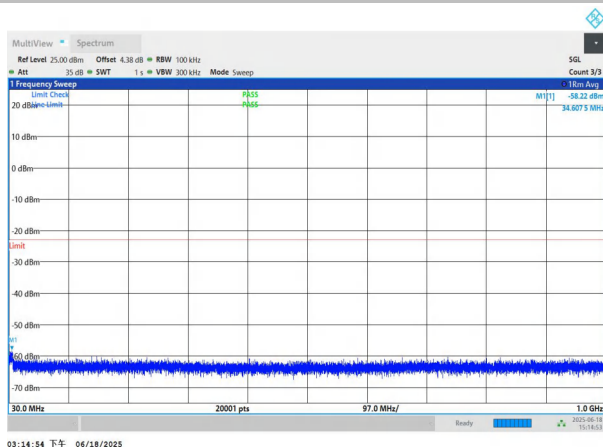
NTNV-n78(3700-3800)-PC3-30-60-M-DFT-BPSK-Edge_1RB_Left -30-1000-PASS
