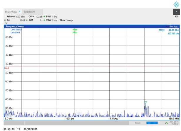
NTNV-n78(3700-3800)-PC3-30-60-L-DFT-QPSK-Edge_1RB_Left- 0.009-0.15-PASS
