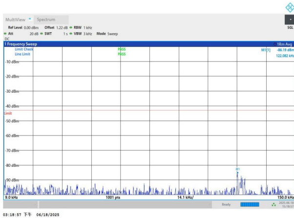
NTNV-n78(3700-3800)-PC3-30-70-L-DFT-BPSK-Edge_1RB_Left- 0.009-0.15-PASS
