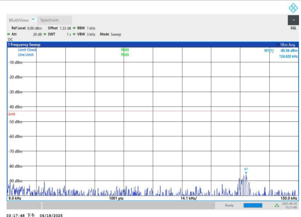
NTNV-n78(3700-3800)-PC3-30-60-H-DFT-QPSK-Edge_1RB_Left -0.009-0.15-PASS
