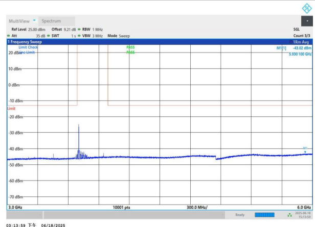
NTNV-n78(3700-3800)-PC3-30-60-L-DFT-QPSK-Edge_1RB_Left- 3000-6000-PASS
