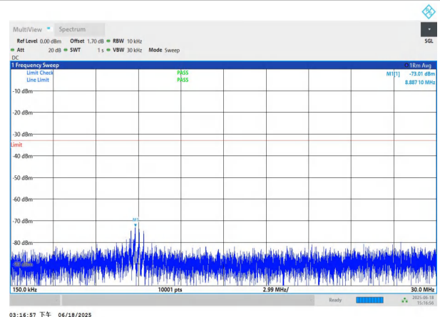
NTNV-n78(3700-3800)-PC3-30-60-H-DFT-BPSK-Edge_1RB_Left 0.15-30-PASS
