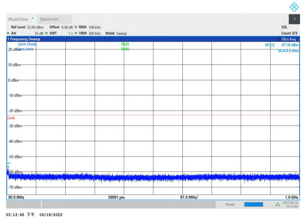
NTNV-n78(3700-3800)-PC3-30-60-L-DFT-QPSK-Edge_1RB_Left- 30-1000-PASS
