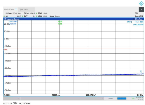
NTNV-n78(3700-3800)-PC3-30-60-H-DFT-BPSK-Edge_1RB_Left 1000-3000-PASS
