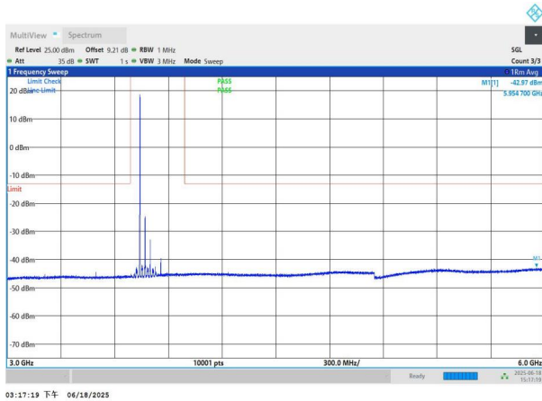
NTNV-n78(3700-3800)-PC3-30-60-H-DFT-BPSK-Edge_1RB_Left -3000-6000-PASS
