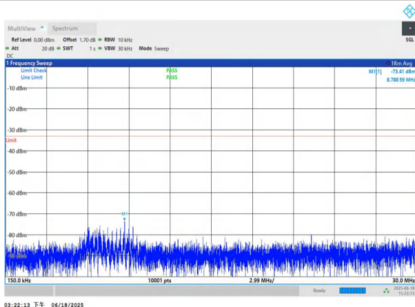
NTNV-n78(3700-3800)-PC3-30-70-M-DFT-QPSK-Edge_1RB_Left -0.15-30-PASS
