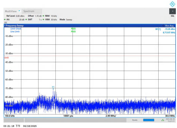
NTNV-n78(3700-3800)-PC3-30-70-M-DFT-BPSK-Edge_1RB_Left -0.15-30-PASS
