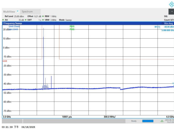
NTNV-n78(3700-3800)-PC3-30-70-M-DFT-BPSK-Edge_1RB_Left -3000-6000-PASS
