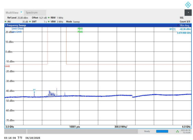
NTNV-n78(3700-3800)-PC3-30-60-M-DFT-QPSK-Edge_1RB_Left -3000-6000-PASS
