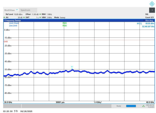
NTNV-n78(3700-3800)-PC3-30-70-L-DFT-QPSK-Edge_1RB_Left- 26000-40000-PASS
