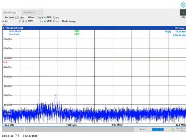
NTNV-n78(3700-3800)-PC3-30-60-H-DFT-QPSK-Edge_1RB_Left -0.15-30-PASS
