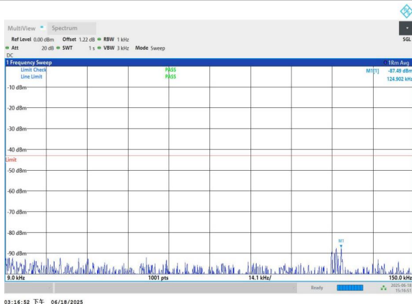
NTNV-n78(3700-3800)-PC3-30-60-H-DFT-BPSK-Edge_1RB_Left -0.009-0.15-PASS
