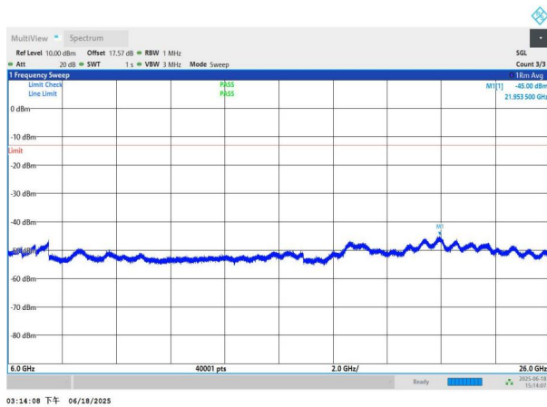
NTNV-n78(3700-3800)-PC3-30-60-L-DFT-QPSK-Edge_1RB_Left- 6000-26000-PASS
