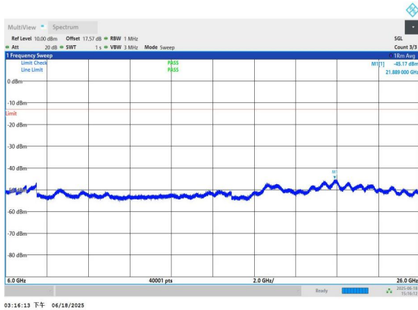
NTNV-n78(3700-3800)-PC3-30-60-M-DFT-QPSK-Edge_1RB_Left -6000-26000-PASS
