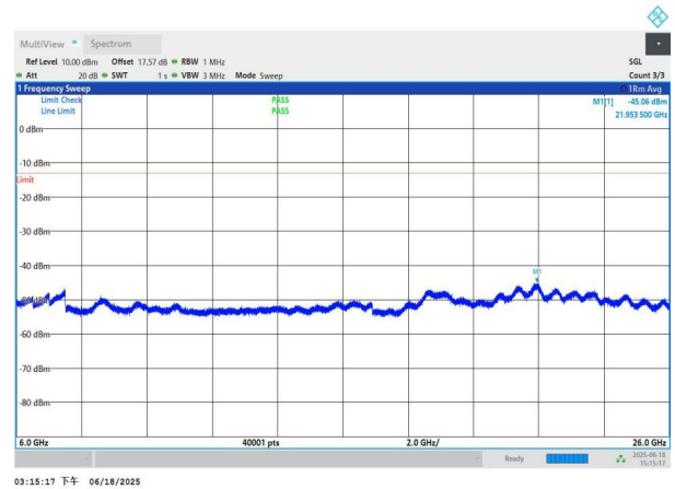
NTNV-n78(3700-3800)-PC3-30-60-M-DFT-BPSK-Edge_1RB_Left -6000-26000-PASS
