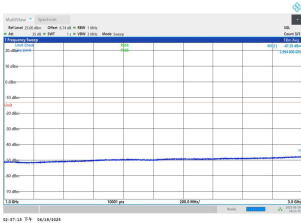
NTNV-n78(3700-3800)-PC3-30-30-H-DFT-QPSK-Edge_1RB_Left -1000-3000-PASS
