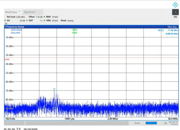
NTNV-n78(3700-3800)-PC3-30-30-H-DFT-BPSK-Edge_1RB_Left 0.15-30-PASS
