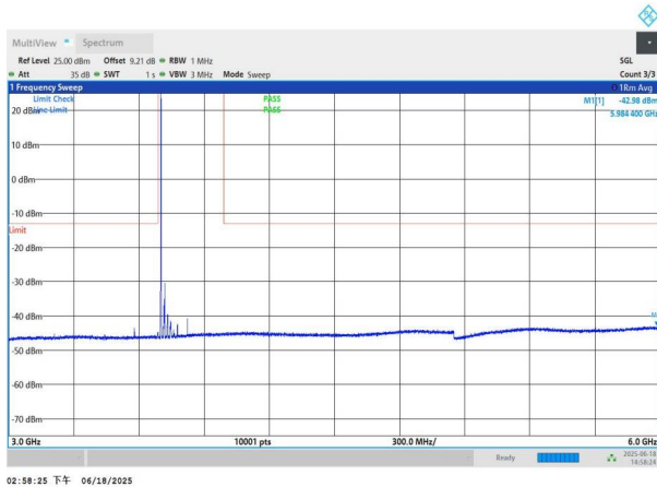
NTNV-n78(3700-3800)-PC3-30-40-L-DFT-BPSK-Edge_1RB_Left- 3000-6000-PASS
