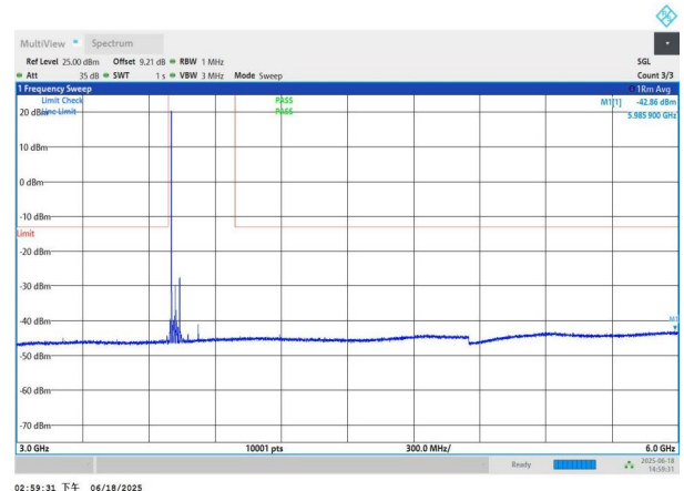
NTNV-n78(3700-3800)-PC3-30-40-L-DFT-QPSK-Edge_1RB_Left- 3000-6000-PASS
