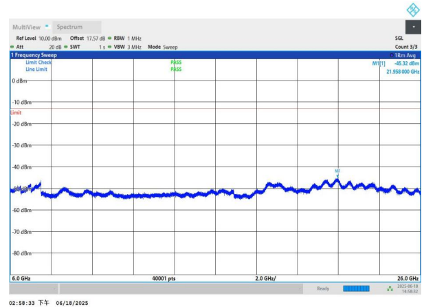
NTNV-n78(3700-3800)-PC3-30-40-L-DFT-BPSK-Edge_1RB_Left- 6000-26000-PASS
