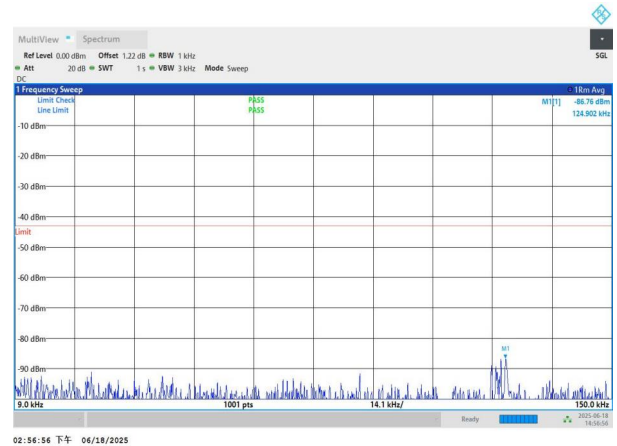
NTNV-n78(3700-3800)-PC3-30-30-H-DFT-QPSK-Edge_1RB_Left -0.009-0.15-PASS
