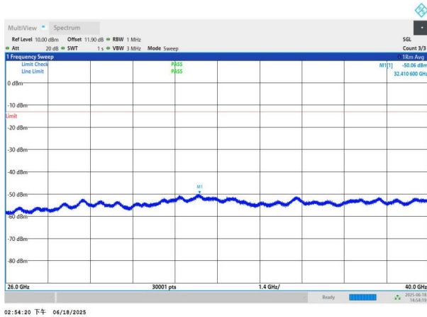
NTNV-n78(3700-3800)-PC3-30-30-M-DFT-BPSK-Edge_1RB_Left -26000-40000-PASS
