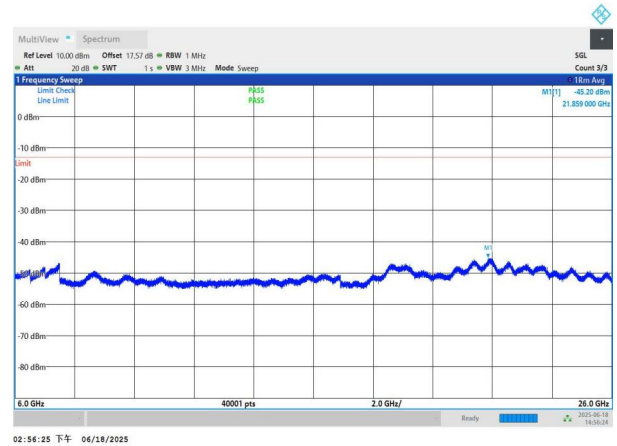
NTNV-n78(3700-3800)-PC3-30-30-H-DFT-BPSK-Edge_1RB_Left 6000-26000-PASS
