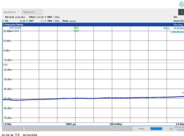
NTNV-n78(3700-3800)-PC3-30-40-L-DFT-QPSK-Edge_1RB_Left- 1000-3000-PASS
