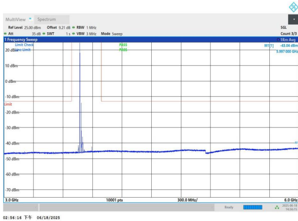
NTNV-n78(3700-3800)-PC3-30-30-H-DFT-BPSK-Edge_1RB_Left -3000-6000-PASS
