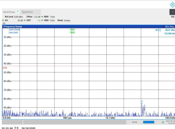
NTNV-n78(3700-3800)-PC3-30-40-H-DFT-BPSK-Edge_1RB_Left -0.009-0.15-PASS
