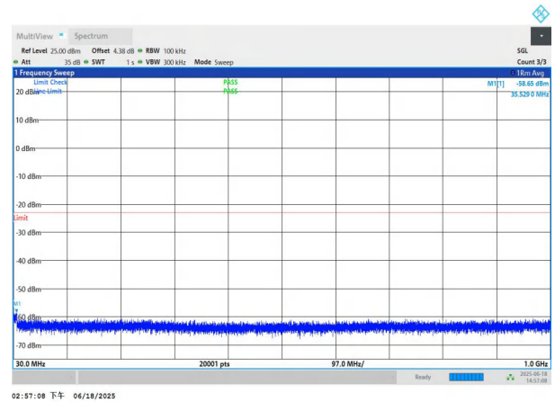
NTNV-n78(3700-3800)-PC3-30-30-H-DFT-QPSK-Edge_1RB_Left -30-1000-PASS
