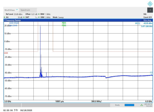
NTNV-n78(3700-3800)-PC3-30-30-M-DFT-QPSK-Edge_1RB_Left -3000-6000-PASS
