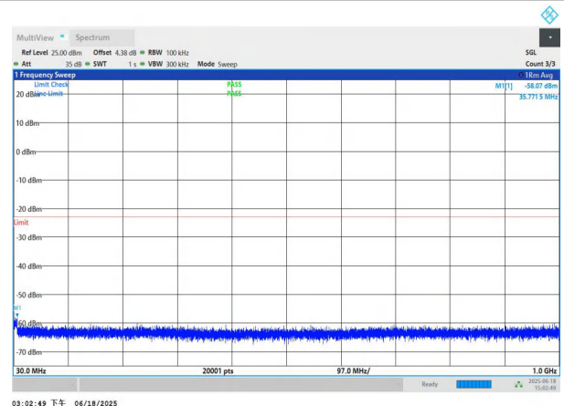
NTNV-n78(3700-3800)-PC3-30-40-M-DFT-QPSK-Edge_1RB_Left -30-1000-PASS
