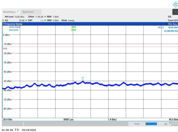
NTNV-n78(3700-3800)-PC3-30-40-L-DFT-BPSK-Edge_1RB_Left- 26000-40000-PASS
