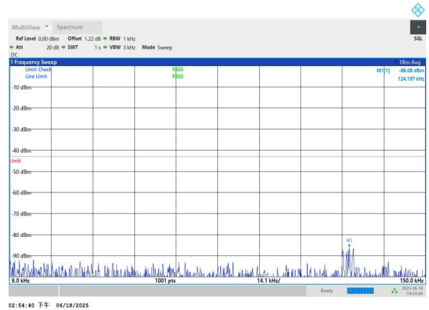
NTNV-n78(3700-3800)-PC3-30-30-M-DFT-QPSK-Edge_1RB_Left -0.009-0.15-PASS
