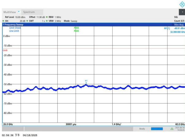
NTNV-n78(3700-3800)-PC3-30-30-H-DFT-BPSK-Edge_1RB_Left -26000-40000-PASS
