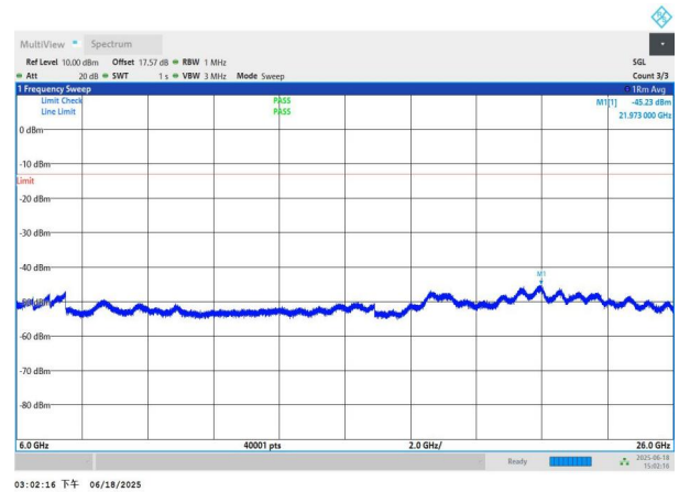
NTNV-n78(3700-3800)-PC3-30-40-M-DFT-BPSK-Edge_1RB_Left -6000-26000-PASS
