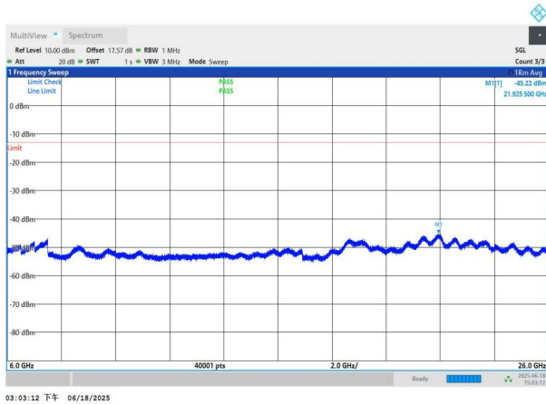
NTNV-n78(3700-3800)-PC3-30-40-M-DFT-QPSK-Edge_1RB_Left -6000-26000-PASS
