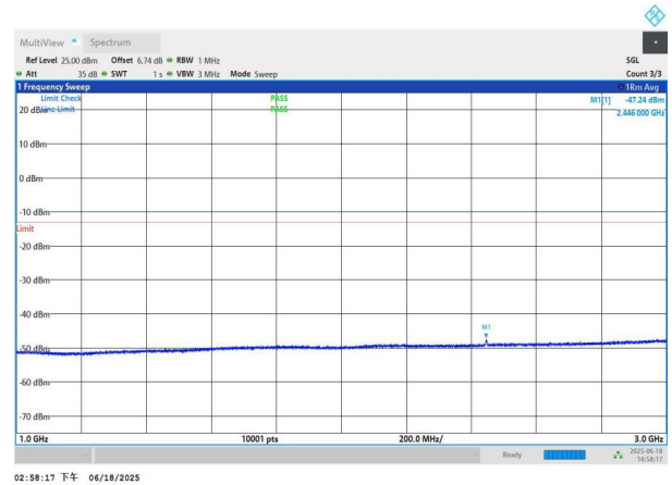
NTNV-n78(3700-3800)-PC3-30-40-L-DFT-BPSK-Edge_1RB_Left- 1000-3000-PASS
