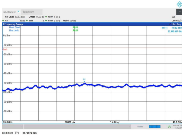
NTNV-n78(3700-3800)-PC3-30-40-M-DFT-BPSK-Edge_1RB_Left -26000-40000-PASS
