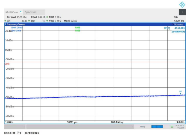
NTNV-n78(3700-3800)-PC3-30-30-H-DFT-BPSK-Edge_1RB_Left 1000-3000-PASS
