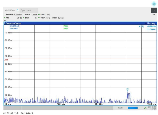
NTNV-n78(3700-3800)-PC3-30-40-L-DFT-QPSK-Edge_1RB_Left- 0.009-0.15-PASS
