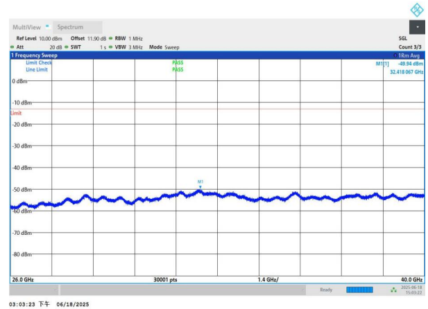
NTNV-n78(3700-3800)-PC3-30-40-M-DFT-QPSK-Edge_1RB_Left -26000-40000-PASS
