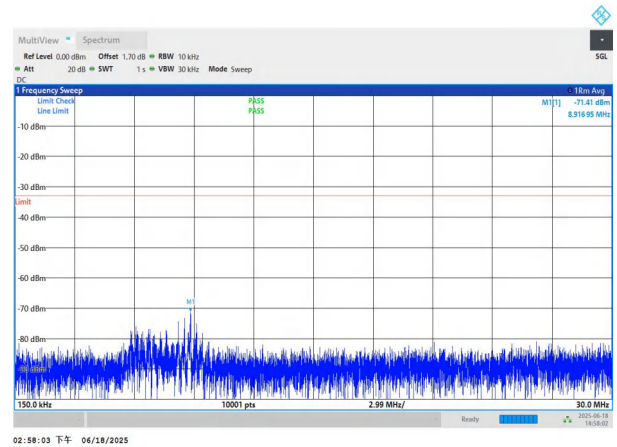
NTNV-n78(3700-3800)-PC3-30-40-L-DFT-BPSK-Edge_1RB_Left- 0.15-30-PASS
