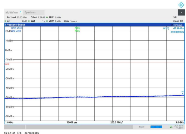
NTNV-n78(3700-3800)-PC3-30-40-M-DFT-BPSK-Edge_1RB_Left -1000-3000-PASS
