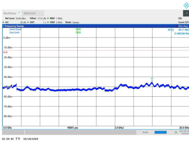
NTNV-n78(3700-3800)-PC3-30-40-L-DFT-QPSK-Edge_1RB_Left- 6000-26000-PASS
