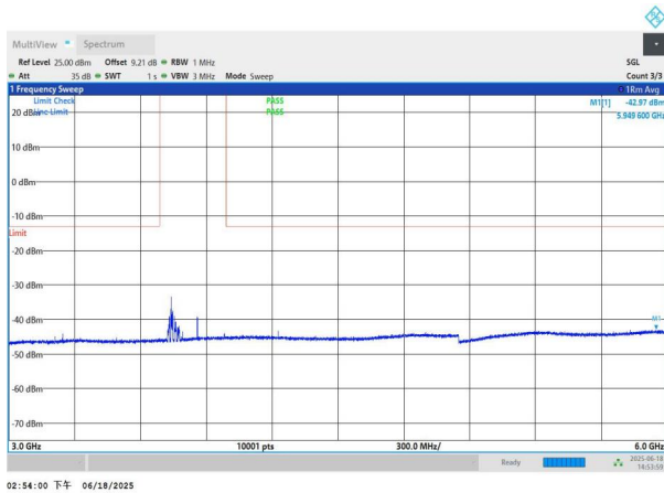
NTNV-n78(3700-3800)-PC3-30-30-M-DFT-BPSK-Edge_1RB_Left -3000-6000-PASS
