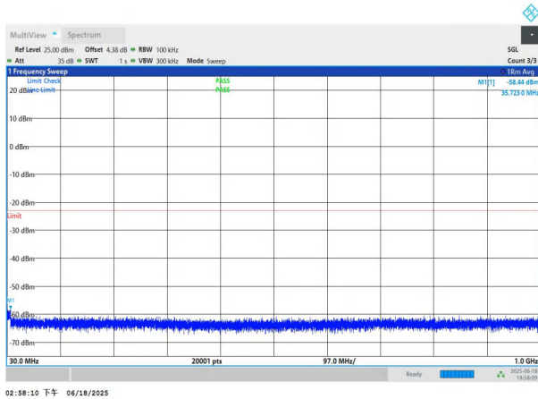
NTNV-n78(3700-3800)-PC3-30-40-L-DFT-BPSK-Edge_1RB_Left- 30-1000-PASS
