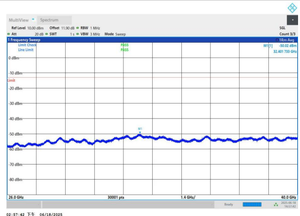
NTNV-n78(3700-3800)-PC3-30-30-H-DFT-QPSK-Edge_1RB_Left -26000-40000-PASS
