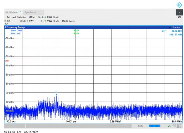
NTNV-n78(3700-3800)-PC3-30-40-H-DFT-BPSK-Edge_1RB_Left 0.15-30-PASS
