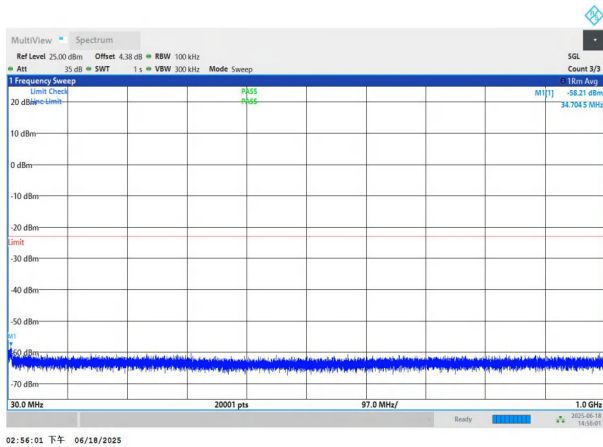
NTNV-n78(3700-3800)-PC3-30-30-H-DFT-BPSK-Edge_1RB_Left -30-1000-PASS
