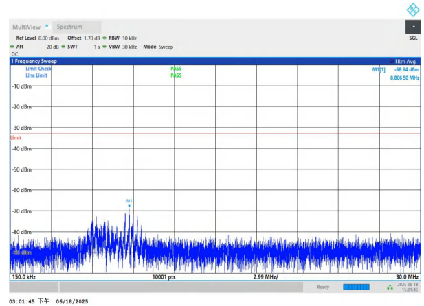
NTNV-n78(3700-3800)-PC3-30-40-M-DFT-BPSK-Edge_1RB_Left -0.15-30-PASS
