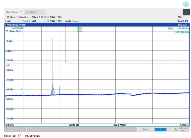
NTNV-n78(3700-3800)-PC3-30-30-H-DFT-QPSK-Edge_1RB_Left -3000-6000-PASS
