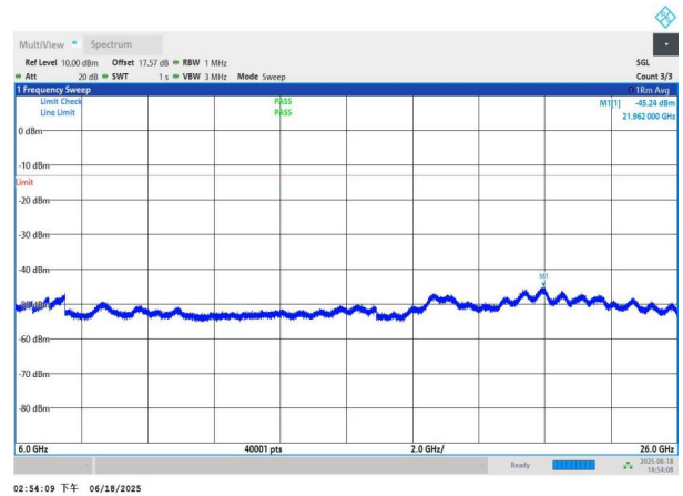
NTNV-n78(3700-3800)-PC3-30-30-M-DFT-BPSK-Edge_1RB_Left -6000-26000-PASS
