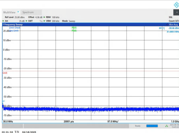
NTNV-n78(3700-3800)-PC3-30-40-M-DFT-BPSK-Edge_1RB_Left -30-1000-PASS
