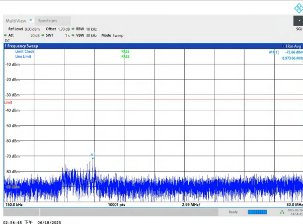
NTNV-n78(3700-3800)-PC3-30-30-M-DFT-QPSK-Edge_1RB_Left -0.15-30-PASS
