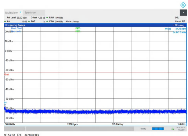
NTNV-n78(3700-3800)-PC3-30-30-M-DFT-QPSK-Edge_1RB_Left -30-1000-PASS
