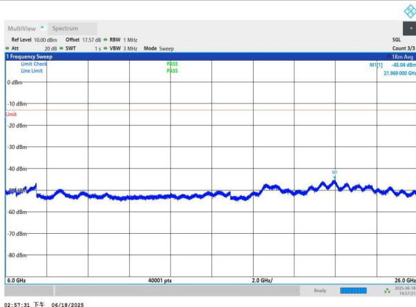
NTNV-n78(3700-3800)-PC3-30-30-H-DFT-QPSK-Edge_1RB_Left -6000-26000-PASS
