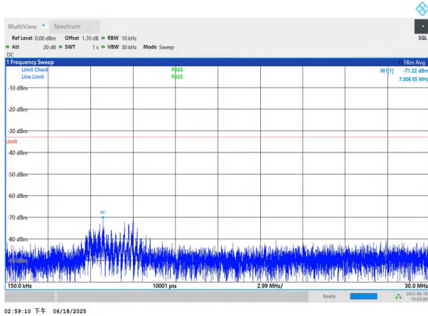
NTNV-n78(3700-3800)-PC3-30-40-L-DFT-QPSK-Edge_1RB_Left- 0.15-30-PASS
