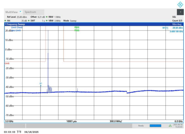
NTNV-n78(3700-3800)-PC3-30-40-M-DFT-QPSK-Edge_1RB_Left -3000-6000-PASS
