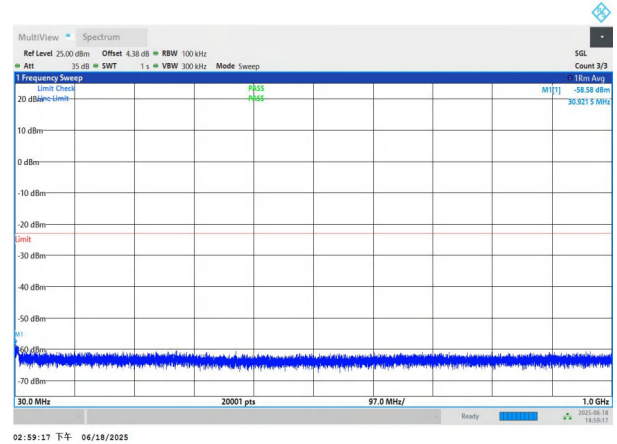
NTNV-n78(3700-3800)-PC3-30-40-L-DFT-QPSK-Edge_1RB_Left- 30-1000-PASS
