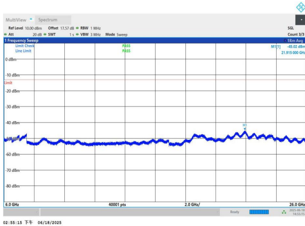
NTNV-n78(3700-3800)-PC3-30-30-M-DFT-QPSK-Edge_1RB_Left -6000-26000-PASS
