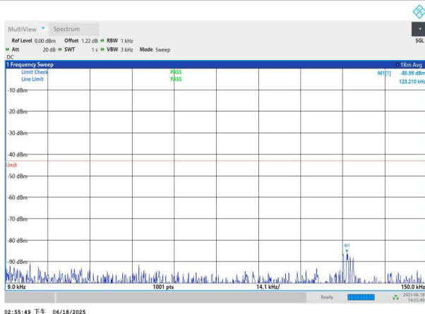
NTNV-n78(3700-3800)-PC3-30-30-H-DFT-BPSK-Edge_1RB_Left -0.009-0.15-PASS
