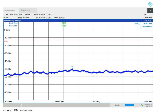
NTNV-n78(3700-3800)-PC3-30-40-L-DFT-QPSK-Edge_1RB_Left- 26000-40000-PASS
