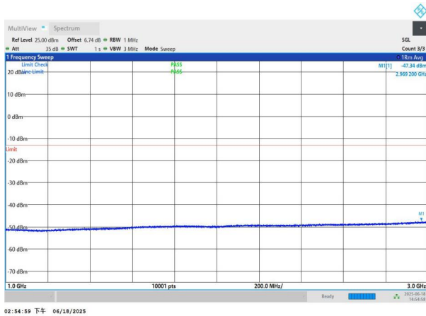
NTNV-n78(3700-3800)-PC3-30-30-M-DFT-QPSK-Edge_1RB_Left -1000-3000-PASS
