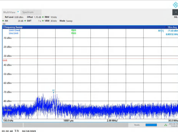
NTNV-n78(3700-3800)-PC3-30-40-M-DFT-QPSK-Edge_1RB_Left -0.15-30-PASS
