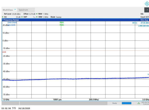
NTNV-n78(3700-3800)-PC3-30-40-M-DFT-QPSK-Edge_1RB_Left -1000-3000-PASS
