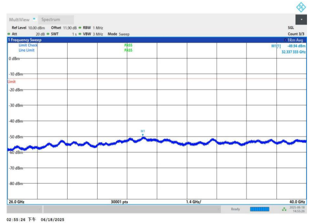
NTNV-n78(3700-3800)-PC3-30-30-M-DFT-QPSK-Edge_1RB_Left -26000-40000-PASS
