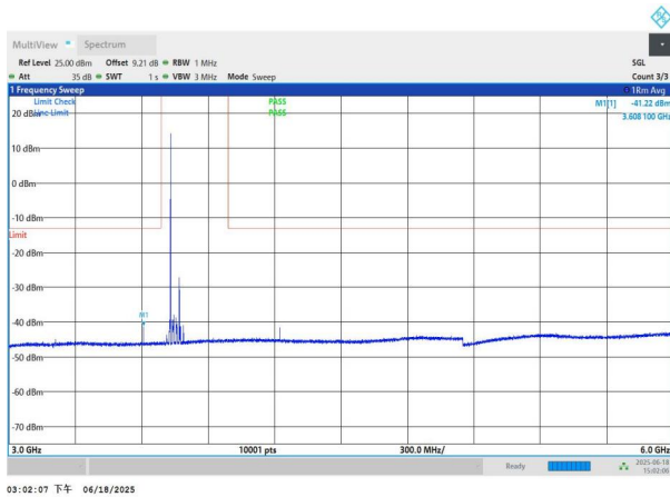
NTNV-n78(3700-3800)-PC3-30-40-M-DFT-BPSK-Edge_1RB_Left -3000-6000-PASS
