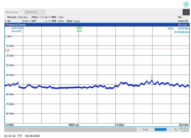
NTNV-n77(3700-3980)-PC3-30-90-H-DFT-BPSK-Edge_1RB_Left 6000-26000-PASS
