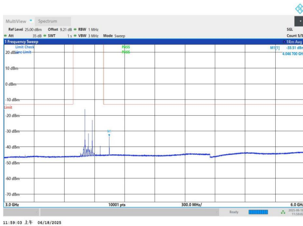
NTNV-n77(3700-3980)-PC3-30-80-M-DFT-BPSK-Edge_1RB_Left -3000-6000-PASS
