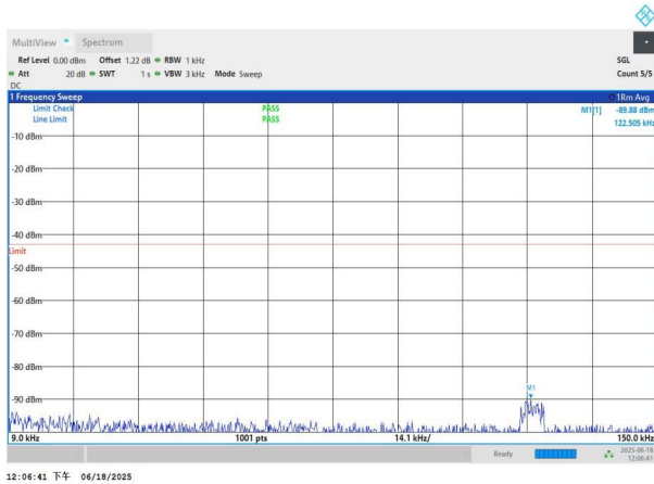
NTNV-n77(3700-3980)-PC3-30-90-M-DFT-BPSK-Edge_1RB_Left -0.009-0.15-PASS
