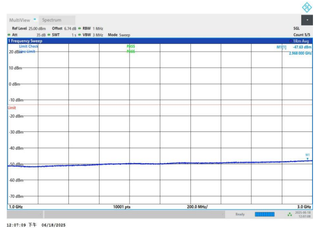
NTNV-n77(3700-3980)-PC3-30-90-M-DFT-BPSK-Edge_1RB_Left -1000-3000-PASS
