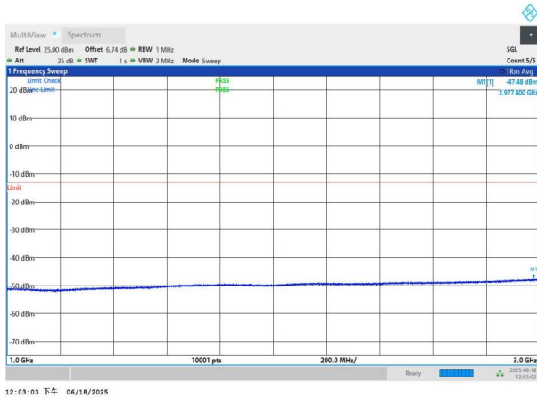
NTNV-n77(3700-3980)-PC3-30-80-H-DFT-QPSK-Edge_1RB_Left -1000-3000-PASS
