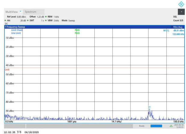
NTNV-n77(3700-3980)-PC3-30-80-H-DFT-QPSK-Edge_1RB_Left -0.009-0.15-PASS
