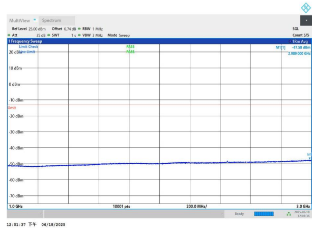
NTNV-n77(3700-3980)-PC3-30-80-H-DFT-BPSK-Edge_1RB_Left 1000-3000-PASS
