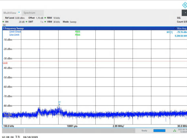
NTNV-n77(3700-3980)-PC3-30-90-M-DFT-QPSK-Edge_1RB_Left -0.15-30-PASS
