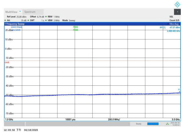
NTNV-n77(3700-3980)-PC3-30-90-H-DFT-BPSK-Edge_1RB_Left 1000-3000-PASS
