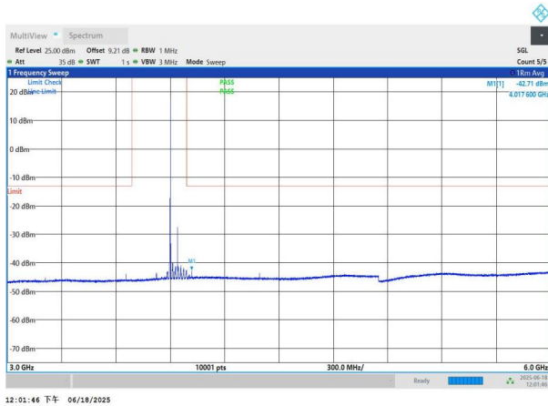
NTNV-n77(3700-3980)-PC3-30-80-H-DFT-BPSK-Edge_1RB_Left -3000-6000-PASS
