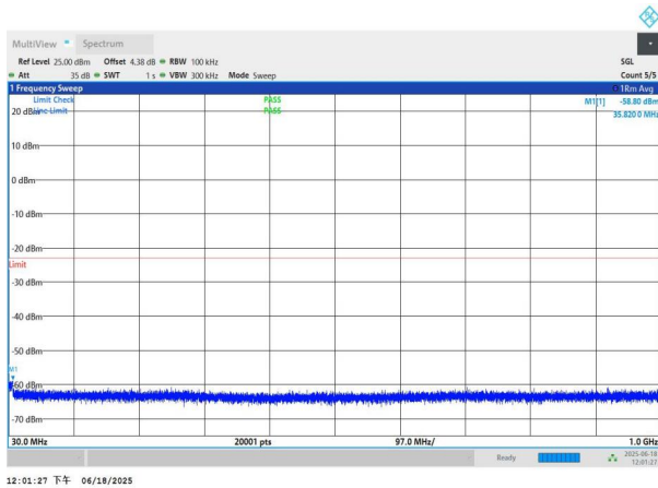
NTNV-n77(3700-3980)-PC3-30-80-H-DFT-BPSK-Edge_1RB_Left -30-1000-PASS
