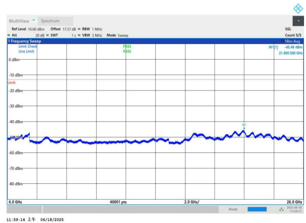
NTNV-n77(3700-3980)-PC3-30-80-M-DFT-BPSK-Edge_1RB_Left -6000-26000-PASS
