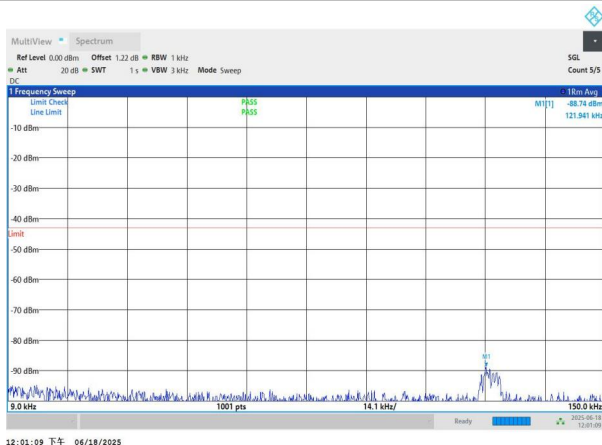
NTNV-n77(3700-3980)-PC3-30-80-H-DFT-BPSK-Edge_1RB_Left -0.009-0.15-PASS
