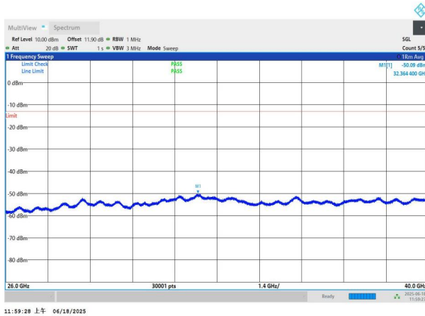
NTNV-n77(3700-3980)-PC3-30-80-M-DFT-BPSK-Edge_1RB_Left -26000-40000-PASS
