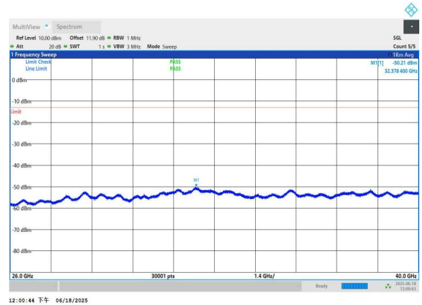
NTNV-n77(3700-3980)-PC3-30-80-M-DFT-QPSK-Edge_1RB_Left -26000-40000-PASS
