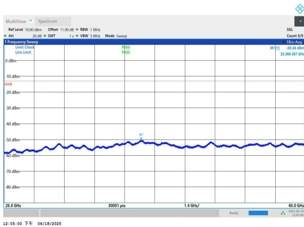
NTNV-n77(3700-3980)-PC3-30-90-L-DFT-BPSK-Edge_1RB_Left- 26000-40000-PASS
