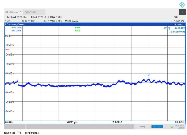
NTNV-n77(3700-3980)-PC3-30-90-M-DFT-BPSK-Edge_1RB_Left -6000-26000-PASS
