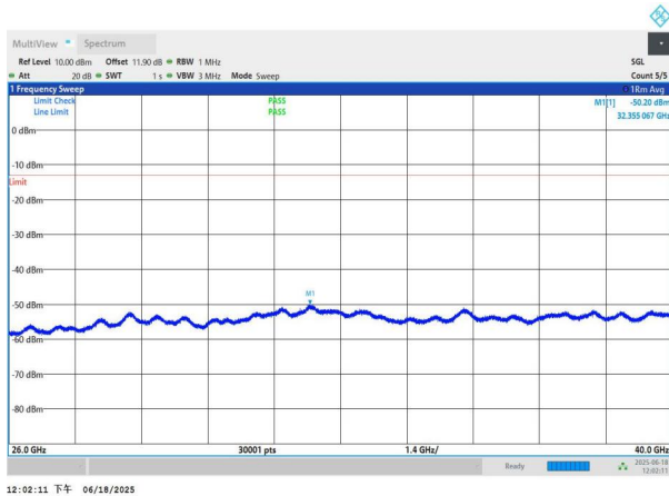
NTNV-n77(3700-3980)-PC3-30-80-H-DFT-BPSK-Edge_1RB_Left -26000-40000-PASS
