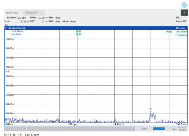
NTNV-n77(3700-3980)-PC3-30-90-H-DFT-QPSK-Edge_1RB_Left -0.009-0.15-PASS
