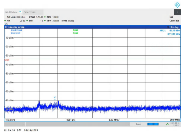
NTNV-n77(3700-3980)-PC3-30-90-H-DFT-BPSK-Edge_1RB_Left 0.15-30-PASS
