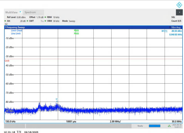
NTNV-n77(3700-3980)-PC3-30-80-H-DFT-BPSK-Edge_1RB_Left 0.15-30-PASS
