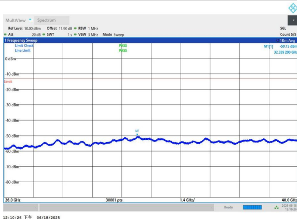
NTNV-n77(3700-3980)-PC3-30-90-H-DFT-BPSK-Edge_1RB_Left -26000-40000-PASS
