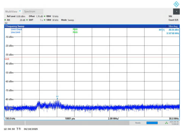
NTNV-n77(3700-3980)-PC3-30-90-M-DFT-BPSK-Edge_1RB_Left -0.15-30-PASS
