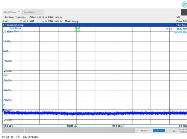
NTNV-n77(3700-3980)-PC3-30-90-M-DFT-BPSK-Edge_1RB_Left -30-1000-PASS
