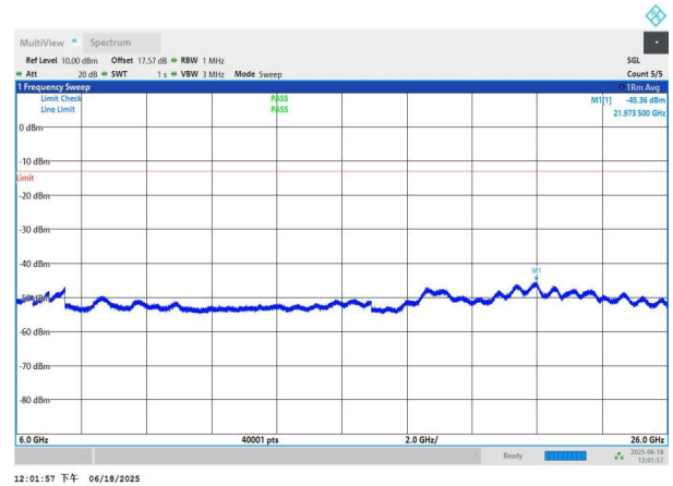
NTNV-n77(3700-3980)-PC3-30-80-H-DFT-BPSK-Edge_1RB_Left 6000-26000-PASS
