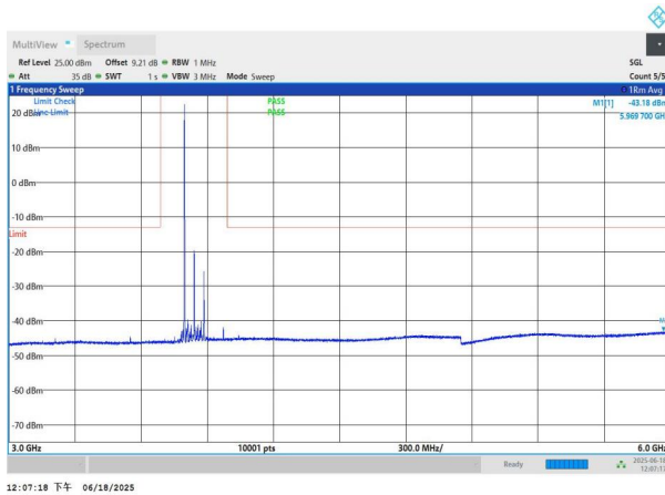
NTNV-n77(3700-3980)-PC3-30-90-M-DFT-BPSK-Edge_1RB_Left -3000-6000-PASS
