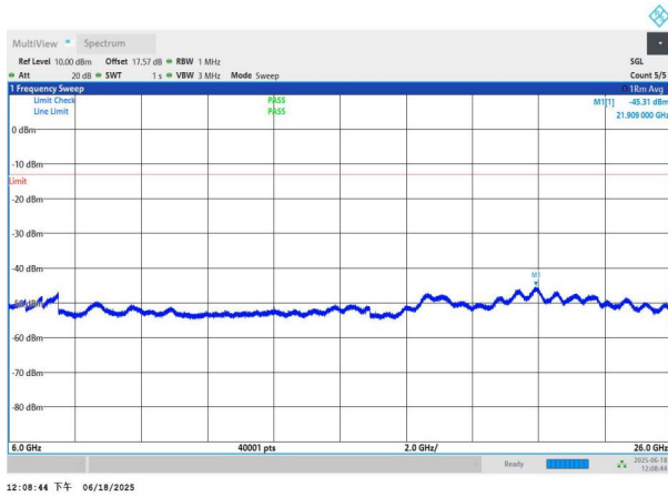
NTNV-n77(3700-3980)-PC3-30-90-M-DFT-QPSK-Edge_1RB_Left -6000-26000-PASS
