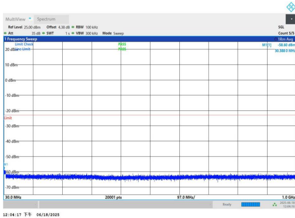
NTNV-n77(3700-3980)-PC3-30-90-L-DFT-BPSK-Edge_1RB_Left- 30-1000-PASS
