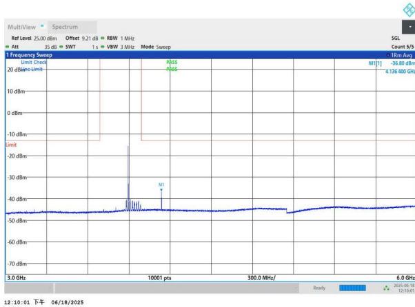
NTNV-n77(3700-3980)-PC3-30-90-H-DFT-BPSK-Edge_1RB_Left -3000-6000-PASS
