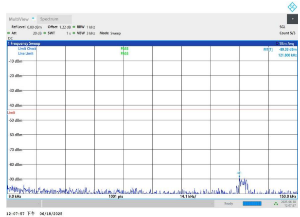
NTNV-n77(3700-3980)-PC3-30-90-M-DFT-QPSK-Edge_1RB_Left -0.009-0.15-PASS
