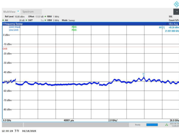
NTNV-n77(3700-3980)-PC3-30-80-M-DFT-QPSK-Edge_1RB_Left -6000-26000-PASS
