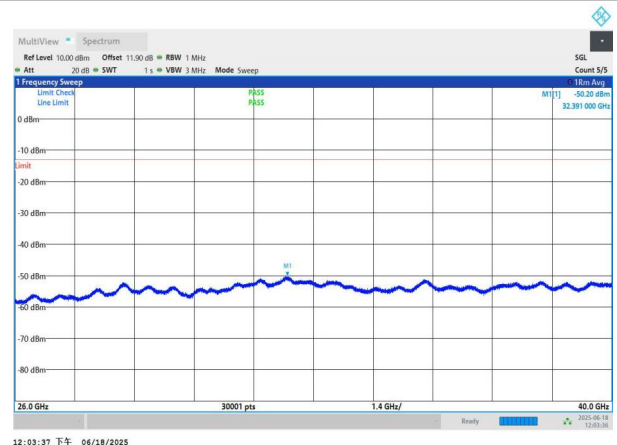
NTNV-n77(3700-3980)-PC3-30-80-H-DFT-QPSK-Edge_1RB_Left -26000-40000-PASS
