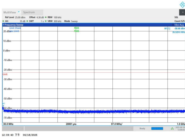
NTNV-n77(3700-3980)-PC3-30-90-H-DFT-BPSK-Edge_1RB_Left -30-1000-PASS
