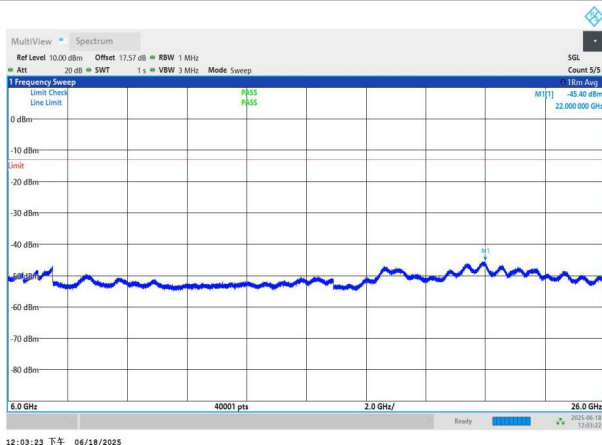
NTNV-n77(3700-3980)-PC3-30-80-H-DFT-QPSK-Edge_1RB_Left -6000-26000-PASS
