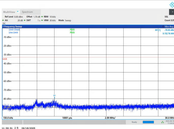
NTNV-n77(3700-3980)-PC3-30-80-M-DFT-QPSK-Edge_1RB_Left -0.15-30-PASS
