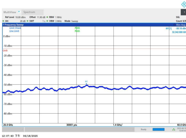
NTNV-n77(3700-3980)-PC3-30-90-M-DFT-BPSK-Edge_1RB_Left -26000-40000-PASS
