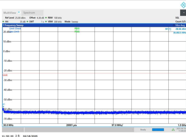
NTNV-n77(3700-3980)-PC3-30-70-M-DFT-BPSK-Edge_1RB_Left -30-1000-PASS
