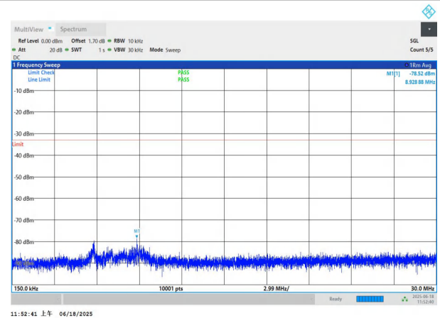
NTNV-n77(3700-3980)-PC3-30-70-H-DFT-BPSK-Edge_1RB_Left 0.15-30-PASS
