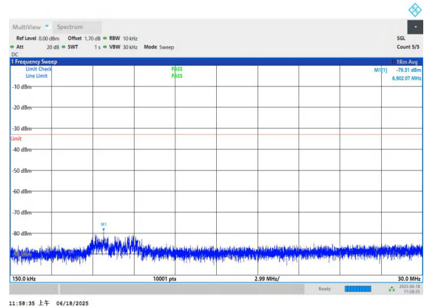
NTNV-n77(3700-3980)-PC3-30-80-M-DFT-BPSK-Edge_1RB_Left -0.15-30-PASS
