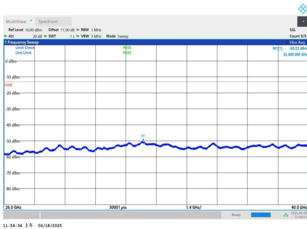
NTNV-n77(3700-3980)-PC3-30-80-L-DFT-BPSK-Edge_1RB_Left- 26000-40000-PASS
