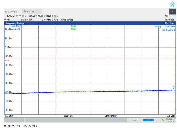
NTNV-n77(3700-3980)-PC3-30-70-H-DFT-BPSK-Edge_1RB_Left 1000-3000-PASS
