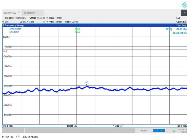
NTNV-n77(3700-3980)-PC3-30-70-H-DFT-BPSK-Edge_1RB_Left -26000-40000-PASS
