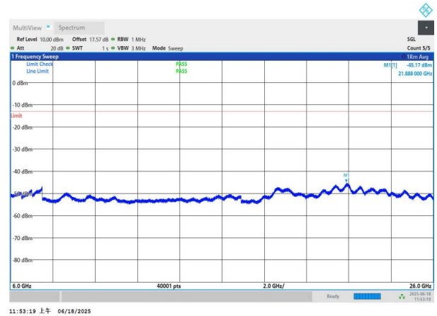
NTNV-n77(3700-3980)-PC3-30-70-H-DFT-BPSK-Edge_1RB_Left 6000-26000-PASS
