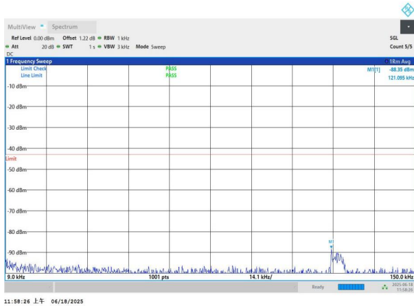
NTNV-n77(3700-3980)-PC3-30-80-M-DFT-BPSK-Edge_1RB_Left -0.009-0.15-PASS
