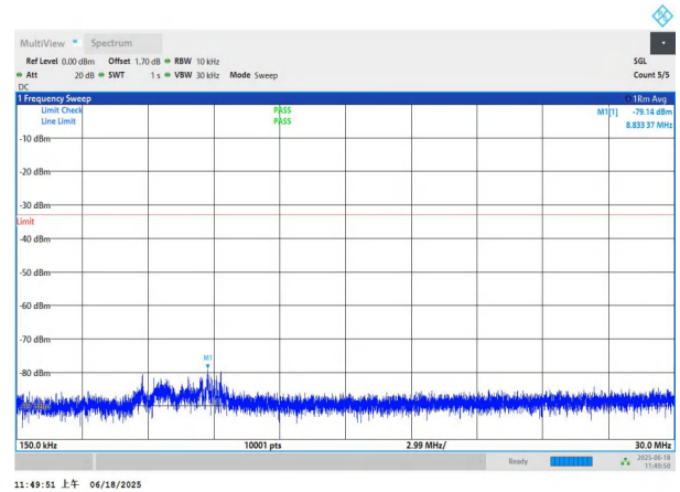
NTNV-n77(3700-3980)-PC3-30-70-M-DFT-BPSK-Edge_1RB_Left -0.15-30-PASS
