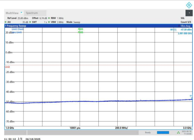
NTNV-n77(3700-3980)-PC3-30-70-M-DFT-BPSK-Edge_1RB_Left -1000-3000-PASS
