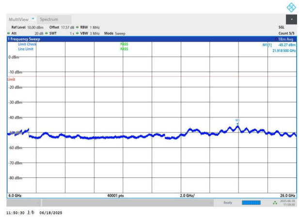
NTNV-n77(3700-3980)-PC3-30-70-M-DFT-BPSK-Edge_1RB_Left -6000-26000-PASS
