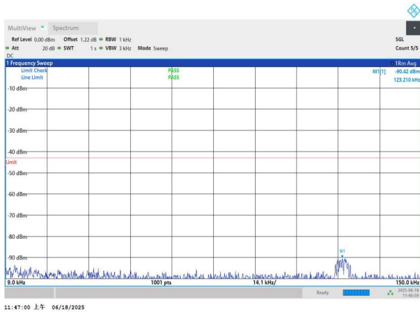
NTNV-n77(3700-3980)-PC3-30-70-L-DFT-BPSK-Edge_1RB_Left- 0.009-0.15-PASS
