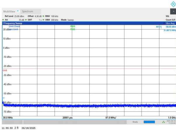
NTNV-n77(3700-3980)-PC3-30-80-L-DFT-BPSK-Edge_1RB_Left- 30-1000-PASS
