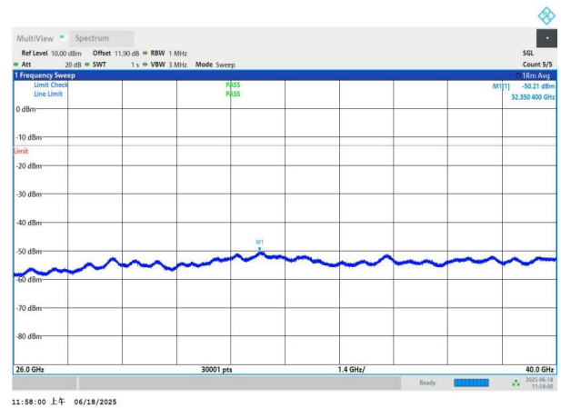
NTNV-n77(3700-3980)-PC3-30-80-L-DFT-QPSK-Edge_1RB_Left- 26000-40000-PASS
