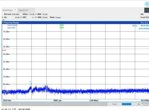
NTNV-n77(3700-3980)-PC3-30-70-M-DFT-QPSK-Edge_1RB_Left -0.15-30-PASS
