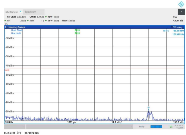
NTNV-n77(3700-3980)-PC3-30-70-M-DFT-QPSK-Edge_1RB_Left -0.009-0.15-PASS
