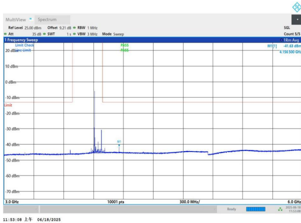
NTNV-n77(3700-3980)-PC3-30-70-H-DFT-BPSK-Edge_1RB_Left -3000-6000-PASS
