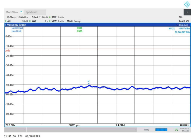
NTNV-n77(3700-3980)-PC3-30-70-H-DFT-QPSK-Edge_1RB_Left -26000-40000-PASS
