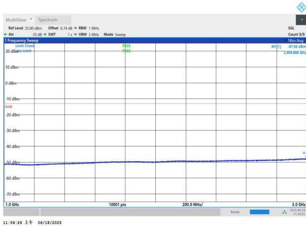
NTNV-n77(3700-3980)-PC3-30-70-H-DFT-QPSK-Edge_1RB_Left -1000-3000-PASS
