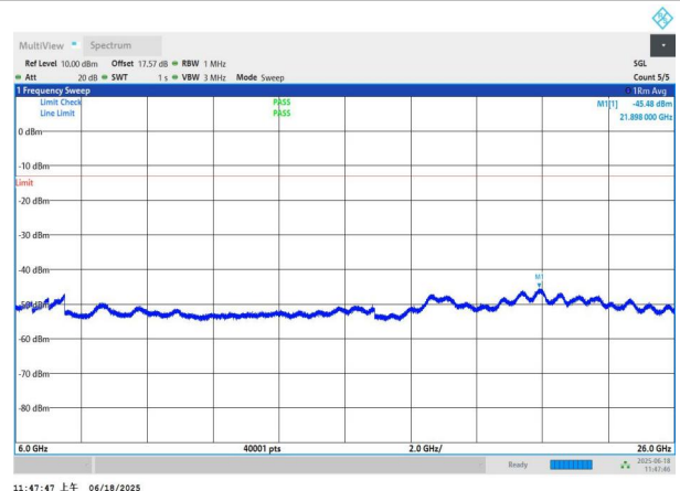
NTNV-n77(3700-3980)-PC3-30-70-L-DFT-BPSK-Edge_1RB_Left- 6000-26000-PASS
