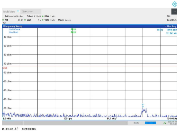
NTNV-n77(3700-3980)-PC3-30-70-M-DFT-BPSK-Edge_1RB_Left -0.009-0.15-PASS
