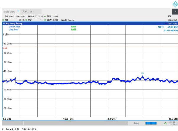
NTNV-n77(3700-3980)-PC3-30-70-H-DFT-QPSK-Edge_1RB_Left -6000-26000-PASS
