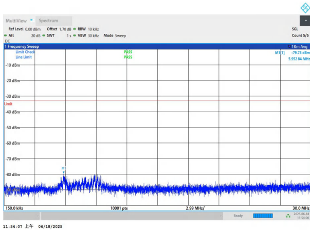
NTNV-n77(3700-3980)-PC3-30-70-H-DFT-QPSK-Edge_1RB_Left -0.15-30-PASS
