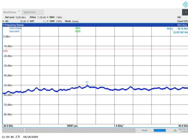
NTNV-n77(3700-3980)-PC3-30-70-M-DFT-BPSK-Edge_1RB_Left -26000-40000-PASS
