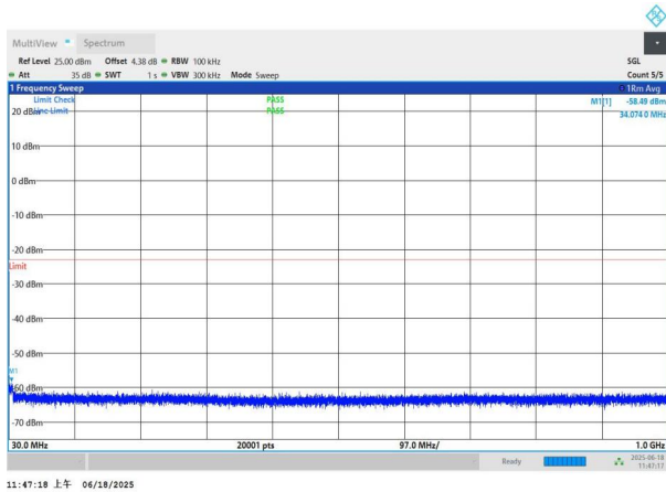
NTNV-n77(3700-3980)-PC3-30-70-L-DFT-BPSK-Edge_1RB_Left- 30-1000-PASS
