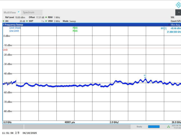
NTNV-n77(3700-3980)-PC3-30-70-M-DFT-QPSK-Edge_1RB_Left -6000-26000-PASS
