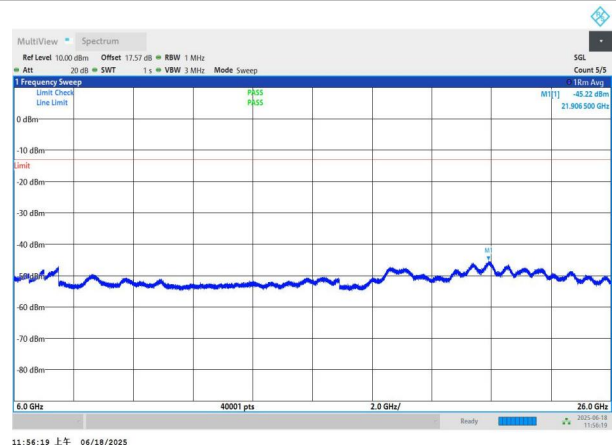
NTNV-n77(3700-3980)-PC3-30-80-L-DFT-BPSK-Edge_1RB_Left- 6000-26000-PASS
