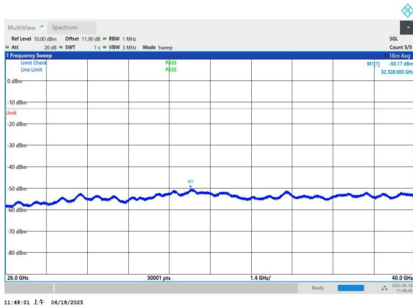
NTNV-n77(3700-3980)-PC3-30-70-L-DFT-BPSK-Edge_1RB_Left- 26000-40000-PASS
