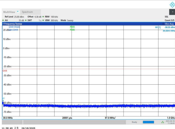
NTNV-n77(3700-3980)-PC3-30-80-M-DFT-BPSK-Edge_1RB_Left -30-1000-PASS
