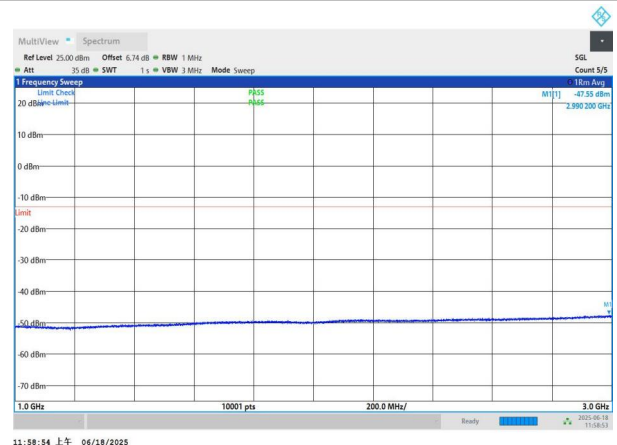
NTNV-n77(3700-3980)-PC3-30-80-M-DFT-BPSK-Edge_1RB_Left -1000-3000-PASS
