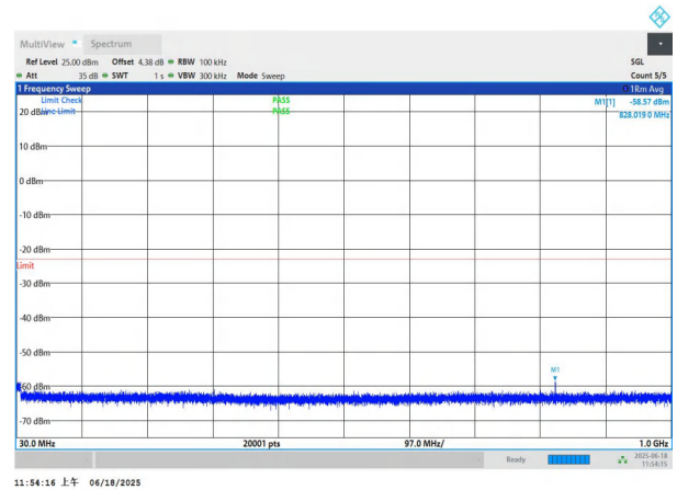
NTNV-n77(3700-3980)-PC3-30-70-H-DFT-QPSK-Edge_1RB_Left -30-1000-PASS
