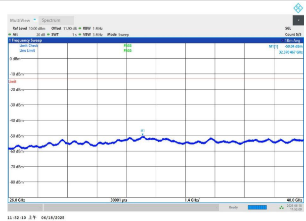
NTNV-n77(3700-3980)-PC3-30-70-M-DFT-QPSK-Edge_1RB_Left -26000-40000-PASS
