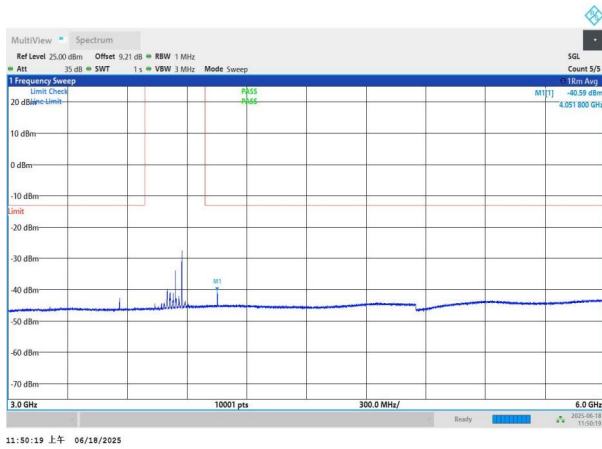
NTNV-n77(3700-3980)-PC3-30-70-M-DFT-BPSK-Edge_1RB_Left -3000-6000-PASS
