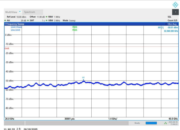
NTNV-n77(3700-3980)-PC3-30-60-H-DFT-QPSK-Edge_1RB_Left -26000-40000-PASS
