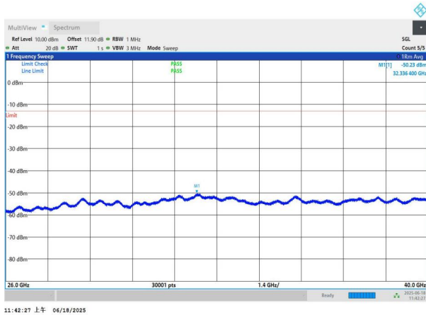
NTNV-n77(3700-3980)-PC3-30-60-M-DFT-BPSK-Edge_1RB_Left -26000-40000-PASS
