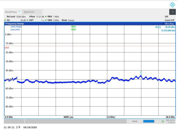
NTNV-n77(3700-3980)-PC3-30-60-L-DFT-BPSK-Edge_1RB_Left- 6000-26000-PASS
