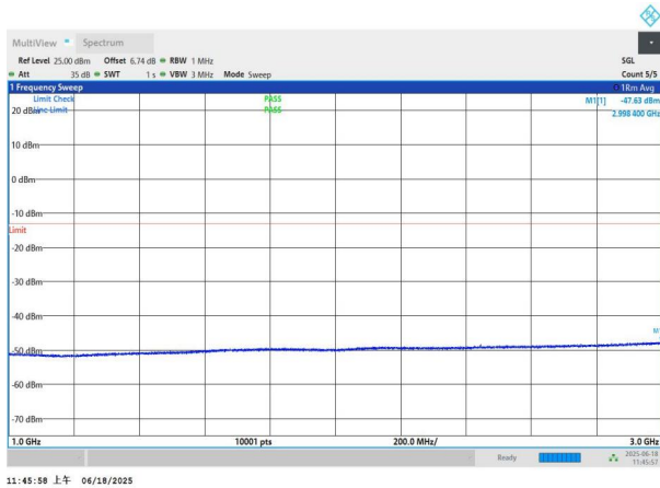
NTNV-n77(3700-3980)-PC3-30-60-H-DFT-QPSK-Edge_1RB_Left -1000-3000-PASS
