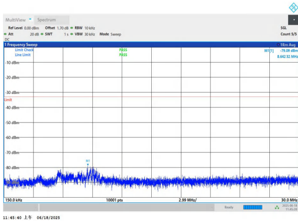
NTNV-n77(3700-3980)-PC3-30-60-H-DFT-QPSK-Edge_1RB_Left -0.15-30-PASS
