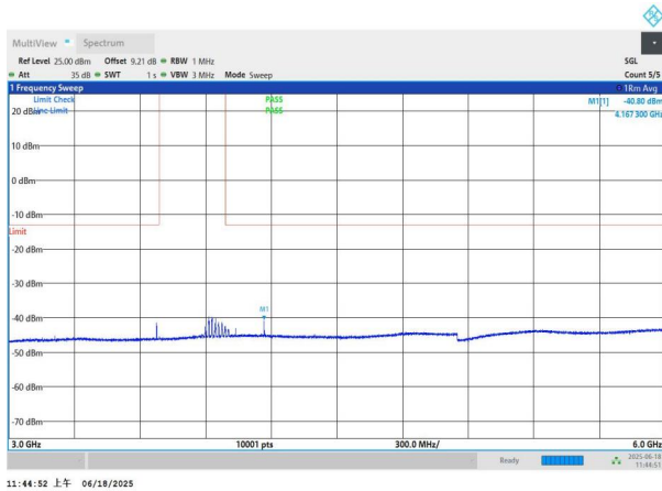
NTNV-n77(3700-3980)-PC3-30-60-H-DFT-BPSK-Edge_1RB_Left -3000-6000-PASS
