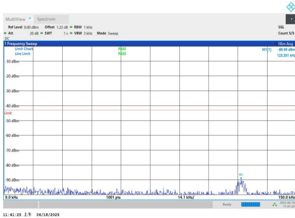
NTNV-n77(3700-3980)-PC3-30-60-M-DFT-BPSK-Edge_1RB_Left -0.009-0.15-PASS
