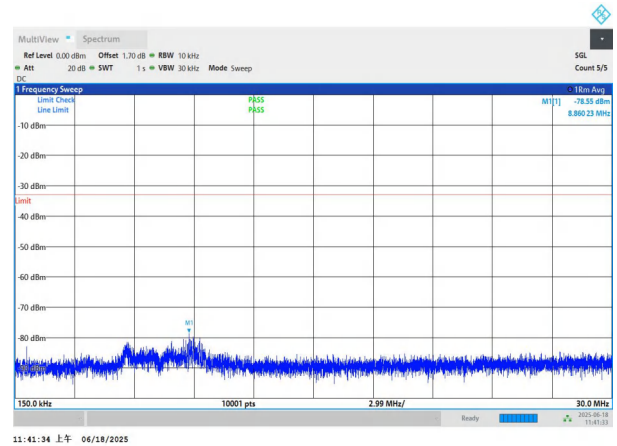
NTNV-n77(3700-3980)-PC3-30-60-M-DFT-BPSK-Edge_1RB_Left -0.15-30-PASS
