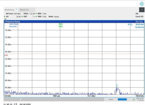
NTNV-n77(3700-3980)-PC3-30-60-H-DFT-QPSK-Edge_1RB_Left -0.009-0.15-PASS
