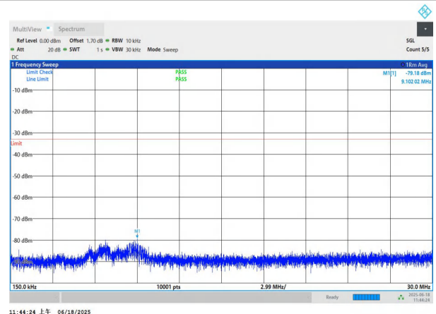
NTNV-n77(3700-3980)-PC3-30-60-H-DFT-BPSK-Edge_1RB_Left 0.15-30-PASS
