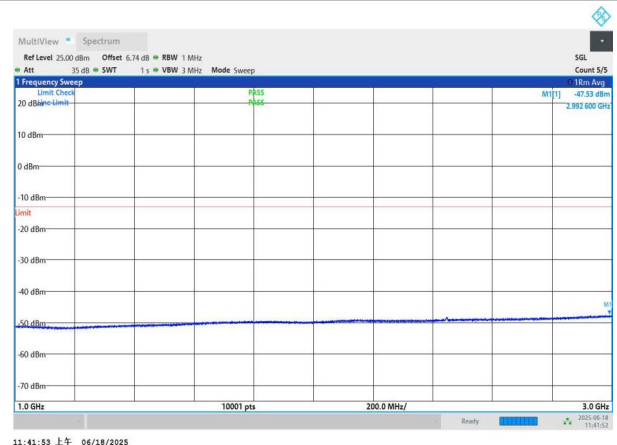
NTNV-n77(3700-3980)-PC3-30-60-M-DFT-BPSK-Edge_1RB_Left -1000-3000-PASS
