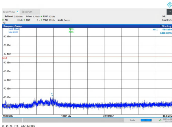
NTNV-n77(3700-3980)-PC3-30-60-M-DFT-QPSK-Edge_1RB_Left -0.15-30-PASS
