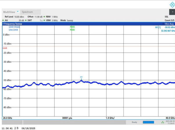
NTNV-n77(3700-3980)-PC3-30-50-H-DFT-BPSK-Edge_1RB_Left -26000-40000-PASS
