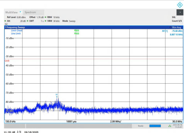
NTNV-n77(3700-3980)-PC3-30-50-H-DFT-BPSK-Edge_1RB_Left 0.15-30-PASS
