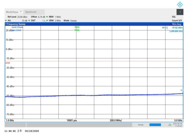
NTNV-n77(3700-3980)-PC3-30-60-H-DFT-BPSK-Edge_1RB_Left 1000-3000-PASS
