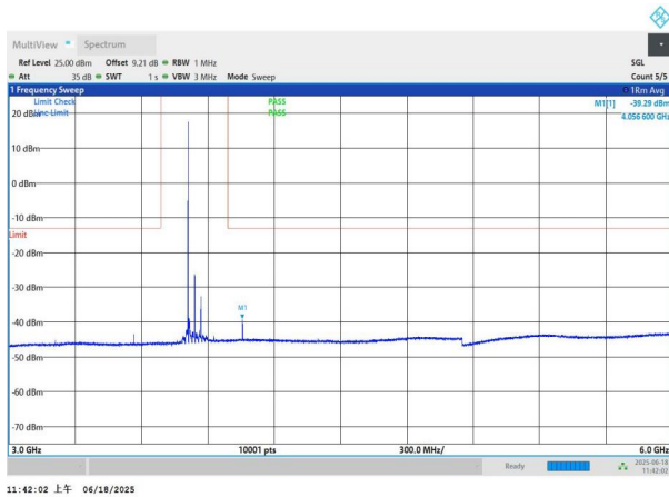
NTNV-n77(3700-3980)-PC3-30-60-M-DFT-BPSK-Edge_1RB_Left -3000-6000-PASS
