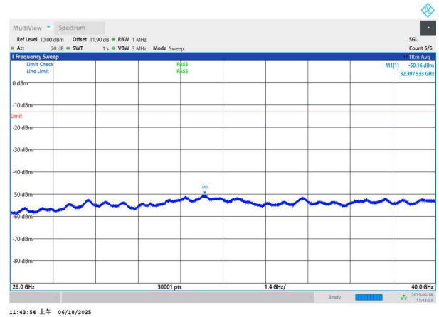
NTNV-n77(3700-3980)-PC3-30-60-M-DFT-QPSK-Edge_1RB_Left -26000-40000-PASS
