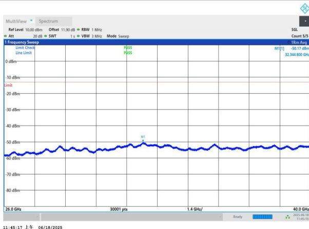
NTNV-n77(3700-3980)-PC3-30-60-H-DFT-BPSK-Edge_1RB_Left -26000-40000-PASS
