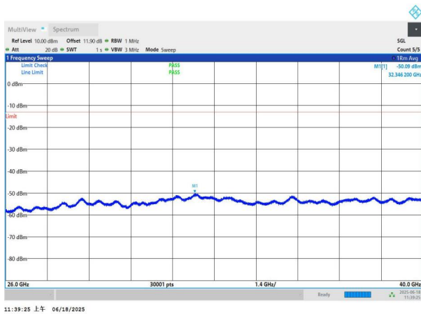
NTNV-n77(3700-3980)-PC3-30-60-L-DFT-BPSK-Edge_1RB_Left- 26000-40000-PASS
