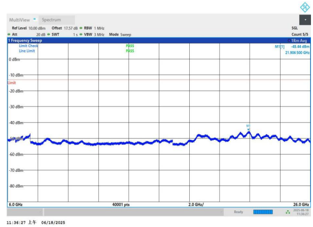
NTNV-n77(3700-3980)-PC3-30-50-H-DFT-BPSK-Edge_1RB_Left 6000-26000-PASS
