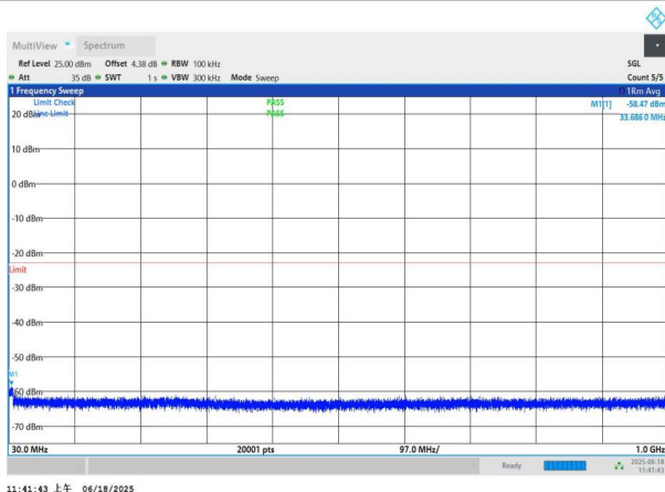
NTNV-n77(3700-3980)-PC3-30-60-M-DFT-BPSK-Edge_1RB_Left -30-1000-PASS
