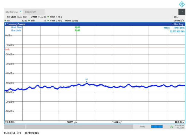
NTNV-n77(3700-3980)-PC3-30-50-M-DFT-QPSK-Edge_1RB_Left -26000-40000-PASS
