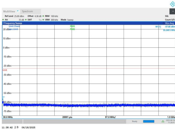
NTNV-n77(3700-3980)-PC3-30-60-L-DFT-BPSK-Edge_1RB_Left- 30-1000-PASS
