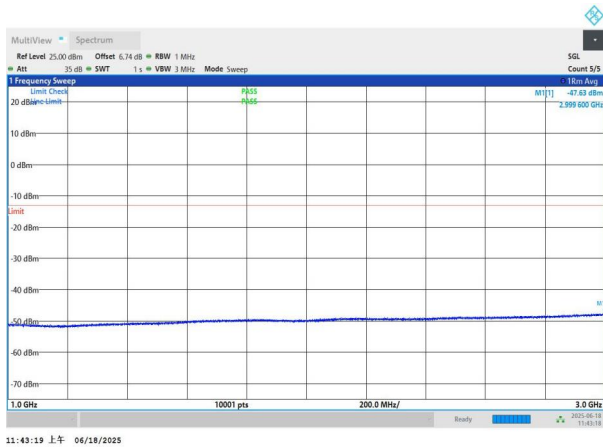
NTNV-n77(3700-3980)-PC3-30-60-M-DFT-QPSK-Edge_1RB_Left -1000-3000-PASS
