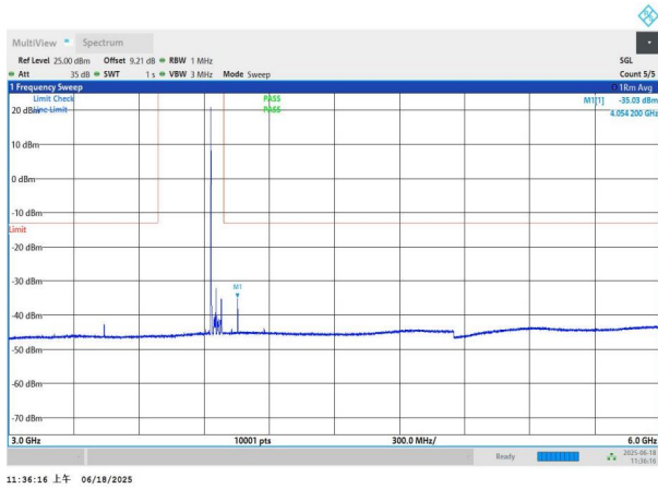
NTNV-n77(3700-3980)-PC3-30-50-H-DFT-BPSK-Edge_1RB_Left -3000-6000-PASS
