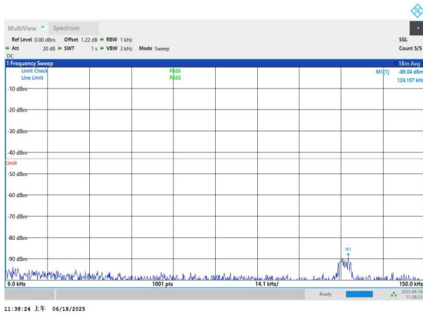
NTNV-n77(3700-3980)-PC3-30-60-L-DFT-BPSK-Edge_1RB_Left- 0.009-0.15-PASS
