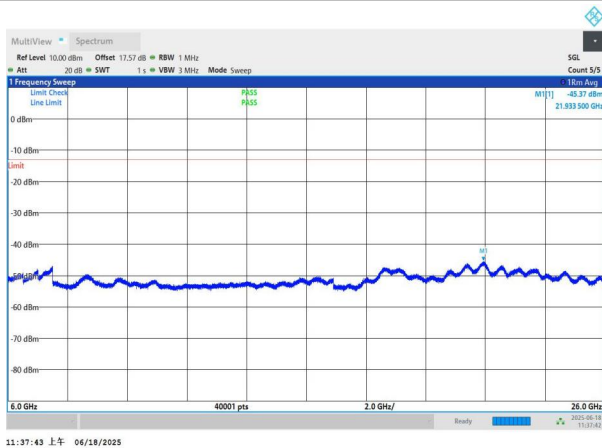
NTNV-n77(3700-3980)-PC3-30-50-H-DFT-QPSK-Edge_1RB_Left -6000-26000-PASS
