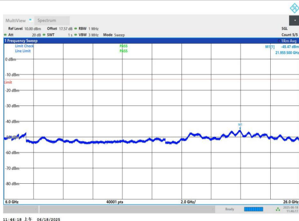
NTNV-n77(3700-3980)-PC3-30-60-H-DFT-QPSK-Edge_1RB_Left -6000-26000-PASS
