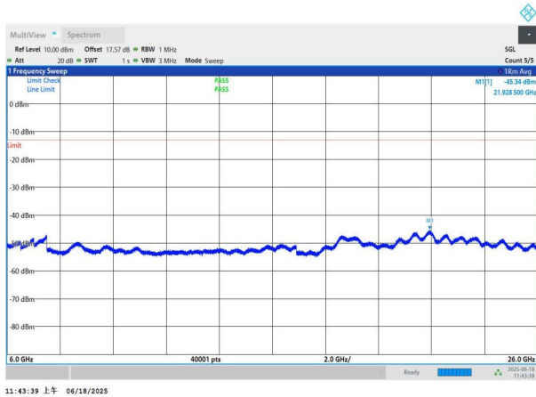
NTNV-n77(3700-3980)-PC3-30-60-M-DFT-QPSK-Edge_1RB_Left -6000-26000-PASS
