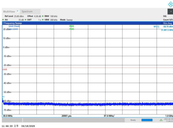
NTNV-n77(3700-3980)-PC3-30-60-H-DFT-BPSK-Edge_1RB_Left -30-1000-PASS
