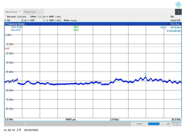
NTNV-n77(3700-3980)-PC3-30-60-M-DFT-BPSK-Edge_1RB_Left -6000-26000-PASS
