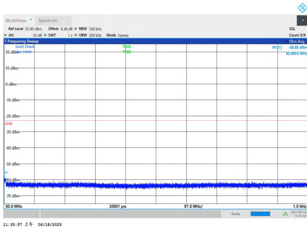
NTNV-n77(3700-3980)-PC3-30-50-H-DFT-BPSK-Edge_1RB_Left -30-1000-PASS
