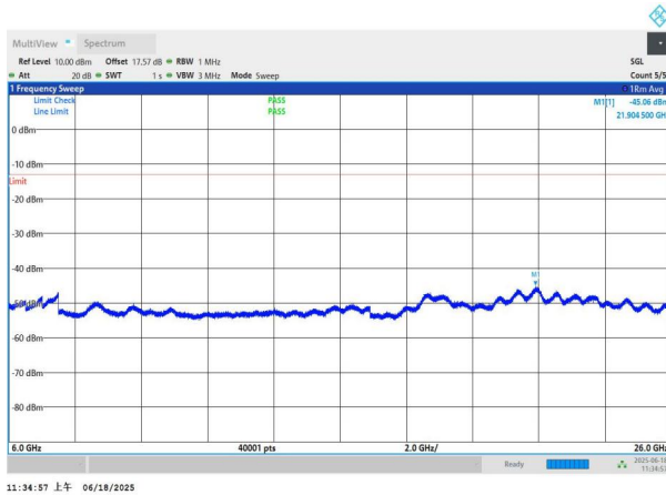
NTNV-n77(3700-3980)-PC3-30-50-M-DFT-QPSK-Edge_1RB_Left -6000-26000-PASS
