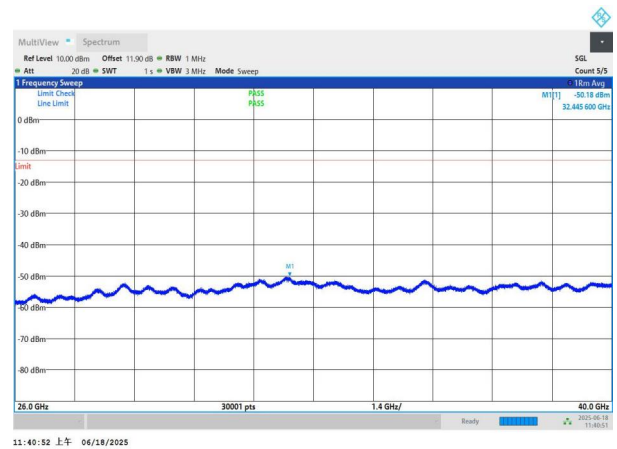
NTNV-n77(3700-3980)-PC3-30-60-L-DFT-QPSK-Edge_1RB_Left- 26000-40000-PASS
