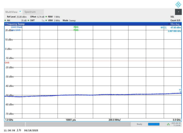
NTNV-n77(3700-3980)-PC3-30-50-H-DFT-BPSK-Edge_1RB_Left 1000-3000-PASS
