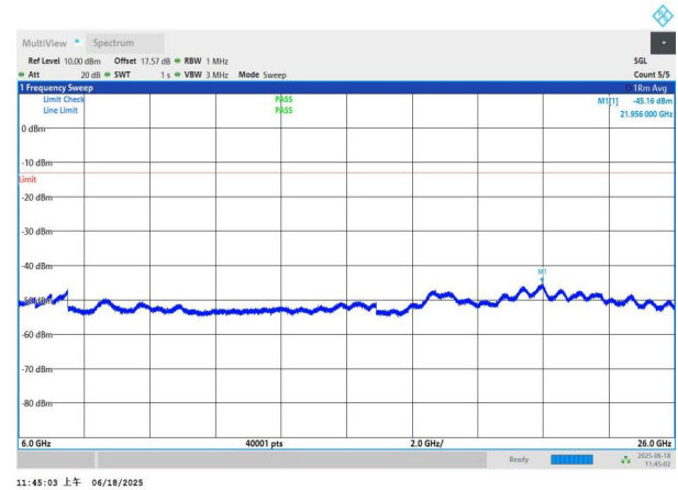
NTNV-n77(3700-3980)-PC3-30-60-H-DFT-BPSK-Edge_1RB_Left 6000-26000-PASS
