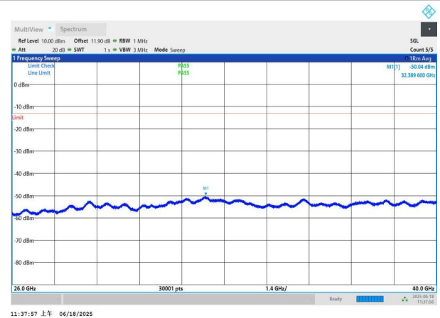
NTNV-n77(3700-3980)-PC3-30-50-H-DFT-QPSK-Edge_1RB_Left -26000-40000-PASS
