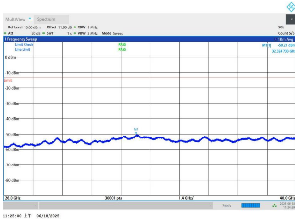
NTNV-n77(3700-3980)-PC3-30-40-M-DFT-BPSK-Edge_1RB_Left -26000-40000-PASS
