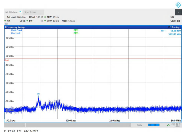
NTNV-n77(3700-3980)-PC3-30-40-H-DFT-BPSK-Edge_1RB_Left 0.15-30-PASS
