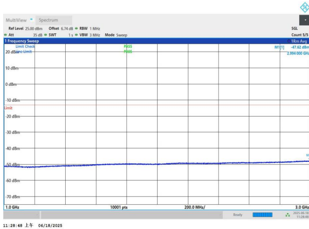
NTNV-n77(3700-3980)-PC3-30-40-H-DFT-QPSK-Edge_1RB_Left -1000-3000-PASS
