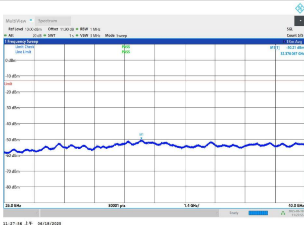
NTNV-n77(3700-3980)-PC3-30-40-H-DFT-BPSK-Edge_1RB_Left -26000-40000-PASS
