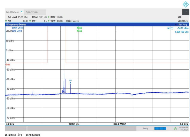
NTNV-n77(3700-3980)-PC3-30-40-H-DFT-QPSK-Edge_1RB_Left -3000-6000-PASS
