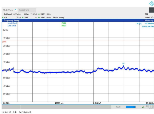
NTNV-n77(3700-3980)-PC3-30-40-M-DFT-QPSK-Edge_1RB_Left -6000-26000-PASS
