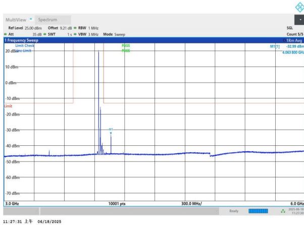
NTNV-n77(3700-3980)-PC3-30-40-H-DFT-BPSK-Edge_1RB_Left -3000-6000-PASS
