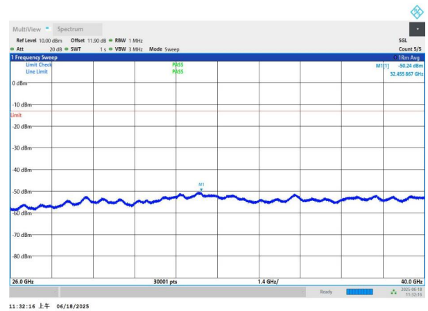
NTNV-n77(3700-3980)-PC3-30-50-L-DFT-QPSK-Edge_1RB_Left- 26000-40000-PASS
