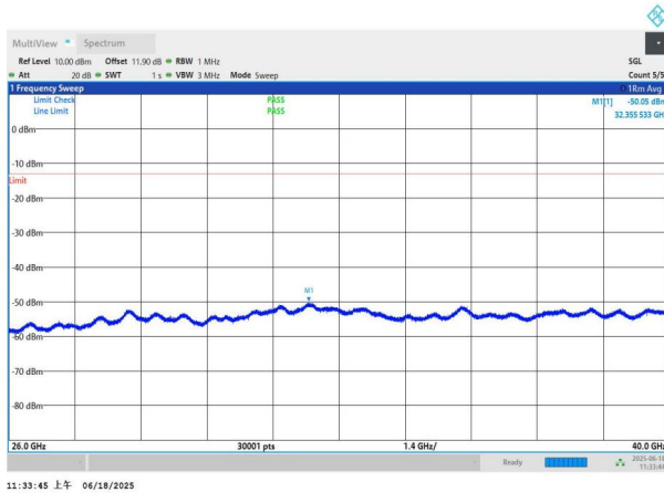
NTNV-n77(3700-3980)-PC3-30-50-M-DFT-BPSK-Edge_1RB_Left -26000-40000-PASS
