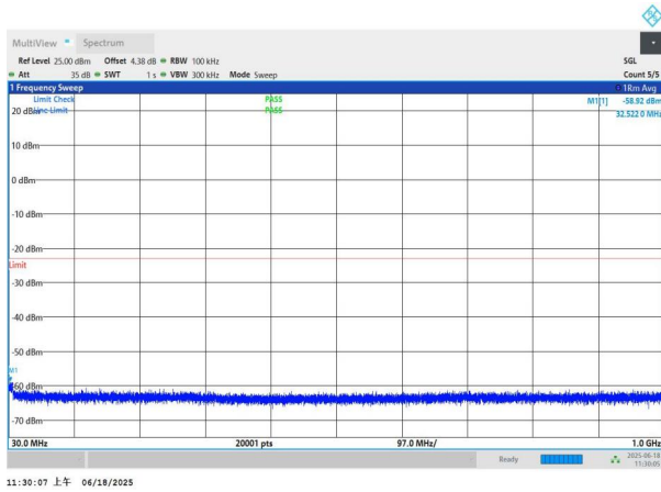
NTNV-n77(3700-3980)-PC3-30-50-L-DFT-BPSK-Edge_1RB_Left- 30-1000-PASS
