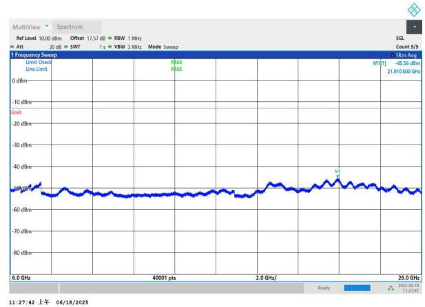
NTNV-n77(3700-3980)-PC3-30-40-H-DFT-BPSK-Edge_1RB_Left 6000-26000-PASS
