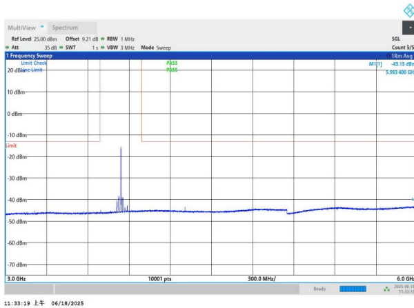
NTNV-n77(3700-3980)-PC3-30-50-M-DFT-BPSK-Edge_1RB_Left -3000-6000-PASS
