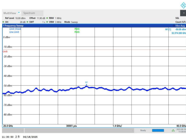
NTNV-n77(3700-3980)-PC3-30-50-L-DFT-BPSK-Edge_1RB_Left- 26000-40000-PASS
