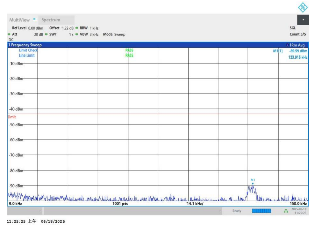
NTNV-n77(3700-3980)-PC3-30-40-M-DFT-QPSK-Edge_1RB_Left -0.009-0.15-PASS
