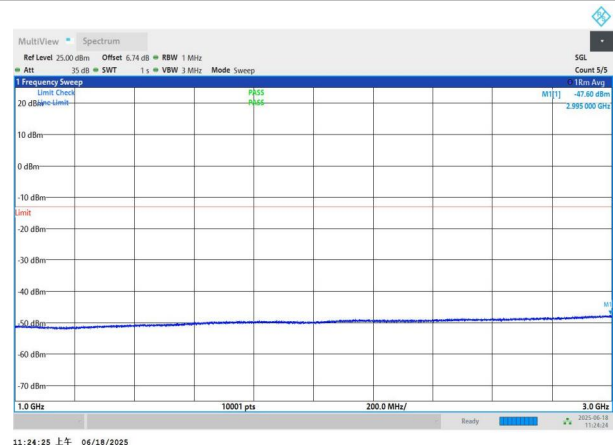
NTNV-n77(3700-3980)-PC3-30-40-M-DFT-BPSK-Edge_1RB_Left -1000-3000-PASS
