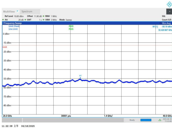
NTNV-n77(3700-3980)-PC3-30-40-L-DFT-BPSK-Edge_1RB_Left- 26000-40000-PASS
