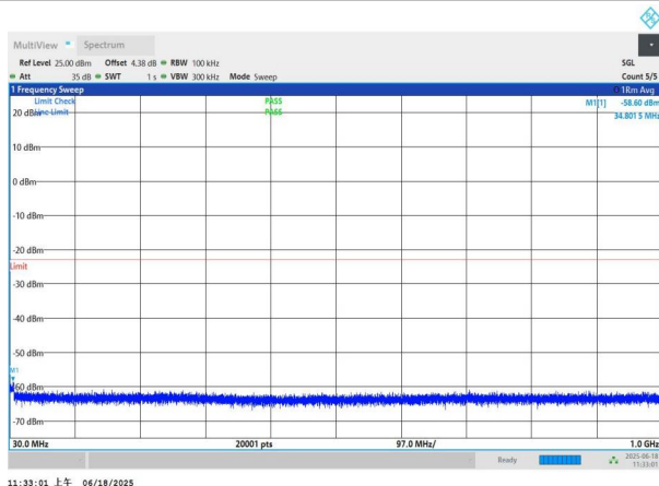
NTNV-n77(3700-3980)-PC3-30-50-M-DFT-BPSK-Edge_1RB_Left -30-1000-PASS
