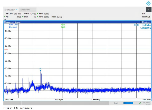
NTNV-n77(3700-3980)-PC3-30-40-M-DFT-BPSK-Edge_1RB_Left -0.15-30-PASS
