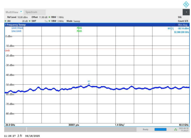
NTNV-n77(3700-3980)-PC3-30-40-M-DFT-QPSK-Edge_1RB_Left -26000-40000-PASS
