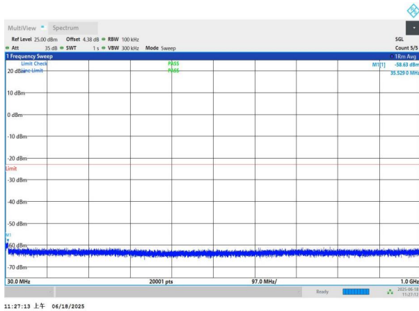
NTNV-n77(3700-3980)-PC3-30-40-H-DFT-BPSK-Edge_1RB_Left -30-1000-PASS
