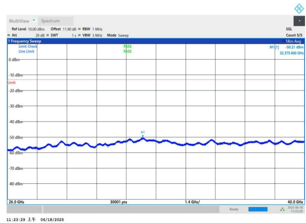
NTNV-n77(3700-3980)-PC3-30-40-L-DFT-QPSK-Edge_1RB_Left- 26000-40000-PASS
