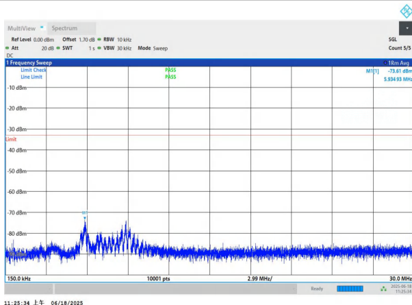
NTNV-n77(3700-3980)-PC3-30-40-M-DFT-QPSK-Edge_1RB_Left -0.15-30-PASS
