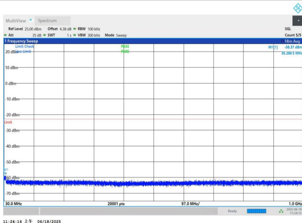
NTNV-n77(3700-3980)-PC3-30-40-M-DFT-BPSK-Edge_1RB_Left -30-1000-PASS
