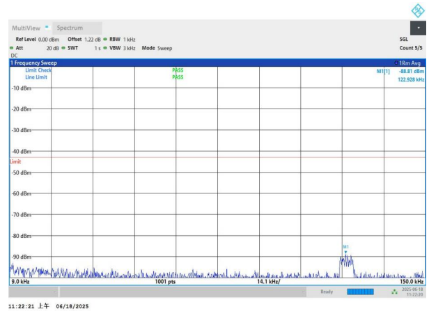
NTNV-n77(3700-3980)-PC3-30-40-L-DFT-QPSK-Edge_1RB_Left- 0.009-0.15-PASS
