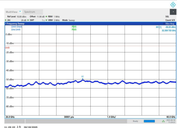
NTNV-n77(3700-3980)-PC3-30-40-H-DFT-QPSK-Edge_1RB_Left -26000-40000-PASS
