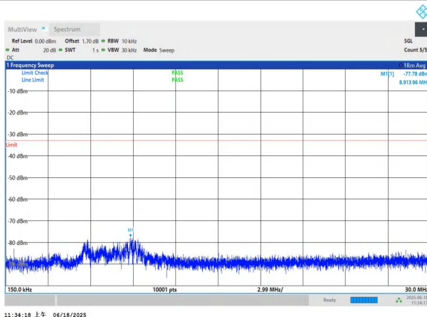
NTNV-n77(3700-3980)-PC3-30-50-M-DFT-QPSK-Edge_1RB_Left -0.15-30-PASS
