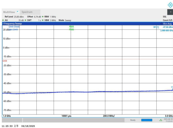
NTNV-n77(3700-3980)-PC3-30-40-M-DFT-QPSK-Edge_1RB_Left -1000-3000-PASS
