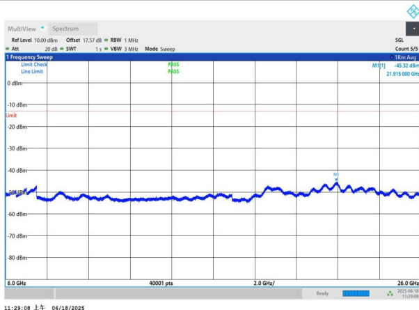
NTNV-n77(3700-3980)-PC3-30-40-H-DFT-QPSK-Edge_1RB_Left -6000-26000-PASS
