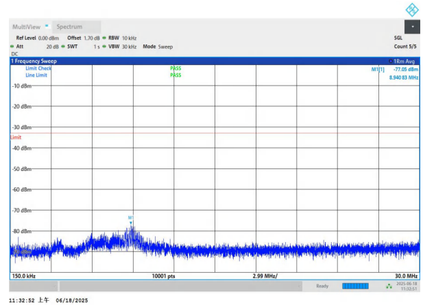
NTNV-n77(3700-3980)-PC3-30-50-M-DFT-BPSK-Edge_1RB_Left -0.15-30-PASS
