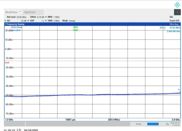
NTNV-n77(3700-3980)-PC3-30-50-M-DFT-BPSK-Edge_1RB_Left -1000-3000-PASS
