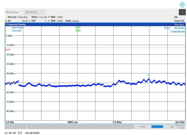
NTNV-n77(3700-3980)-PC3-30-50-M-DFT-BPSK-Edge_1RB_Left -6000-26000-PASS
