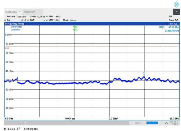
NTNV-n77(3700-3980)-PC3-30-40-M-DFT-BPSK-Edge_1RB_Left -6000-26000-PASS
