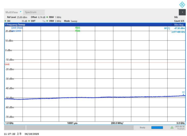
NTNV-n77(3700-3980)-PC3-30-40-H-DFT-BPSK-Edge_1RB_Left 1000-3000-PASS
