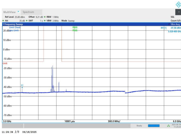
NTNV-n77(3700-3980)-PC3-30-40-M-DFT-BPSK-Edge_1RB_Left -3000-6000-PASS
