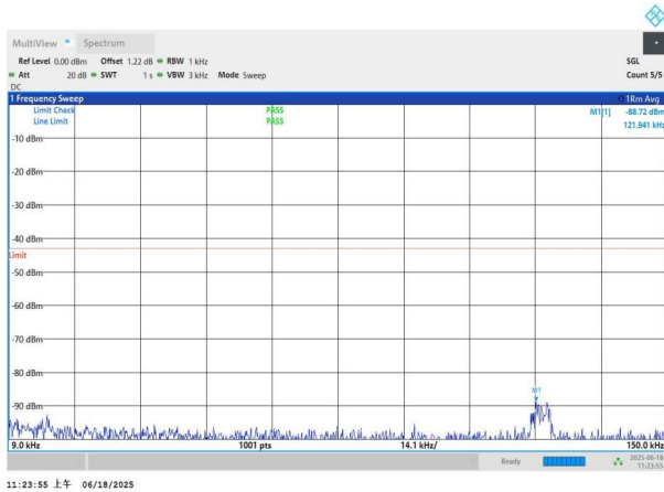
NTNV-n77(3700-3980)-PC3-30-40-M-DFT-BPSK-Edge_1RB_Left -0.009-0.15-PASS
