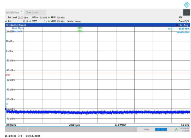
NTNV-n77(3700-3980)-PC3-30-40-H-DFT-QPSK-Edge_1RB_Left -30-1000-PASS
