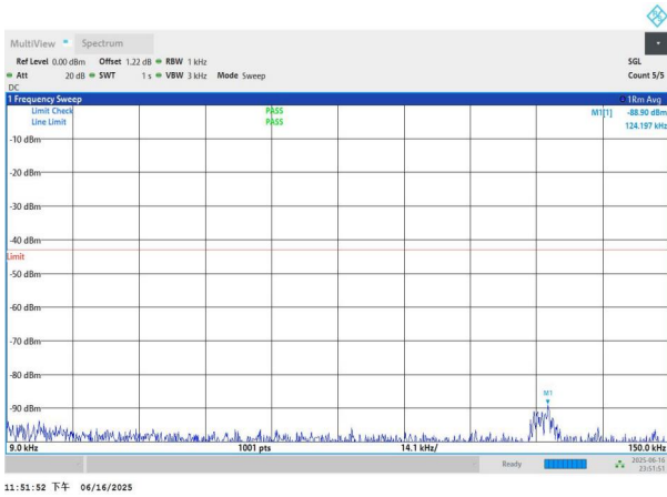
NTNV-n77(3450-3550)-PC3-30-90-M-DFT-BPSK-Edge_1RB_Left-0.009-0.15-PASS
