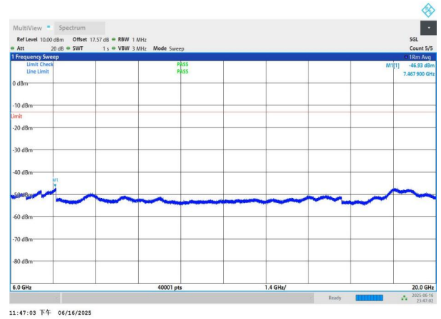
NTNV-n77(3450-3550)-PC3-30-80-H-DFT-BPSK-Edge_1RB_Left 6000-20000-PASS
