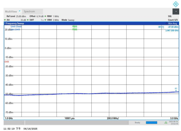
NTNV-n77(3450-3550)-PC3-30-90-M-DFT-BPSK-Edge_1RB_Left-1000-3000-PASS
