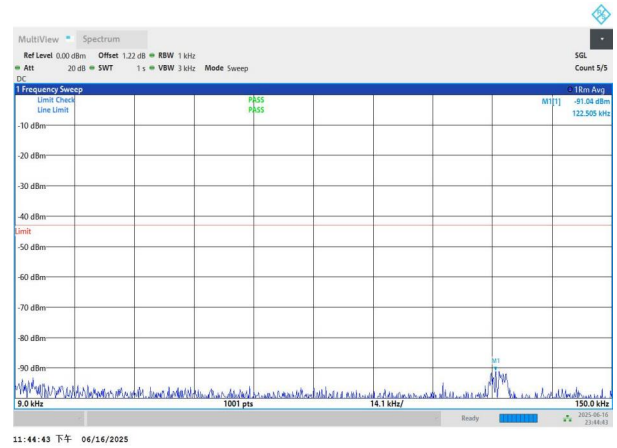
NTNV-n77(3450-3550)-PC3-30-80-M-DFT-QPSK-Edge_1RB_Left -0.009-0.15-PASS
