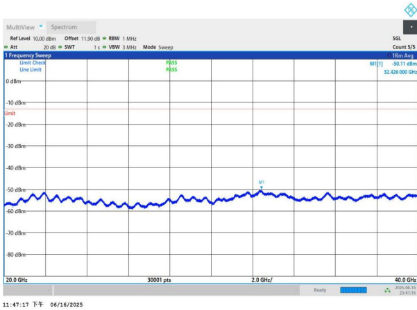
NTNV-n77(3450-3550)-PC3-30-80-H-DFT-BPSK-Edge_1RB_Left -20000-40000-PASS
