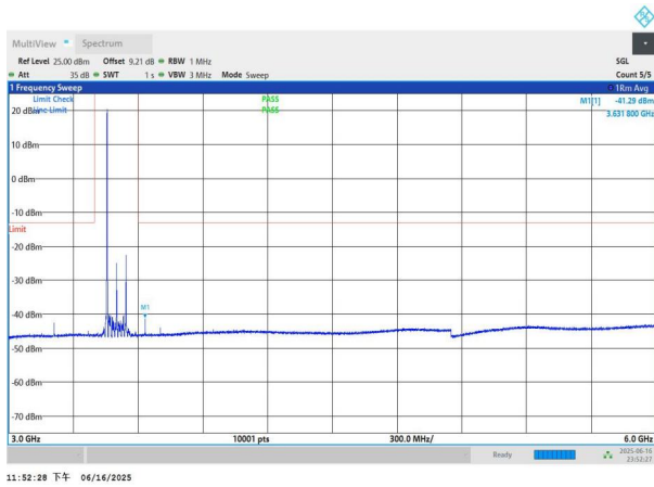
NTNV-n77(3450-3550)-PC3-30-90-M-DFT-BPSK-Edge_1RB_Left -3000-6000-PASS
