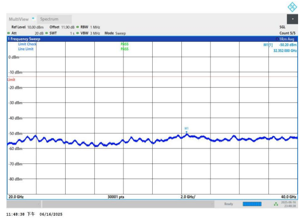
NTNV-n77(3450-3550)-PC3-30-80-H-DFT-QPSK-Edge_1RB_Left -20000-40000-PASS
