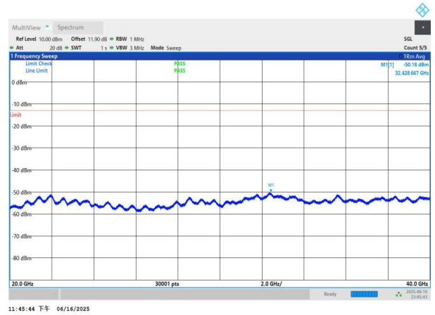
NTNV-n77(3450-3550)-PC3-30-80-M-DFT-QPSK-Edge_1RB_Left -20000-40000-PASS
