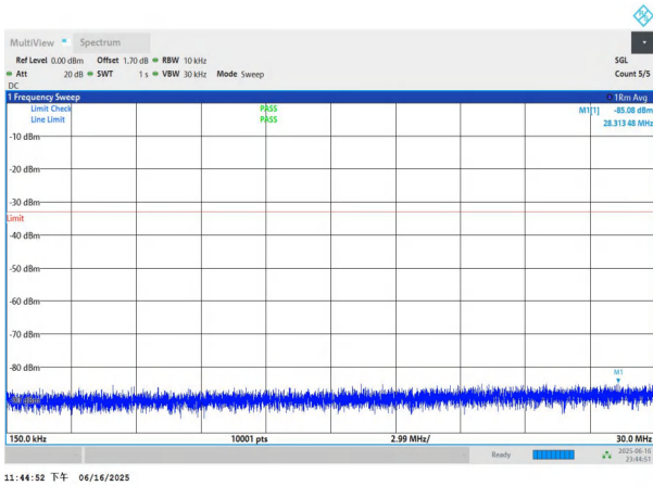
NTNV-n77(3450-3550)-PC3-30-80-M-DFT-QPSK-Edge_1RB_Left -0.15-30-PASS
