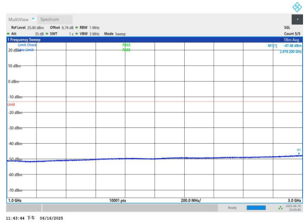
NTNV-n77(3450-3550)-PC3-30-80-M-DFT-BPSK-Edge_1RB_Left-1000-3000-PASS
