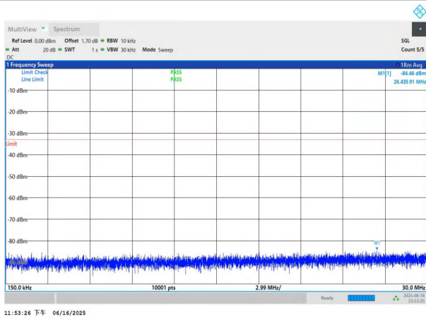
NTNV-n77(3450-3550)-PC3-30-90-M-DFT-QPSK-Edge_1RB_Left -0.15-30-PASS
