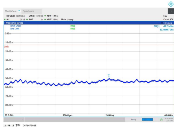
NTNV-n77(3450-3550)-PC3-30-90-M-DFT-QPSK-Edge_1RB_Left -20000-40000-PASS
