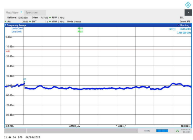
NTNV-n77(3450-3550)-PC3-30-80-M-DFT-BPSK-Edge_1RB_Left -6000-20000-PASS
