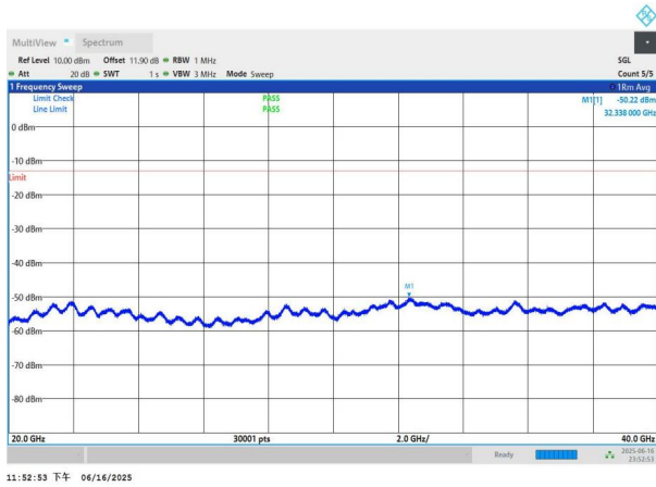
NTNV-n77(3450-3550)-PC3-30-90-M-DFT-BPSK-Edge_1RB_Left -20000-40000-PASS
