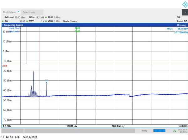
NTNV-n77(3450-3550)-PC3-30-80-H-DFT-BPSK-Edge_1RB_Left -3000-6000-PASS
