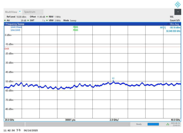
NTNV-n77(3450-3550)-PC3-30-80-L-DFT-QPSK-Edge_1RB_Left-20000-40000-PASS
