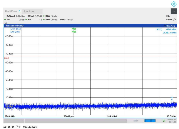
NTNV-n77(3450-3550)-PC3-30-80-H-DFT-BPSK-Edge_1RB_Left 0.15-30-PASS
