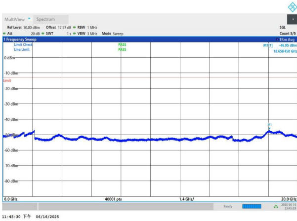
NTNV-n77(3450-3550)-PC3-30-80-M-DFT-QPSK-Edge_1RB_Left -6000-20000-PASS
