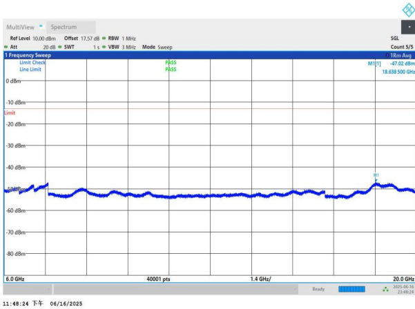
NTNV-n77(3450-3550)-PC3-30-80-H-DFT-QPSK-Edge_1RB_Left -6000-20000-PASS
