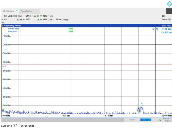
NTNV-n77(3450-3550)-PC3-30-90-H-DFT-BPSK-Edge_1RB_Left -0.009-0.15-PASS
