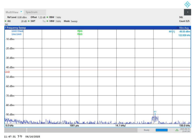
NTNV-n77(3450-3550)-PC3-30-80-H-DFT-QPSK-Edge_1RB_Left -0.009-0.15-PASS
