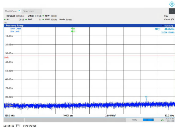
NTNV-n77(3450-3550)-PC3-30-90-H-DFT-BPSK-Edge_1RB_Left 0.15-30-PASS
