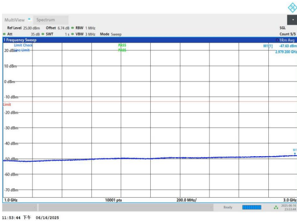
NTNV-n77(3450-3550)-PC3-30-90-M-DFT-QPSK-Edge_1RB_Left -1000-3000-PASS
