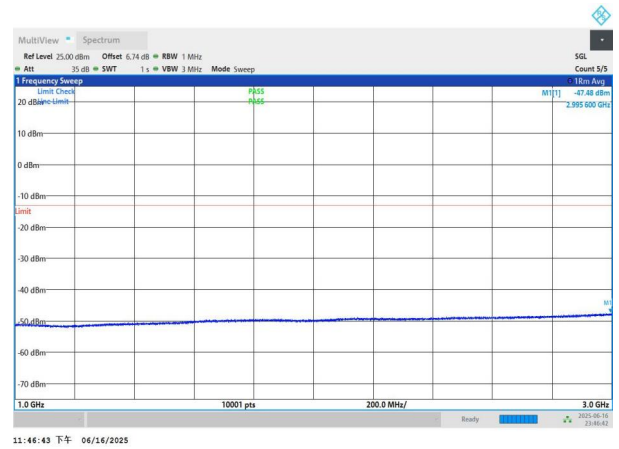
NTNV-n77(3450-3550)-PC3-30-80-H-DFT-BPSK-Edge_1RB_Left 1000-3000-PASS
