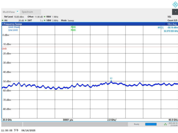
NTNV-n77(3450-3550)-PC3-30-90-L-DFT-BPSK-Edge_1RB_Left- 20000-40000-PASS
