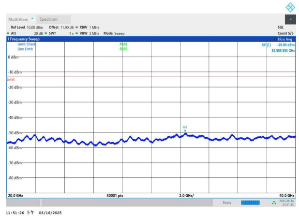
NTNV-n77(3450-3550)-PC3-30-90-L-DFT-QPSK-Edge_1RB_Left-20000-40000-PASS
