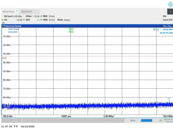
NTNV-n77(3450-3550)-PC3-30-80-H-DFT-QPSK-Edge_1RB_Left -0.15-30-PASS
