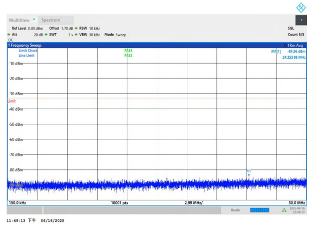
NTNV-n77(3450-3550)-PC3-30-90-L-DFT-BPSK-Edge_1RB_Left-0.009-0.15-PASS NTVN-n77(3450-3550)-PC3-30-90-L-DFT-BPSK-Edge_1RB_Left-0.15-30-PASS
