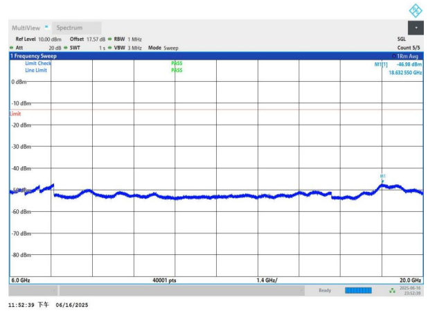
NTNV-n77(3450-3550)-PC3-30-90-M-DFT-BPSK-Edge_1RB_Left -6000-20000-PASS
