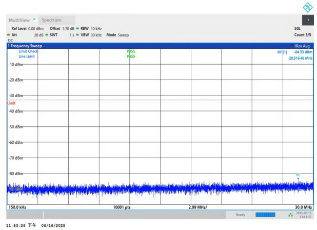
NTNV-n77(3450-3550)-PC3-30-80-M-DFT-BPSK-Edge_1RB_Left-0.15-30-PASS
