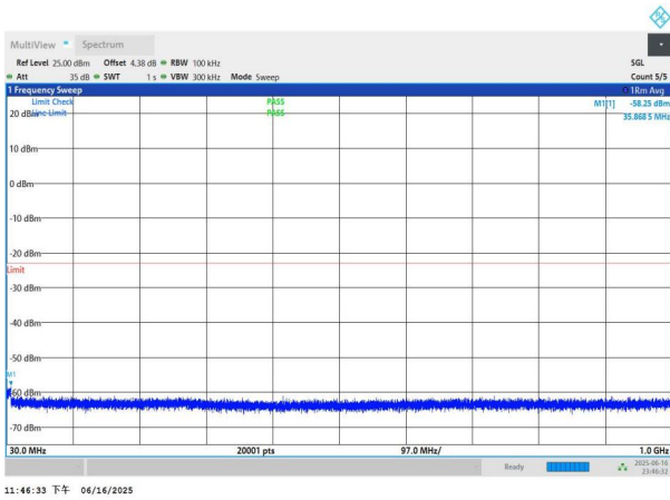
NTNV-n77(3450-3550)-PC3-30-80-H-DFT-BPSK-Edge_1RB_Left -30-1000-PASS
