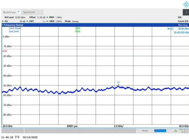
NTNV-n77(3450-3550)-PC3-30-80-M-DFT-BPSK-Edge_1RB_Left -20000-40000-PASS
