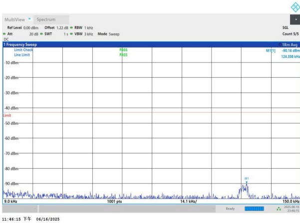
NTNV-n77(3450-3550)-PC3-30-80-H-DFT-BPSK-Edge_1RB_Left -0.009-0.15-PASS
