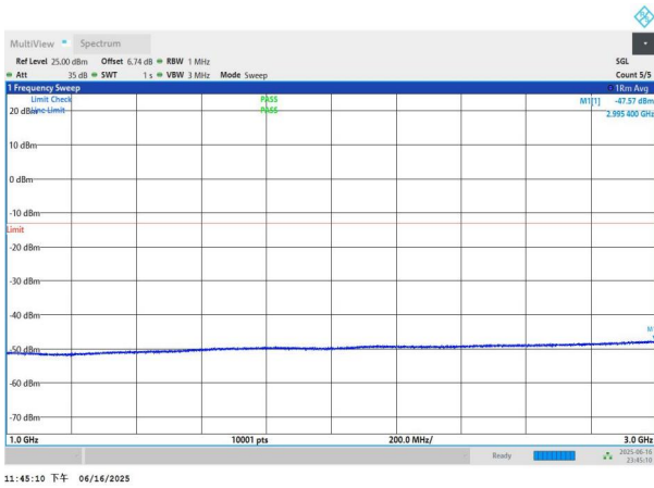
NTNV-n77(3450-3550)-PC3-30-80-M-DFT-QPSK-Edge_1RB_Left -1000-3000-PASS
