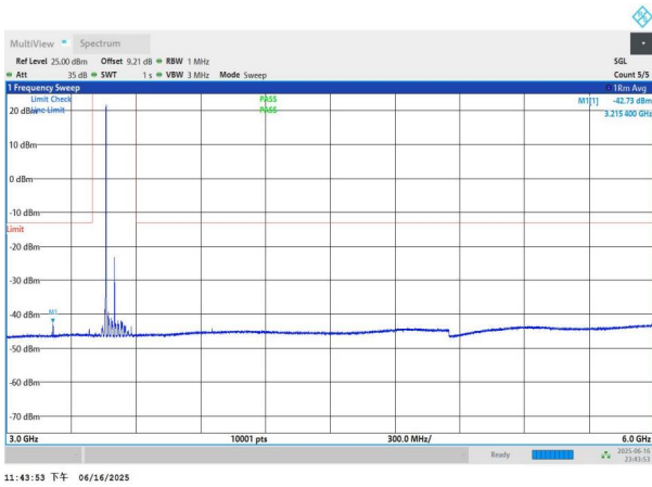
NTNV-n77(3450-3550)-PC3-30-80-M-DFT-BPSK-Edge_1RB_Left -3000-6000-PASS
