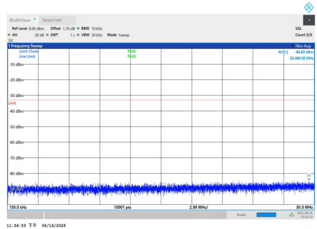
NTNV-n77(3450-3550)-PC3-30-70-M-DFT-BPSK-Edge_1RB_Left -0.15-30-PASS
