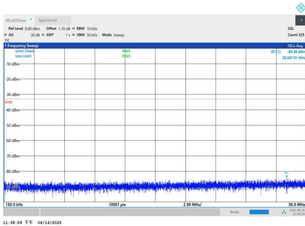
NTNV-n77(3450-3550)-PC3-30-70-H-DFT-QPSK-Edge_1RB_Left -0.15-30-PASS
