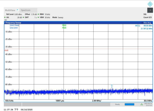
NTNV-n77(3450-3550)-PC3-30-70-H-DFT-BPSK-Edge_1RB_Left 0.15-30-PASS
