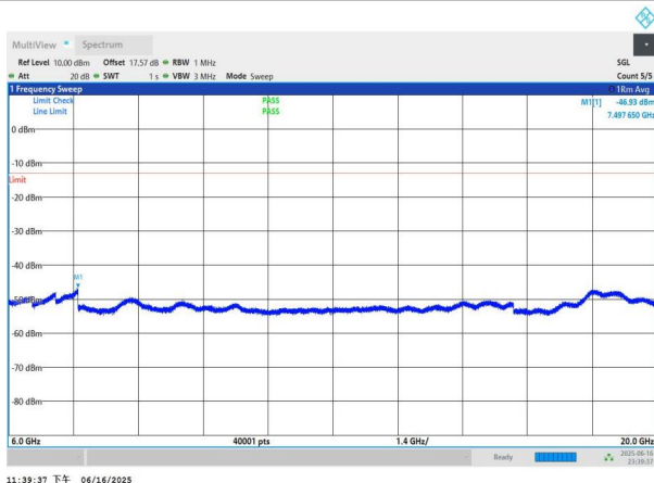
NTNV-n77(3450-3550)-PC3-30-70-H-DFT-QPSK-Edge_1RB_Left -6000-20000-PASS
