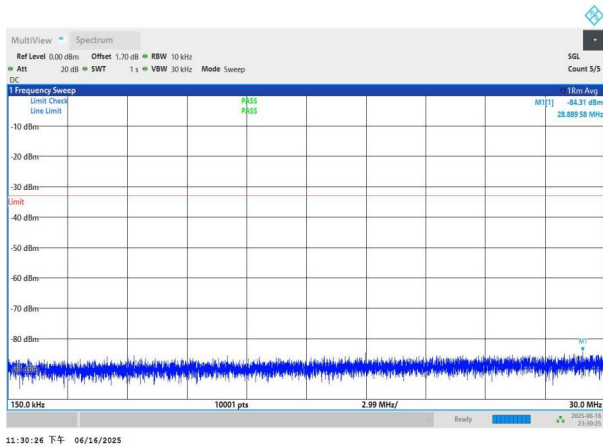
NTNV-n77(3450-3550)-PC3-30-60-H-DFT-QPSK-Edge_1RB_Left -0.15-30-PASS
