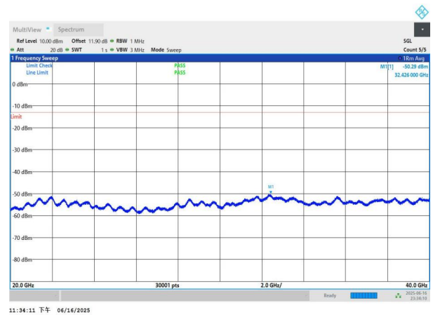
NTNV-n77(3450-3550)-PC3-30-70-L-DFT-QPSK-Edge_1RB_Left- 20000-40000-PASS
