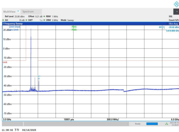
NTNV-n77(3450-3550)-PC3-30-70-H-DFT-BPSK-Edge_1RB_Left -3000-6000-PASS
