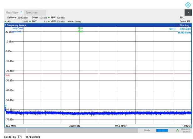
NTNV-n77(3450-3550)-PC3-30-60-H-DFT-QPSK-Edge_1RB_Left -30-1000-PASS
