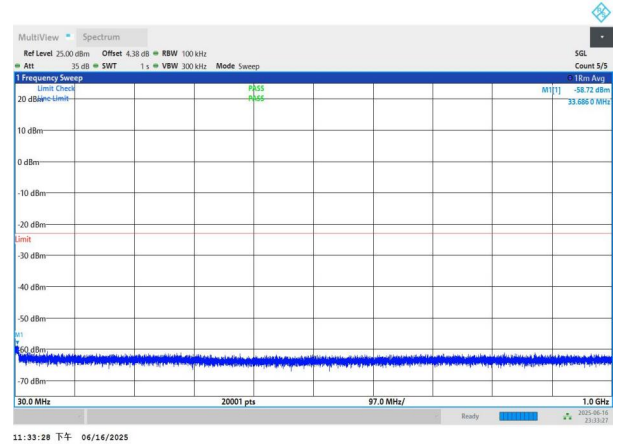
NTNV-n77(3450-3550)-PC3-30-70-L-DFT-QPSK-Edge_1RB_Left- 30-1000-PASS
