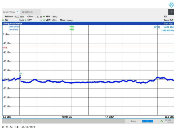
NTNV-n77(3450-3550)-PC3-30-60-H-DFT-QPSK-Edge_1RB_Left -6000-20000-PASS
