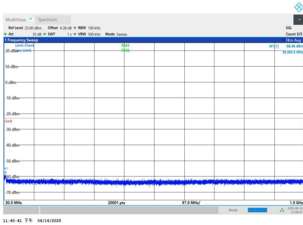
NTNV-n77(3450-3550)-PC3-30-80-L-DFT-BPSK-Edge_1RB_Left- 30-1000-PASS
