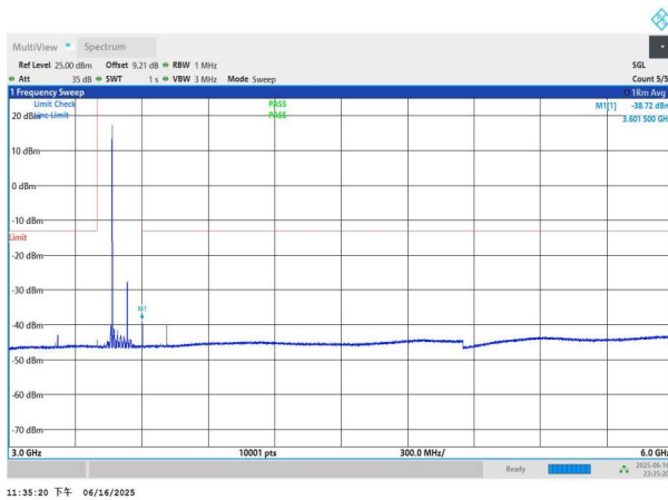
NTNV-n77(3450-3550)-PC3-30-70-M-DFT-BPSK-Edge_1RB_Left -3000-6000-PASS
