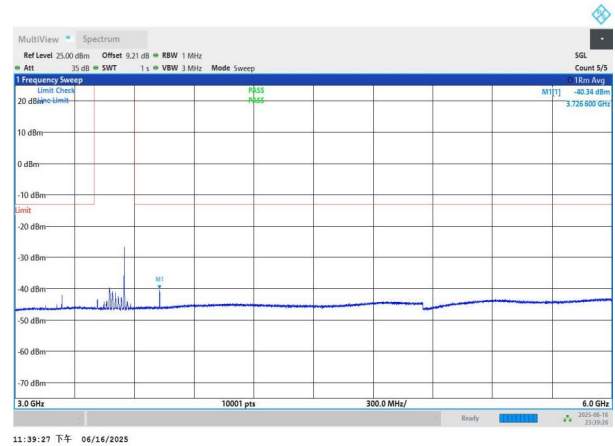
NTNV-n77(3450-3550)-PC3-30-70-H-DFT-QPSK-Edge_1RB_Left -3000-6000-PASS
