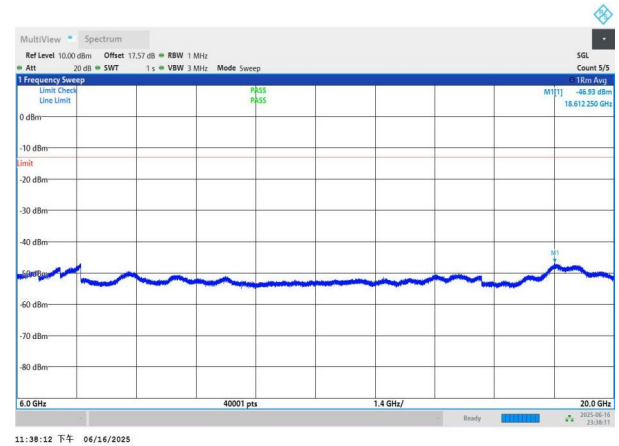
NTNV-n77(3450-3550)-PC3-30-70-H-DFT-BPSK-Edge_1RB_Left 6000-20000-PASS
