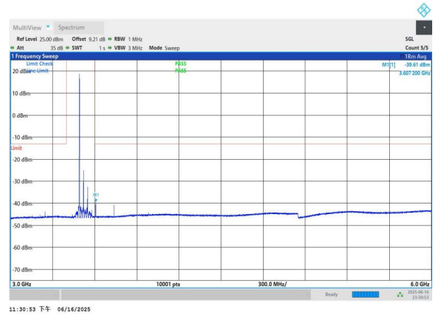
NTNV-n77(3450-3550)-PC3-30-60-H-DFT-QPSK-Edge_1RB_Left -3000-6000-PASS
