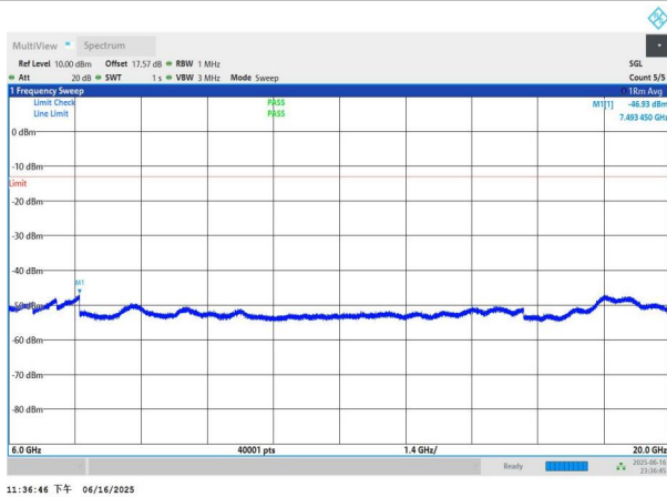
NTNV-n77(3450-3550)-PC3-30-70-M-DFT-QPSK-Edge_1RB_Left -6000-20000-PASS
