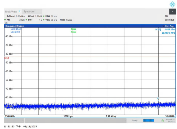
NTNV-n77(3450-3550)-PC3-30-70-L-DFT-BPSK-Edge_1RB_Left- 0.15-30-PASS
