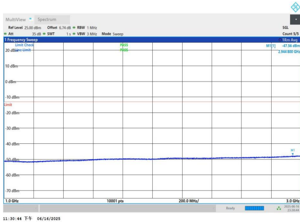
NTNV-n77(3450-3550)-PC3-30-60-H-DFT-QPSK-Edge_1RB_Left -1000-3000-PASS
