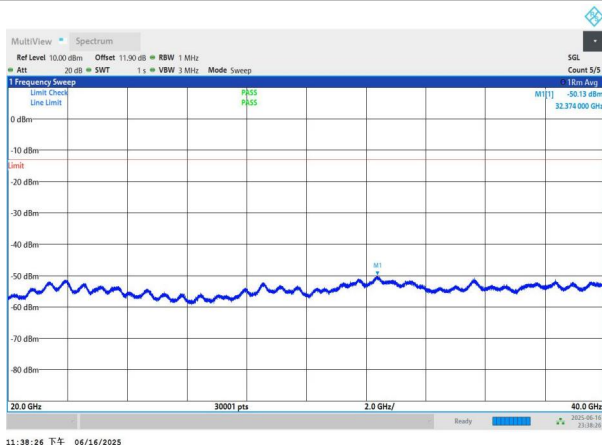
NTNV-n77(3450-3550)-PC3-30-70-H-DFT-BPSK-Edge_1RB_Left -20000-40000-PASS
