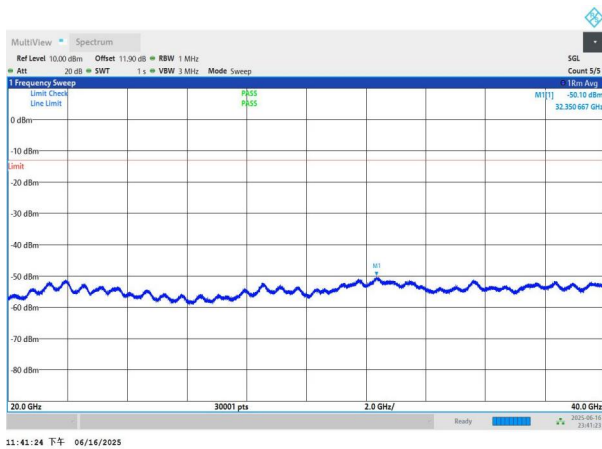
NTNV-n77(3450-3550)-PC3-30-80-L-DFT-BPSK-Edge_1RB_Left- 20000-40000-PASS
