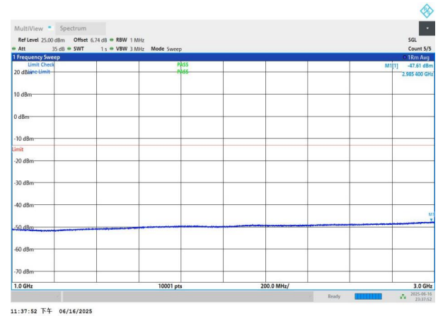
NTNV-n77(3450-3550)-PC3-30-70-H-DFT-BPSK-Edge_1RB_Left 1000-3000-PASS
