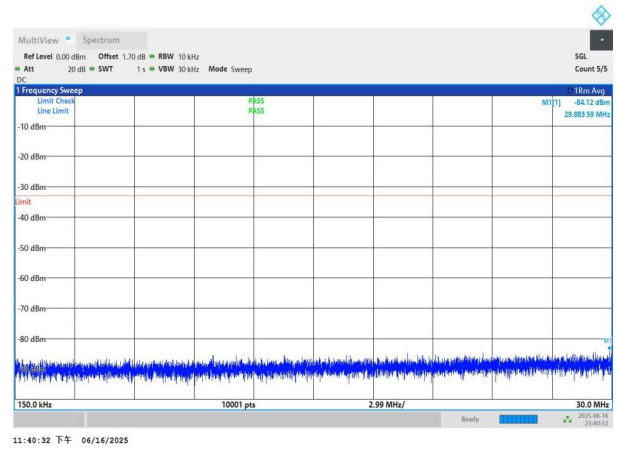
NTNV-n77(3450-3550)-PC3-30-80-L-DFT-BPSK-Edge_1RB_Left- 0.15-30-PASS
