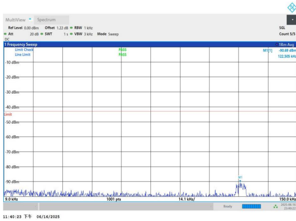
NTNV-n77(3450-3550)-PC3-30-80-L-DFT-BPSK-Edge_1RB_Left- 0.009-0.15-PASS
