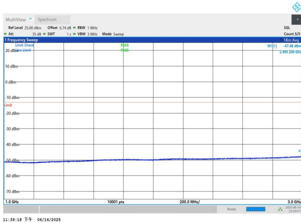
NTNV-n77(3450-3550)-PC3-30-70-H-DFT-QPSK-Edge_1RB_Left -1000-3000-PASS
