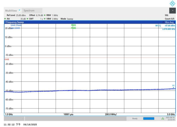
NTNV-n77(3450-3550)-PC3-30-70-L-DFT-BPSK-Edge_1RB_Left- 1000-3000-PASS
