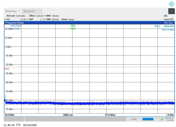
NTNV-n77(3450-3550)-PC3-30-80-L-DFT-QPSK-Edge_1RB_Left- 30-1000-PASS
