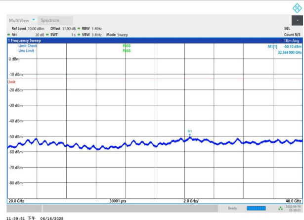
NTNV-n77(3450-3550)-PC3-30-70-H-DFT-QPSK-Edge_1RB_Left -20000-40000-PASS
