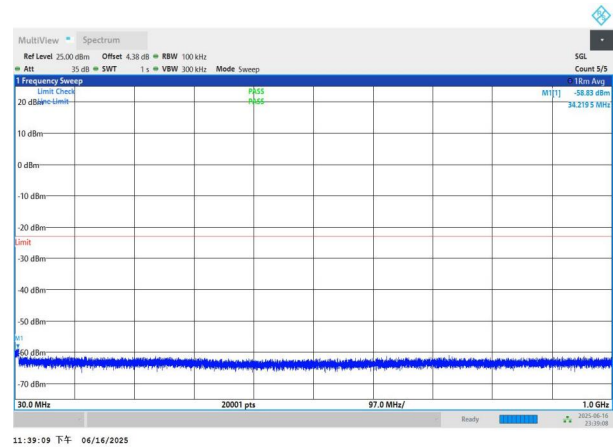
NTNV-n77(3450-3550)-PC3-30-70-H-DFT-QPSK-Edge_1RB_Left -30-1000-PASS
