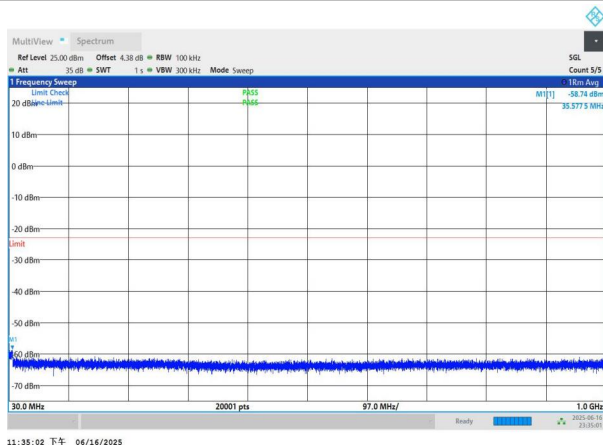
NTNV-n77(3450-3550)-PC3-30-70-M-DFT-BPSK-Edge_1RB_Left -30-1000-PASS
