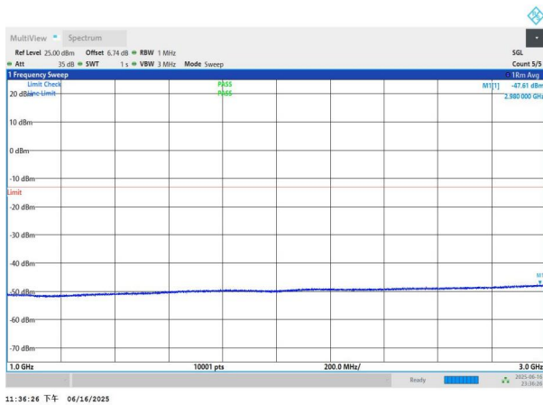
NTNV-n77(3450-3550)-PC3-30-70-M-DFT-QPSK-Edge_1RB_Left -1000-3000-PASS
