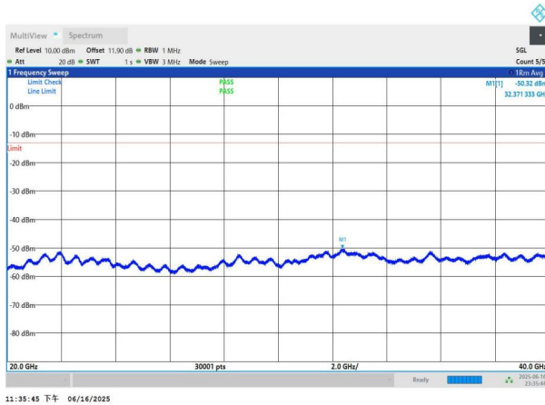
NTNV-n77(3450-3550)-PC3-30-70-M-DFT-BPSK-Edge_1RB_Left -20000-40000-PASS
