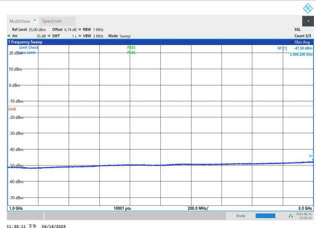
NTNV-n77(3450-3550)-PC3-30-70-M-DFT-BPSK-Edge_1RB_Left -1000-3000-PASS
