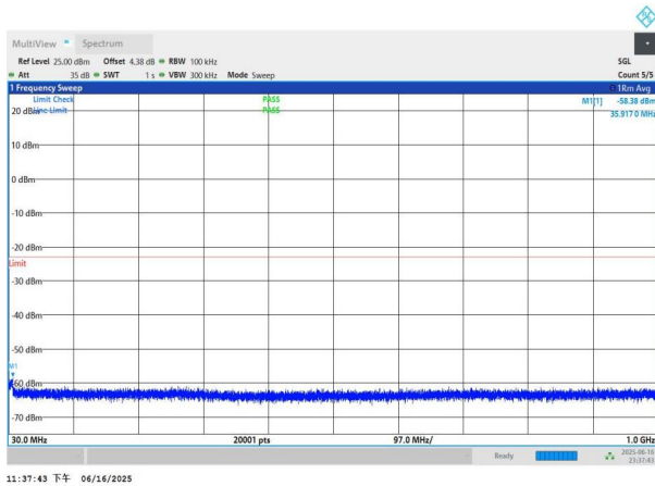
NTNV-n77(3450-3550)-PC3-30-70-H-DFT-BPSK-Edge_1RB_Left -30-1000-PASS
