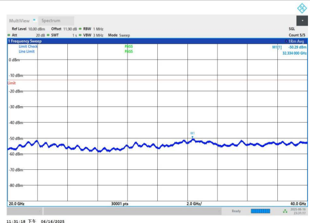
NTNV-n77(3450-3550)-PC3-30-60-H-DFT-QPSK-Edge_1RB_Left -20000-40000-PASS
