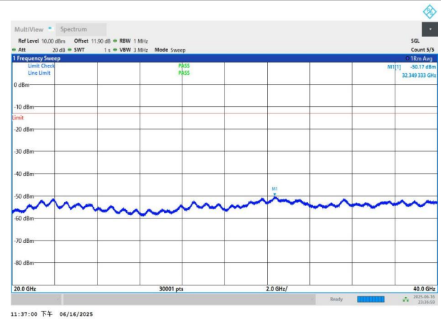
NTNV-n77(3450-3550)-PC3-30-70-M-DFT-QPSK-Edge_1RB_Left -20000-40000-PASS
