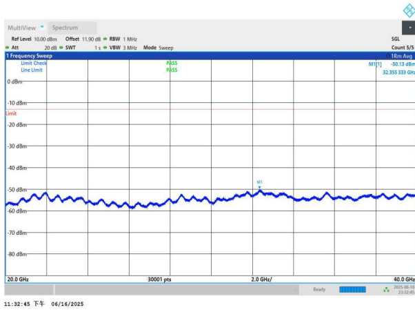
NTNV-n77(3450-3550)-PC3-30-70-L-DFT-BPSK-Edge_1RB_Left- 20000-40000-PASS
