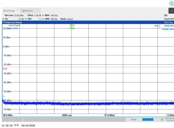
NTNV-n77(3450-3550)-PC3-30-70-L-DFT-BPSK-Edge_1RB_Left- 30-1000-PASS
