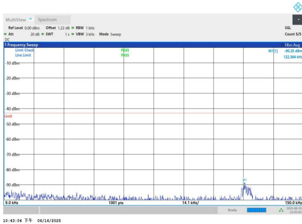
NTNV-n77(3450-3550)-PC3-30-20-M-DFT-BPSK-Edge_1RB_Left -0.009-0.15-PASS
