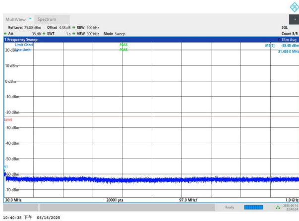
NTNV-n77(3450-3550)-PC3-30-20-L-DFT-BPSK-Edge_1RB_Left- 30-1000-PASS
