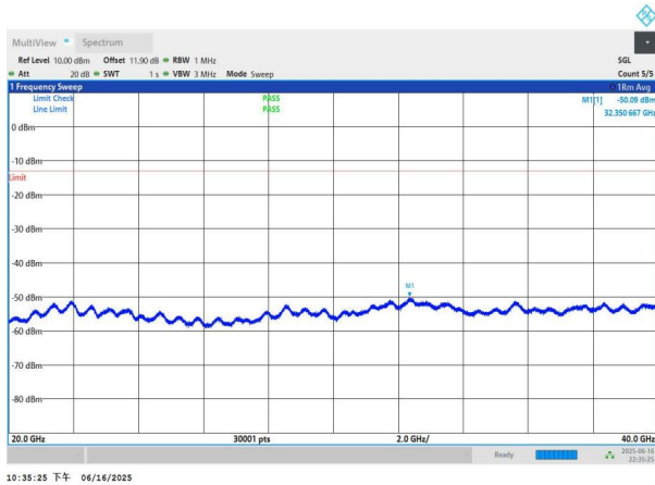
NTNV-n77(3450-3550)-PC3-30-15-M-DFT-BPSK-Edge_1RB_Left -20000-40000-PASS
