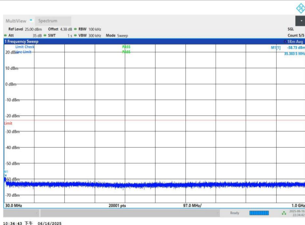
NTNV-n77(3450-3550)-PC3-30-15-M-DFT-BPSK-Edge_1RB_Left -30-1000-PASS
