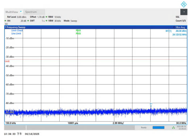
NTNV-n77(3450-3550)-PC3-30-15-M-DFT-BPSK-Edge_1RB_Left -0.15-30-PASS
