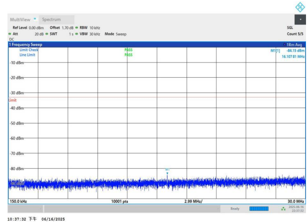
NTNV-n77(3450-3550)-PC3-30-15-H-DFT-BPSK-Edge_1RB_Left 0.15-30-PASS
