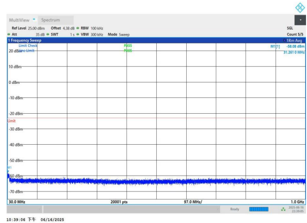
NTNV-n77(3450-3550)-PC3-30-15-H-DFT-QPSK-Edge_1RB_Left -30-1000-PASS
