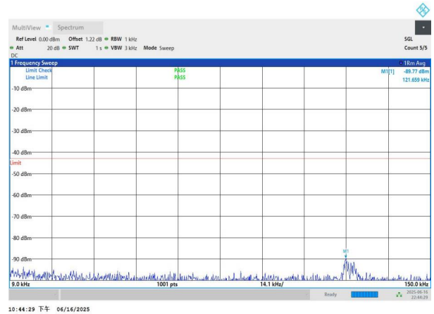
NTNV-n77(3450-3550)-PC3-30-20-M-DFT-QPSK-Edge_1RB_Left -0.009-0.15-PASS
