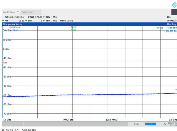
NTNV-n77(3450-3550)-PC3-30-15-L-DFT-QPSK-Edge_1RB_Left- 1000-3000-PASS
