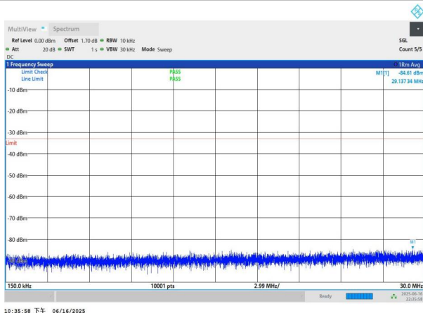
NTNV-n77(3450-3550)-PC3-30-15-M-DFT-QPSK-Edge_1RB_Left -0.15-30-PASS
