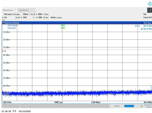
NTNV-n77(3450-3550)-PC3-30-15-H-DFT-QPSK-Edge_1RB_Left -0.15-30-PASS
