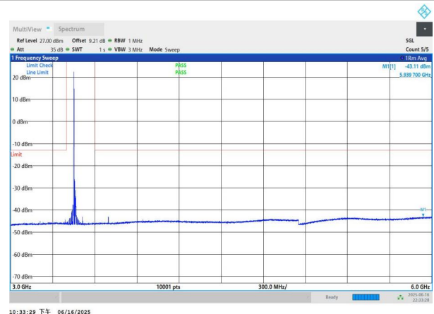
NTNV-n77(3450-3550)-PC3-30-15-L-DFT-QPSK-Edge_1RB_Left- 3000-6000-PASS
