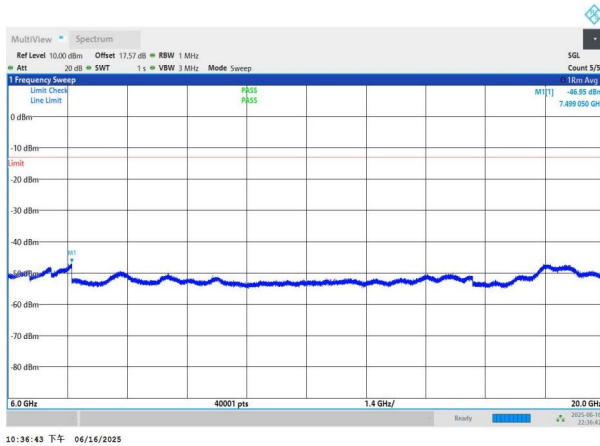
NTNV-n77(3450-3550)-PC3-30-15-M-DFT-QPSK-Edge_1RB_Left -6000-20000-PASS
