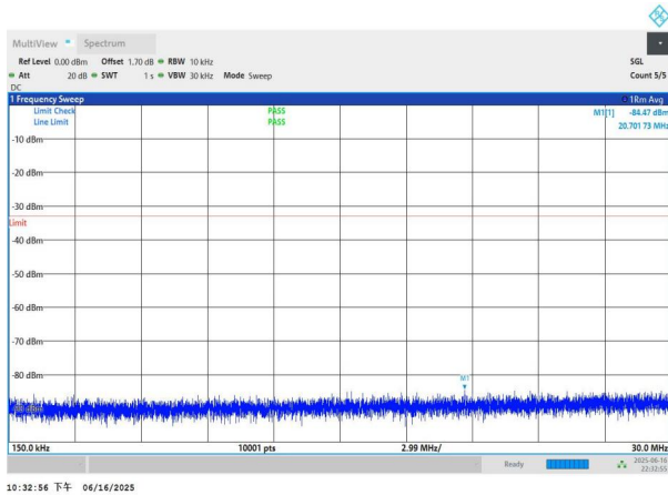
NTNV-n77(3450-3550)-PC3-30-15-L-DFT-QPSK-Edge_1RB_Left- 0.15-30-PASS
