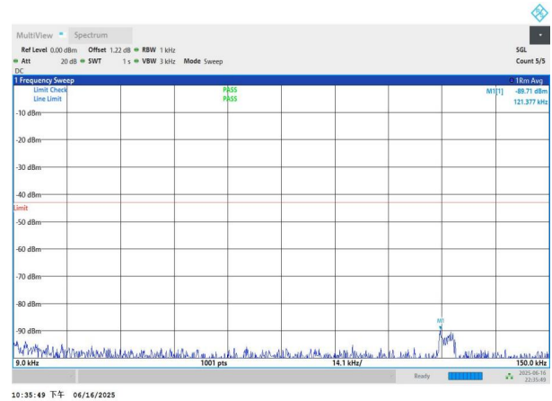
NTNV-n77(3450-3550)-PC3-30-15-M-DFT-QPSK-Edge_1RB_Left -0.009-0.15-PASS
