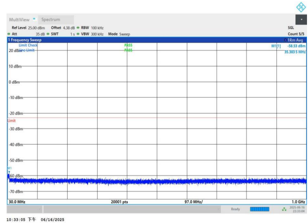
NTNV-n77(3450-3550)-PC3-30-15-L-DFT-QPSK-Edge_1RB_Left- 30-1000-PASS
