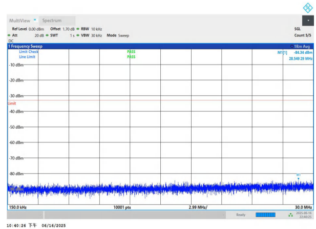
NTNV-n77(3450-3550)-PC3-30-20-L-DFT-BPSK-Edge_1RB_Left- 0.15-30-PASS
