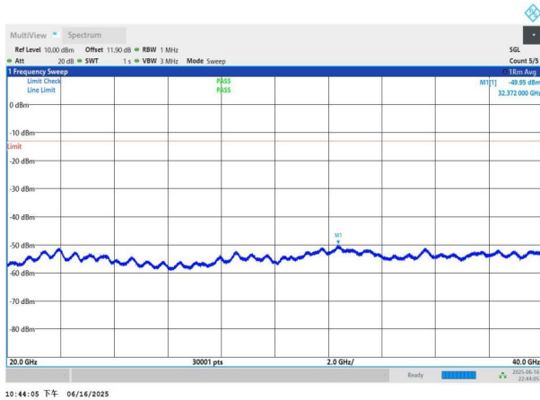
NTNV-n77(3450-3550)-PC3-30-20-M-DFT-BPSK-Edge_1RB_Left -20000-40000-PASS
