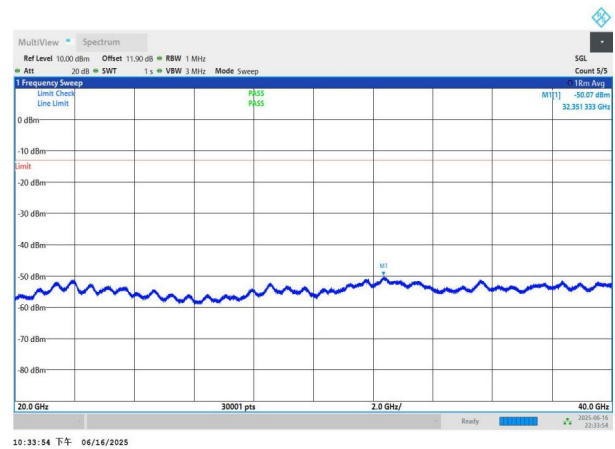
NTNV-n77(3450-3550)-PC3-30-15-L-DFT-QPSK-Edge_1RB_Left- 20000-40000-PASS
