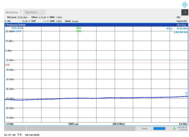
NTNV-n77(3450-3550)-PC3-30-15-H-DFT-BPSK-Edge_1RB_Left 1000-3000-PASS
