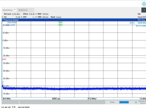
NTNV-n77(3450-3550)-PC3-30-20-M-DFT-BPSK-Edge_1RB_Left -30-1000-PASS
