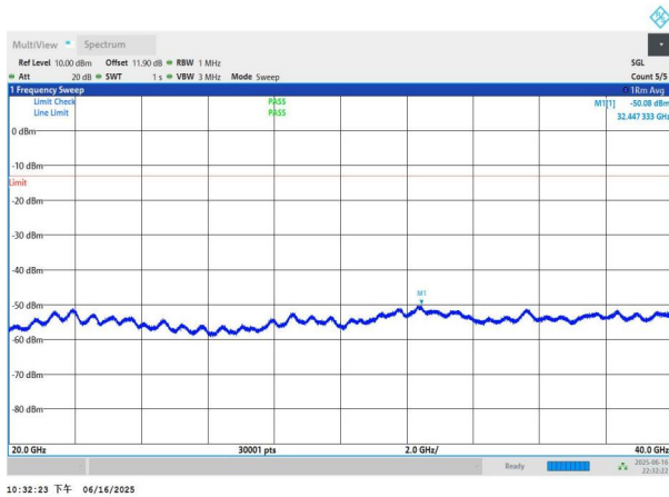
NTNV-n77(3450-3550)-PC3-30-15-L-DFT-BPSK-Edge_1RB_Left- 20000-40000-PASS
