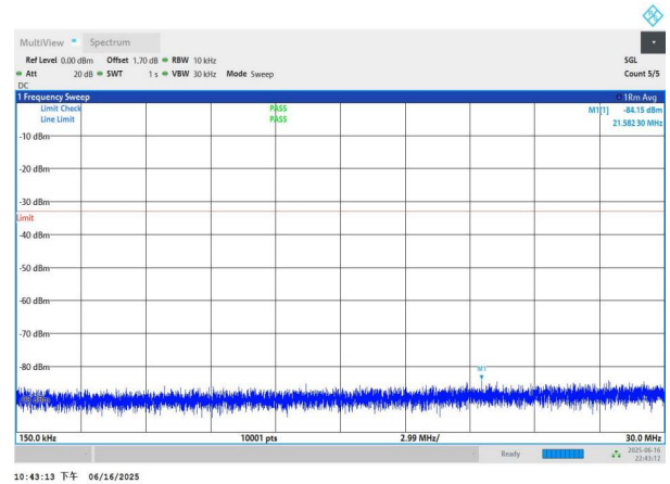
NTNV-n77(3450-3550)-PC3-30-20-M-DFT-BPSK-Edge_1RB_Left -0.15-30-PASS
