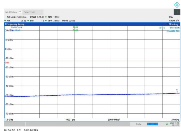
NTNV-n77(3450-3550)-PC3-30-15-M-DFT-BPSK-Edge_1RB_Left -1000-3000-PASS
