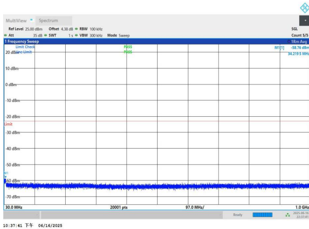
NTNV-n77(3450-3550)-PC3-30-15-H-DFT-BPSK-Edge_1RB_Left -30-1000-PASS
