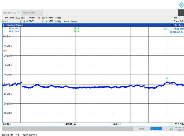
NTNV-n77(3450-3550)-PC3-30-15-H-DFT-QPSK-Edge_1RB_Left -6000-20000-PASS
