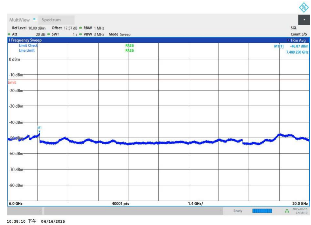
NTNV-n77(3450-3550)-PC3-30-15-H-DFT-BPSK-Edge_1RB_Left 6000-20000-PASS
