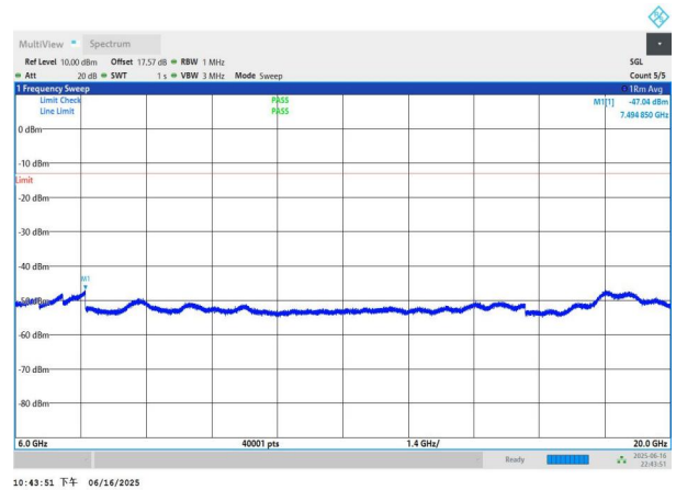
NTNV-n77(3450-3550)-PC3-30-20-M-DFT-BPSK-Edge_1RB_Left -6000-20000-PASS
