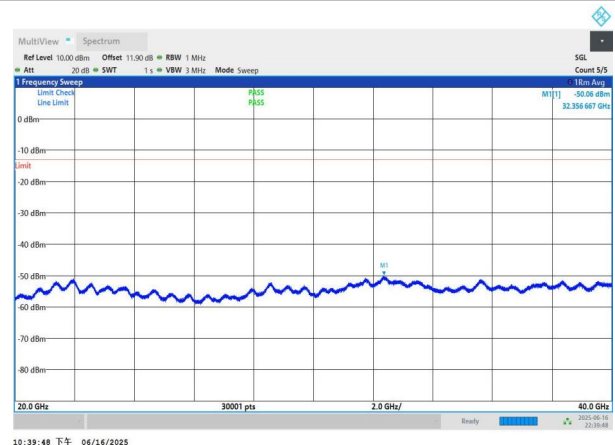
NTNV-n77(3450-3550)-PC3-30-15-H-DFT-QPSK-Edge_1RB_Left -20000-40000-PASS
