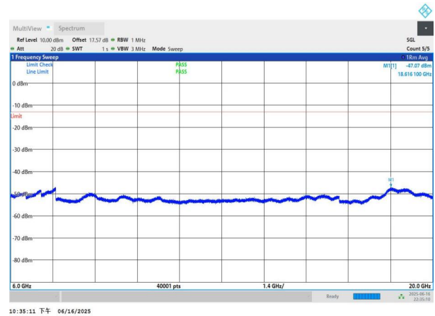
NTNV-n77(3450-3550)-PC3-30-15-M-DFT-BPSK-Edge_1RB_Left -6000-20000-PASS
