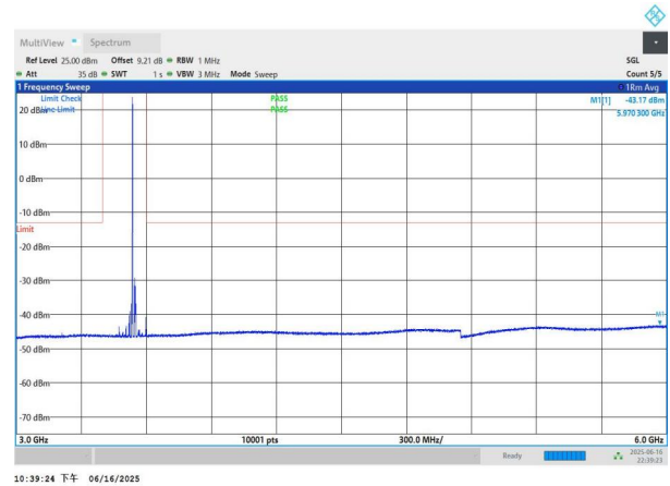
NTNV-n77(3450-3550)-PC3-30-15-H-DFT-QPSK-Edge_1RB_Left -3000-6000-PASS
