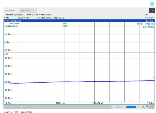
NTNV-n77(3450-3550)-PC3-30-20-M-DFT-BPSK-Edge_1RB_Left -1000-3000-PASS
