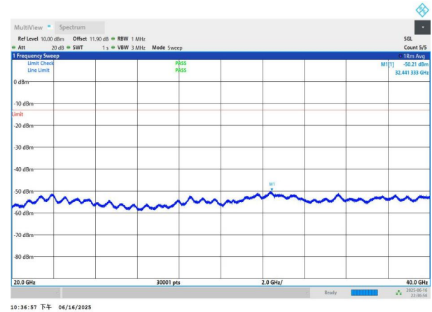
NTNV-n77(3450-3550)-PC3-30-15-M-DFT-QPSK-Edge_1RB_Left -20000-40000-PASS
