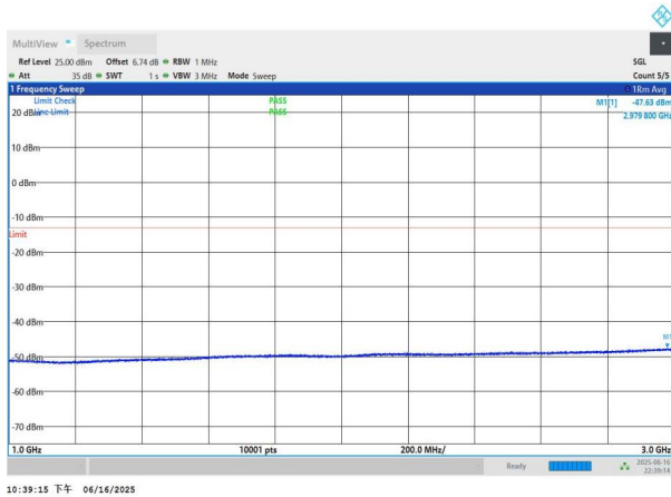
NTNV-n77(3450-3550)-PC3-30-15-H-DFT-QPSK-Edge_1RB_Left -1000-3000-PASS
