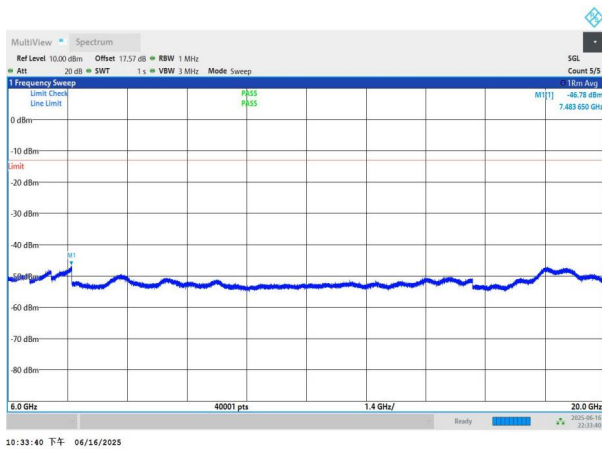
NTNV-n77(3450-3550)-PC3-30-15-L-DFT-QPSK-Edge_1RB_Left- 6000-20000-PASS
