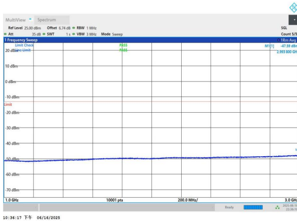
NTNV-n77(3450-3550)-PC3-30-15-M-DFT-QPSK-Edge_1RB_Left -1000-3000-PASS
