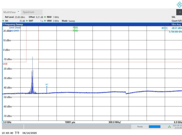
NTNV-n77(3450-3550)-PC3-30-20-M-DFT-BPSK-Edge_1RB_Left -3000-6000-PASS
