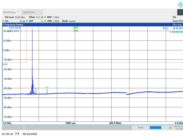
NTNV-n77(3450-3550)-PC3-30-15-M-DFT-BPSK-Edge_1RB_Left -3000-6000-PASS
