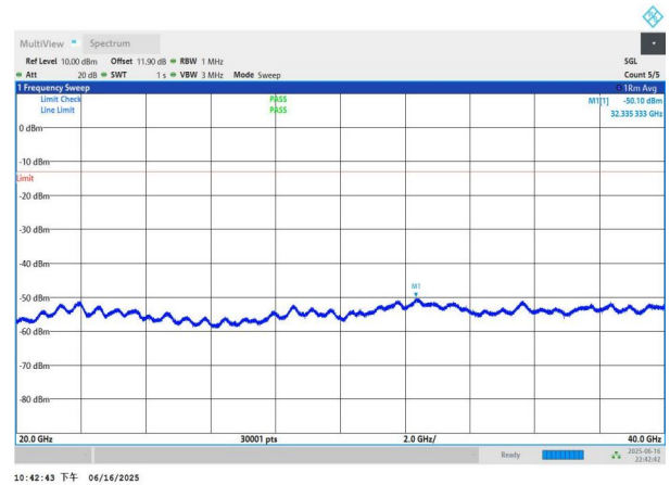
NTNV-n77(3450-3550)-PC3-30-20-L-DFT-QPSK-Edge_1RB_Left- 20000-40000-PASS
