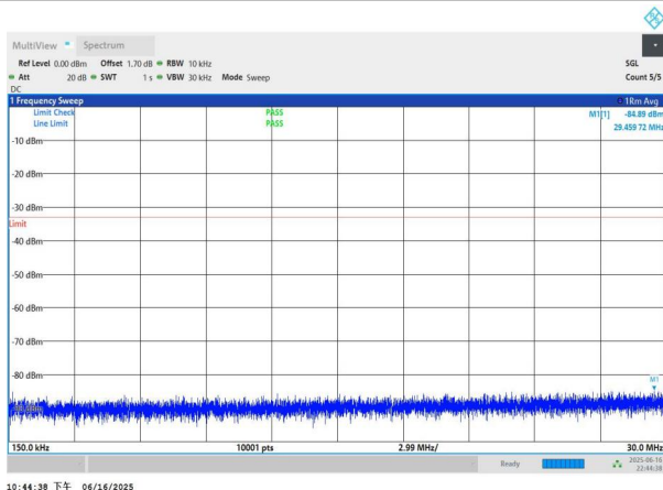
NTNV-n77(3450-3550)-PC3-30-20-M-DFT-QPSK-Edge_1RB_Left -0.15-30-PASS
