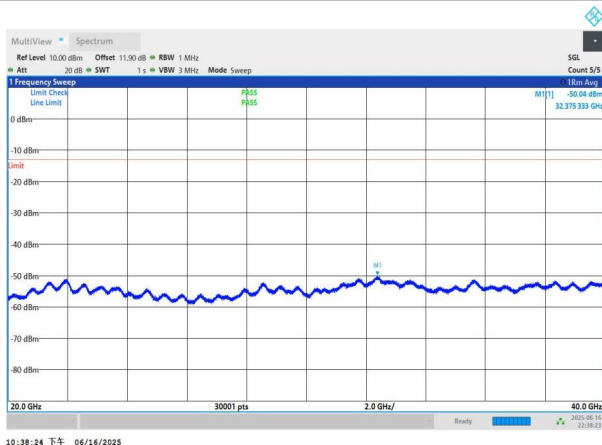
NTNV-n77(3450-3550)-PC3-30-15-H-DFT-BPSK-Edge_1RB_Left -20000-40000-PASS
