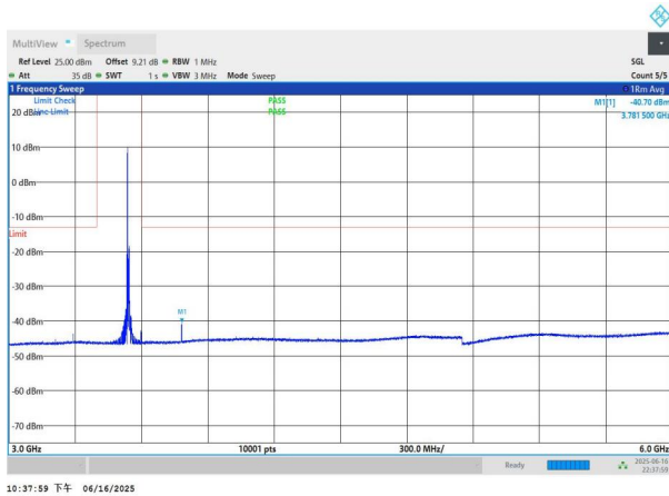
NTNV-n77(3450-3550)-PC3-30-15-H-DFT-BPSK-Edge_1RB_Left -3000-6000-PASS
