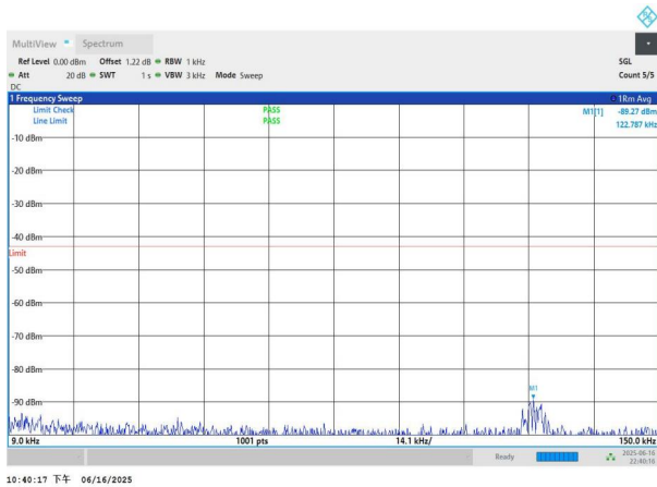
NTNV-n77(3450-3550)-PC3-30-20-L-DFT-BPSK-Edge_1RB_Left- 0.009-0.15-PASS
