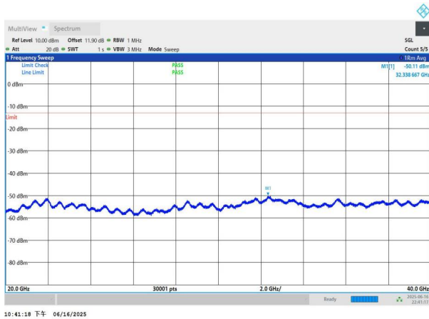
NTNV-n77(3450-3550)-PC3-30-20-L-DFT-BPSK-Edge_1RB_Left- 20000-40000-PASS
