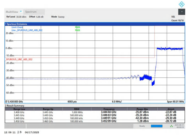
NTNV-n77(3450-3550)-PC3-30-10-L-DFT-BPSK-Outer_Full-P ASS
