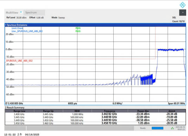
NTNV-n77(3450-3550)-PC3-30-10-L-DFT-QPSK-Outer_Full-P ASS
