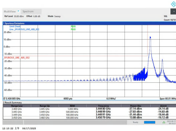
NTNV-n77(3450-3550)-PC3-30-10-L-DFT-BPSK-Edge_1RB_Left-PA SS
