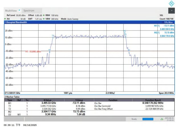
NTNV-n77(3450-3550)-PC3-30-10-M-DFT-256QAM-Outet_Full-An t1-PASS
