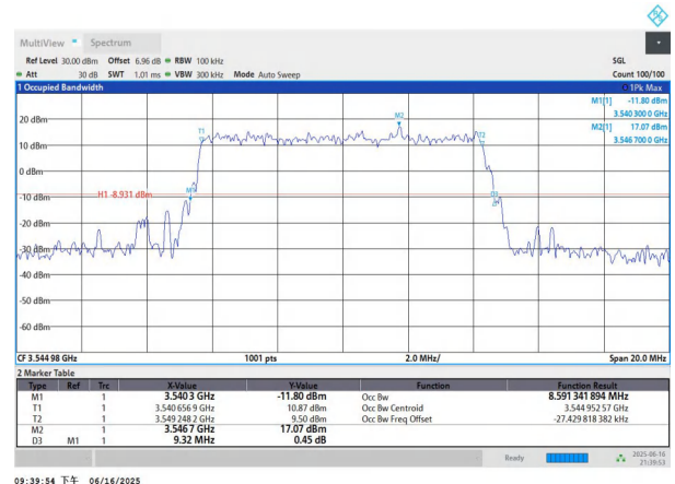
NTNV-n77(3450-3550)-PC3-30-10-H-DFT-QPSK-Outet_Full-Ant1-1 PASS
