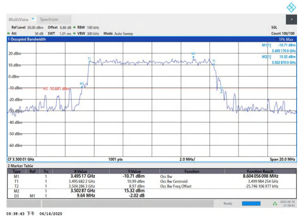
NTNV-n77(3450-3550)-PC3-30-10-M-DFT-16QAM-Outet_Full-Ant 1-PASS
