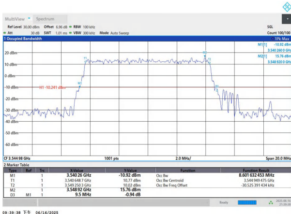
NTNV-n77(3450-3550)-PC3-30-10-H-DFT-BPSK-Outet_Full-Ant1 -PASS
