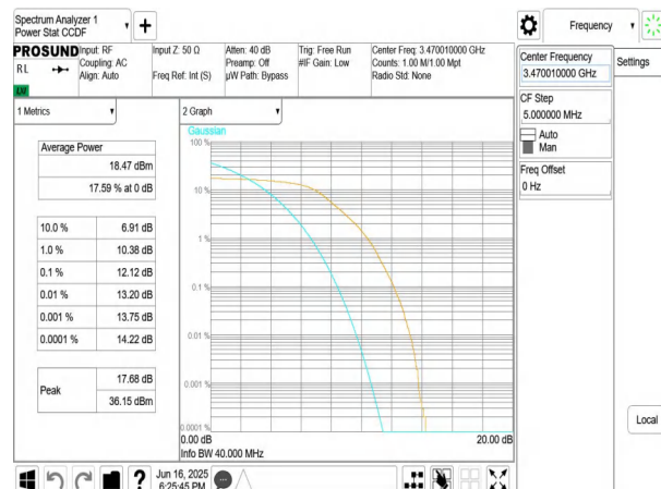
NTNV-n77(3450-3550)-PC3-30-40-L-DFT-QPSK-Outer Full-PAS
