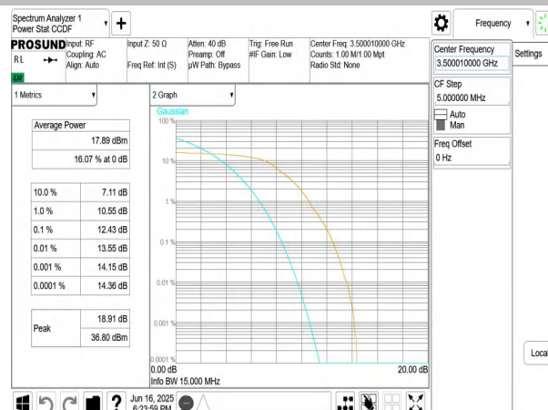
NTNV-n77(3450-3550)-PC3-30-15-M-DFT-QPSK-Outer Full-PAS
