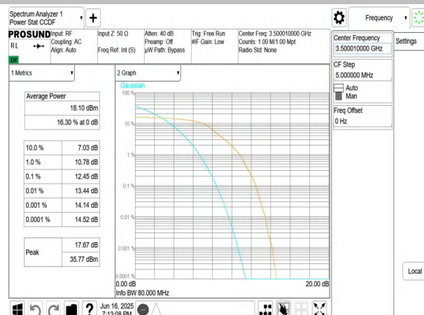
NTNV-n77(3450-3550)-PC3-30-80-M-DFT-QPSK-Outer Full-PAS
