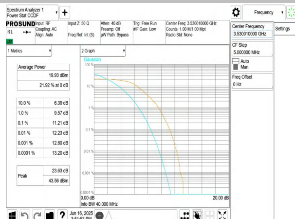
NTNV-n77(3450-3550)-PC3-30-40-H-DFT-QPSK-Outer Full-PAS
