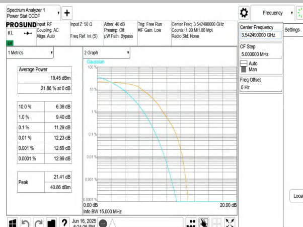
NTNV-n77(3450-3550)-PC3-30-15-H-DFT-QPSK-Outer Full-PAS
