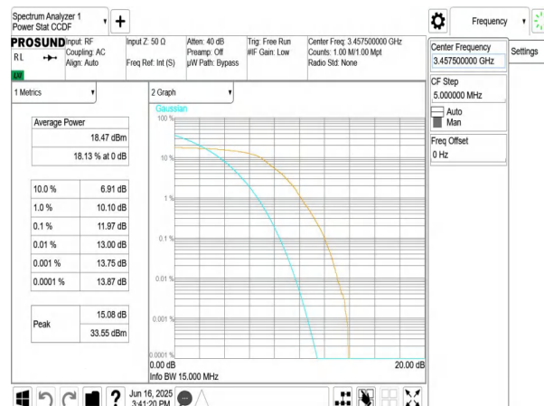
NTNV-n77(3450-3550)-PC3-30-15-L-DFT-QPSK-Outer Full-PAS
