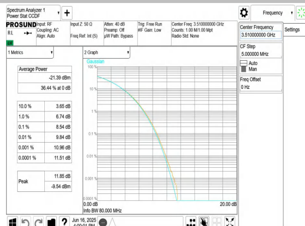
NTNV-n77(3450-3550)-PC3-30-80-H-DFT-QPSK-Outer Full-PAS
