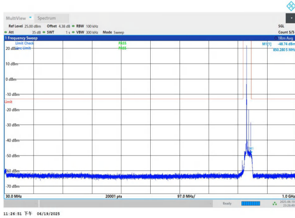
NTNV-n26(824-849)-PC3-15-15-H-DFT-BPSK-Edge_1RB_Left-30-1000-PASS
