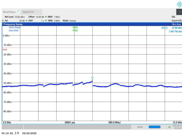
NTNV-n26(824-849)-PC3-15-20-M-DFT-QPSK-Edge_1RB_Left-3.000-12000-PASS
