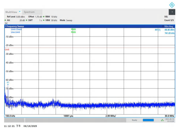
NTNV-n26(824-849)-PC3-15-5-H-DFT-QPSK-Edge_1RB_Left-0.1 5-30-PASS
