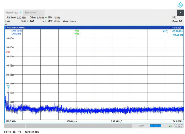
NTNV-n26(824-849)-PC3-15-20-L-DFT-QPSK-Edge_1RB_Left-0.1 5-30-PASS
