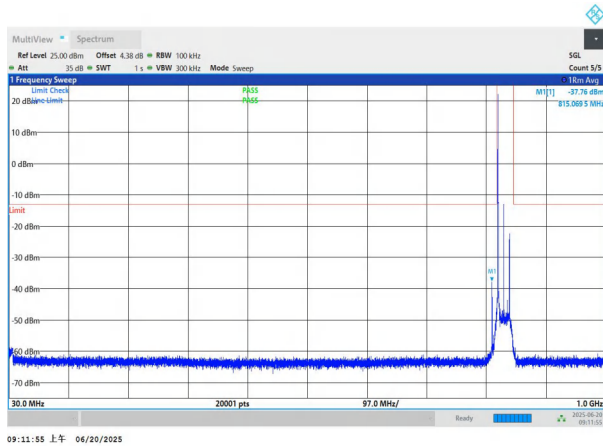
NTNV-n26(824-849)-PC3-15-20-L-DFT-QPSK-Edge_1RB_Left-3 0-1000-PASS
