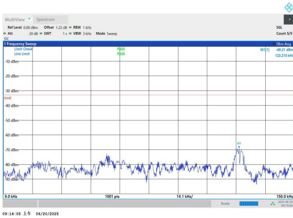
NTNV-n26(824-849)-PC3-15-20-M-DFT-QPSK-Edge_1RB_Left-0.009-0.15-PASS
