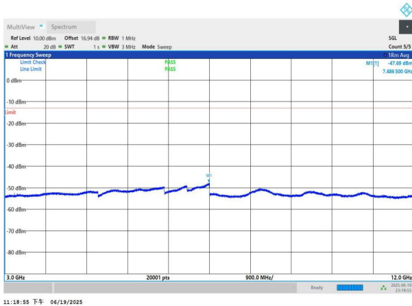
NTNV-n26(824-849)-PC3-15-10-M-DFT-QPSK-Edge_1RB_Left-3 000-12000-PASS
