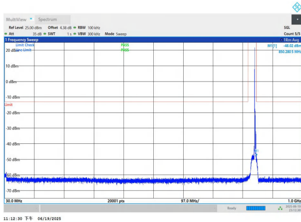
NTNV-n26(824-849)-PC3-15-5-H-DFT-QPSK-Edge_1RB_Left-30 -1000-PASS
