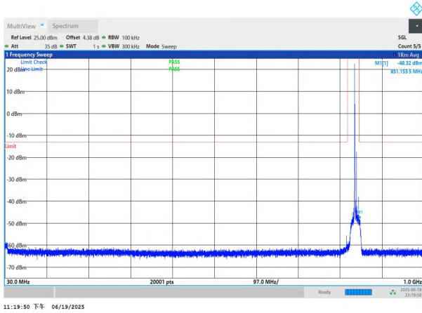
NTNV-n26(824-849)-PC3-15-10-H-DFT-BPSK-Edge_1RB_Left-3 0-1000-PASS
