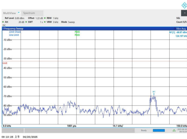
NTNV-n26(824-849)-PC3-15-20-L-DFT-BPSK-Edge_1RB_Left-0. 009-0.15-PASS
