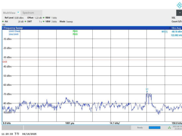
NTNV-n26(824-849)-PC3-15-10-H-DFT-QPSK-Edge_1RB_Left-0 .009-0.15-PASS
