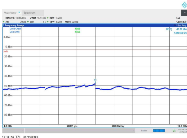
NTNV-n26(824-849)-PC3-15-5-H-DFT-QPSK-Edge_1RB_Left-30 00-12000-PASS
