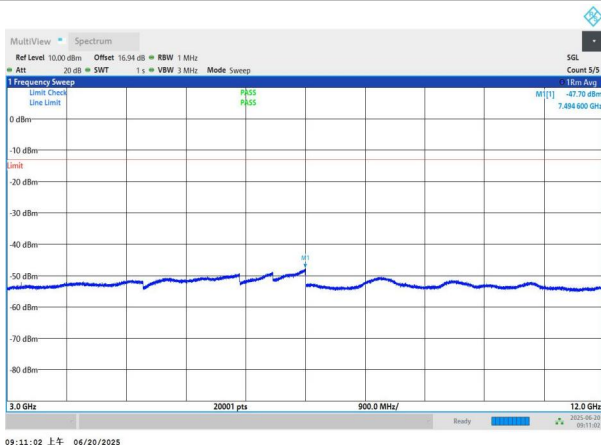
NTNV-n26(824-849)-PC3-15-20-L-DFT-BPSK-Edge_1RB_Left-3 000-12000-PASS
