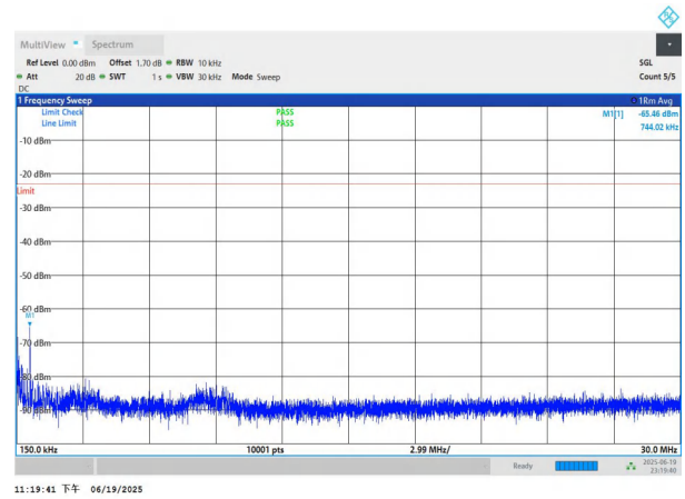
NTNV-n26(824-849)-PC3-15-10-H-DFT-BPSK-Edge_1RB_Left-0. 15-30-PASS
