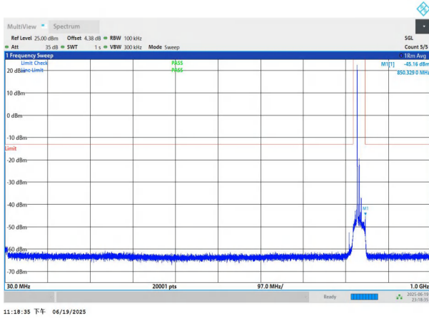
NTNV-n26(824-849)-PC3-15-10-M-DFT-QPSK-Edge_1RB_Left-3 0-1000-PASS
