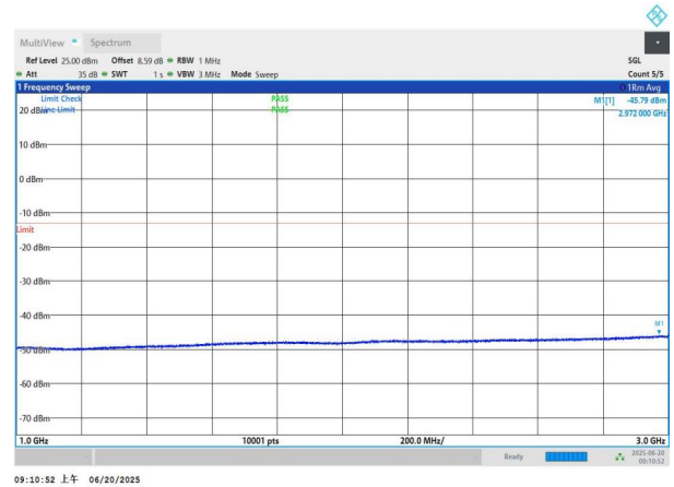
NTNV-n26(824-849)-PC3-15-20-L-DFT-BPSK-Edge_1RB_Left-10 00-3000-PASS
