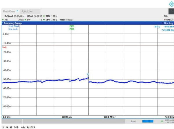
NTNV-n26(824-849)-PC3-15-15-M-DFT-BPSK-Edge_1RB_Left-3 000-12000-PASS
