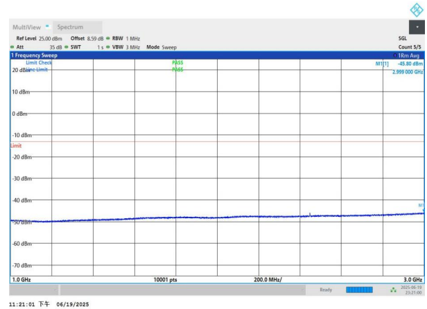
NTNV-n26(824-849)-PC3-15-10-H-DFT-QPSK-Edge_1RB_Left-10 00-3000-PASS
