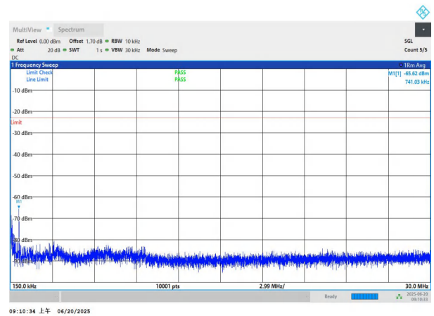
NTNV-n26(824-849)-PC3-15-20-L-DFT-BPSK-Edge_1RB_Left-0.1 5-30-PASS
