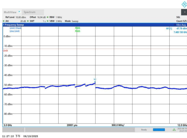
NTNV-n26(824-849)-PC3-15-15-H-DFT-BPSK-Edge_1RB_Left-3000-12000-PASS
