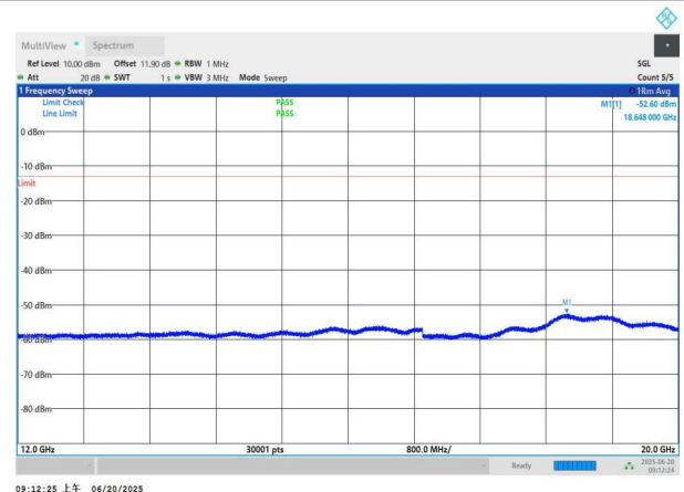
NTNV-n26(824-849)-PC3-15-20-L-DFT-QPSK-Edge_1RB_Left-12 000-20000-PASS
