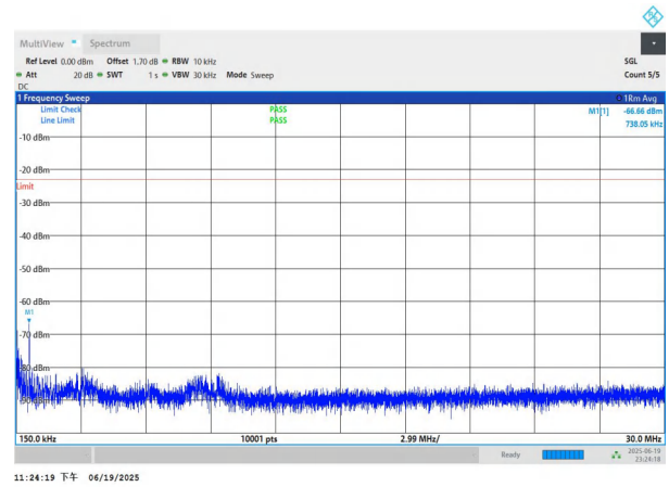
NTNV-n26(824-849)-PC3-15-15-M-DFT-BPSK-Edge_1RB_Left-0. 15-30-PASS
