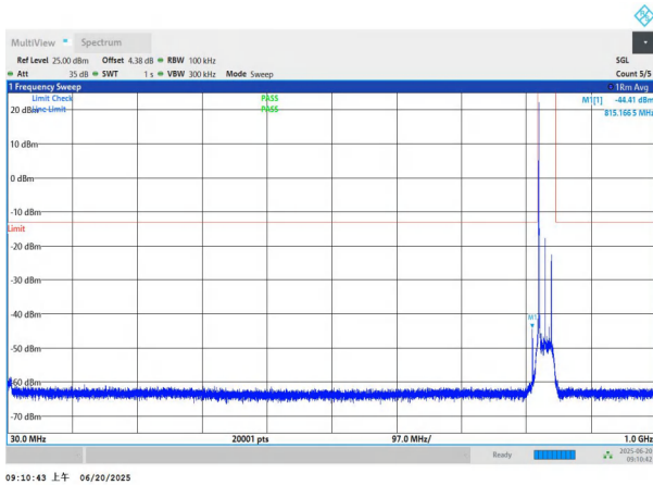
NTNV-n26(824-849)-PC3-15-20-L-DFT-BPSK-Edge_1RB_Left-3 0-1000-PASS
