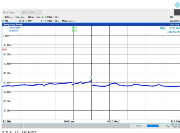
NTNV-n26(824-849)-PC3-15-10-H-DFT-QPSK-Edge_1RB_Left-3 000-12000-PASS
