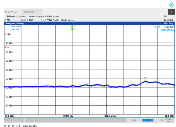
NTNV-n26(824-849)-PC3-15-20-L-DFT-BPSK-Edge_1RB_Left-12 000-20000-PASS
