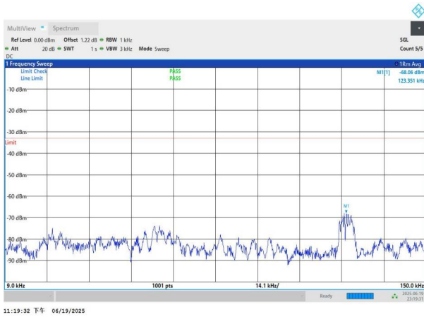
NTNV-n26(824-849)-PC3-15-10-H-DFT-BPSK-Edge_1RB_Left-0. 009-0.15-PASS
