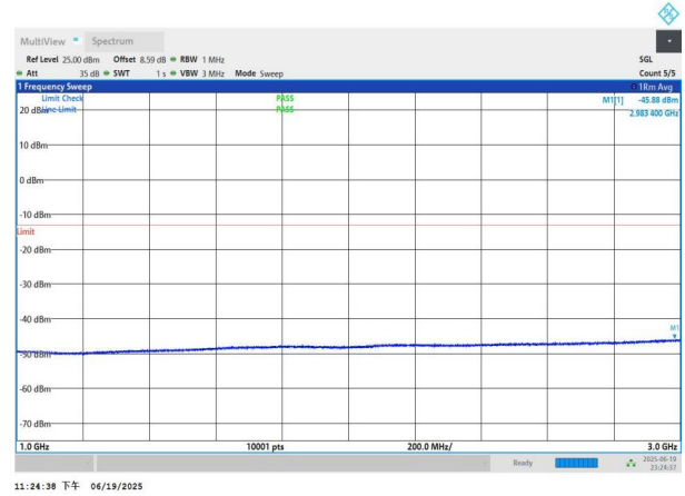
NTNV-n26(824-849)-PC3-15-15-M-DFT-BPSK-Edge_1RB_Left-10 00-3000-PASS
