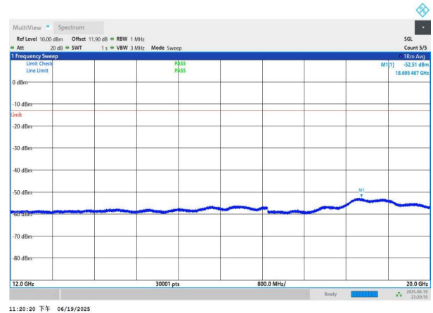
NTNV-n26(824-849)-PC3-15-10-H-DFT-BPSK-Edge_1RB_Left-12 000-20000-PASS
