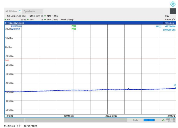
NTNV-n26(824-849)-PC3-15-5-H-DFT-QPSK-Edge_1RB_Left-100 0-3000-PASS
