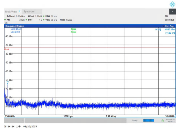
NTNV-n26(824-849)-PC3-15-20-M-DFT-QPSK-Edge_1RB_Left-0.15-30-PASS
