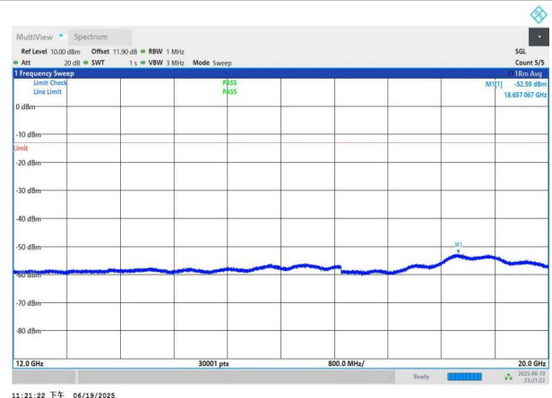
NTNV-n26(824-849)-PC3-15-10-H-DFT-QPSK-Edge_1RB_Left-12 000-20000-PASS
