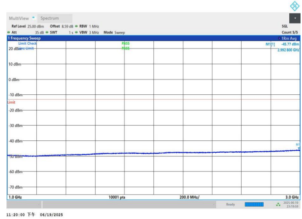
NTNV-n26(824-849)-PC3-15-10-H-DFT-BPSK-Edge_1RB_Left-10 00-3000-PASS
