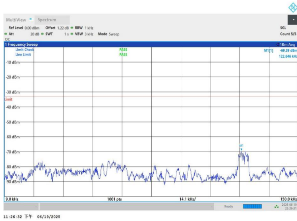
NTNV-n26(824-849)-PC3-15-15-H-DFT-BPSK-Edge_1RB_Left-0.009-0.15-PASS
