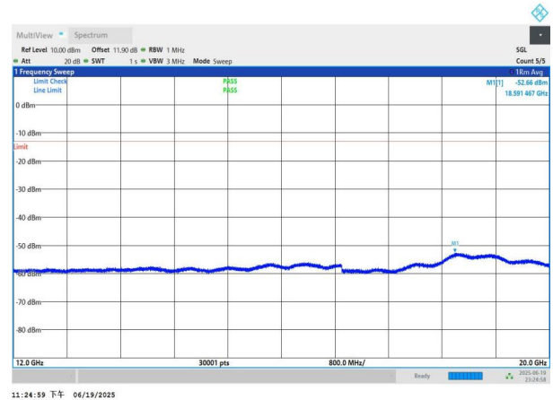
NTNV-n26(824-849)-PC3-15-15-M-DFT-BPSK-Edge_1RB_Left-12 000-20000-PASS
