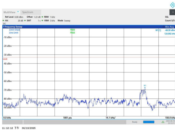
NTNV-n26(824-849)-PC3-15-5-H-DFT-QPSK-Edge_1RB_Left-0. 009-0.15-PASS
