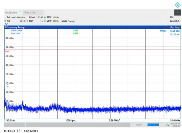
NTNV-n26(824-849)-PC3-15-10-H-DFT-QPSK-Edge_1RB_Left-0. 15-30-PASS
