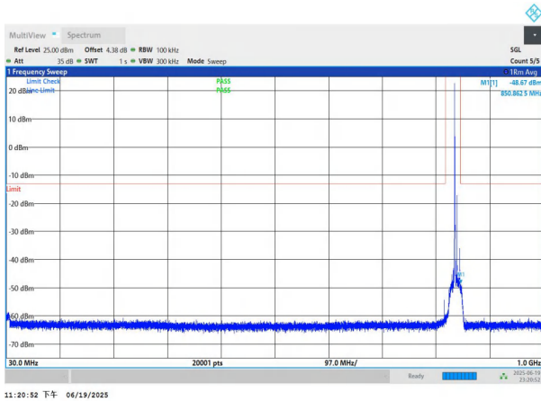
NTNV-n26(824-849)-PC3-15-10-H-DFT-QPSK-Edge_1RB_Left-3 0-1000-PASS
