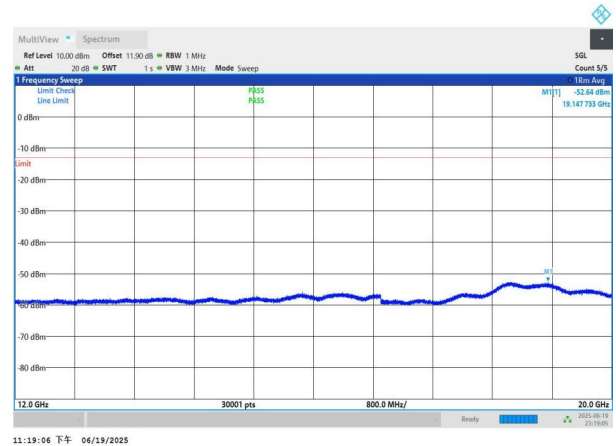
NTNV-n26(824-849)-PC3-15-10-M-DFT-QPSK-Edge_1RB_Left-12 000-20000-PASS
