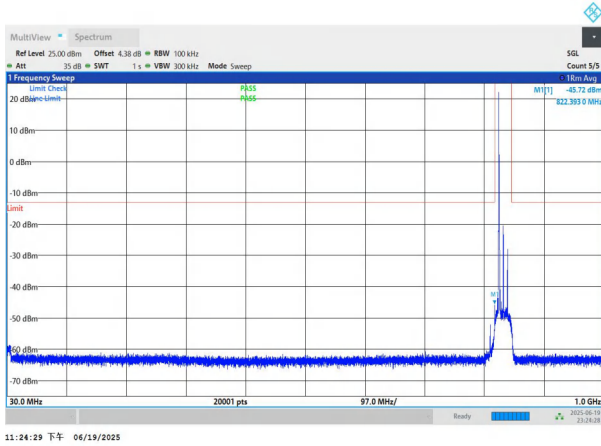
NTNV-n26(824-849)-PC3-15-15-M-DFT-BPSK-Edge_1RB_Left-3 0-1000-PASS
