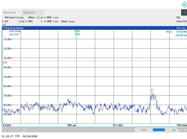
NTNV-n26(824-849)-PC3-15-10-M-DFT-QPSK-Edge_1RB_Left-0 .009-0.15-PASS
