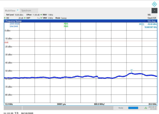
NTNV-n26(824-849)-PC3-15-5-H-DFT-QPSK-Edge_1RB_Left-120 00-20000-PASS
