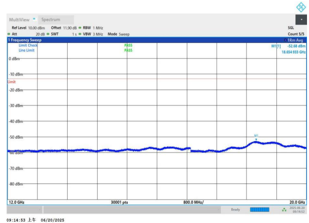
NTNV-n26(824-849)-PC3-15-20-M-DFT-QPSK-Edge_1RB_Left-12.000-20000-PASS
