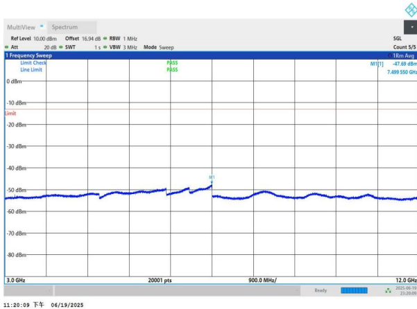
NTNV-n26(824-849)-PC3-15-10-H-DFT-BPSK-Edge_1RB_Left-3 000-12000-PASS
