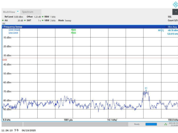
NTNV-n26(824-849)-PC3-15-15-M-DFT-BPSK-Edge_1RB_Left-0 .009-0.15-PASS
