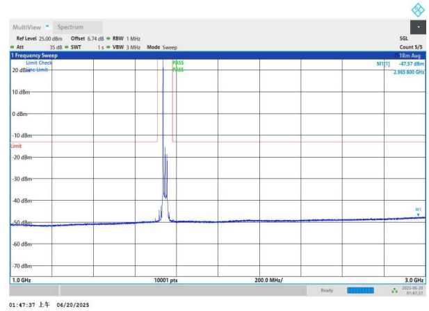
NTNV-n66-PC3-15-20-M-DFT-BPSK-Edge_1RB_Left-1000-3000- PASS
