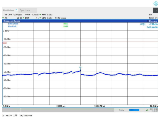
NTNV-n66-PC3-15-10-H-DFT-QPSK-Edge_1RB_Left-3000-1200 0-PASS
