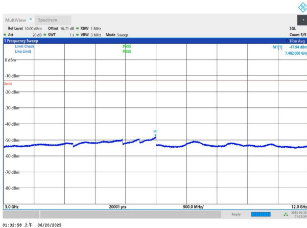
NTNV-n66-PC3-15-10-M-DFT-BPSK-Edge_1RB_Left-3000-1200 0-PASS
