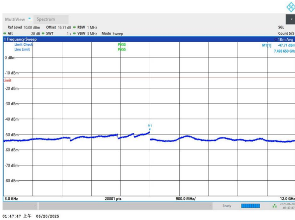
NTNV-n66-PC3-15-20-M-DFT-BPSK-Edge_1RB_Left-3000-1200 0-PASS
