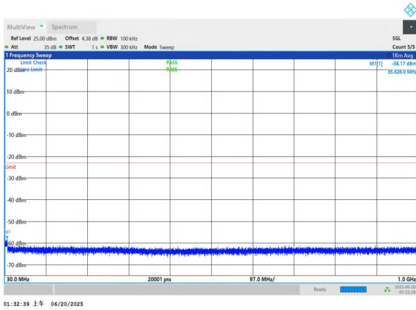
NTNV-n66-PC3-15-10-M-DFT-BPSK-Edge_1RB_Left-30-1000-P ASS
