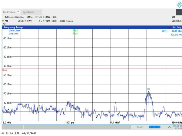
NTNV-n66-PC3-15-10-M-DFT-BPSK-Edge_1RB_Left-0.009-0.15- PASS
