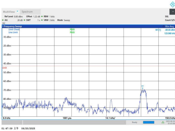
NTNV-n66-PC3-15-20-M-DFT-BPSK-Edge_1RB_Left-0.009-0.15- PASS
