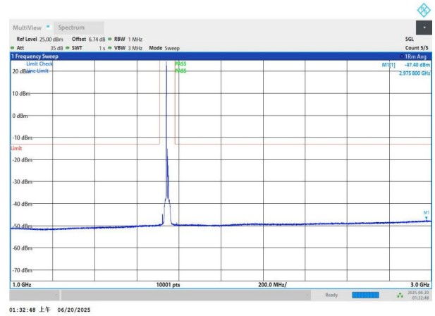
NTNV-n66-PC3-15-10-M-DFT-BPSK-Edge_1RB_Left-1000-3000- PASS
