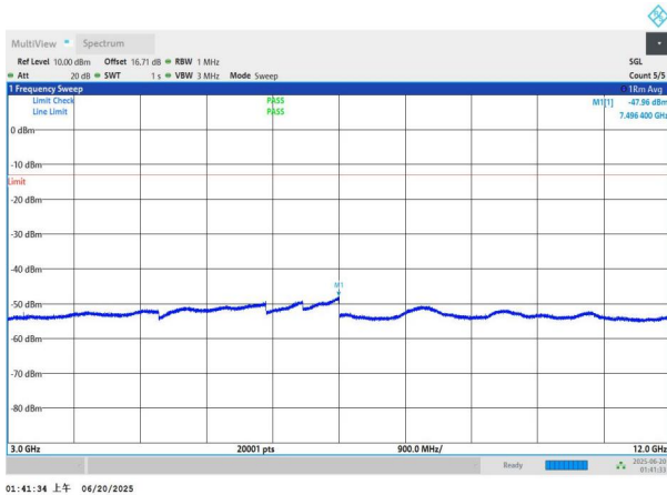
NTNV-n66-PC3-15-15-M-DFT-QPSK-Edge_1RB_Left-3000-1200 0-PASS
