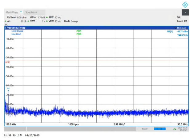
NTNV-n66-PC3-15-10-M-DFT-BPSK-Edge_1RB_Left-0.15-30-PA SS
