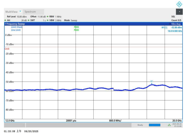
NTNV-n66-PC3-15-10-M-DFT-BPSK-Edge_1RB_Left-12000-2000 0-PASS
