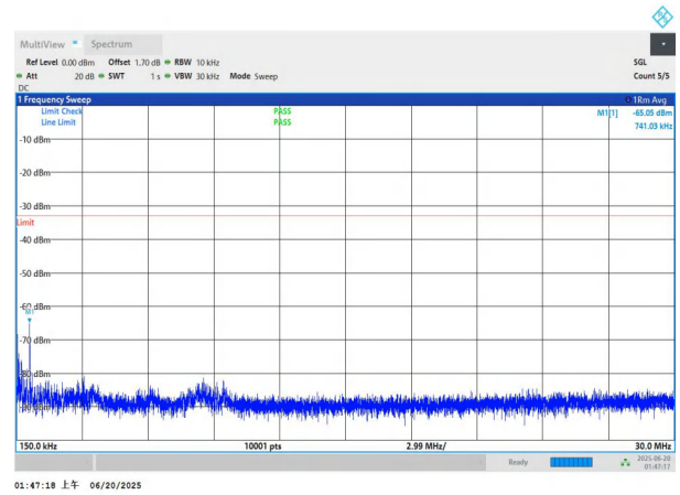
NTNV-n66-PC3-15-20-M-DFT-BPSK-Edge_1RB_Left-0.15-30-PA SS
